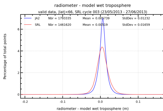
FIGURE 12 – Histogram of wet troposphere differences between radiometer and ECMWF model for cycle 003.
