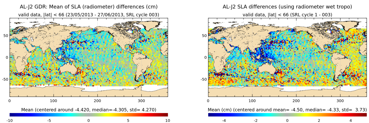
FIGURE 20 – Saral/AltiKa – Jason-2 SLA differences for cycle 003 (left) and averaged over the whole Saral/AltiKa period (right)
