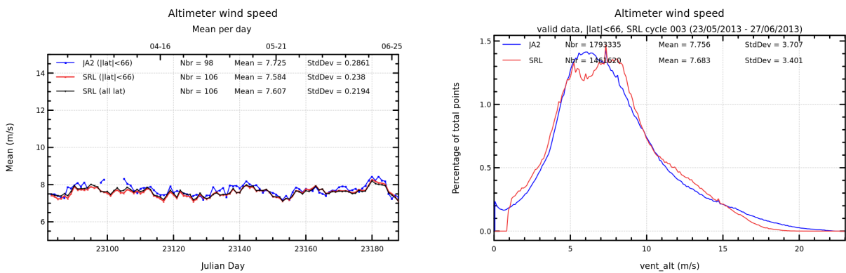
FIGURE 10 – Daily monitoring of altimeter wind speed for Saral/AltiKa and Jason-2 on the left and histogram for cycle 003 on the right (limited to 66° latitude).
