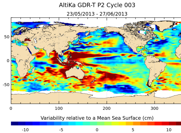
FIGURE 18 – Sea level anomaly relative to MSS for cycle 003.
