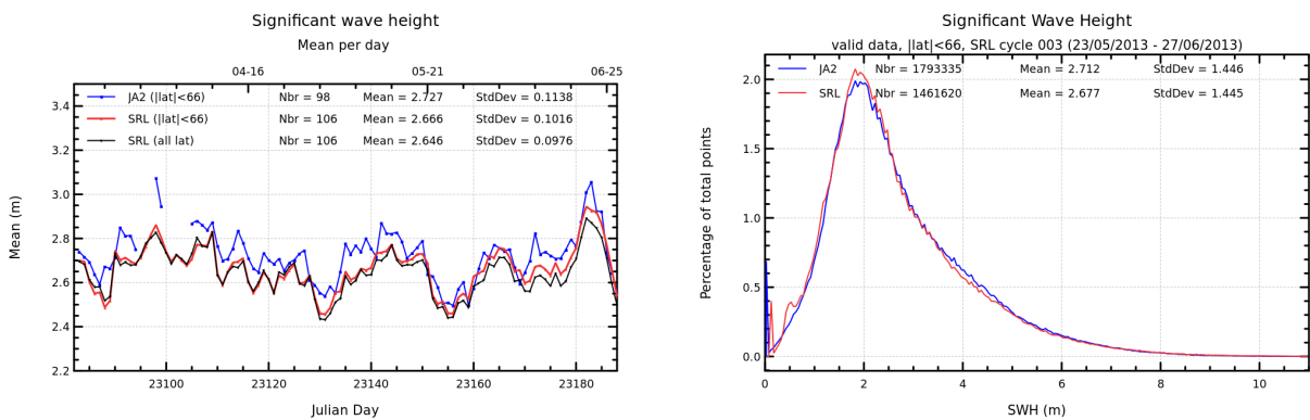
FIGURE 6 – Daily monitoring of significant wave height for AltiKa (Ka-band) and Jason-2 (Ku-band) on the left and histogram for cycle 003 on the right (limited to 66° latitude).
