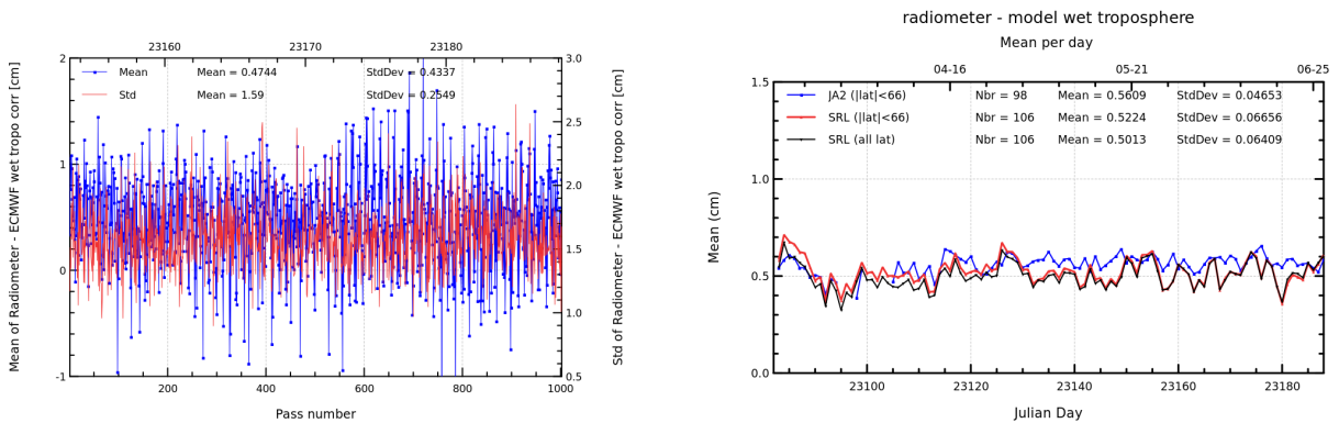
FIGURE 11 – Pass monitoring of wet troposphere differences between radiometer and ECMWF model for Saral/AltiKa cycle 003 (left) and daily monitoring of wet troposphere differences between radiometer and ECMWF model (right).
