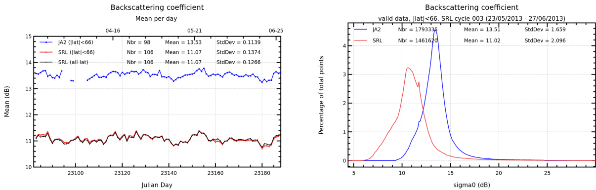
FIGURE 7 – Daily monitoring of backscattering coefficient for Saral/AltiKa and Jason-2 on the left and histogram for cycle 003 on the right (limited to 66° latitude).
