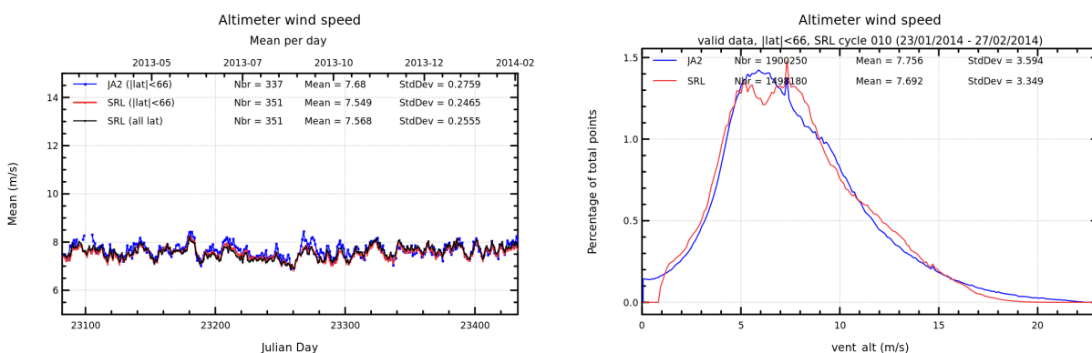
FIGURE 10 – Daily monitoring of altimeter wind speed for Saral/AltiKa and Jason-2 on the left and histogram for cycle 010 on the right (limited to 66° latitude).
