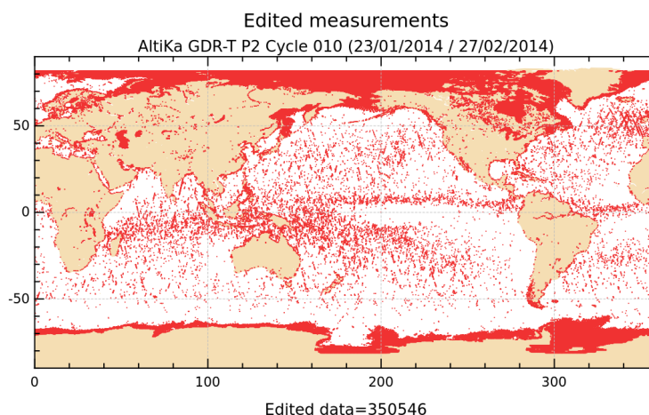
FIGURE 2 – Edited measurements for cycle 010.
