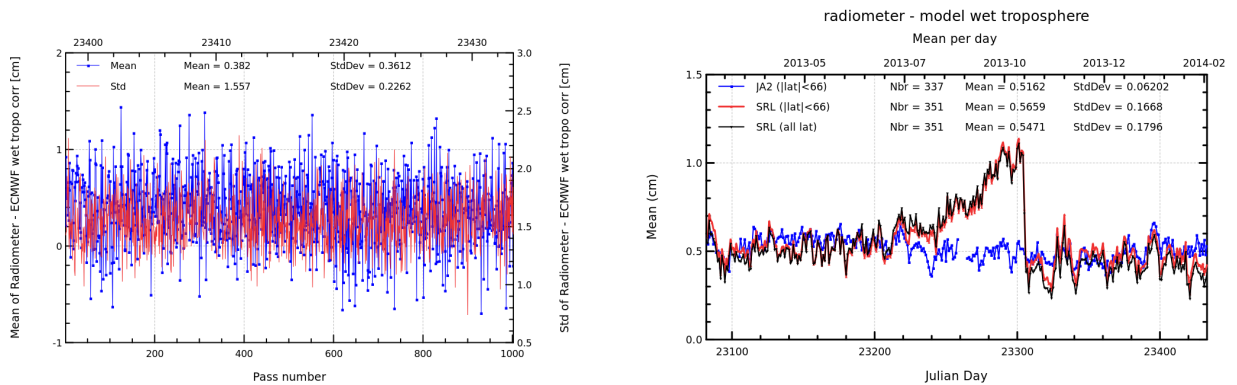
FIGURE 11 – Pass monitoring of wet troposphere differences between radiometer and ECMWF model for Saral/AltiKa cycle 010 (left) and daily monitoring of wet troposphere differences between radiometer and ECMWF model (right).
