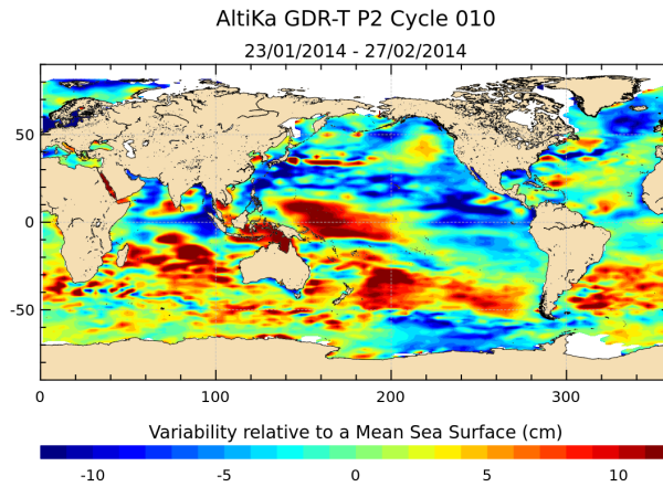
FIGURE 18 – Sea level anomaly relative to MSS for cycle 010.
