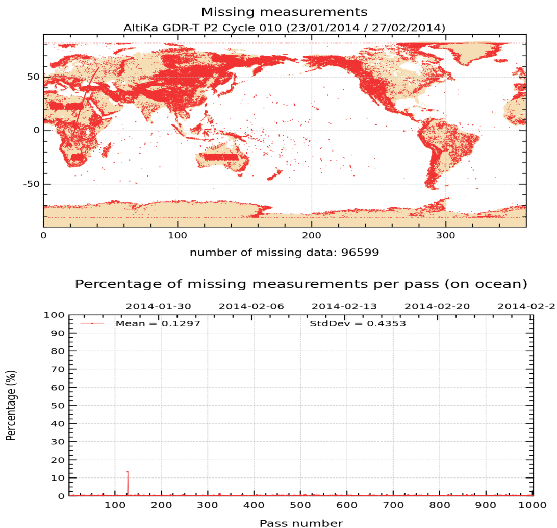
FIGURE 1 – Map of missing measurements for cycle 010 on top. Monitoring of percentage of missing ocean measurements per pass on bottom
