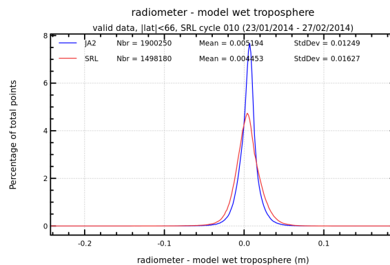
FIGURE 12 – Histogram of wet troposphere differences between radiometer and ECMWF model for cycle 010.
