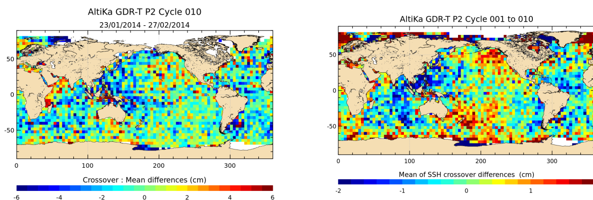
FIGURE 13 – Mean SSH at crossovers for cycle 010 (left) and over the whole Saral/AltiKa period (right).
