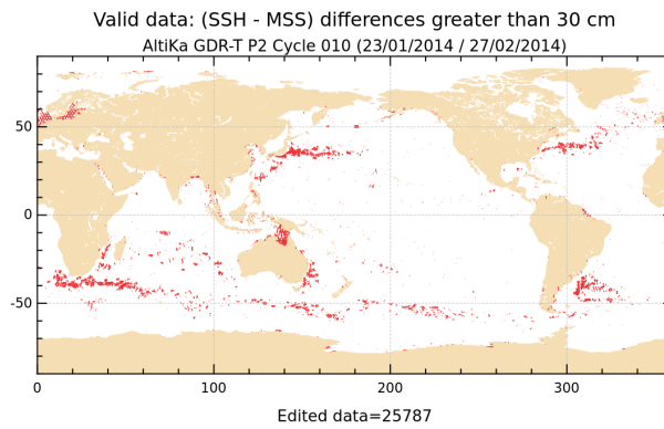
FIGURE 19 – Differences higher than a 30 cm threshold for cycle 010.
