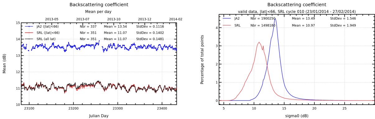
FIGURE 7 – Daily monitoring of backscattering coefficient for Saral/AltiKa and Jason-2 on the left and histogram for cycle 010 on the right (limited to 66° latitude).
