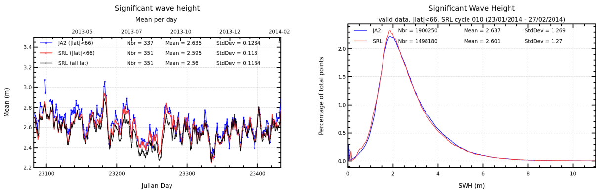
FIGURE 6 – Daily monitoring of significant wave height for AltiKa (Ka-band) and Jason-2 (Ku-band) on the left and histogram for cycle 010 on the right (limited to 66° latitude).
