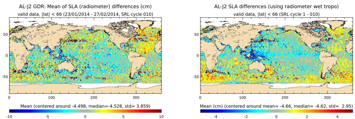
FIGURE 20 – Saral/AltiKa – Jason-2 SLA differences for cycle 010 (left) and averaged over the whole Saral/AltiKa period (right)
