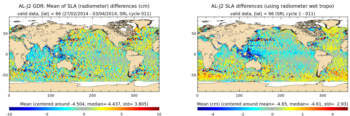
FIGURE 20 – Saral/AltiKa – Jason-2 SLA differences for cycle 011 (left) and averaged over the whole Saral/AltiKa period (right)
