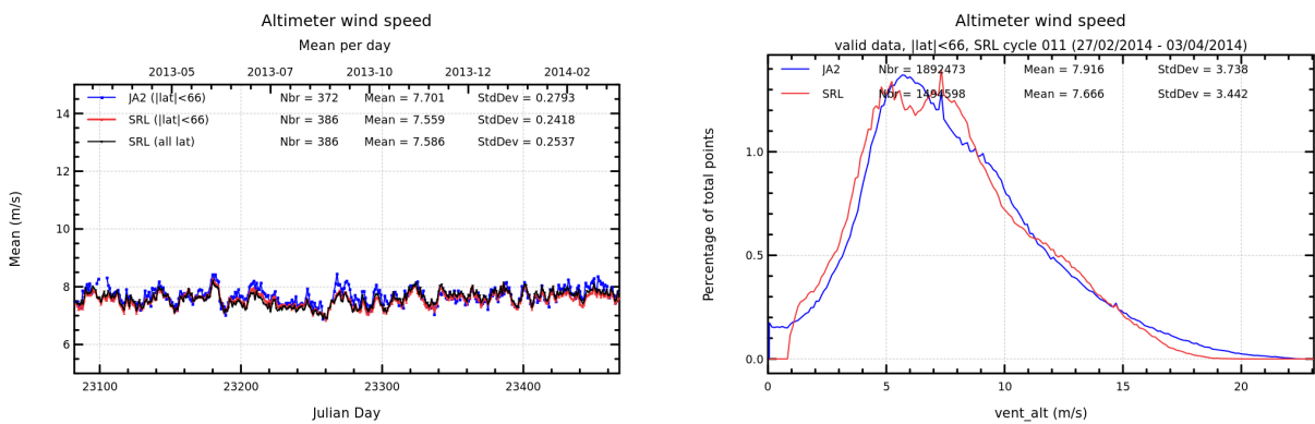
FIGURE 10 – Daily monitoring of altimeter wind speed for Saral/AltiKa and Jason-2 on the left and histogram for cycle 011 on the right (limited to 66° latitude).
