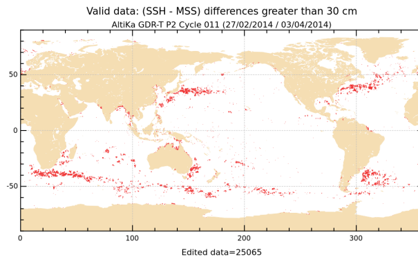
FIGURE 19 – Differences higher than a 30 cm threshold for cycle 011.
