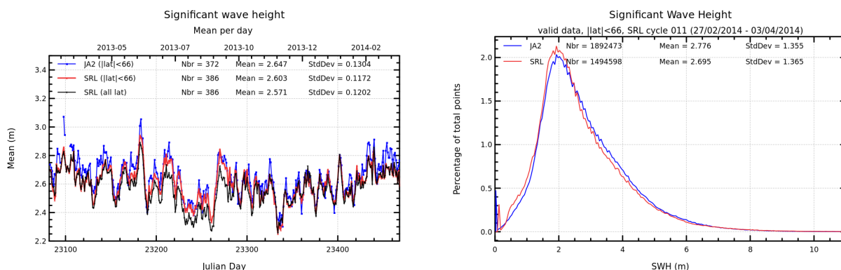
FIGURE 6 – Daily monitoring of significant wave height for AltiKa (Ka-band) and Jason-2 (Ku-band) on the left and histogram for cycle 011 on the right (limited to 66° latitude).
