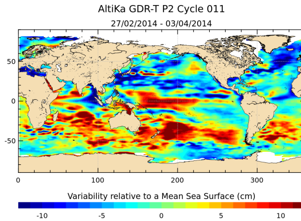
FIGURE 18 – Sea level anomaly relative to MSS for cycle 011.
