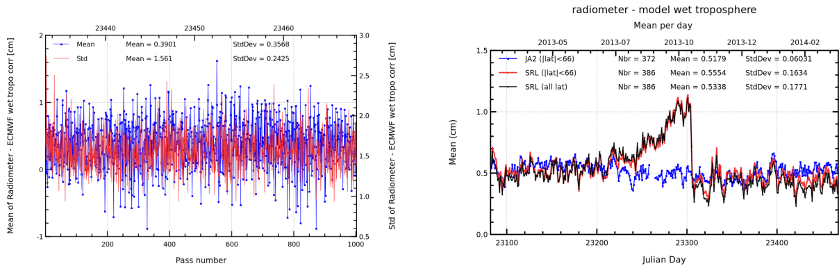
FIGURE 11 – Pass monitoring of wet troposphere differences between radiometer and ECMWF model for Saral/AltiKa cycle 011 (left) and daily monitoring of wet troposphere differences between radiometer and ECMWF model (right).
