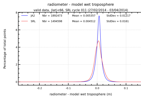
FIGURE 12 – Histogram of wet troposphere differences between radiometer and ECMWF model for cycle 011.
