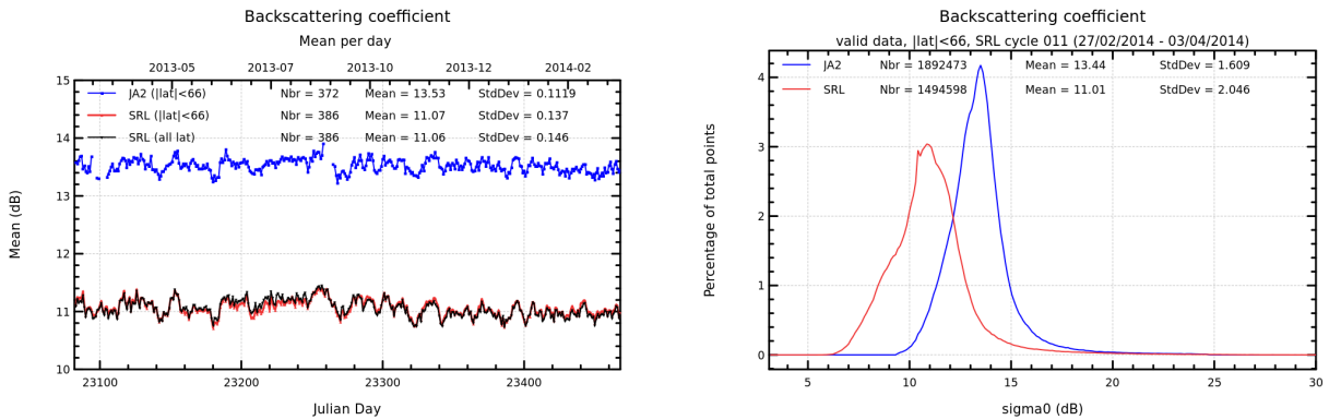
FIGURE 7 – Daily monitoring of backscattering coefficient for Saral/AltiKa and Jason-2 on the left and histogram for cycle 011 on the right (limited to 66° latitude).
