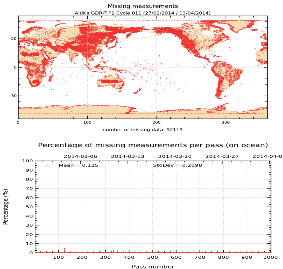
FIGURE 1 – Map of missing measurements for cycle 011 on top. Monitoring of percentage of missing ocean measurements per pass on bottom
