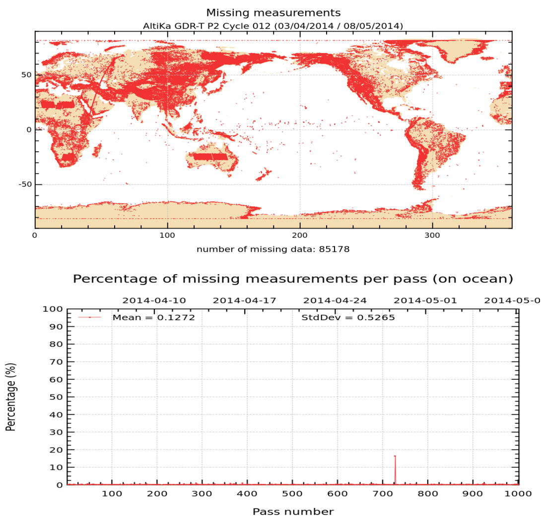
FIGURE 1 – Map of missing measurements for cycle 012 on top. Monitoring of percentage of missing ocean measurements per pass on bottom
