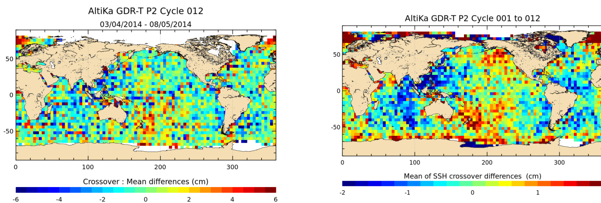
FIGURE 13 – Mean SSH at crossovers for cycle 012 (left) and over the whole Saral/AltiKa period (right).
