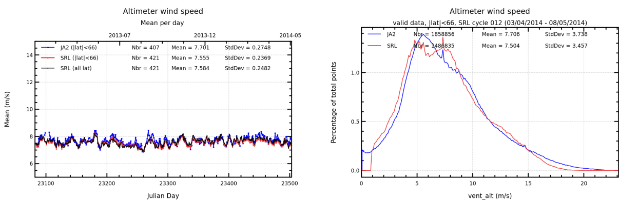
FIGURE 10 – Daily monitoring of altimeter wind speed for Saral/AltiKa and Jason-2 on the left and histogram for cycle 012 on the right (limited to 66° latitude).
