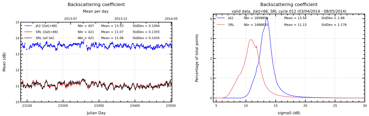
FIGURE 7 – Daily monitoring of backscattering coefficient for Saral/AltiKa and Jason-2 on the left and histogram for cycle 012 on the right (limited to 66° latitude).
