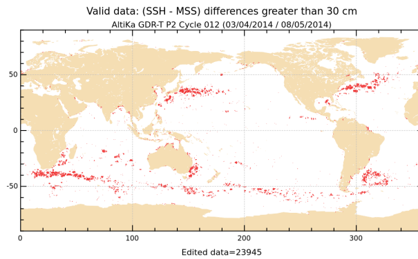
FIGURE 19 – Differences higher than a 30 cm threshold for cycle 012.
