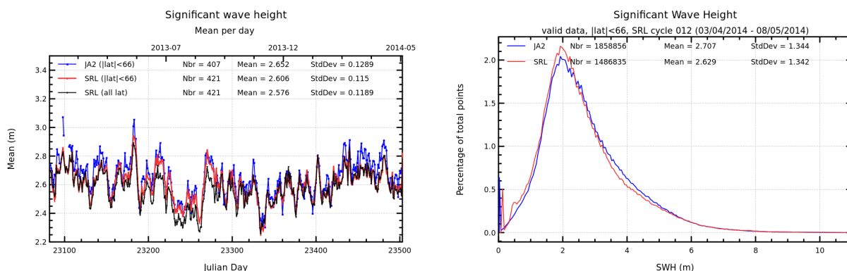
FIGURE 6 – Daily monitoring of significant wave height for AltiKa (Ka-band) and Jason-2 (Ku-band) on the left and histogram for cycle 012 on the right (limited to 66° latitude).
