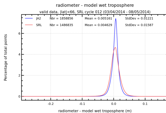
FIGURE 12 – Histogram of wet troposphere differences between radiometer and ECMWF model for cycle 012.
