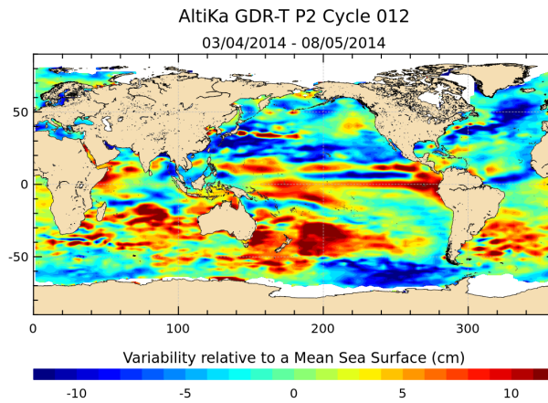
FIGURE 18 – Sea level anomaly relative to MSS for cycle 012.
