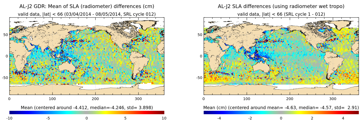
FIGURE 20 – Saral/AltiKa – Jason-2 SLA differences for cycle 012 (left) and averaged over the whole Saral/AltiKa period (right)
