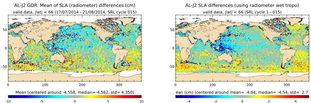
FIGURE 20 – Saral/AltiKa – Jason-2 SLA differences for cycle 015 (left) and averaged over the whole Saral/AltiKa period (right)
