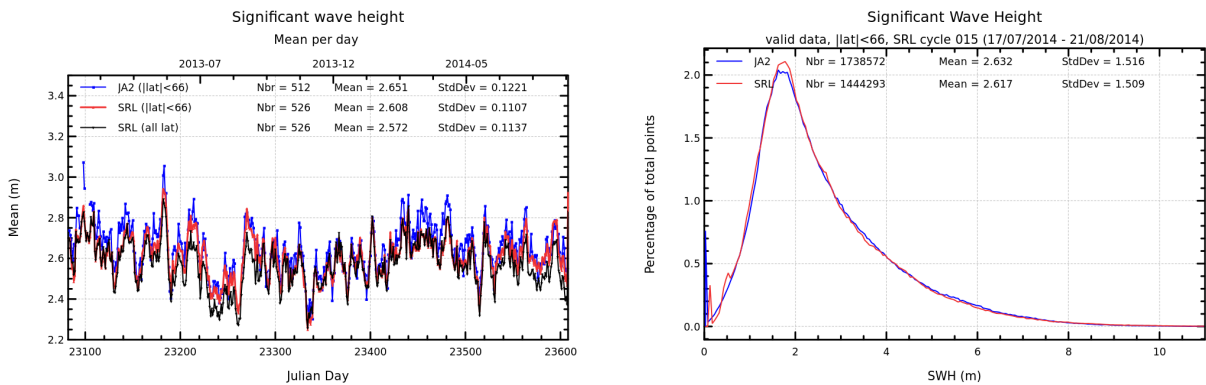
FIGURE 6 – Daily monitoring of significant wave height for AltiKa (Ka-band) and Jason-2 (Ku-band) on the left and histogram for cycle 015 on the right (limited to 66° latitude).
