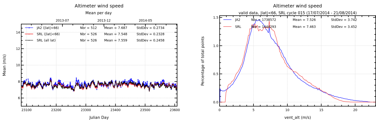
FIGURE 10 – Daily monitoring of altimeter wind speed for Saral/AltiKa and Jason-2 on the left and histogram for cycle 015 on the right (limited to 66° latitude).
