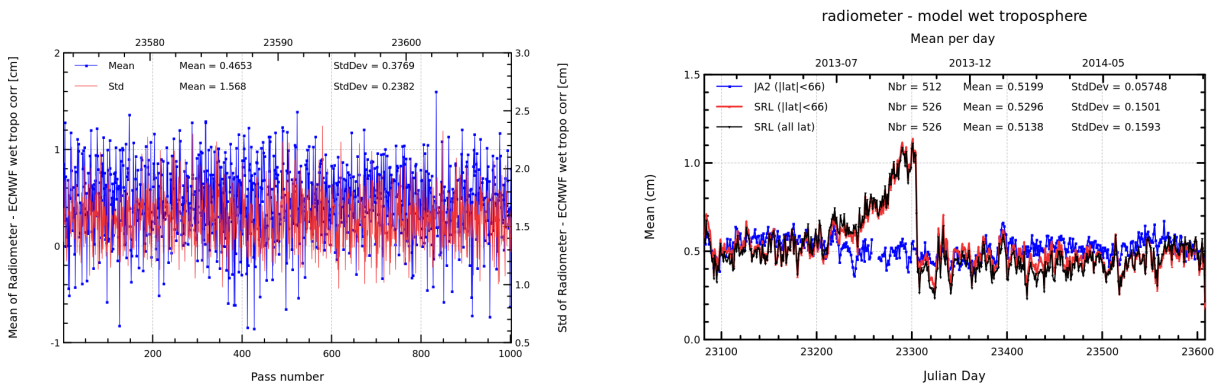
FIGURE 11 – Pass monitoring of wet troposphere differences between radiometer and ECMWF model for Saral/AltiKa cycle 015 (left) and daily monitoring of wet troposphere differences between radiometer and ECMWF model (right).
