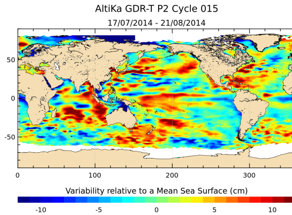
FIGURE 18 – Sea level anomaly relative to MSS for cycle 015.
