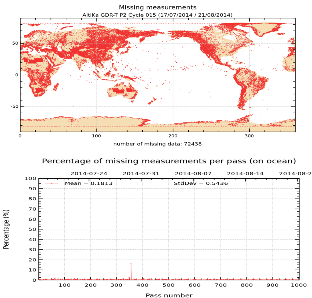
FIGURE 1 – Map of missing measurements for cycle 015 on top. Monitoring of percentage of missing ocean measurements per pass on bottom
