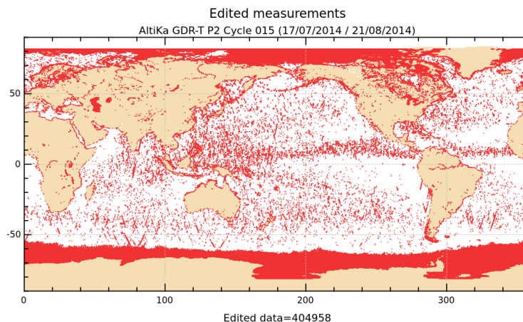
FIGURE 2 – Edited measurements for cycle 015.
