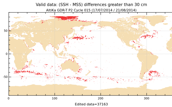
FIGURE 19 – Differences higher than a 30 cm threshold for cycle 015.
