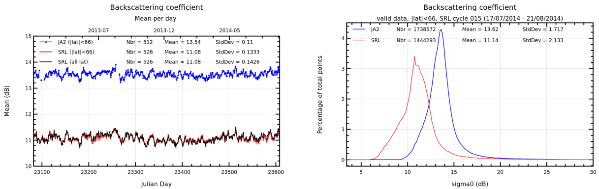
FIGURE 7 – Daily monitoring of backscattering coefficient for Saral/AltiKa and Jason-2 on the left and histogram for cycle 015 on the right (limited to 66° latitude).
