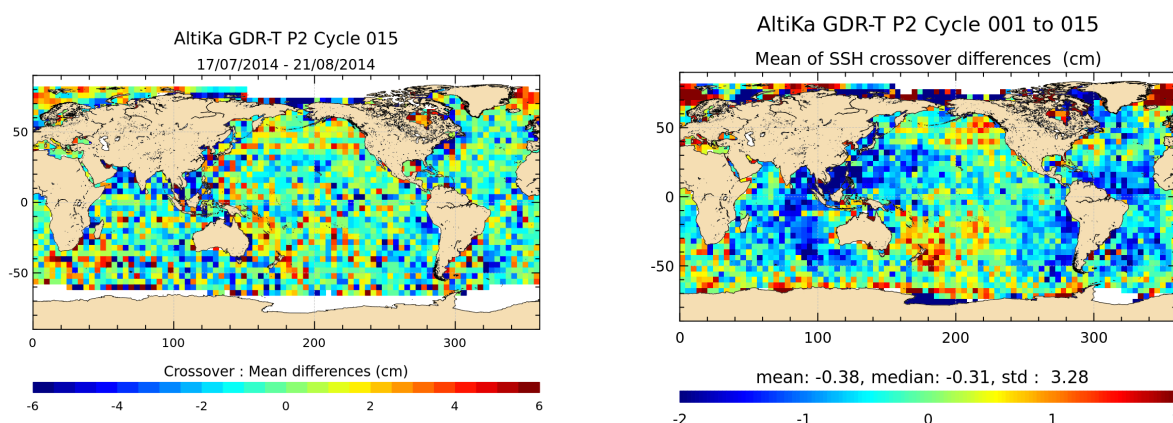
FIGURE 13 – Mean SSH at crossovers for cycle 015 (left) and over the whole Saral/AltiKa period (right).
