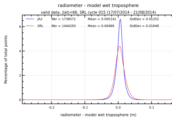
FIGURE 12 – Histogram of wet troposphere differences between radiometer and ECMWF model for cycle 015.
