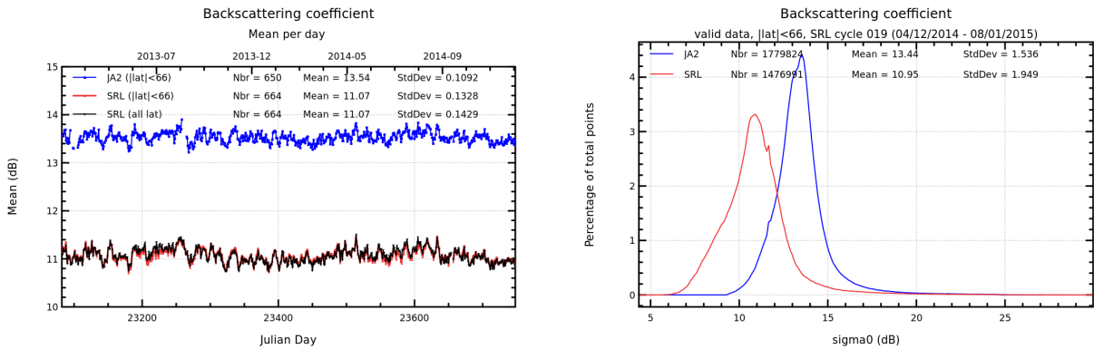
FIGURE 7 – Daily monitoring of backscattering coefficient for Saral/AltiKa and Jason-2 on the left and histogram for cycle 019 on the right (limited to 66° latitude).
