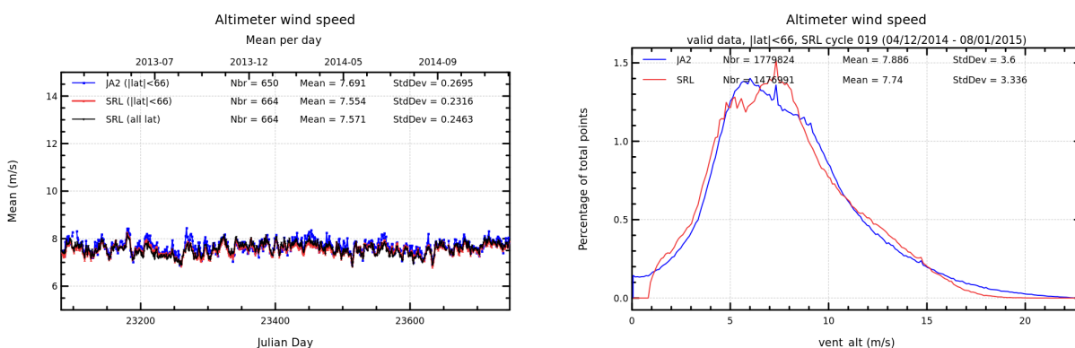
FIGURE 10 – Daily monitoring of altimeter wind speed for Saral/AltiKa and Jason-2 on the left and histogram for cycle 019 on the right (limited to 66° latitude).
