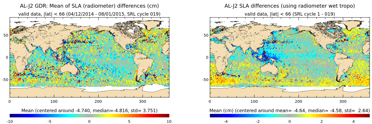
FIGURE 20 – Saral/AltiKa – Jason-2 SLA differences for cycle 019 (left) and averaged over the whole Saral/AltiKa period (right)
