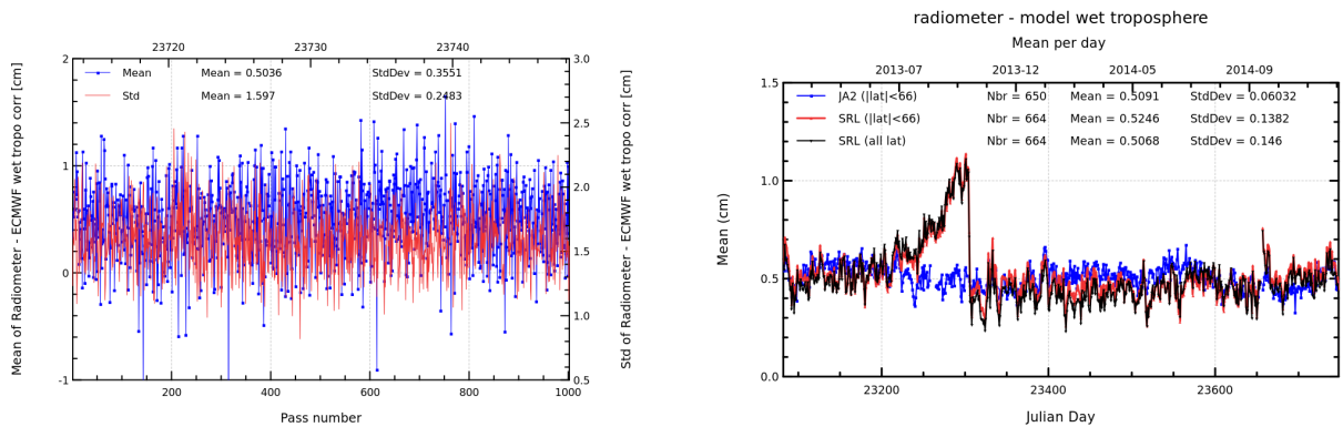
FIGURE 11 – Pass monitoring of wet troposphere differences between radiometer and ECMWF model for Saral/AltiKa cycle 019 (left) and daily monitoring of wet troposphere differences between radiometer and ECMWF model (right).
