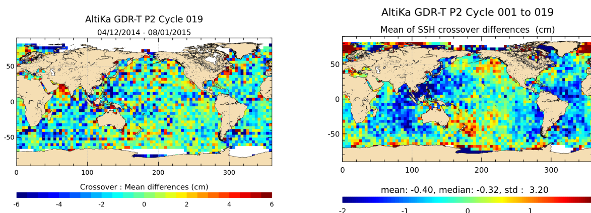
FIGURE 13 – Mean SSH at crossovers for cycle 019 (left) and over the whole Saral/AltiKa period (right).
