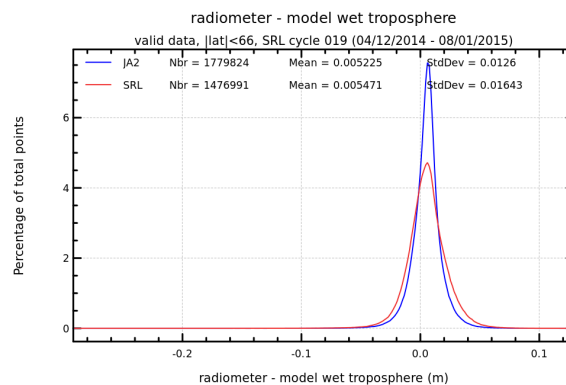
FIGURE 12 – Histogram of wet troposphere differences between radiometer and ECMWF model for cycle 019.
