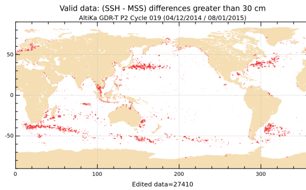
FIGURE 19 – Differences higher than a 30 cm threshold for cycle 019.
