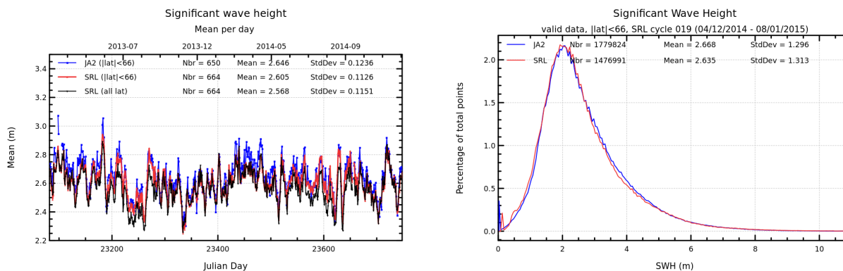
FIGURE 6 – Daily monitoring of significant wave height for AltiKa (Ka-band) and Jason-2 (Ku-band) on the left and histogram for cycle 019 on the right (limited to 66° latitude).
