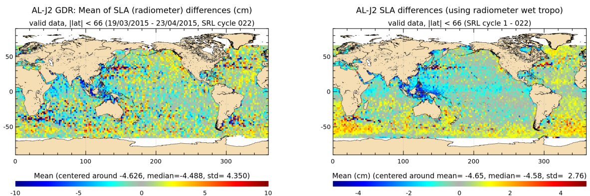
FIGURE 20 – Saral/AltiKa – Jason-2 SLA differences for cycle 022 (left) and averaged over the whole Saral/AltiKa period (right)
