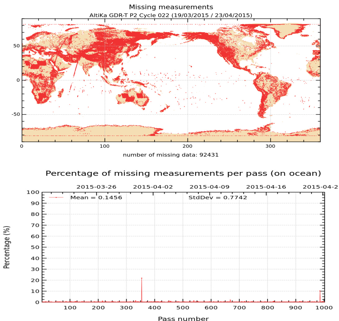
FIGURE 1 – Map of missing measurements for cycle 022 on top. Monitoring of percentage of missing ocean measurements per pass on bottom
