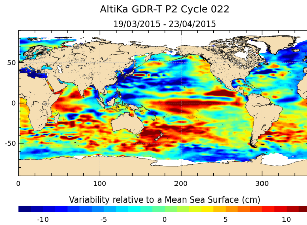
FIGURE 18 – Sea level anomaly relative to MSS for cycle 022.
