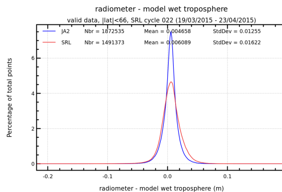
FIGURE 12 – Histogram of wet troposphere differences between radiometer and ECMWF model for cycle 022.
