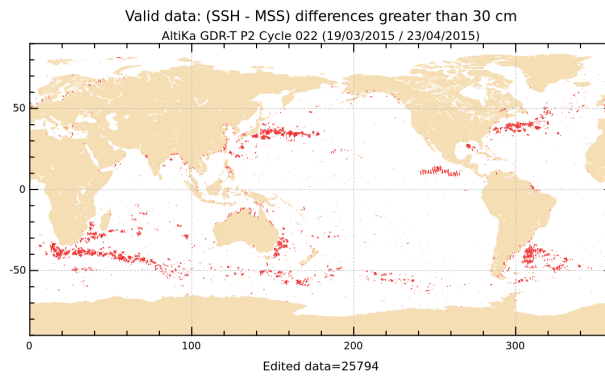
FIGURE 19 – Differences higher than a 30 cm threshold for cycle 022.
