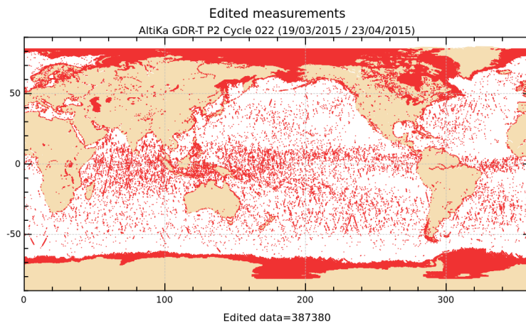
FIGURE 2 – Edited measurements for cycle 022.
