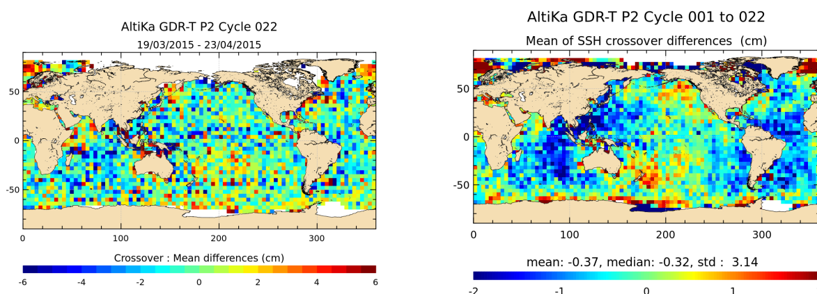
FIGURE 13 – Mean SSH at crossovers for cycle 022 (left) and over the whole Saral/AltiKa period (right).
