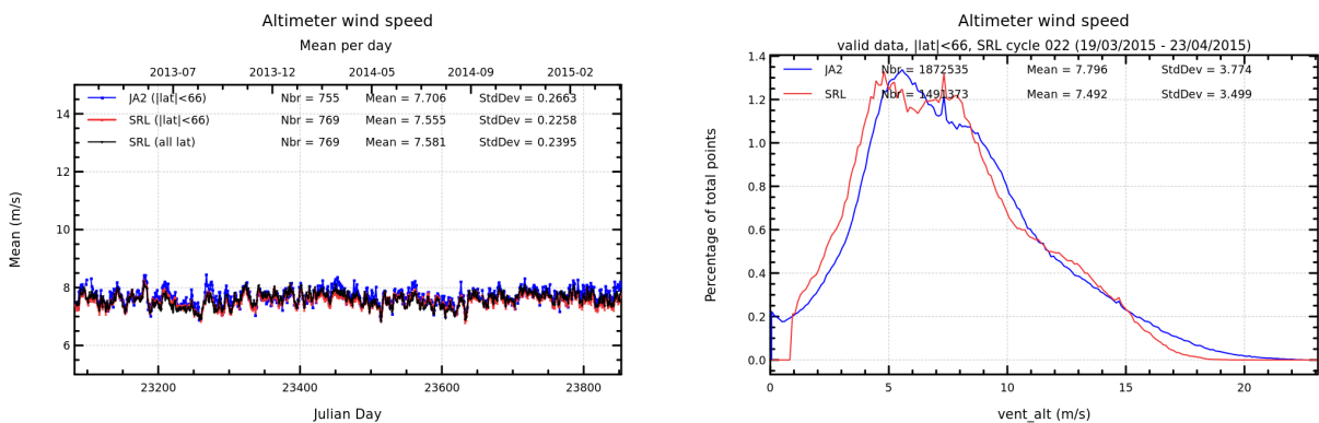
FIGURE 10 – Daily monitoring of altimeter wind speed for Saral/AltiKa and Jason-2 on the left and histogram for cycle 022 on the right (limited to 66° latitude).
