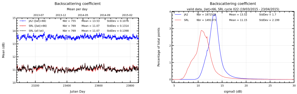
FIGURE 7 – Daily monitoring of backscattering coefficient for Saral/AltiKa and Jason-2 on the left and histogram for cycle 022 on the right (limited to 66° latitude).
