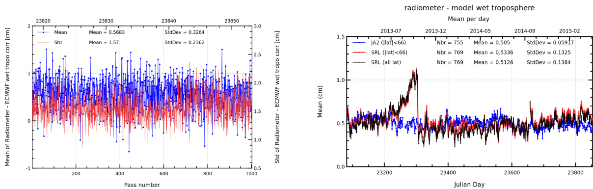
FIGURE 11 – Pass monitoring of wet troposphere differences between radiometer and ECMWF model for Saral/AltiKa cycle 022 (left) and daily monitoring of wet troposphere differences between radiometer and ECMWF model (right).
