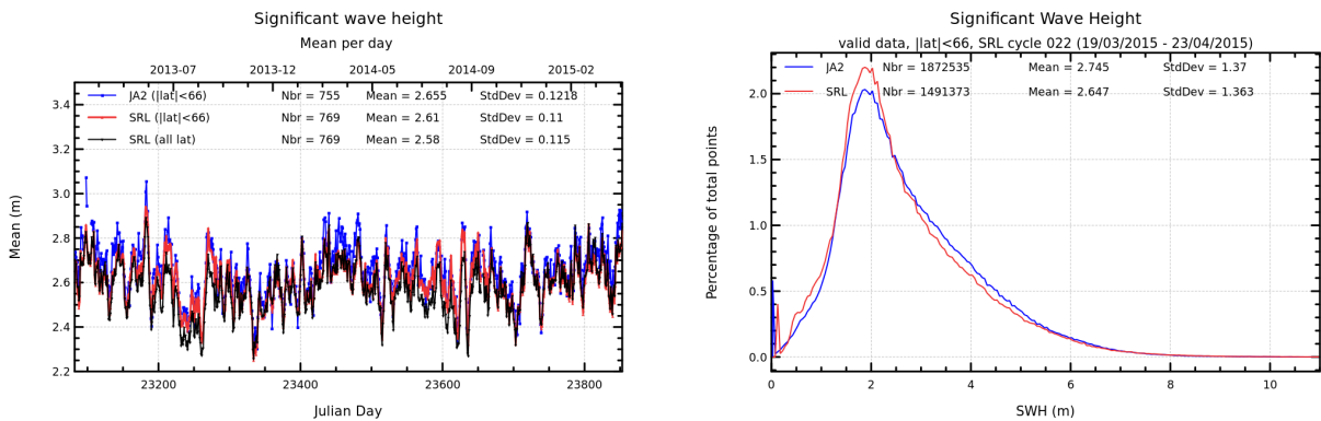
FIGURE 6 – Daily monitoring of significant wave height for AltiKa (Ka-band) and Jason-2 (Ku-band) on the left and histogram for cycle 022 on the right (limited to 66° latitude).
