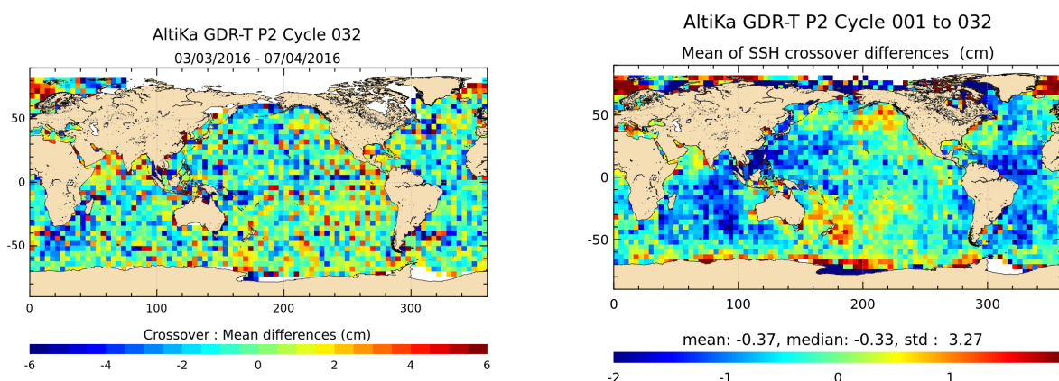
FIGURE 14 – Mean SSH at crossovers for cycle 032 (left) and over the whole Saral/AltiKa period (right).
