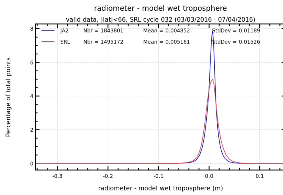
FIGURE 13 – Histogram of wet troposphere differences between radiometer and ECMWF model for cycle 032.
