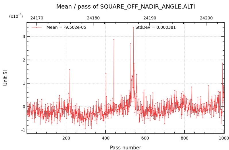
FIGURE 3 – Mispointing angle.
