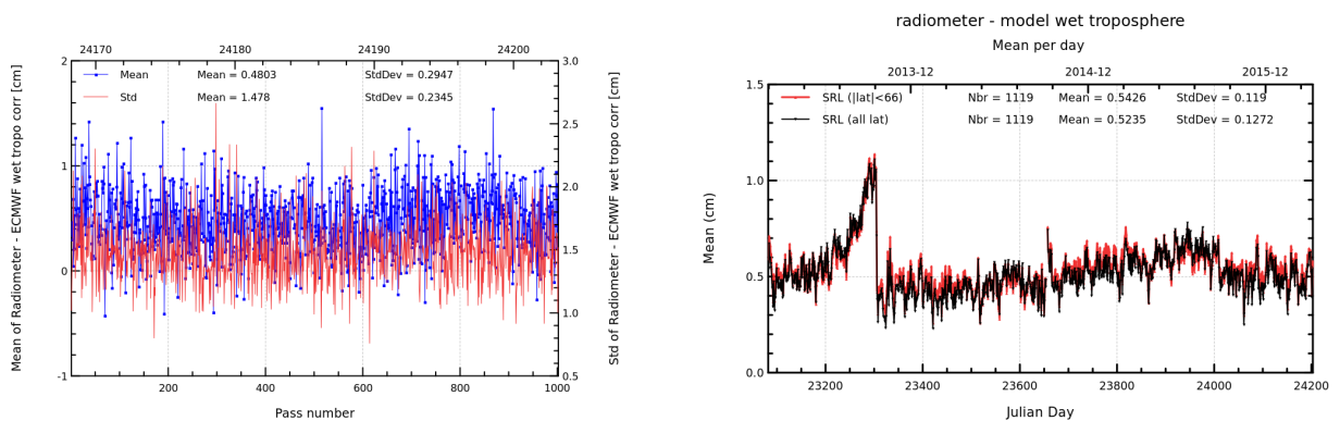
FIGURE 12 – Pass monitoring of wet troposphere differences between radiometer and ECMWF model for Saral/AltiKa cycle 032 (left) and daily monitoring of wet troposphere differences between radiometer and ECMWF model (right).
