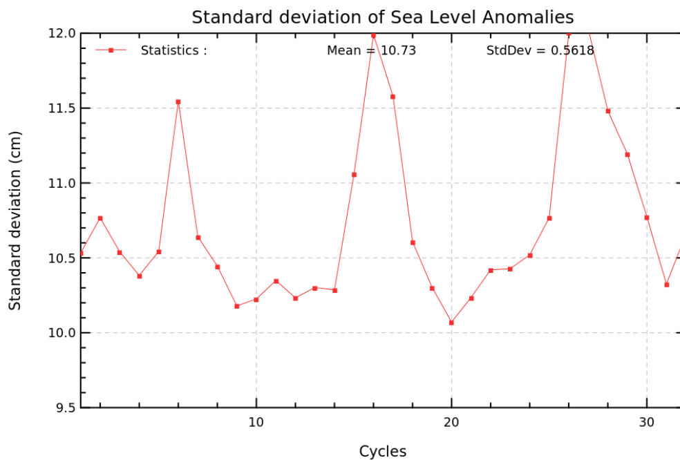
FIGURE 22 – Cyclic monitoring of standard deviation of along track SLA for Saral/AltiKa and Jason-2 (respectively 35 day and almost 10 day cycles).
