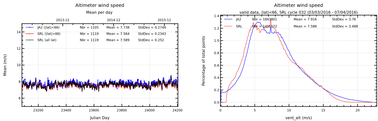
FIGURE 11 – Daily monitoring of altimeter wind speed for Saral/AltiKa and Jason-2 on the left and histogram for cycle 032 on the right (limited to 66° latitude).
