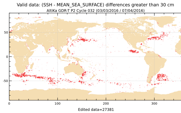
FIGURE 20 – Differences higher than a 30 cm threshold for cycle 032.
