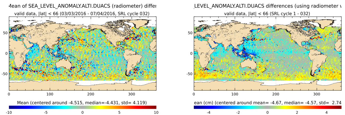
FIGURE 21 – Saral/AltiKa – Jason-2 SLA differences for cycle 032 (left) and averaged over the whole Saral/AltiKa period (right)
