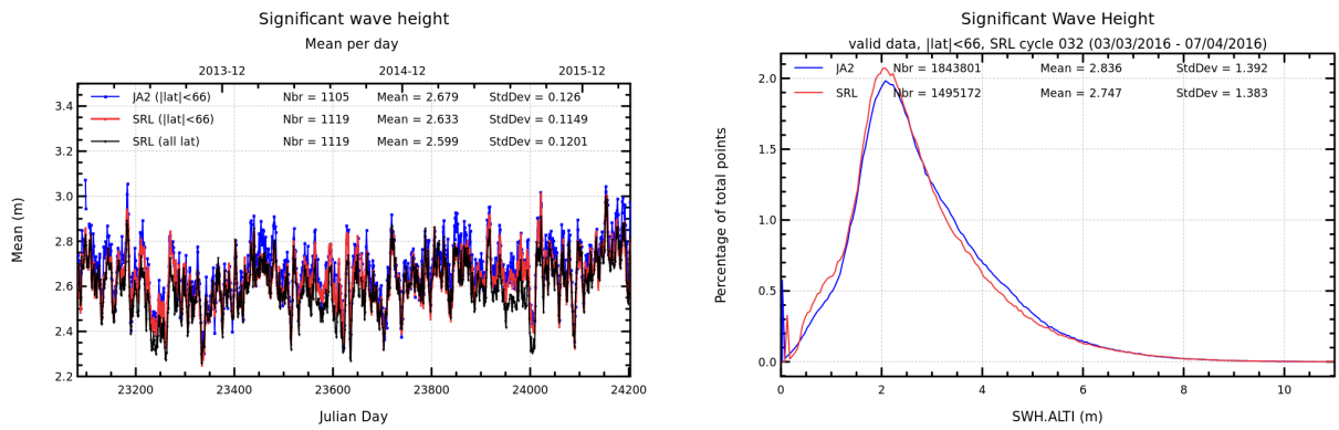
FIGURE 7 – Daily monitoring of significant wave height for AltiKa (Ka-band) and Jason-2 (Ku-band) on the left and histogram for cycle 032 on the right (limited to 66° latitude).
