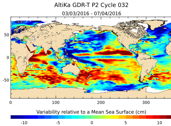
FIGURE 19 – Sea level anomaly relative to MSS for cycle 032.
