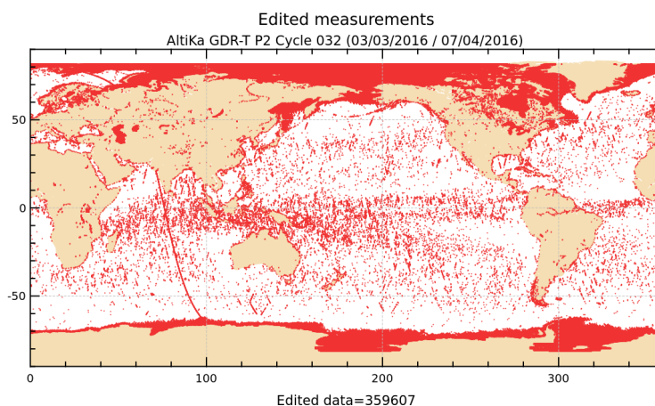
FIGURE 2 – Edited measurements for cycle 032.
