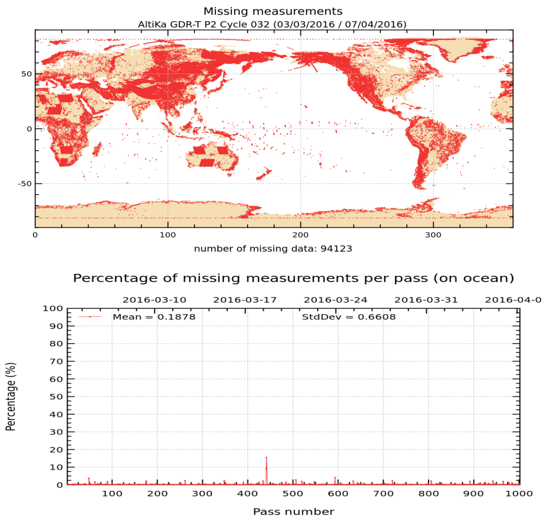
FIGURE 1 – Map of missing measurements for cycle 032 on top. Monitoring of percentage of missing ocean measurements per pass on bottom
