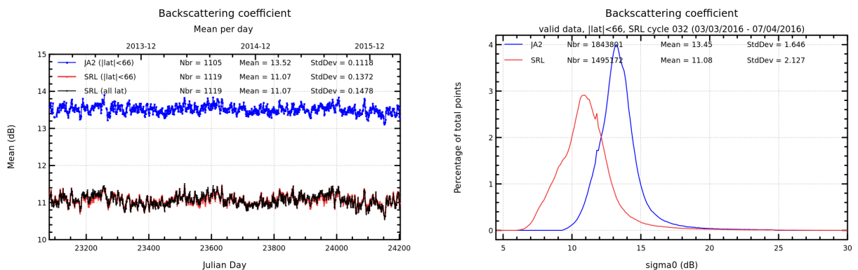
FIGURE 8 – Daily monitoring of backscattering coefficient for Saral/AltiKa and Jason-2 on the left and histogram for cycle 032 on the right (limited to 66° latitude).
