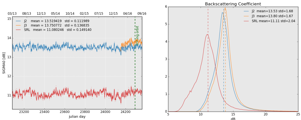
Figure 7: Daily monitoring of backscattering coefficient for Saral/AltiKa, Jason-2 and Jason-3 on the left and histogram for cycle 101 on the right (limited to 66° latitude).
