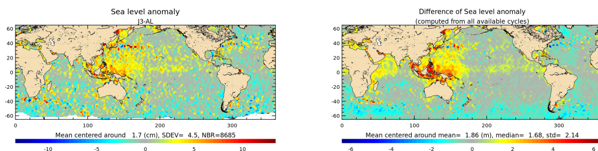
Figure 22: Jason-3 – Saral/AltiKa SLA differences for cycle 101 (left) and averaged over the whole Saral/AltiKa period (right).
