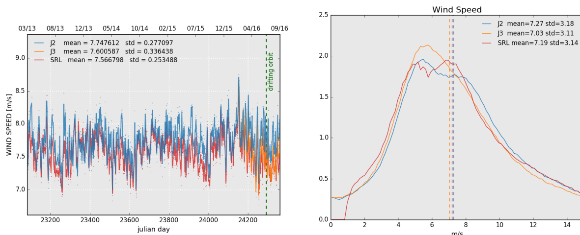
Figure 10: Daily monitoring of altimeter wind speed for Saral/AltiKa, Jason-2 and Jason-3 on the left and histogram for cycle 101 on the right (limited to 66° latitude).
