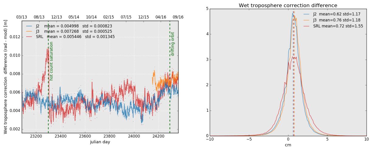
Figure 12: Daily monitoring of wet troposphere differences (Radiometer-ECMWF model) for Saral/AltiKa Jason-2 and Jason-3 (left) and histogram on the right (limited to 66° latitude) for cycle 101 .
