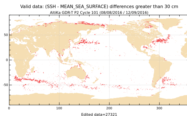
Figure 20: SLA higher than 30 cm for cycle 101.
