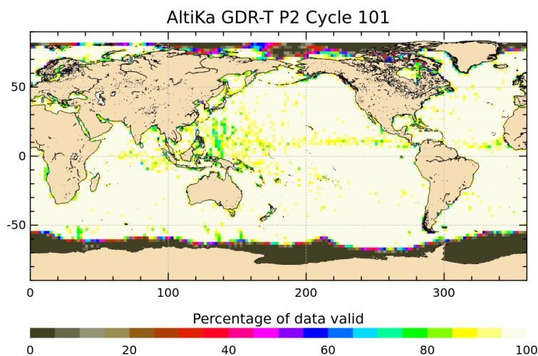
Figure 3: Percentage of valid measurements for cycle 101.
