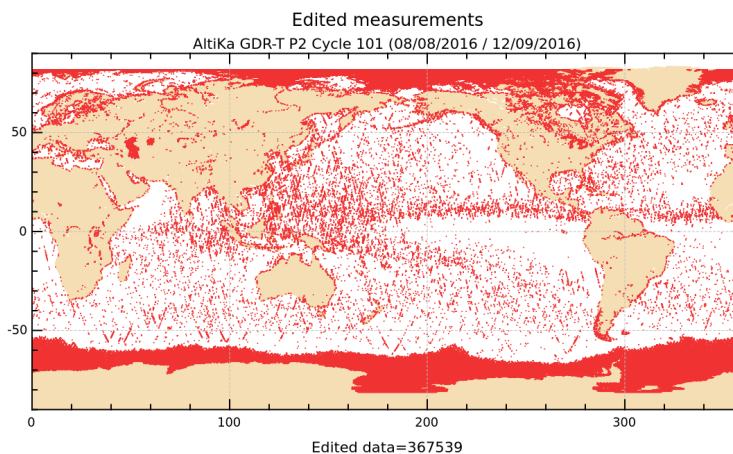
Figure 2: Edited measurements for cycle 101.
