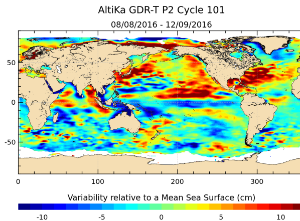
Figure 19: Sea level anomaly relative to MSS for cycle 101.
