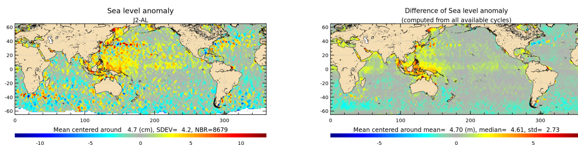
Figure 21: Jason-2 – Saral/AltiKa SLA differences for cycle 101 (left) and averaged over the whole Saral/AltiKa period (right).
