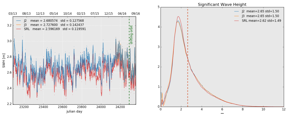
Figure 6: Daily monitoring of significant wave height for AltiKa (Ka-band) Jason-2 and Jason-3 (Ku-band) on the left and histogram for cycle 101 on the right (limited to 66^\circ latitude).
