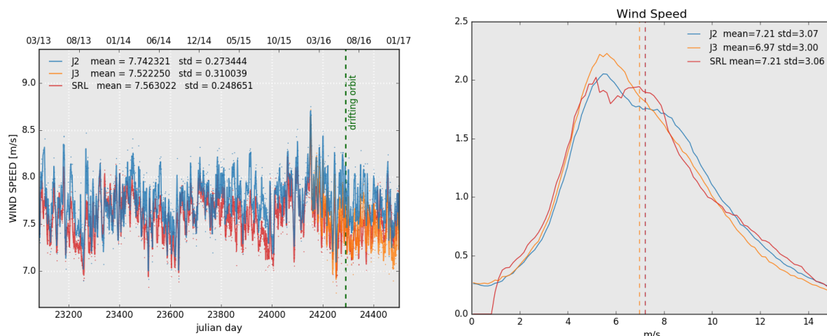
Figure 10: Daily monitoring of altimeter wind speed for Saral/AltiKa, Jason-2 and Jason-3 on the left and histogram for cycle 105 on the right (limited to 66° latitude).
