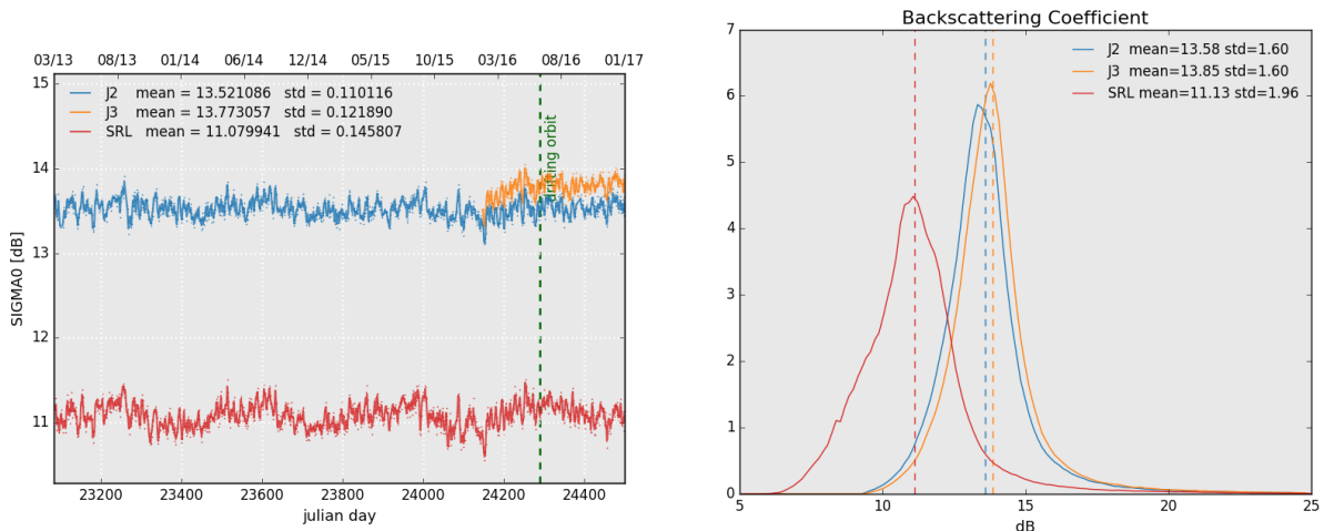
Figure 7: Daily monitoring of backscattering coefficient for Saral/AltiKa, Jason-2 and Jason-3 on the left and histogram for cycle 105 on the right (limited to 66° latitude).
