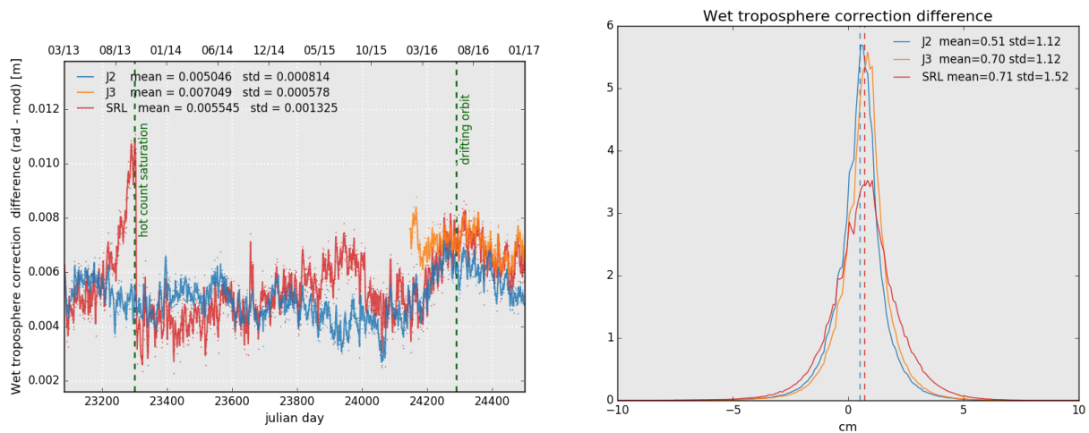
Figure 12: Daily monitoring of wet troposphere differences (Radiometer-ECMWF model) for Saral/AltiKa Jason-2 and Jason-3 (left) and histogram on the right (limited to 66° latitude) for cycle 105 .
