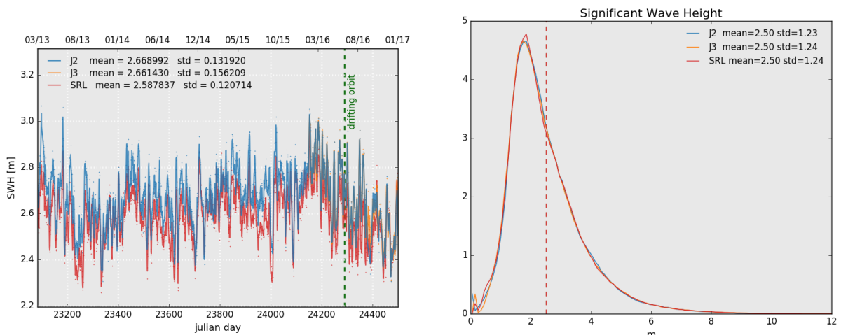
Figure 6: Daily monitoring of significant wave height for AltiKa (Ka-band) Jason-2 and Jason-3 (Ku-band) on the left and histogram for cycle 105 on the right (limited to 66^\circ latitude).
