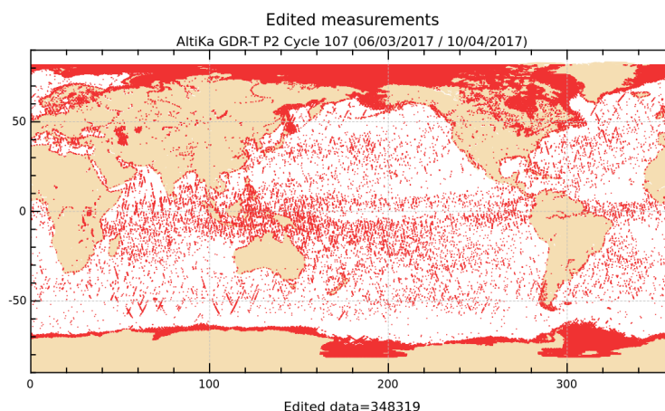
Figure 2: Edited measurements for cycle 107.
