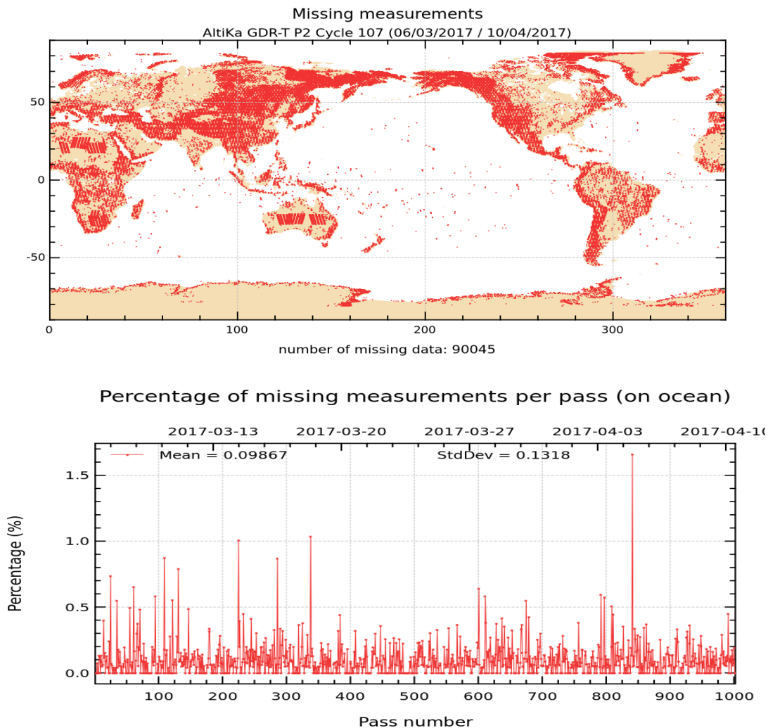
Figure 1: Map of missing measurements for cycle 107 on top. Monitoring of percentage of missing ocean measurements per pass on bottom.
