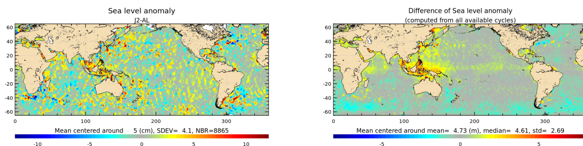
Figure 21: Jason-2 – Saral/AltiKa SLA differences for cycle 107 (left) and averaged over the whole Saral/AltiKa period (right).
