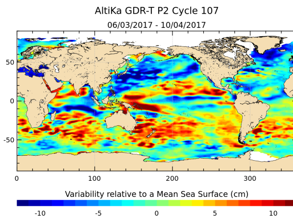
Figure 19: Sea level anomaly relative to MSS for cycle 107.
