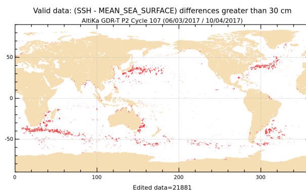
Figure 20: SLA higher than 30 cm for cycle 107.
