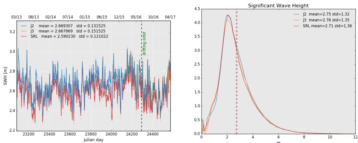
Figure 6: Daily monitoring of significant wave height for AltiKa (Ka-band) Jason-2 and Jason-3 (Ku-band) on the left and histogram for cycle 107 on the right (limited to 66^\circ latitude).
