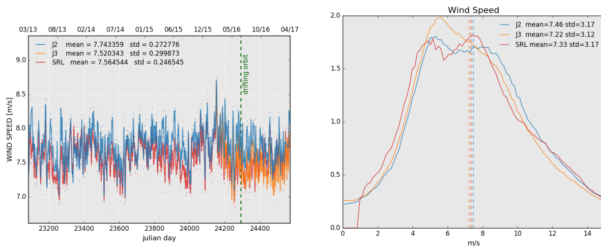
Figure 10: Daily monitoring of altimeter wind speed for Saral/AltiKa, Jason-2 and Jason-3 on the left and histogram for cycle 107 on the right (limited to 66° latitude).
