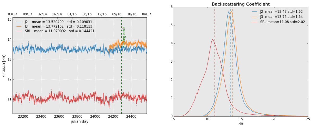
Figure 7: Daily monitoring of backscattering coefficient for Saral/AltiKa, Jason-2 and Jason-3 on the left and histogram for cycle 107 on the right (limited to 66° latitude).
