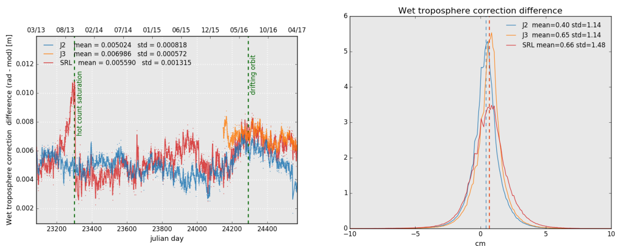
Figure 12: Daily monitoring of wet troposphere differences (Radiometer-ECMWF model) for Saral/AltiKa Jason-2 and Jason-3 (left) and histogram on the right (limited to 66° latitude) for cycle 107 .
