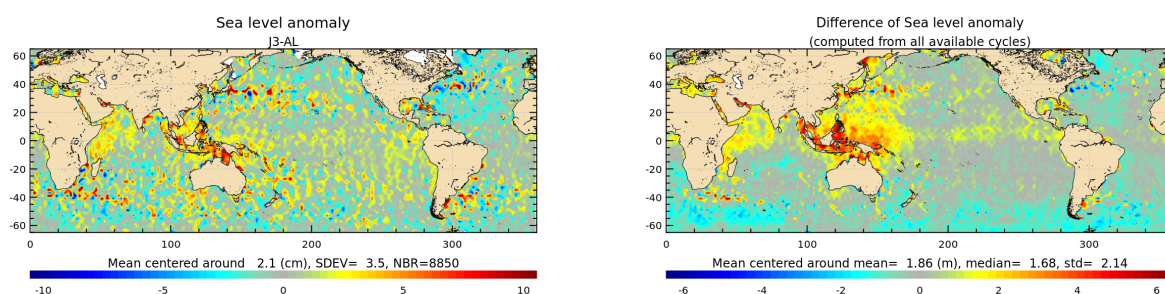
Figure 22: Jason-3 – Saral/AltiKa SLA differences for cycle 107 (left) and averaged over the whole Saral/AltiKa period (right).
