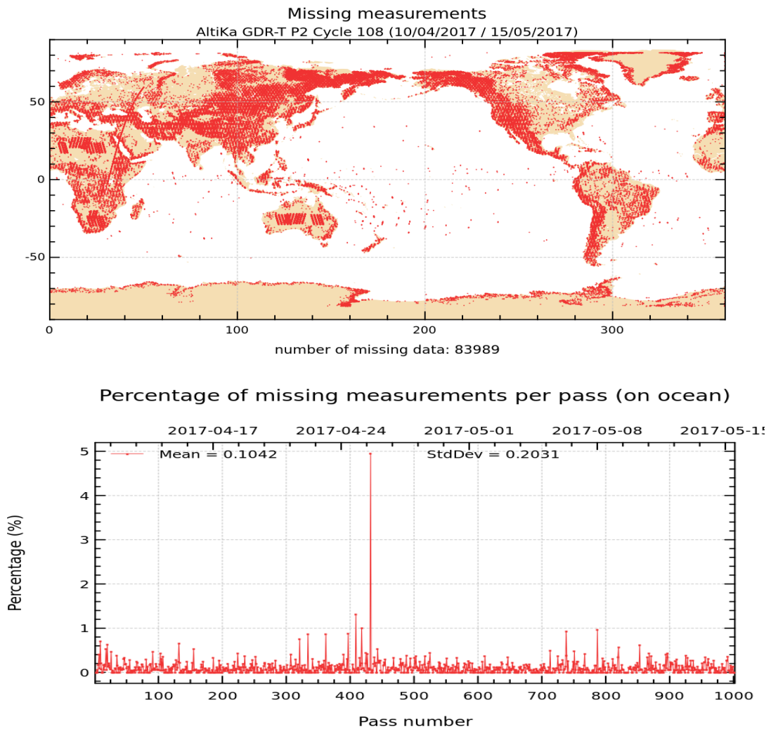
Figure 1: Map of missing measurements for cycle 108 on top. Monitoring of percentage of missing ocean measurements per pass on bottom.
