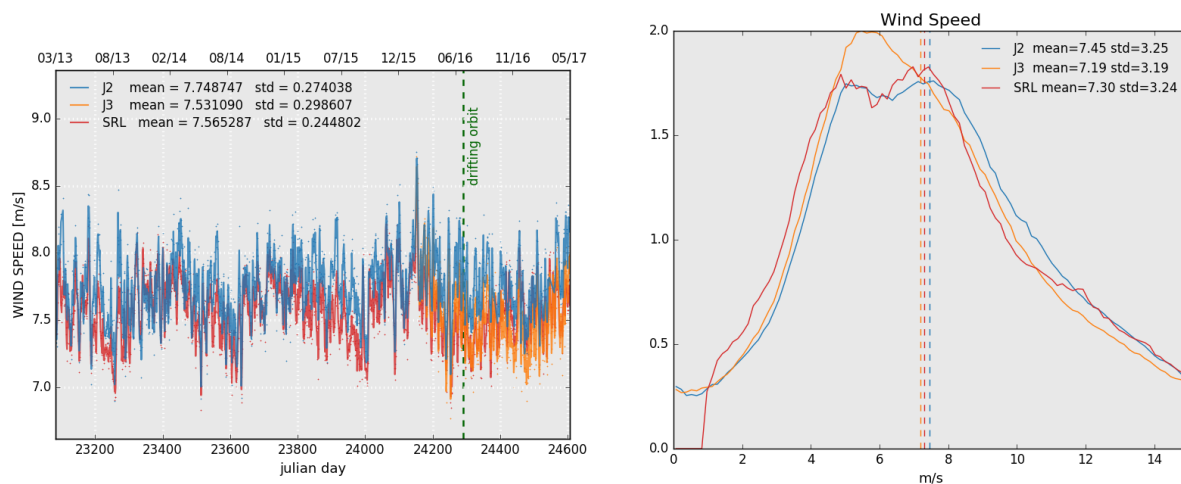
Figure 10: Daily monitoring of altimeter wind speed for Saral/AltiKa, Jason-2 and Jason-3 on the left and histogram for cycle 108 on the right (limited to 66° latitude).
