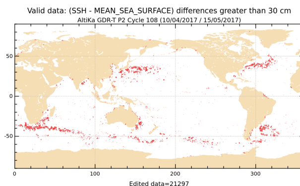
Figure 20: SLA higher than 30 cm for cycle 108.
