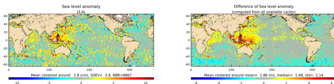
Figure 22: Jason-3 – Saral/AltiKa SLA differences for cycle 108 (left) and averaged over the whole Saral/AltiKa period (right).
