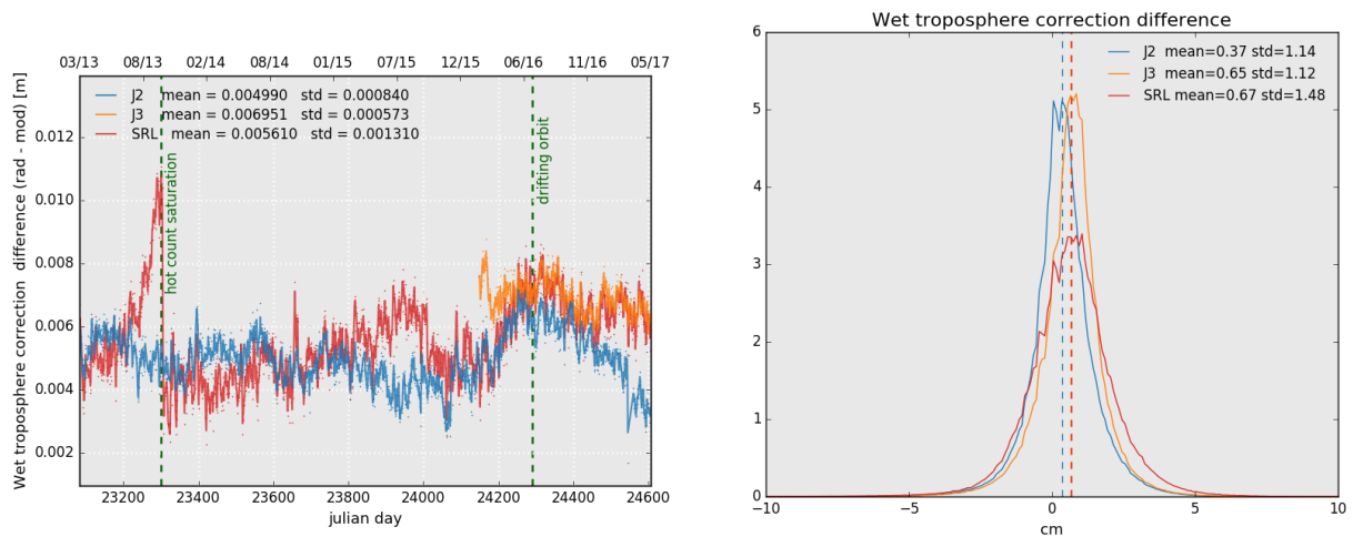
Figure 12: Daily monitoring of wet troposphere differences (Radiometer-ECMWF model) for Saral/AltiKa Jason-2 and Jason-3 (left) and histogram on the right (limited to 66° latitude) for cycle 108 .
