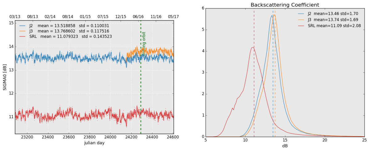
Figure 7: Daily monitoring of backscattering coefficient for Saral/AltiKa, Jason-2 and Jason-3 on the left and histogram for cycle 108 on the right (limited to 66° latitude).
