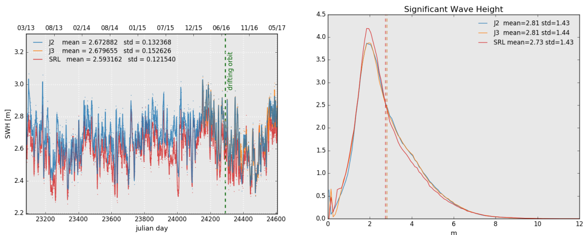
Figure 6: Daily monitoring of significant wave height for AltiKa (Ka-band) Jason-2 and Jason-3 (Ku-band) on the left and histogram for cycle 108 on the right (limited to 66^\circ latitude).
