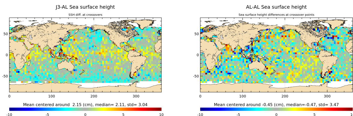
Figure 16: Mean of multi-mission SSH and mono-mission SSH differences at crossovers for cycle 114.
