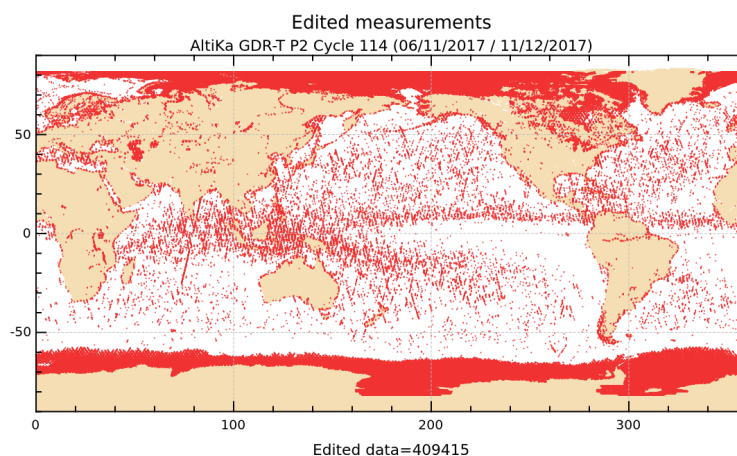
Figure 2: Edited measurements for cycle 114.
