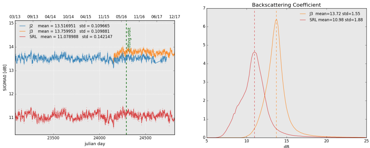
Figure 9: Daily monitoring of backscattering coefficient for Saral/AltiKa, Jason-2 and Jason-3 on the left and histogram for cycle 114 on the right (limited to 66° latitude).
