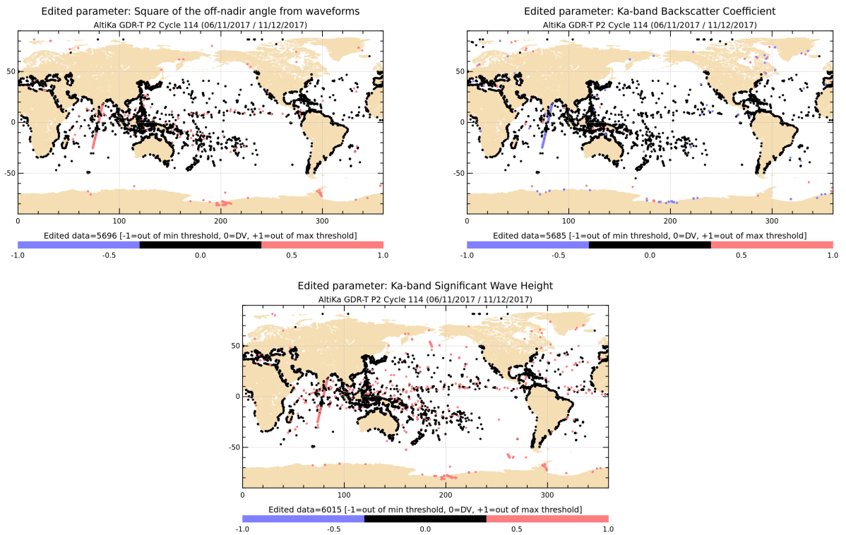
Figure 4: Maps of edited measurements on threshold for Saral/AltiKa, cycle 114 .
