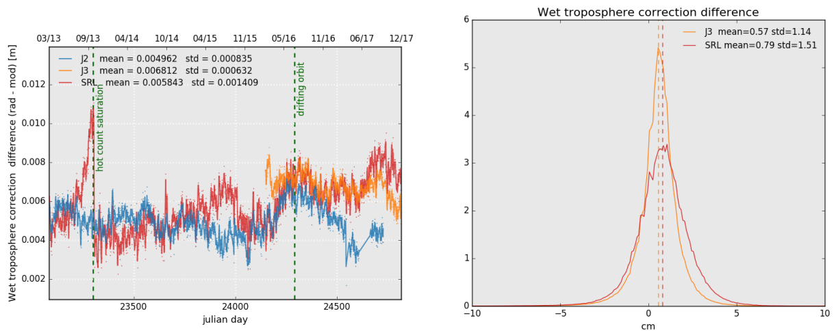
Figure 14: Daily monitoring of wet troposphere differences (Radiometer-ECMWF model) for Saral/AltiKa Jason-2 and Jason-3 (left) and histogram on the right (limited to 66° latitude) for cycle 114 .
