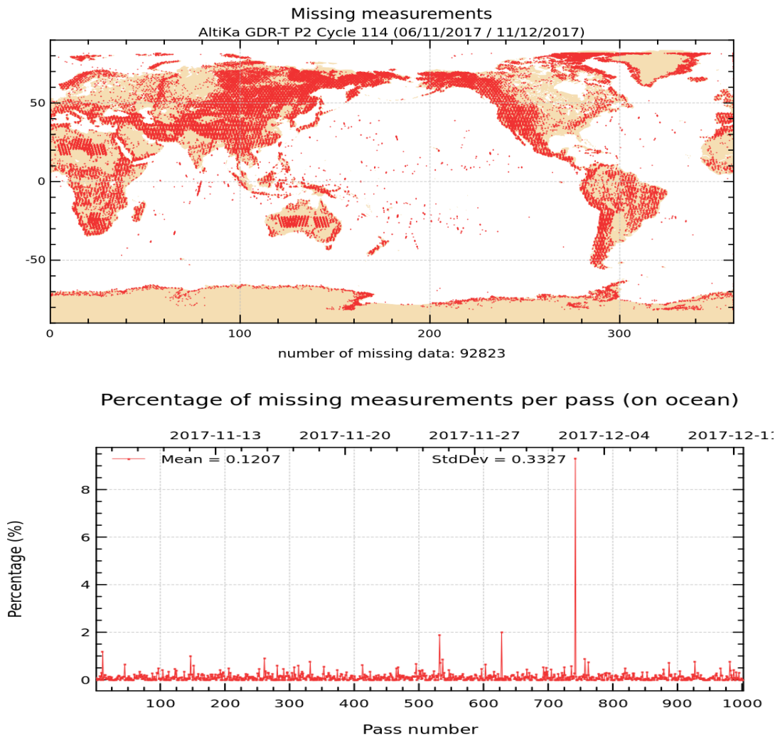
Figure 1: Map of missing measurements for cycle 114 on top. Monitoring of percentage of missing ocean measurements per pass on bottom.
