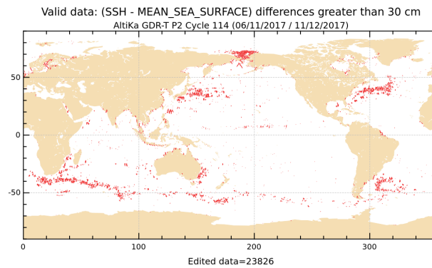
Figure 22: SLA higher than 30 cm for cycle 114.
