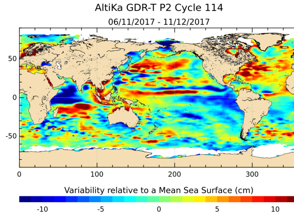
Figure 21: Sea level anomaly relative to MSS for cycle 114.
