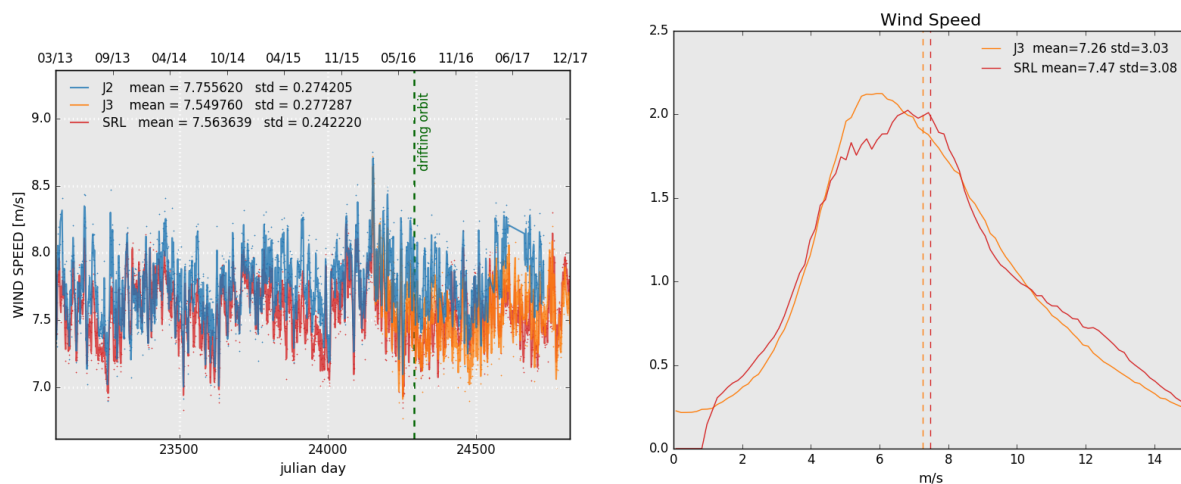
Figure 12: Daily monitoring of altimeter wind speed for Saral/AltiKa, Jason-2 and Jason-3 on the left and histogram for cycle 114 on the right (limited to 66° latitude).
