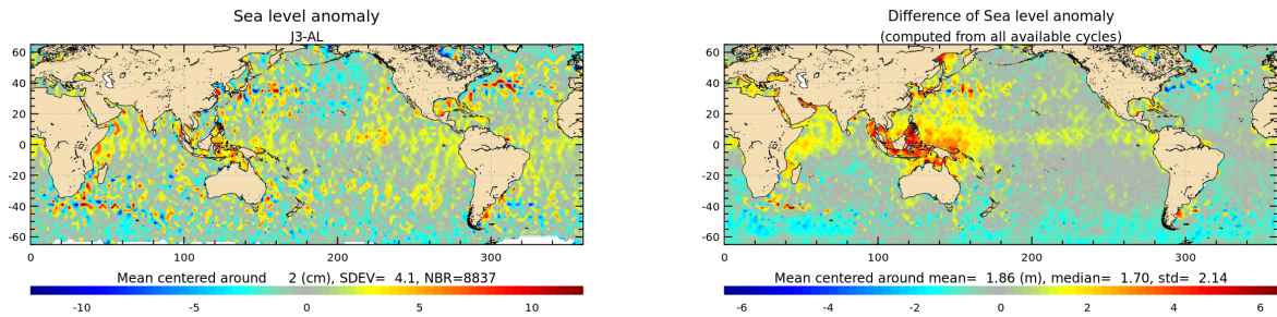
Figure 23: Jason-3 – Saral/AltiKa SLA differences for cycle 114 (left) and averaged over the whole Saral/AltiKa period (right).
