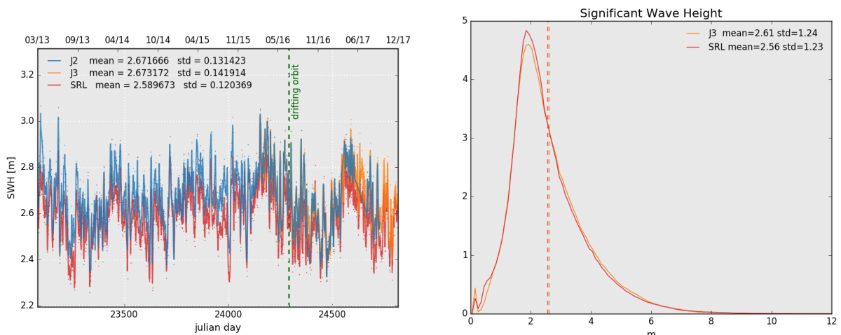
Figure 8: Daily monitoring of significant wave height for AltiKa (Ka-band) Jason-2 and Jason-3 (Ku-band) on the left and histogram for cycle 114 on the right (limited to 66^\circ latitude).
