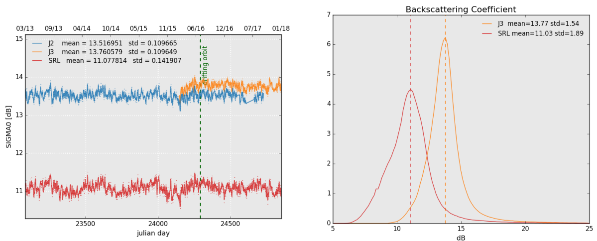
Figure 8: Daily monitoring of backscattering coefficient for Saral/AltiKa, Jason-2 and Jason-3 on the left and histogram for cycle 115 on the right (limited to 66° latitude).
