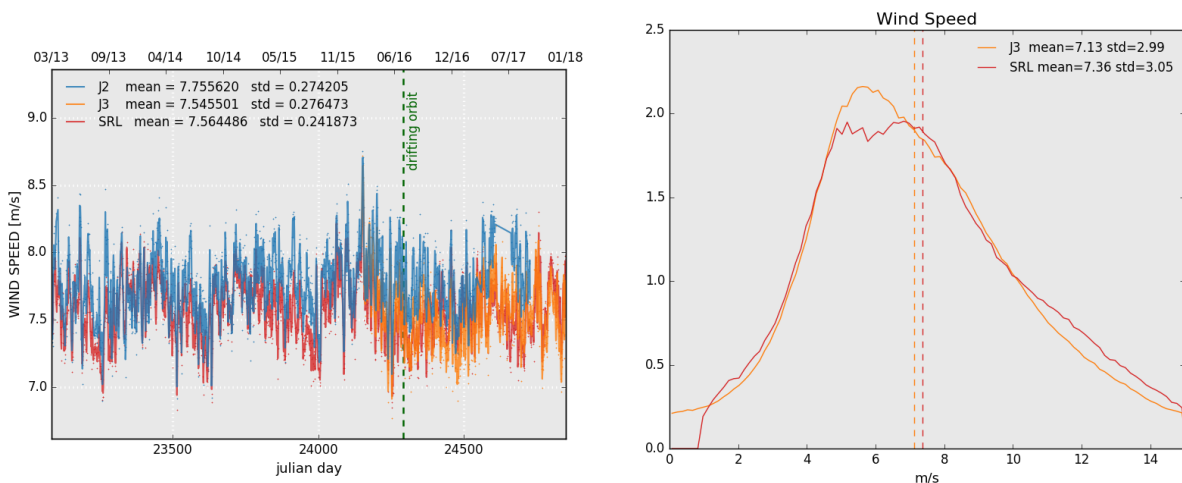
Figure 11: Daily monitoring of altimeter wind speed for Saral/AltiKa, Jason-2 and Jason-3 on the left and histogram for cycle 115 on the right (limited to 66^\circ latitude).
