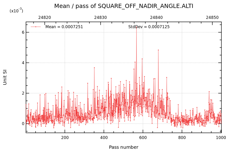
Figure 4: Monitoring of mispointing for cycle 115.
