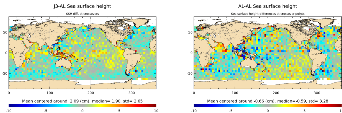
Figure 15: Mean of multi-mission SSH and mono-mission SSH differences at crossovers for cycle 115.
