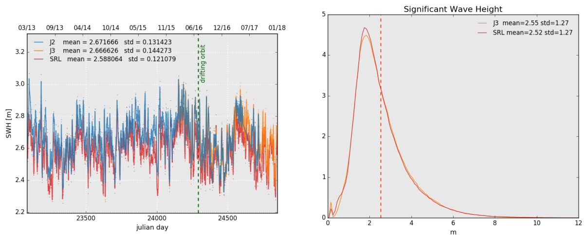
Figure 7: Daily monitoring of significant wave height for AltiKa (Ka-band) Jason-2 and Jason-3 (Ku-band) on the left and histogram for cycle 115 on the right (limited to 66° latitude).
