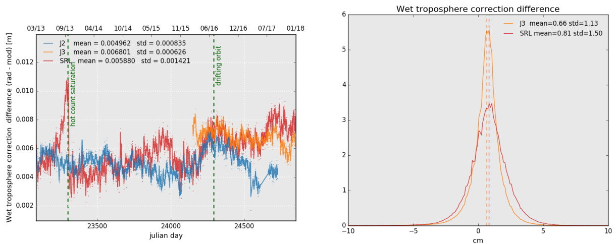
Figure 13: Daily monitoring of wet troposphere differences (Radiometer-ECMWF model) for Saral/AltiKa Jason-2 and Jason-3 (left) and histogram on the right (limited to 66° latitude) for cycle 115 .
