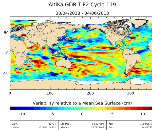
Figure 21: Sea level anomaly relative to MSS for cycle 119.
