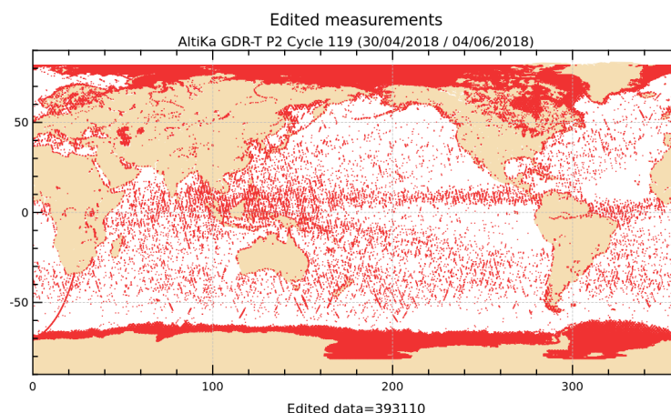
Figure 2: Edited measurements for cycle 119.
