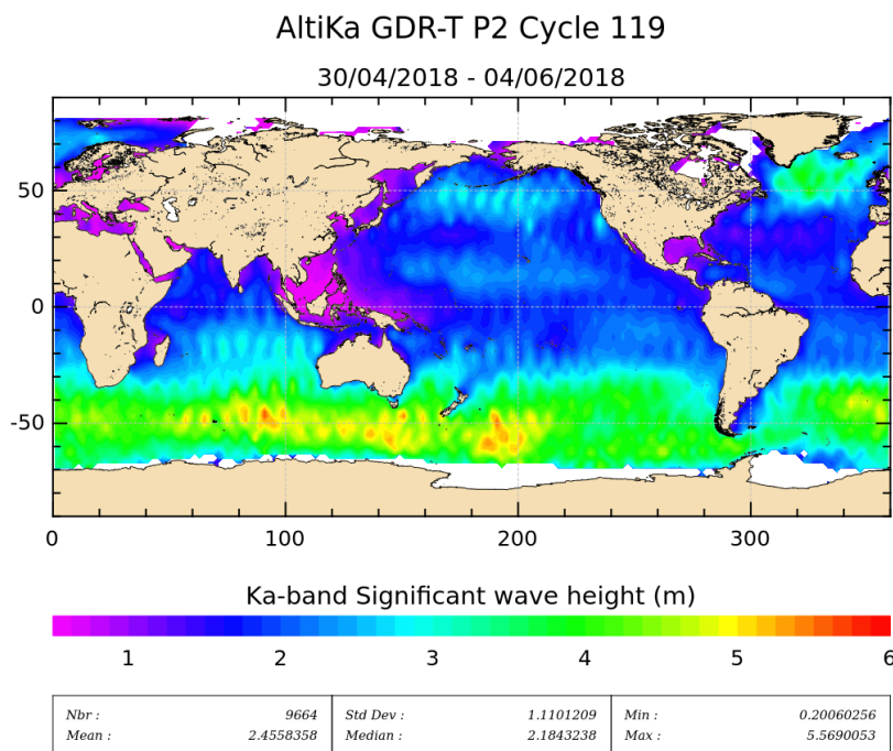
Figure 7: Significant wave height for cycle 119.
