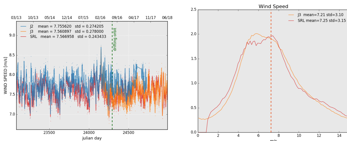
Figure 12: Daily monitoring of altimeter wind speed for Saral/AltiKa, Jason-2 and Jason-3 on the left and histogram for cycle 119 on the right (limited to 66° latitude).
