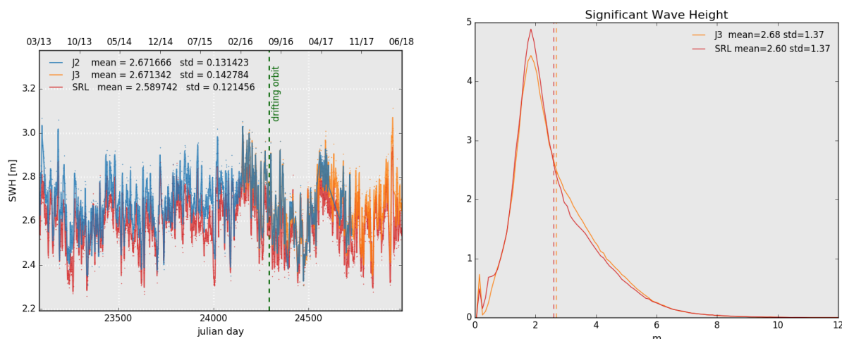
Figure 8: Daily monitoring of significant wave height for AltiKa (Ka-band) Jason-2 and Jason-3 (Ku-band) on the left and histogram for cycle 119 on the right (limited to 66^\circ latitude).
