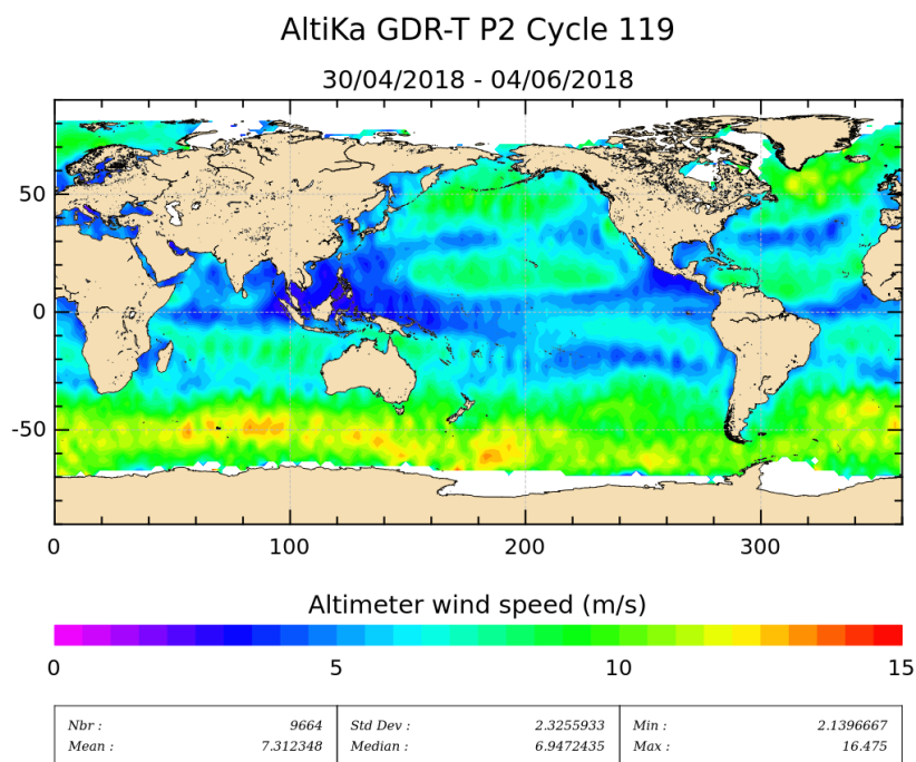
Figure 11: Altimeter wind speed for cycle 119.
