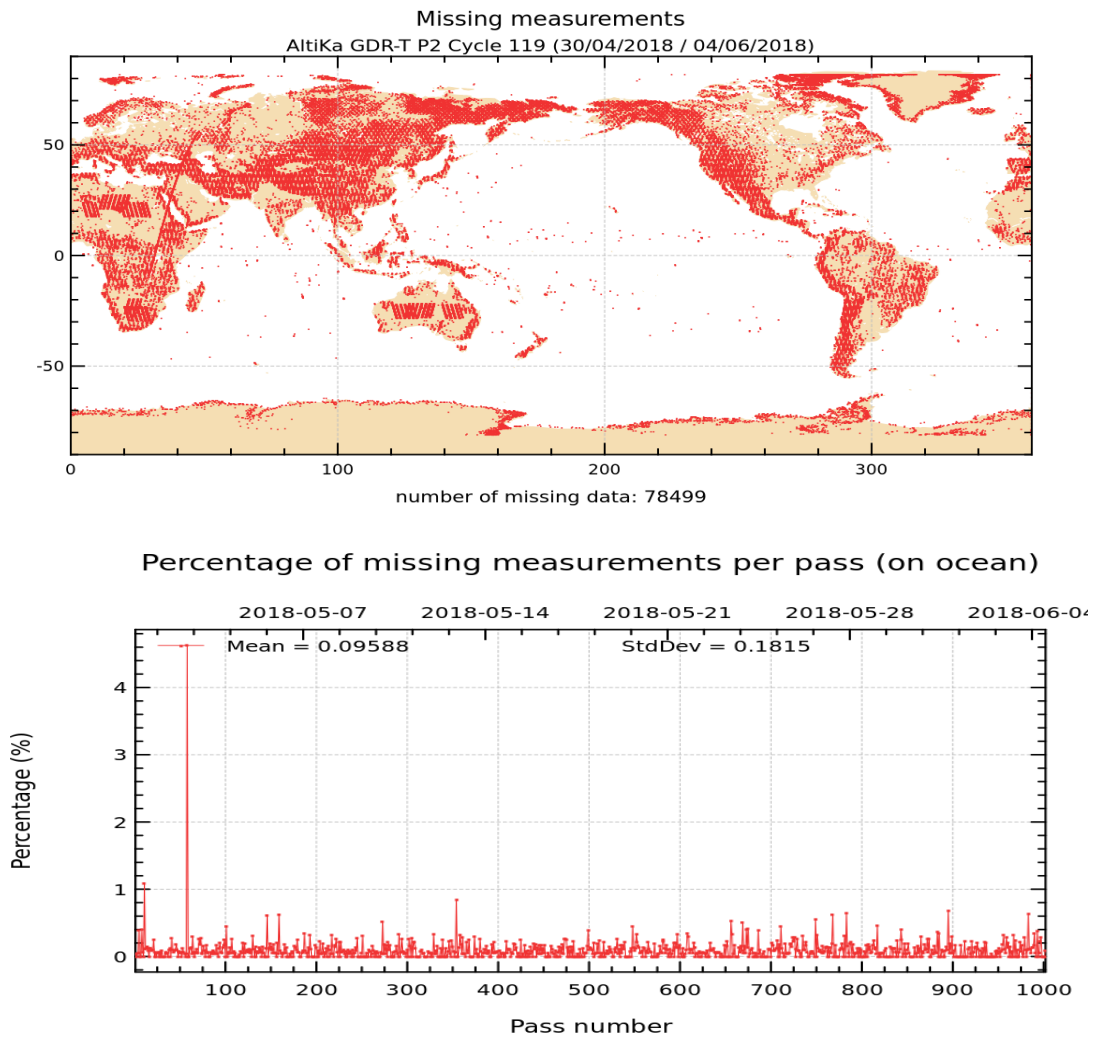
Figure 1: Map of missing measurements for cycle 119 on top. Monitoring of percentage of missing ocean measurements per pass on bottom.
