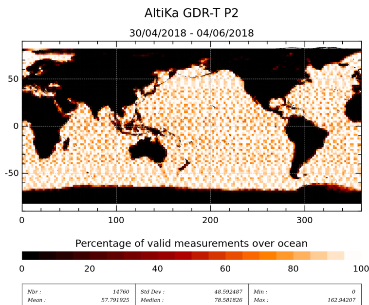
Figure 3: Percentage of valid measurements for cycle 119.
