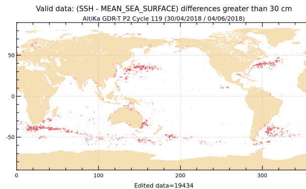
Figure 22: SLA higher than 30 cm for cycle 119.
