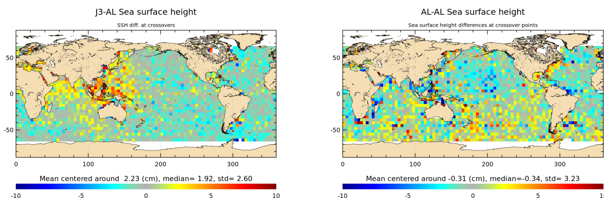
Figure 16: Mean of multi-mission SSH and mono-mission SSH differences at crossovers for cycle 119.
