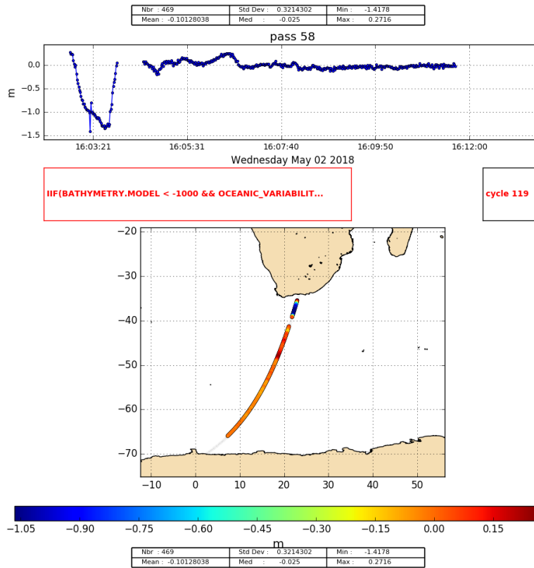
Figure 4: SLA values along track 58.
