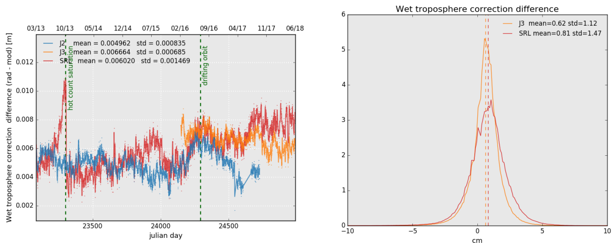
Figure 14: Daily monitoring of wet troposphere differences (Radiometer-ECMWF model) for Saral/AltiKa Jason-2 and Jason-3 (left) and histogram on the right (limited to 66° latitude) for cycle 119 .
