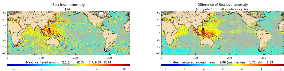
Figure 23: Jason-3 – Saral/AltiKa SLA differences for cycle 119 (left) and averaged over the whole Saral/AltiKa period (right).
