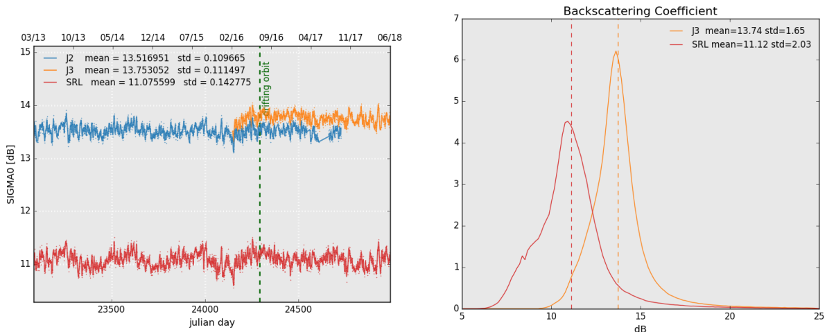
Figure 9: Daily monitoring of backscattering coefficient for Saral/AltiKa, Jason-2 and Jason-3 on the left and histogram for cycle 119 on the right (limited to 66° latitude).
