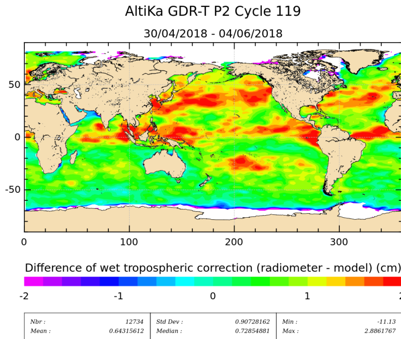
Figure 13: Mean of wet troposphere correction difference (Radiometer-ECMWF model) for cycle 119.
