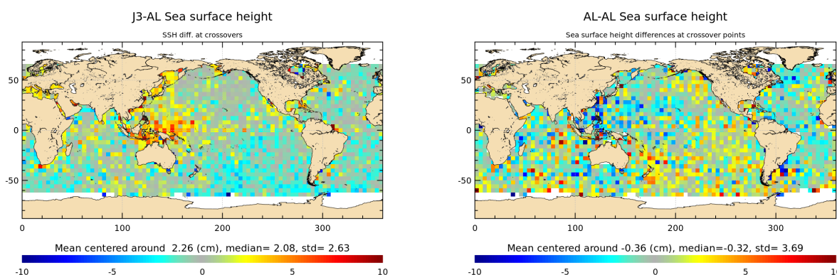
Figure 14: Mean of multi-mission SSH and mono-mission SSH differences at crossovers for cycle 121.
