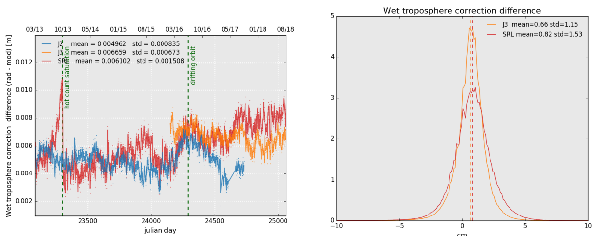
Figure 12: Daily monitoring of wet troposphere differences (Radiometer-ECMWF model) for Saral/AltiKa Jason-2 and Jason-3 (left) and histogram on the right (limited to 66° latitude) for cycle 121 .
