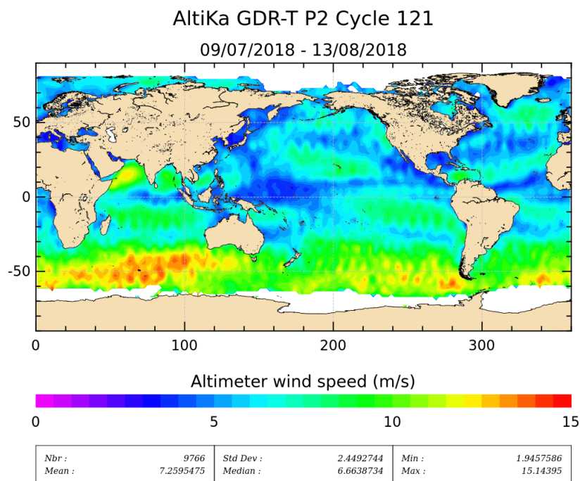
Figure 9: Altimeter wind speed for cycle 121.
