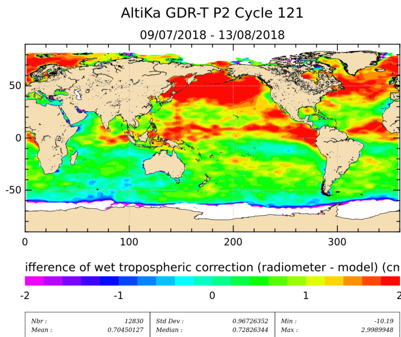
Figure 11: Mean of wet troposphere correction difference (Radiometer-ECMWF model) for cycle 121.
