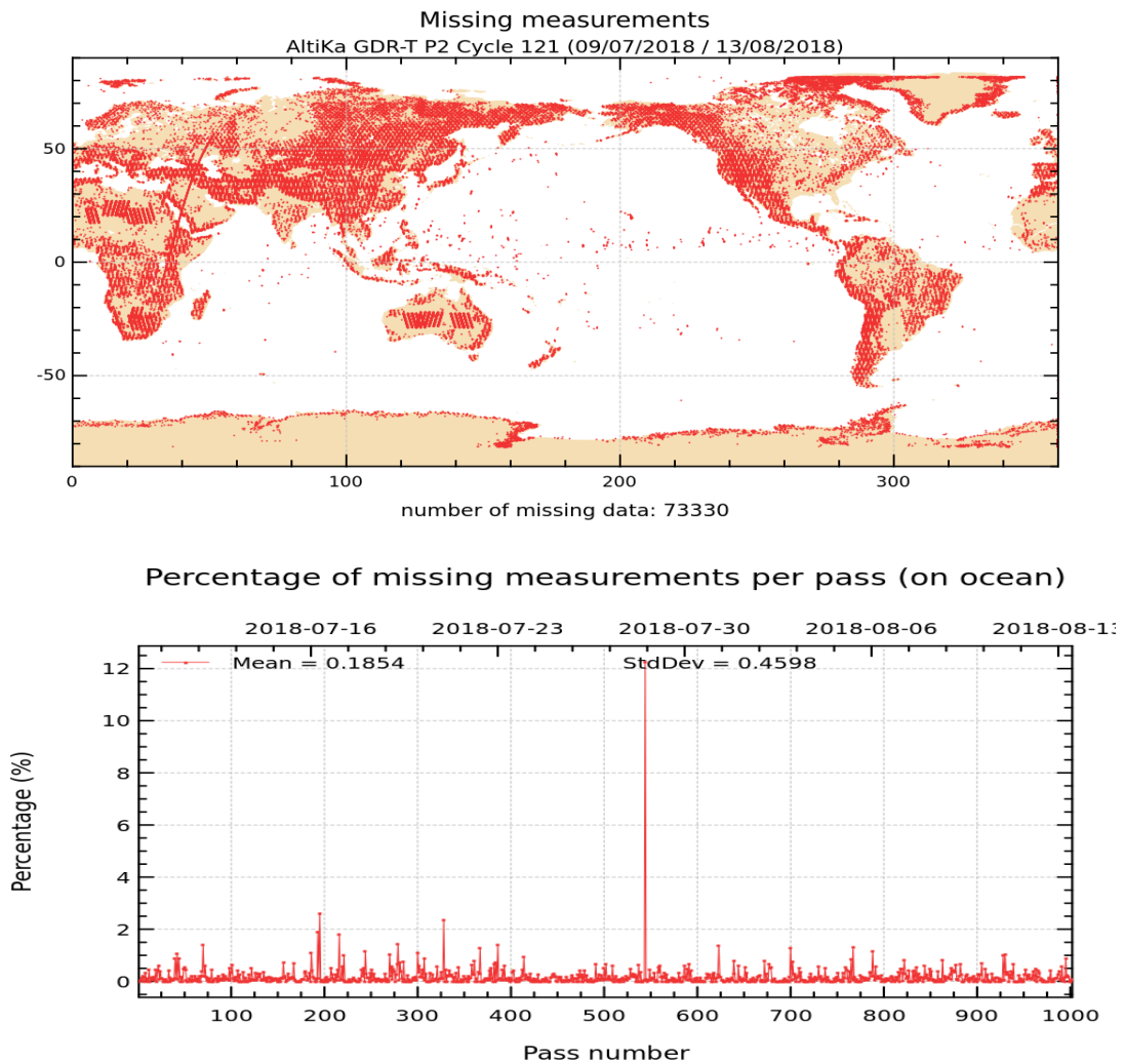
Figure 1: Map of missing measurements for cycle 121 on top. Monitoring of percentage of missing ocean measurements per pass on bottom.
