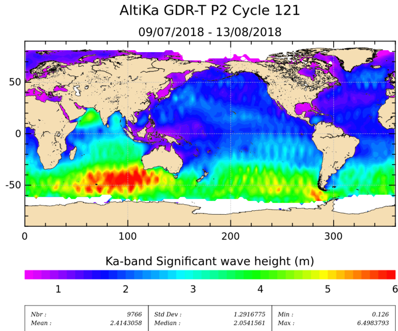
Figure 5: Significant wave height for cycle 121.
