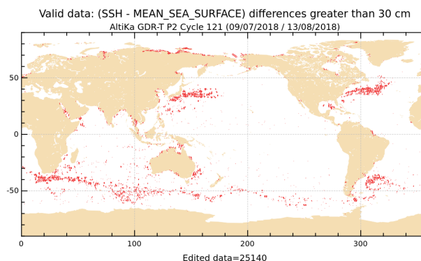
Figure 20: SLA higher than 30 cm for cycle 121.
