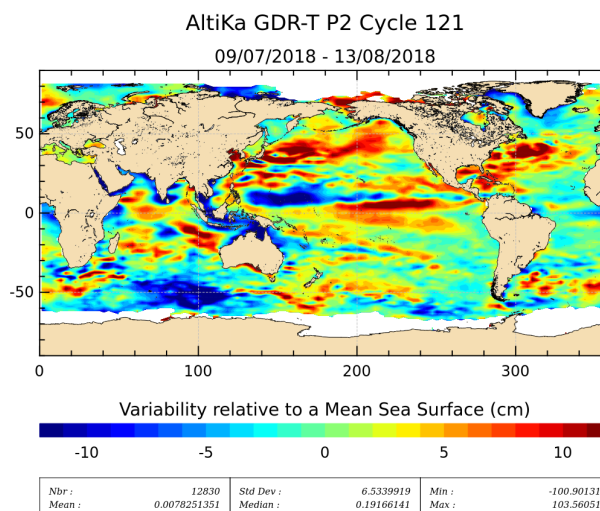
Figure 19: Sea level anomaly relative to MSS for cycle 121.
