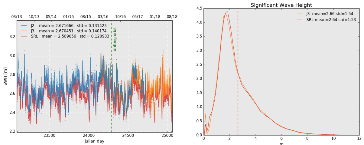
Figure 6: Daily monitoring of significant wave height for AltiKa (Ka-band) Jason-2 and Jason-3 (Ku-band) on the left and histogram for cycle 121 on the right (limited to 66^\circ latitude).
