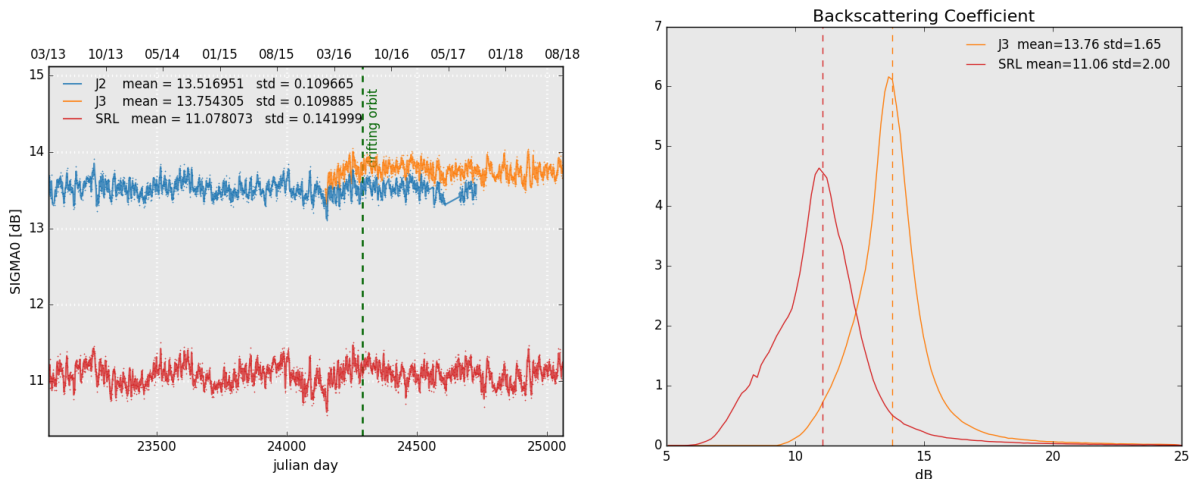
Figure 7: Daily monitoring of backscattering coefficient for Saral/AltiKa, Jason-2 and Jason-3 on the left and histogram for cycle 121 on the right (limited to 66° latitude).
