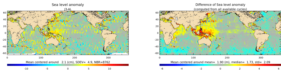
Figure 21: Jason-3 – Saral/AltiKa SLA differences for cycle 121 (left) and averaged over the whole Saral/AltiKa period (right).
