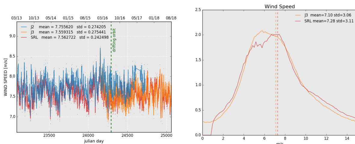
Figure 10: Daily monitoring of altimeter wind speed for Saral/AltiKa, Jason-2 and Jason-3 on the left and histogram for cycle 121 on the right (limited to 66° latitude).
