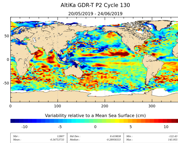
Figure 20: Sea level anomaly relative to MSS for cycle 130.
