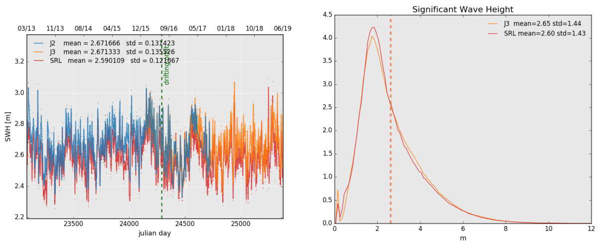
Figure 6: Daily monitoring of significant wave height for AltiKa (Ka-band) Jason-2 and Jason-3 (Ku-band) on the left and histogram for cycle 130 on the right (limited to 66° latitude).
