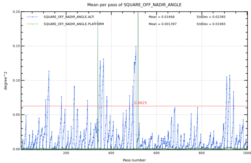
Figure 3: Mispointing cycle 130.
