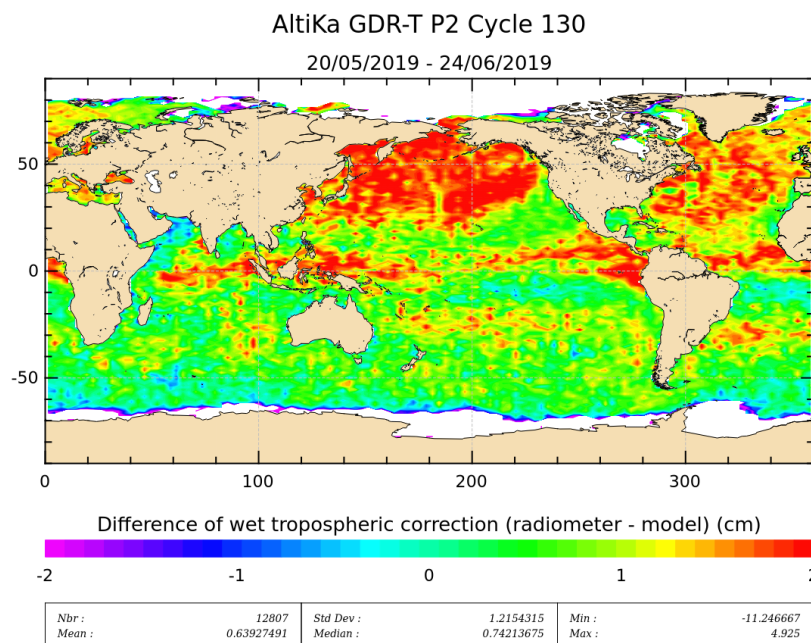
Figure 11: Mean of wet troposphere correction difference (Radiometer-ECMWF model) for cycle 130.
