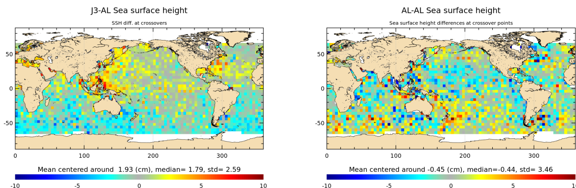
Figure 15: Mean of multi-mission SSH and mono-mission SSH differences at crossovers for cycle 130.
