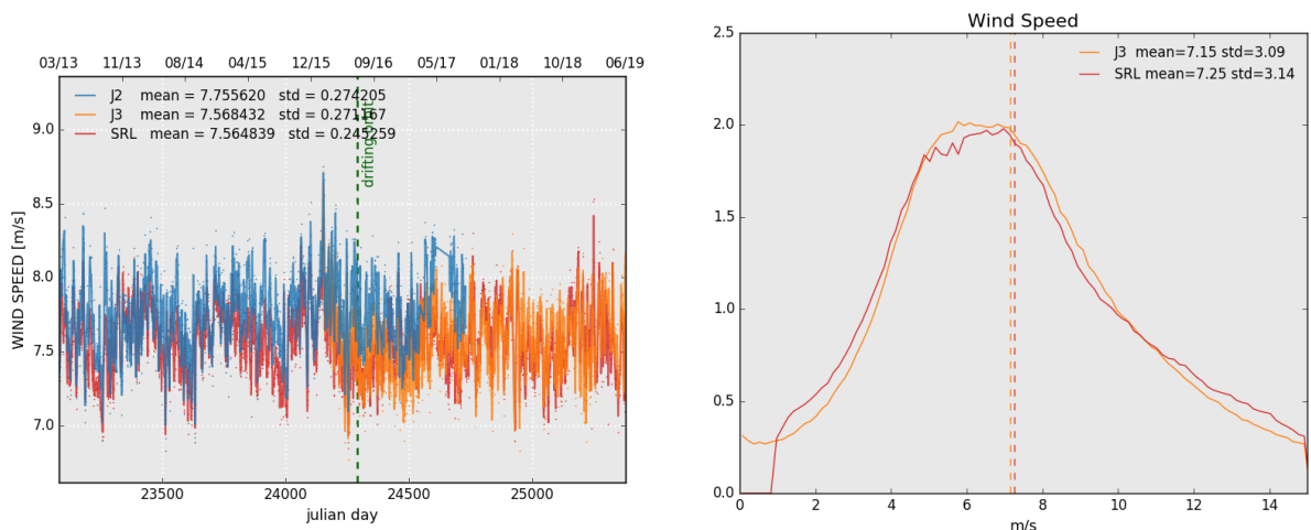
Figure 10: Daily monitoring of altimeter wind speed for Saral/AltiKa, Jason-2 and Jason-3 on the left and histogram for cycle 130 on the right (limited to 66° latitude).
