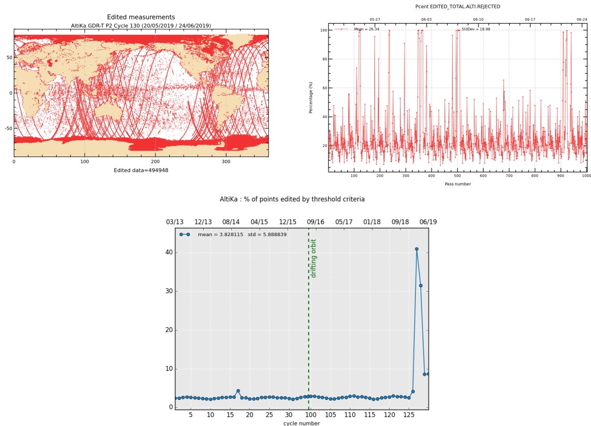
Figure 2: Rejected measurements on thresholds criteria : Cycle 130, map and monitoring of % of rejected measurements per track (top), whole time serie / % of rejected measurements per cycle (bottom).
