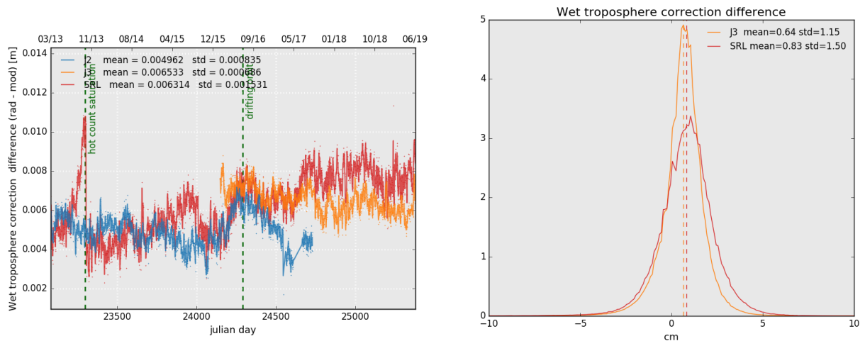
Figure 12: Daily monitoring of wet troposphere differences (Radiometer-ECMWF model) for Saral/AltiKa Jason-2 and Jason-3 (left) and histogram on the right (limited to 66° latitude) for cycle 130 .
