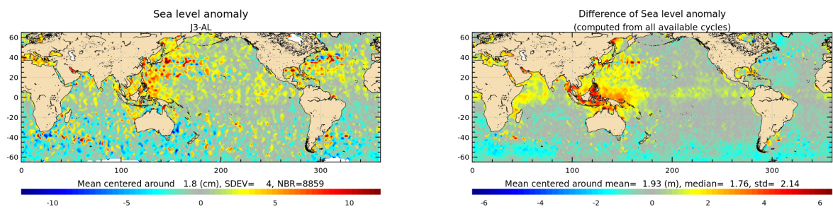
Figure 21: SLA higher than 30 cm for cycle 130.
