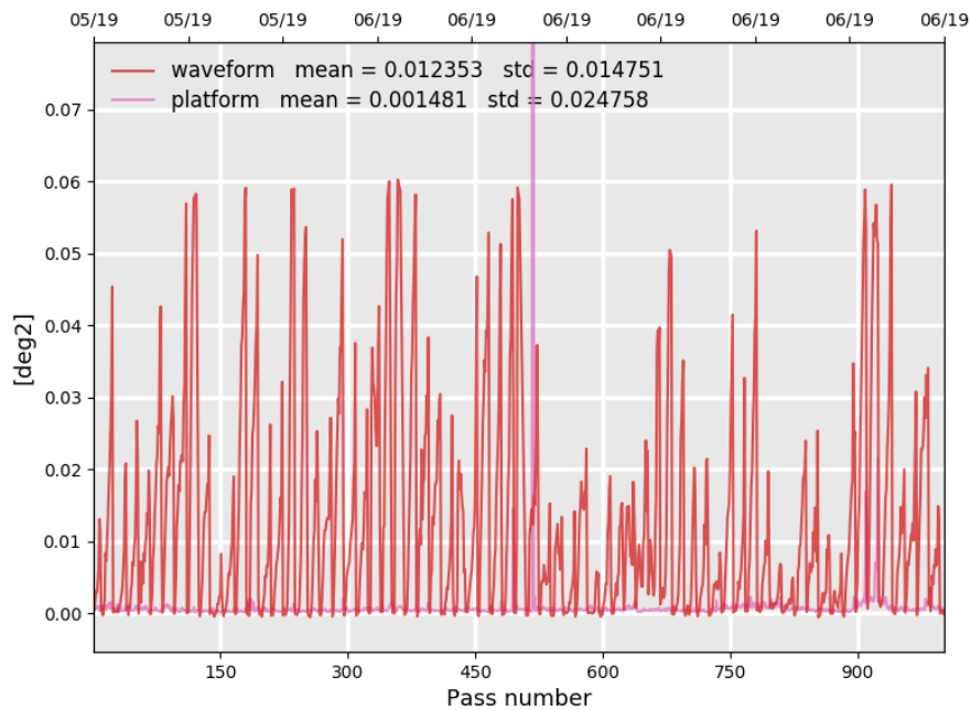
Figure 14: Monitoring per pass for cycle 130 of SARAL/AltiKa's mispointing angle: comparison between the one derived from waveform retracking and the one measured by platform startrackers.
