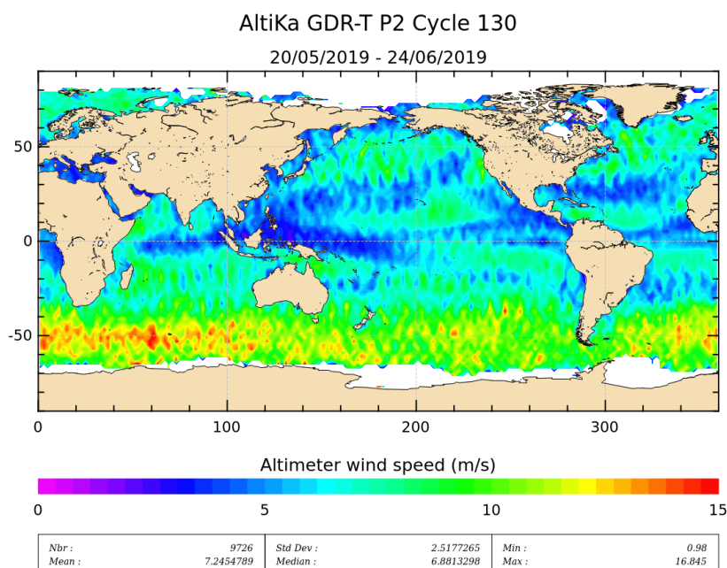
Figure 9: Altimeter wind speed for cycle 130.
