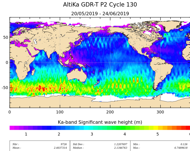
Figure 5: Significant wave height for cycle 130.
