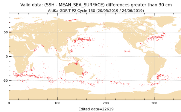
Figure 20: Sea level anomaly relative to MSS for cycle 130.
