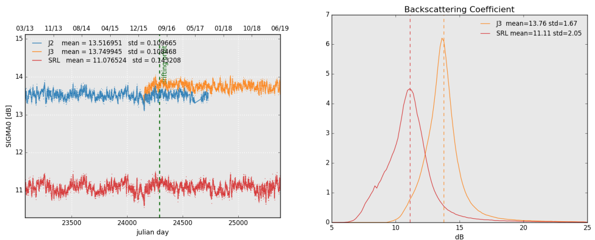
Figure 7: Daily monitoring of backscattering coefficient for Saral/AltiKa, Jason-2 and Jason-3 on the left and histogram for cycle 130 on the right (limited to 66° latitude).
