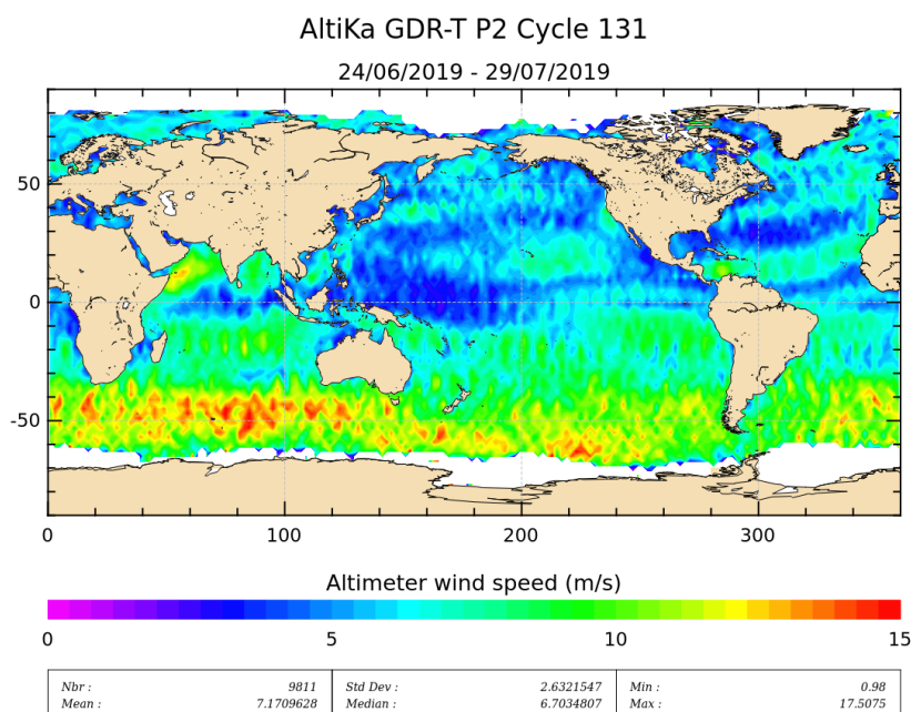
Figure 9: Altimeter wind speed for cycle 131.
