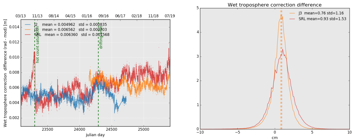
Figure 12: Daily monitoring of wet troposphere differences (Radiometer-ECMWF model) for Saral/AltiKa Jason-2 and Jason-3 (left) and histogram on the right (limited to 66° latitude) for cycle 131 .
