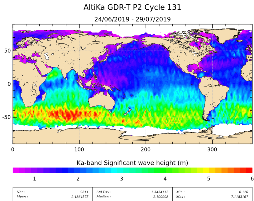
Figure 5: Significant wave height for cycle 131.
