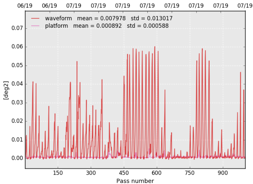
Figure 14: Monitoring per pass for cycle 131 of SARAL/AltiKa's mispointing angle: comparison between the one derived from waveform retracking and the one measured by platform startrackers.
