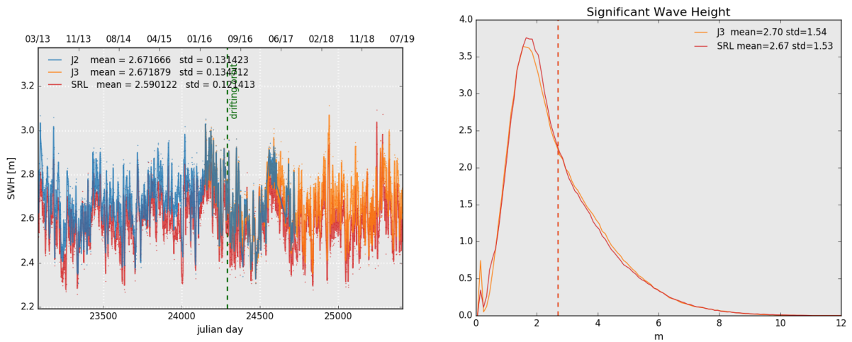
Figure 6: Daily monitoring of significant wave height for AltiKa (Ka-band) Jason-2 and Jason-3 (Ku-band) on the left and histogram for cycle 131 on the right (limited to 66° latitude).
