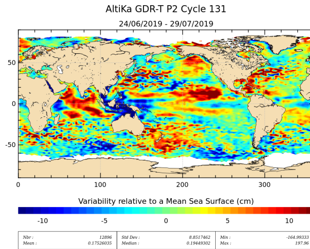
Figure 20: Sea level anomaly relative to MSS for cycle 131.
