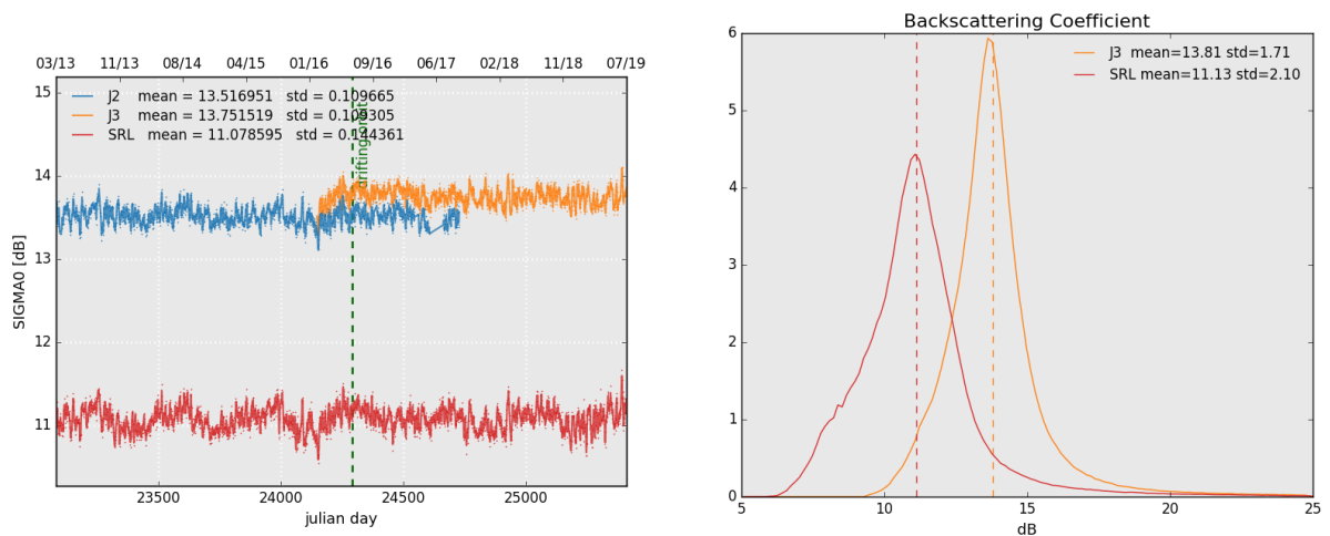
Figure 7: Daily monitoring of backscattering coefficient for Saral/AltiKa, Jason-2 and Jason-3 on the left and histogram for cycle 131 on the right (limited to 66° latitude).
