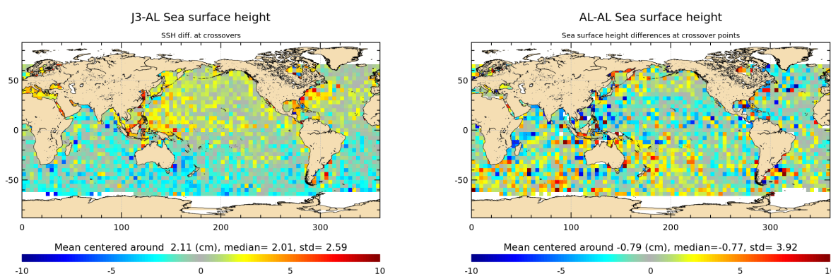
Figure 15: Mean of multi-mission SSH and mono-mission SSH differences at crossovers for cycle 131.
