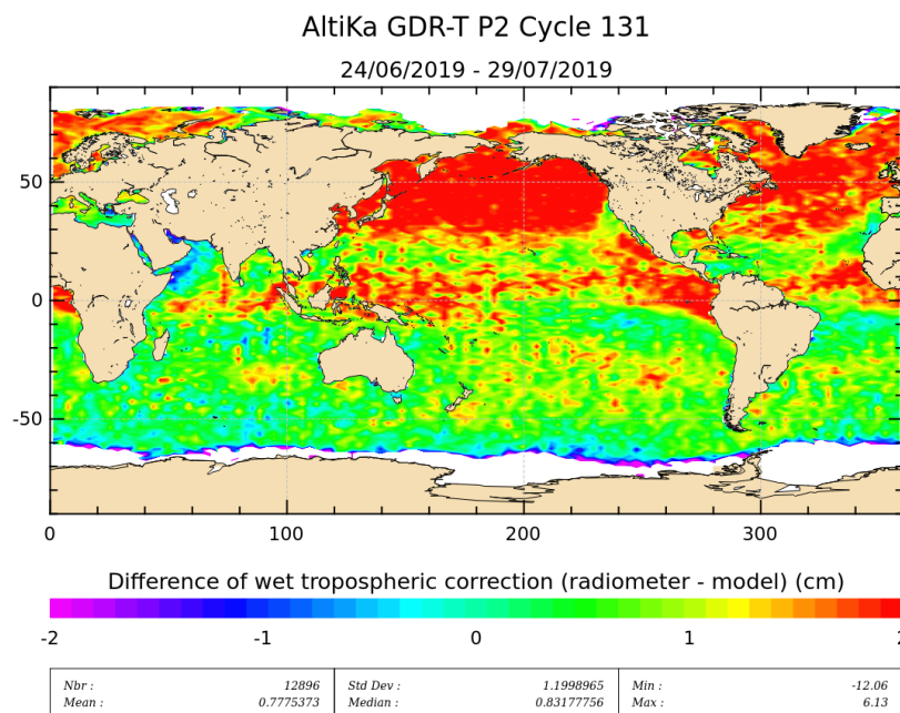
Figure 11: Mean of wet troposphere correction difference (Radiometer-ECMWF model) for cycle 131.
