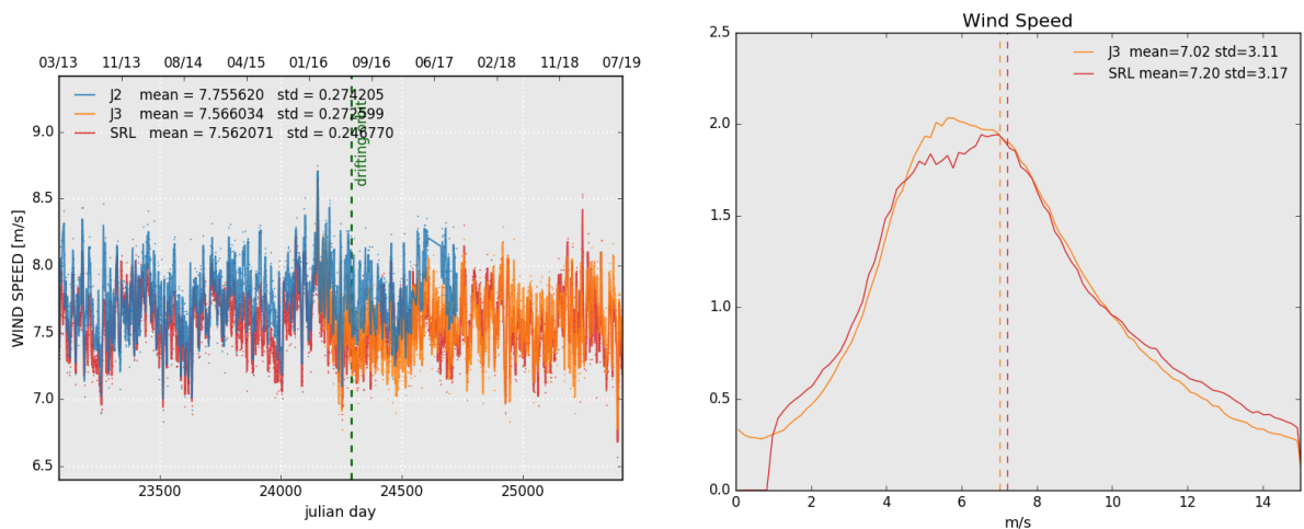
Figure 10: Daily monitoring of altimeter wind speed for Saral/AltiKa, Jason-2 and Jason-3 on the left and histogram for cycle 131 on the right (limited to 66° latitude).
