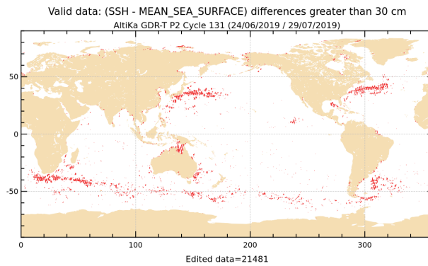
Figure 20: Sea level anomaly relative to MSS for cycle 131.
