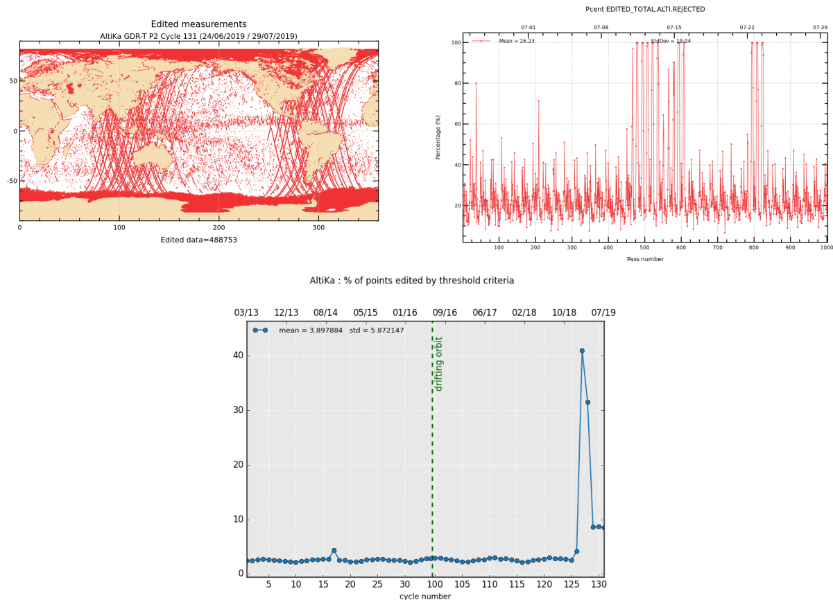
Figure 2: Rejected measurements on thresholds criteria : Cycle 131, map and monitoring of % of rejected measurements per track (top), whole time serie / % of rejected measurements per cycle (bottom).
