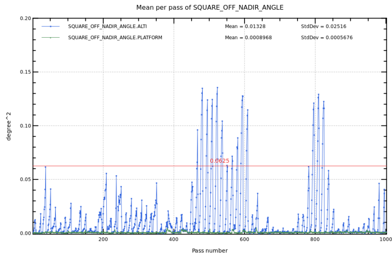
Figure 3: Mispointing cycle 131.
