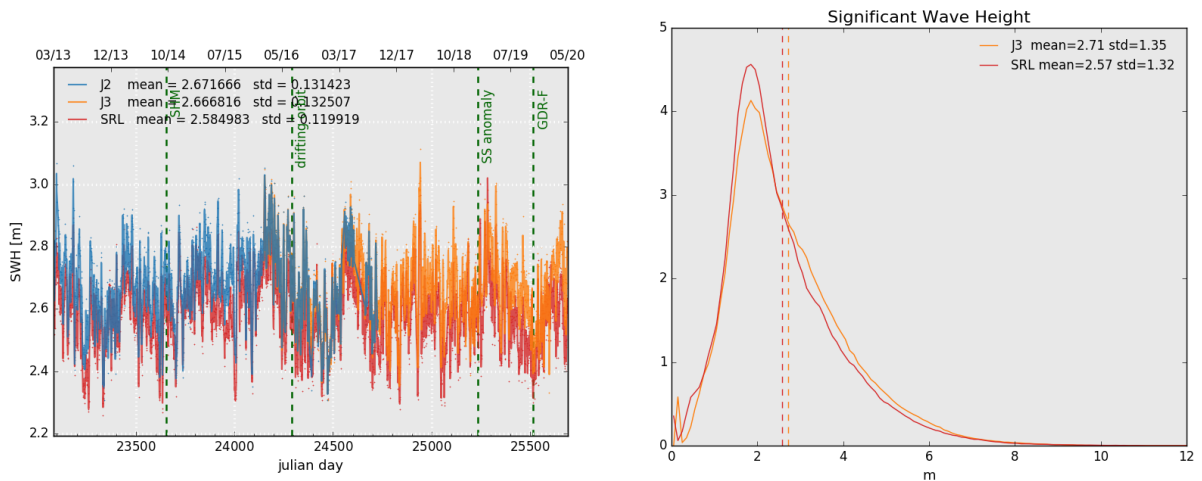
Figure 7: Daily monitoring of significant wave height for AltiKa (Ka-band) Jason-2 and Jason-3 (Ku-band) on the left and histogram for cycle 139 on the right (limited to 66° latitude).
