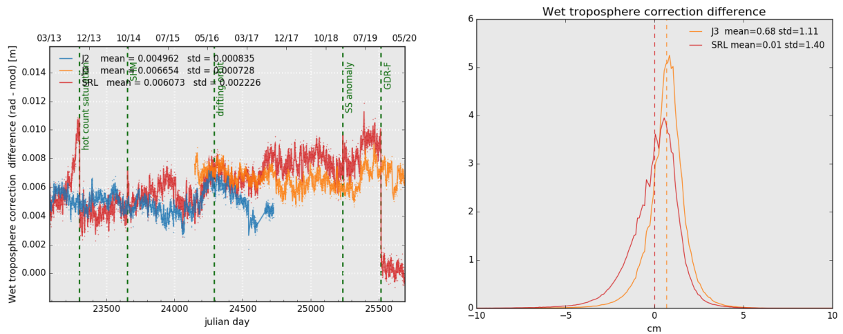
Figure 13: Daily monitoring of wet troposphere differences (Radiometer-ECMWF model) for Saral/AltiKa Jason-2 and Jason-3 (left) and histogram on the right (limited to 66° latitude) for cycle 139 .
