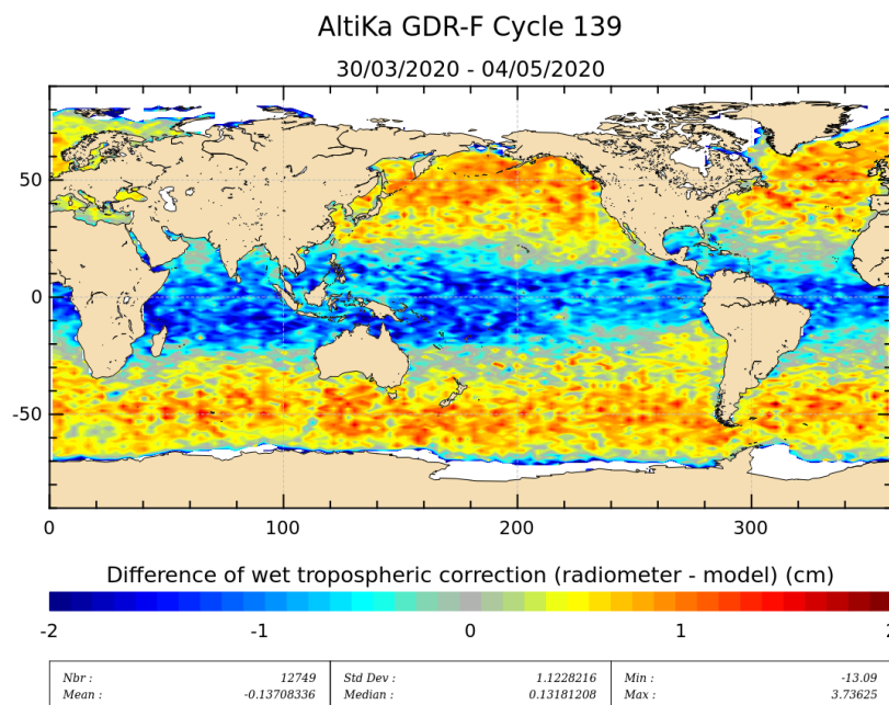
Figure 12: Mean of wet troposphere correction difference (Radiometer-ECMWF model) for cycle 139.
