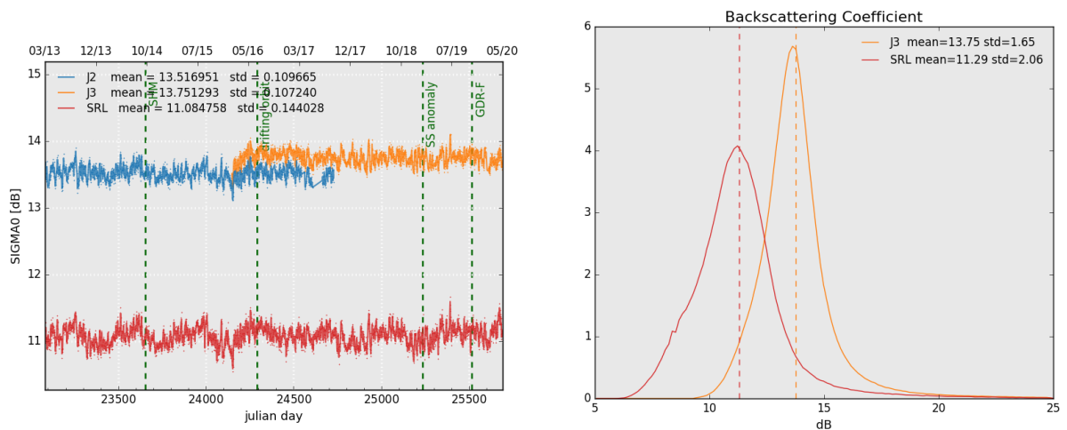
Figure 8: Daily monitoring of backscattering coefficient for Saral/AltiKa, Jason-2 and Jason-3 on the left and histogram for cycle 139 on the right (limited to 66° latitude).
