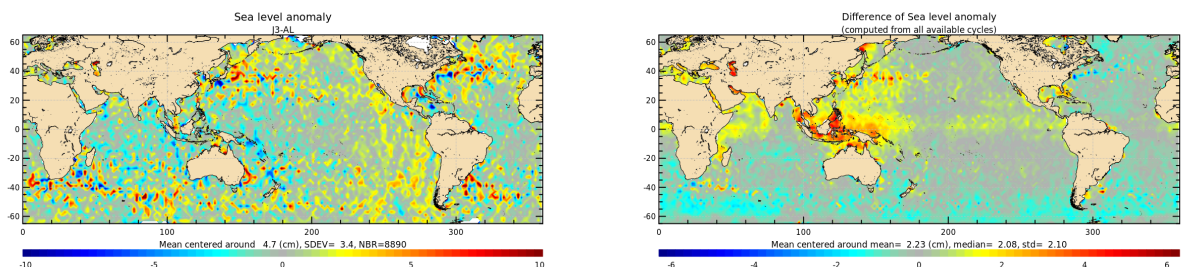
Figure 22: Jason-3 – Saral/AltiKa SLA differences for cycle 139 (left) and averaged over the whole Saral/AltiKa period (right).
