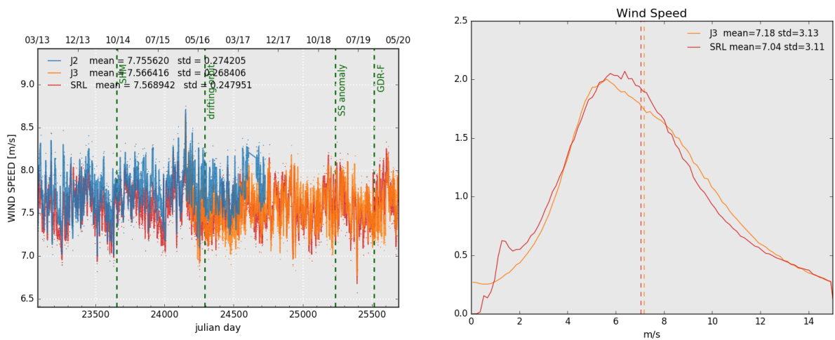
Figure 11: Daily monitoring of altimeter wind speed for Saral/AltiKa, Jason-2 and Jason-3 on the left and histogram for cycle 139 on the right (limited to 66° latitude).
