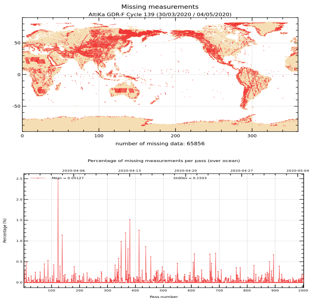
Figure 1: Map of missing measurements for cycle 139 on top. Monitoring of percentage of missing ocean measurements per pass on bottom.
