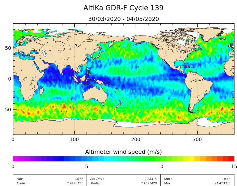
Figure 10: Altimeter wind speed for cycle 139.
