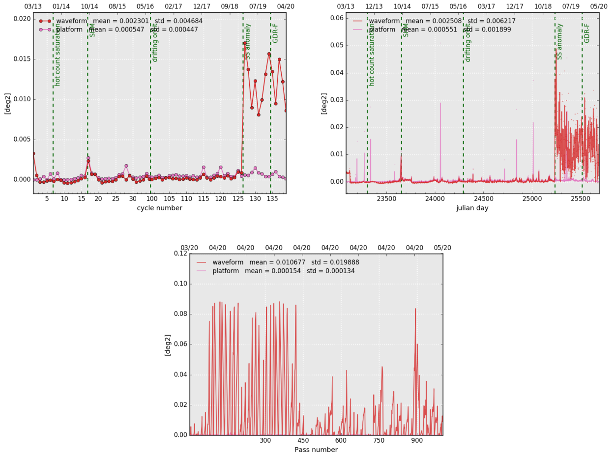
Figure 14: Cyclic monitoring(left), daily monitoring(right) and monitoring per pass for cycle 139 (bottom) of SARAL/AltiKa's mispointing angle: comparison between the one derived from waveform retracking and the one measured by platform startrackers.
