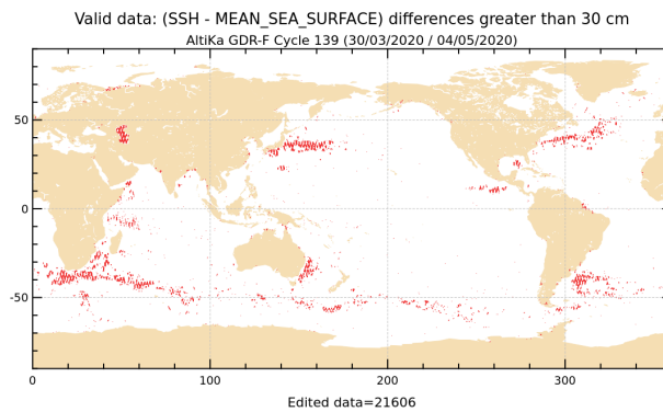
Figure 20: Sea level anomaly relative to MSS for cycle 139.
