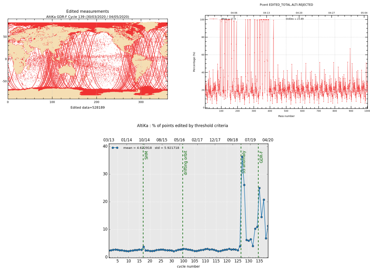
Figure 2: Rejected measurements on thresholds criteria : Cycle 139, map and monitoring of % of rejected measurements per track (top), whole time serie / % of rejected measurements per cycle (bottom).
