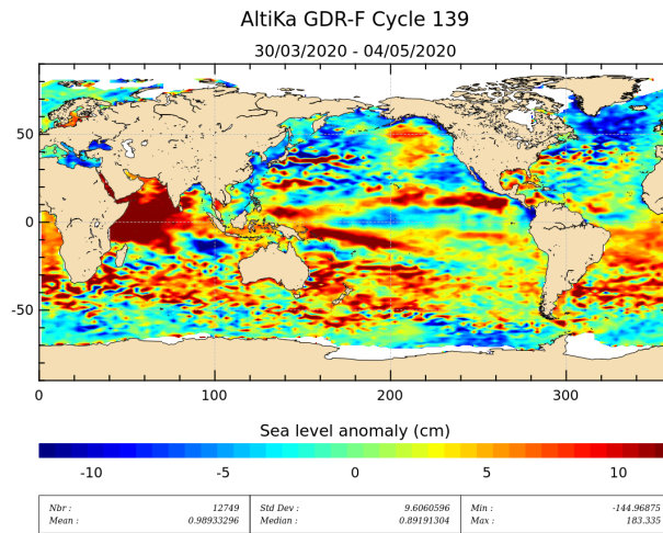
Figure 20: Sea level anomaly relative to MSS for cycle 139.
