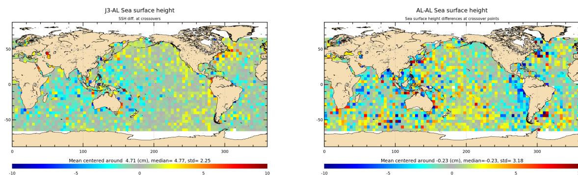
Figure 15: Mean of multi-mission SSH and mono-mission SSH differences at crossovers for cycle 139.
