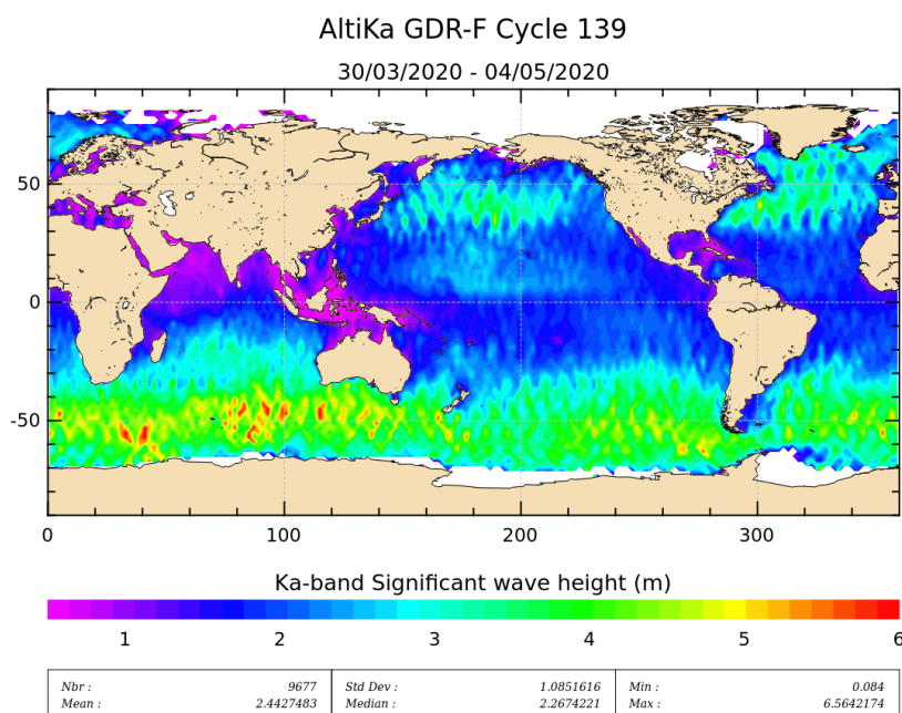
Figure 6: Significant wave height for cycle 139.
