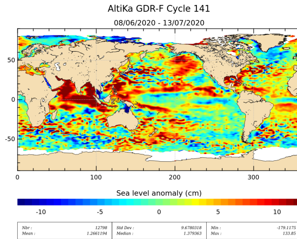
Figure 19: Sea level anomaly relative to MSS for cycle 141.
