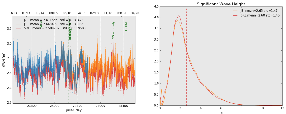
Figure 6: Daily monitoring of significant wave height for AltiKa (Ka-band) Jason-2 and Jason-3 (Ku-band) on the left and histogram for cycle 141 on the right (limited to 66° latitude).
