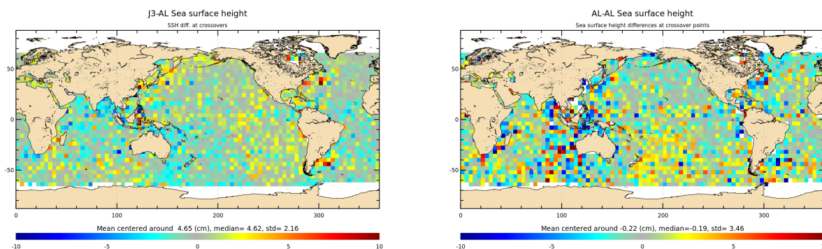
Figure 14: Mean of multi-mission SSH and mono-mission SSH differences at crossovers for cycle 141.
