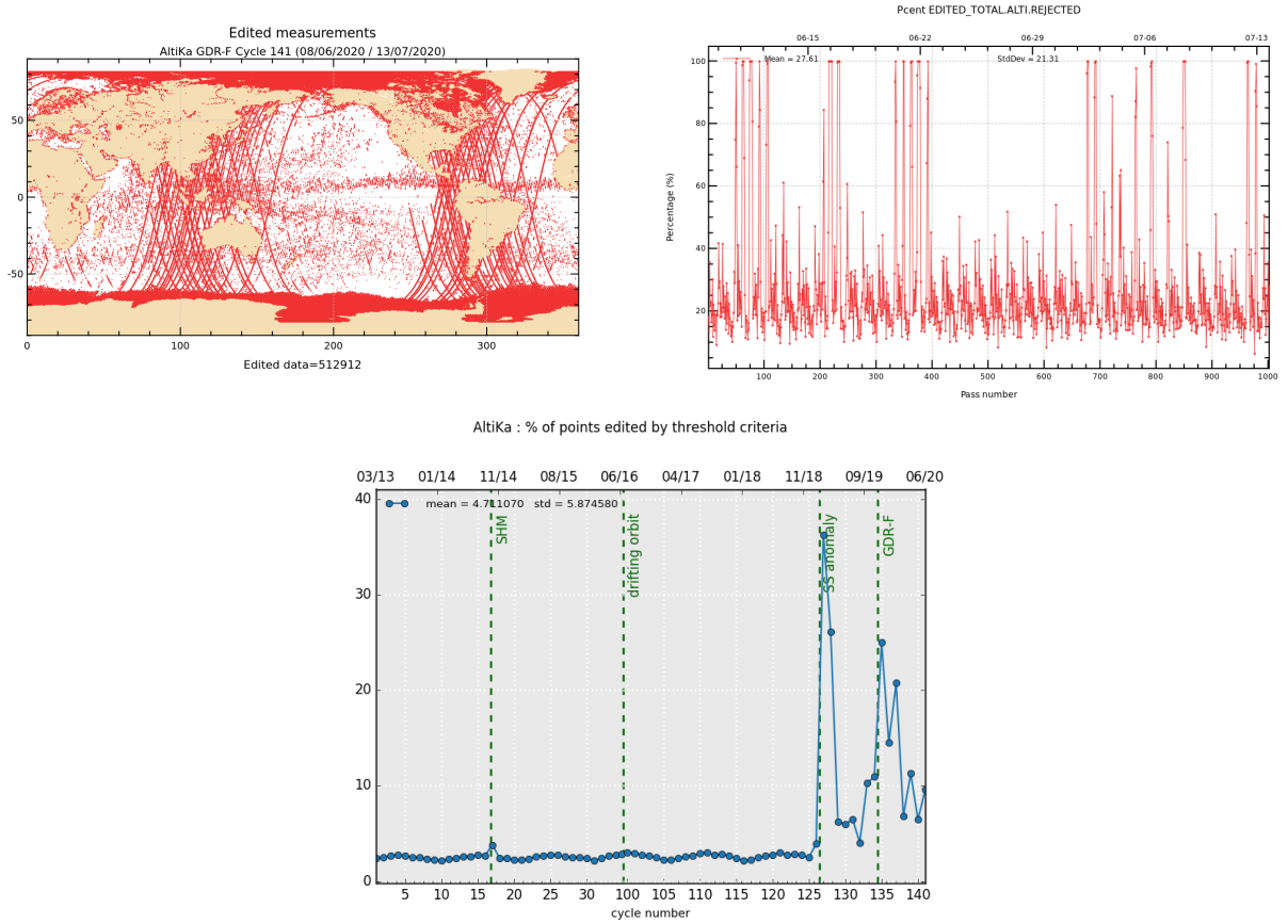
Figure 2: Rejected measurements on thresholds criteria : Cycle 141, map and monitoring of % of rejected measurements per track (top), whole time serie / % of rejected measurements per cycle (bottom).
