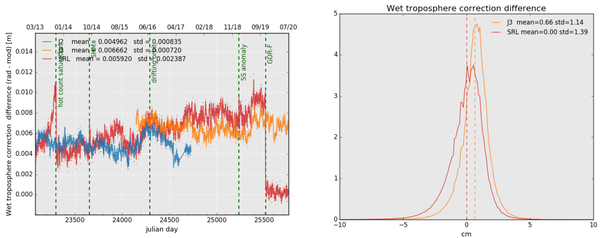
Figure 12: Daily monitoring of wet troposphere differences (Radiometer-ECMWF model) for Saral/AltiKa Jason-2 and Jason-3 (left) and histogram on the right (limited to 66° latitude) for cycle 141 .
