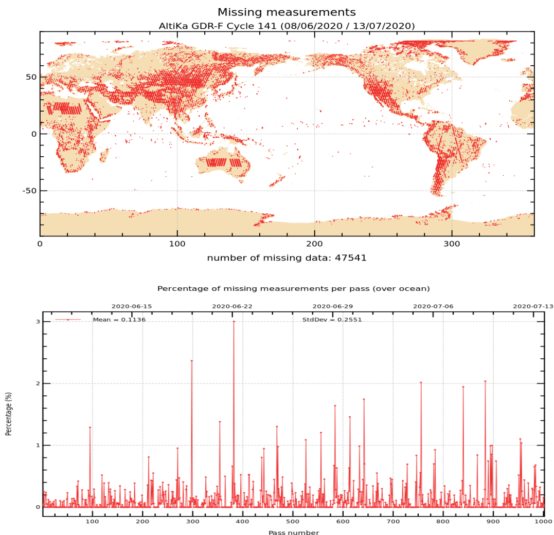
Figure 1: Map of missing measurements for cycle 141 on top. Monitoring of percentage of missing ocean measurements per pass on bottom.
