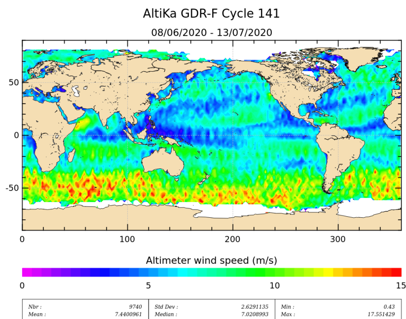
Figure 9: Altimeter wind speed for cycle 141.
