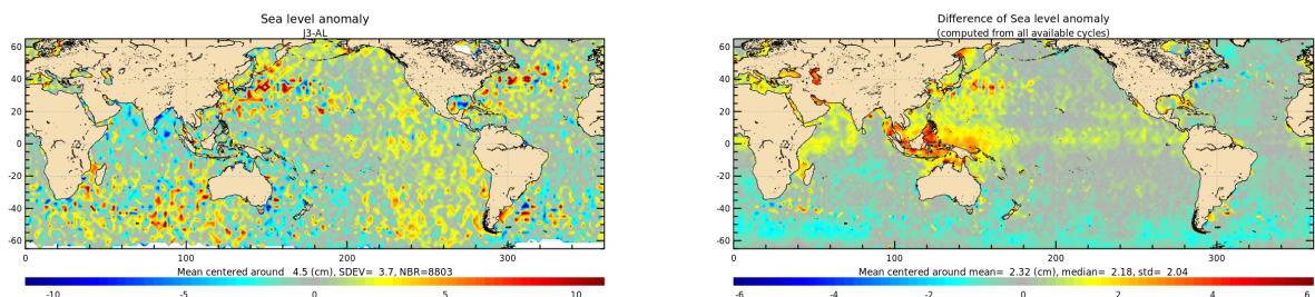
Figure 21: Jason-3 – Saral/AltiKa SLA differences for cycle 141 (left) and averaged over the whole Saral/AltiKa period (right).
