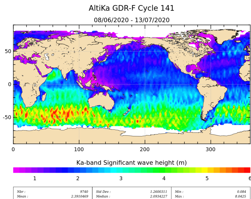
Figure 5: Significant wave height for cycle 141.
