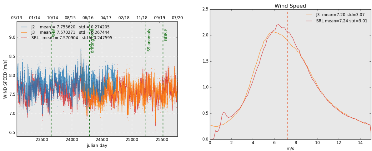
Figure 10: Daily monitoring of altimeter wind speed for Saral/AltiKa, Jason-2 and Jason-3 on the left and histogram for cycle 141 on the right (limited to 66° latitude).
