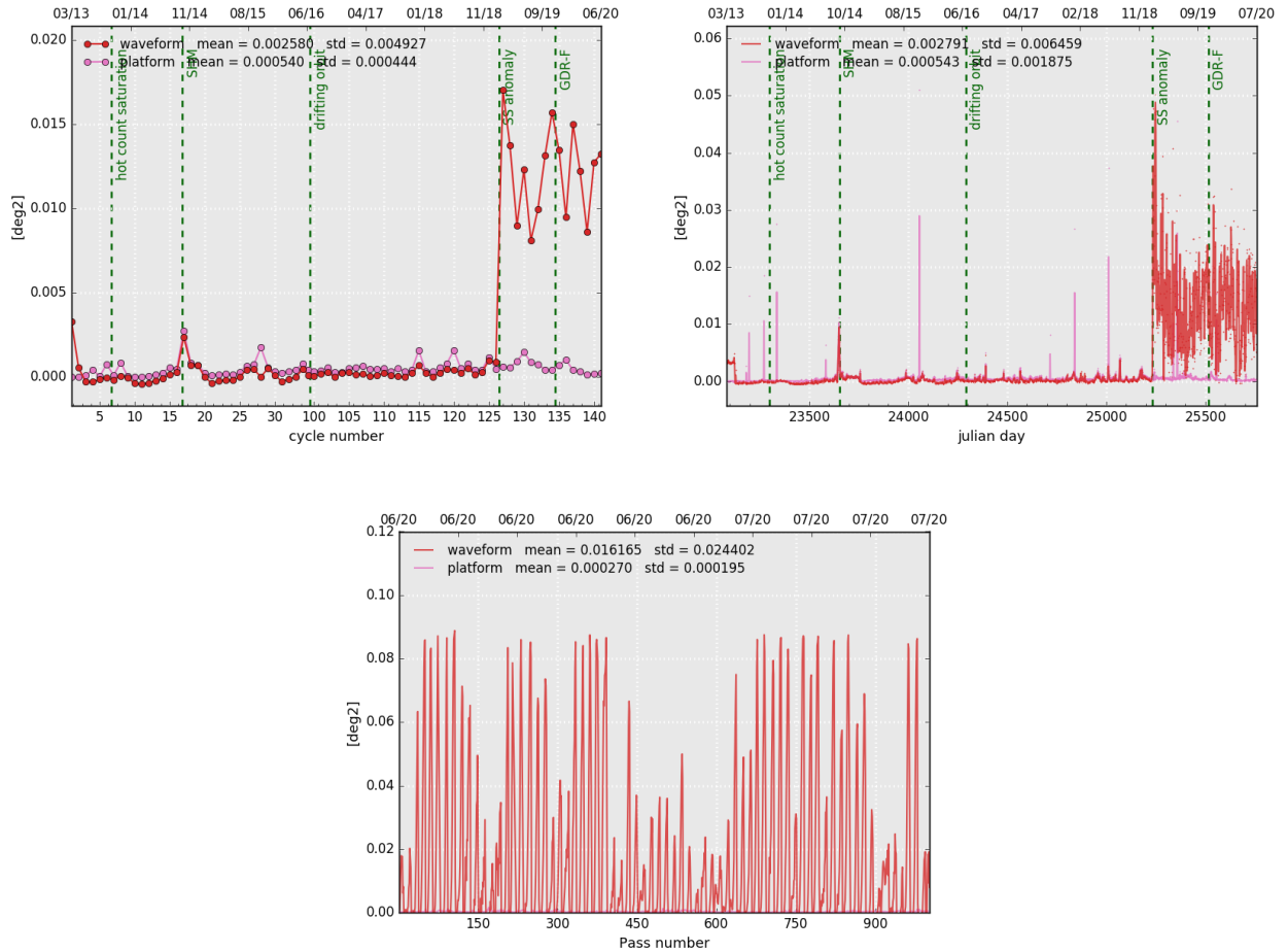
Figure 13: Cyclic monitoring(left), daily monitoring(right) and monitoring per pass for cycle 141 (bottom) of SARAL/AltiKa's mispointing angle: comparison between the one derived from waveform retracking and the one measured by platform startrackers.
