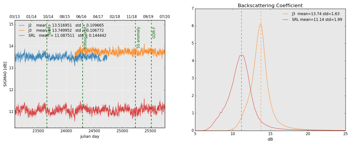
Figure 7: Daily monitoring of backscattering coefficient for Saral/AltiKa, Jason-2 and Jason-3 on the left and histogram for cycle 141 on the right (limited to 66° latitude).
