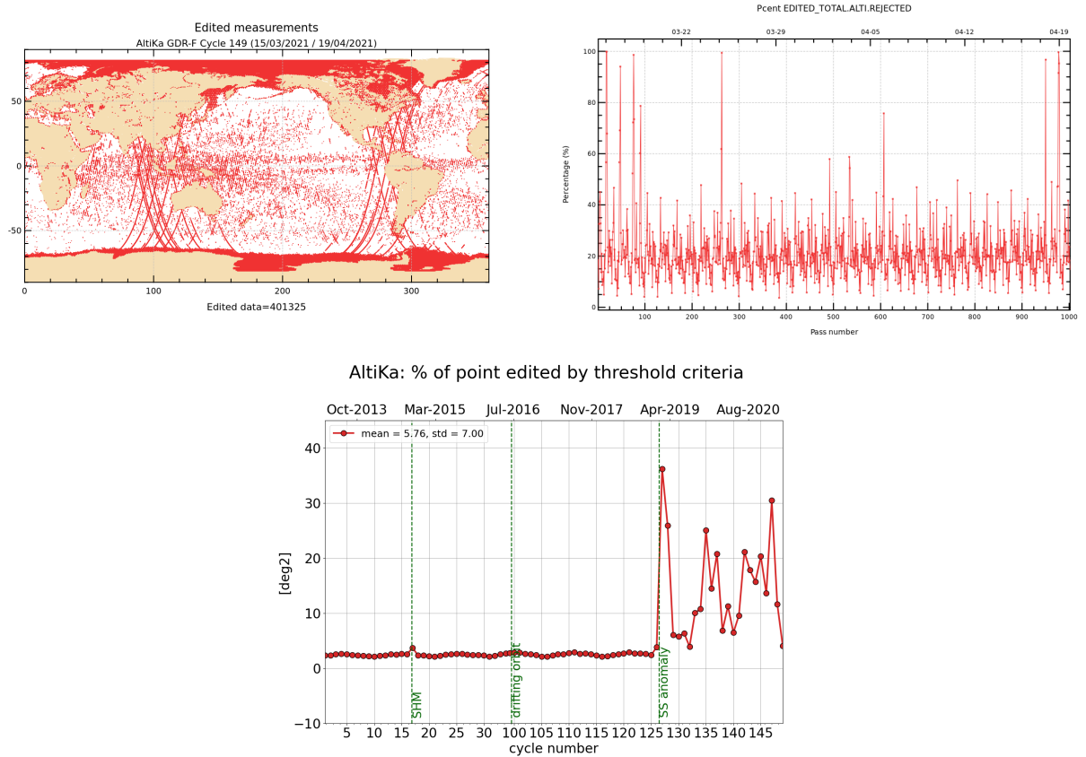
Figure 2: Rejected measurements on thresholds criteria : Cycle 149, map and monitoring of % of rejected measurements per track (top), whole time serie / % of rejected measurements per cycle (bottom).
