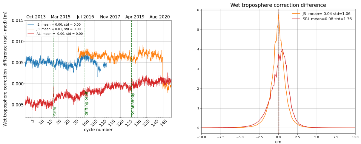
Figure 12: Daily monitoring of wet troposphere differences (Radiometer-ECMWF model) for Saral/AltiKa Jason-2 and Jason-3 (left) and histogram on the right (limited to 66° latitude) for cycle 149 .
