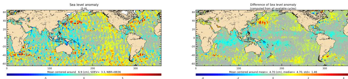
Figure 21: Jason-3 – Saral/AltiKa SLA differences for cycle 149 (left) and averaged over the whole Saral/AltiKa period (right).
