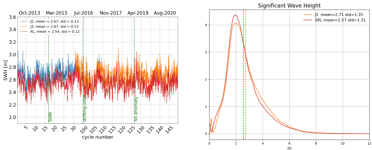
Figure 6: Daily monitoring of significant wave height for AltiKa (Ka-band) Jason-2 and Jason-3 (Ku-band) on the left and histogram for cycle 149 on the right (limited to 66^\circ latitude).
