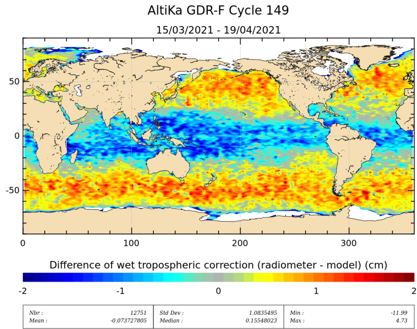
Figure 11: Mean of wet troposphere correction difference (Radiometer-ECMWF model) for cycle 149.
