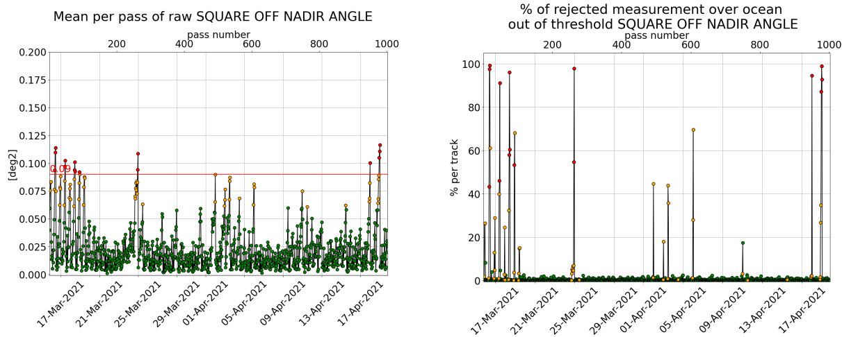
Figure 3: [left] Mispointing cycle 149, [right] Percentage of rejected measurement by threshold on square off-nadir angle.
