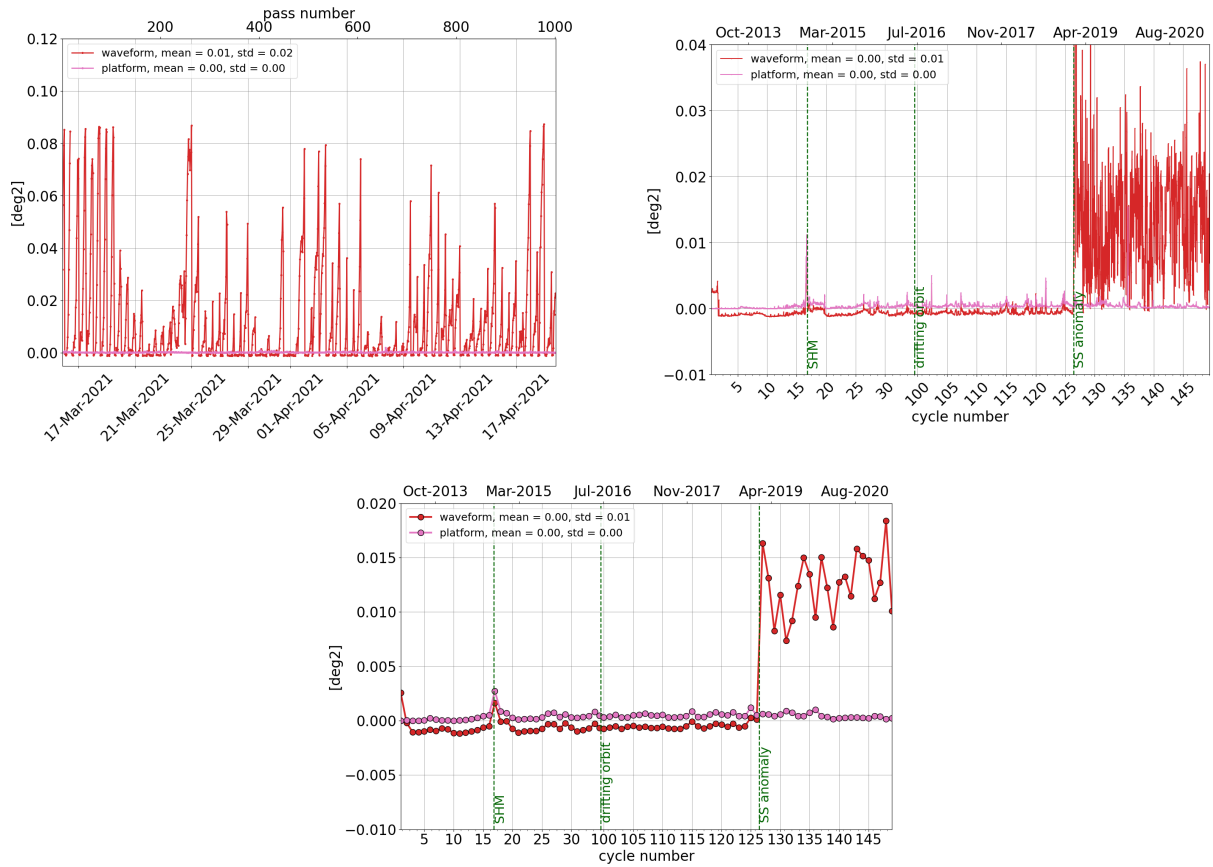
Figure 13: Monitoring per pass for cycle 149 (left), daily monitoring(right) and cyclic monitoring (bottom) of SARAL/AltiKa's mispointing angle: comparison between the one derived from waveform retracking and the one measured by platform startrackers.
