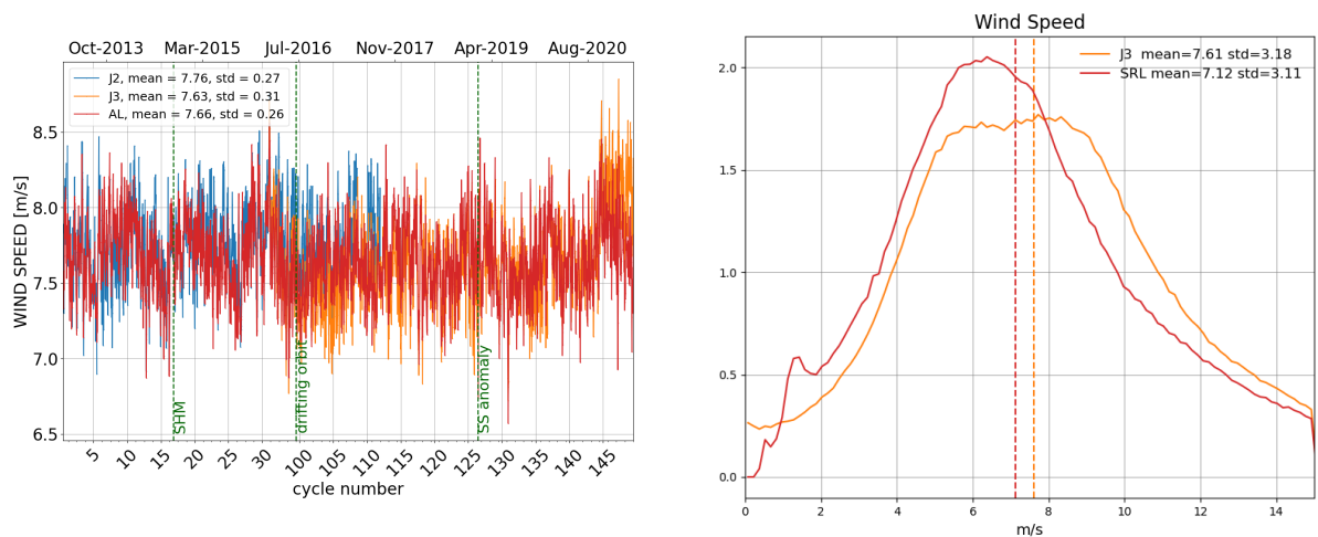
Figure 10: Daily monitoring of altimeter wind speed for Saral/AltiKa, Jason-2 and Jason-3 on the left and histogram for cycle 149 on the right (limited to 66° latitude).
