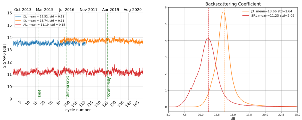
Figure 7: Daily monitoring of backscattering coefficient for Saral/AltiKa, Jason-2 and Jason-3 on the left and histogram for cycle 149 on the right (limited to 66° latitude).
