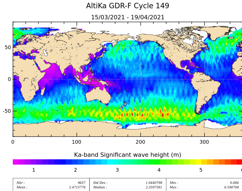
Figure 5: Significant wave height for cycle 149.
