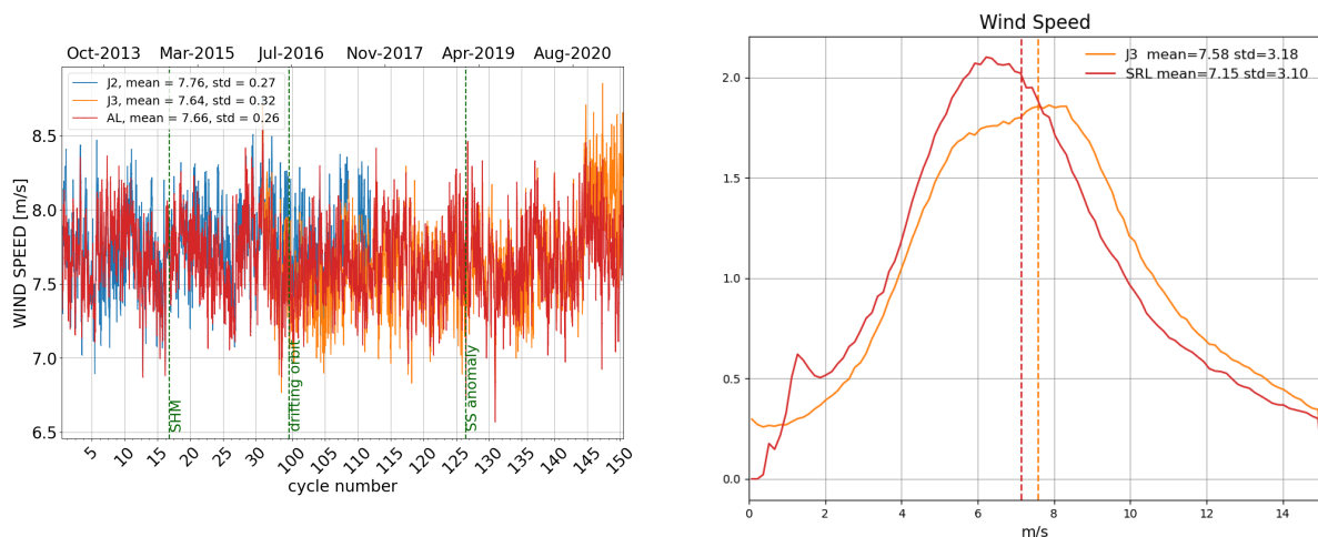
Figure 10: Daily monitoring of altimeter wind speed for Saral/AltiKa, Jason-2 and Jason-3 on the left and histogram for cycle 150 on the right (limited to 66° latitude).
