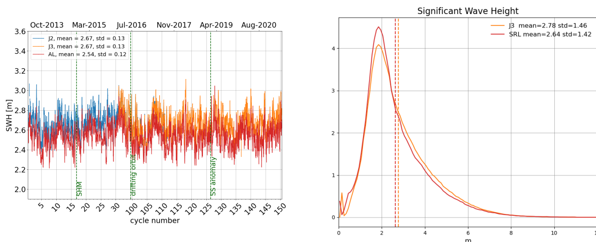
Figure 6: Daily monitoring of significant wave height for AltiKa (Ka-band) Jason-2 and Jason-3 (Ku-band) on the left and histogram for cycle 150 on the right (limited to 66^\circ latitude).
