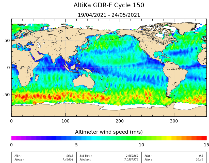
Figure 9: Altimeter wind speed for cycle 150.
