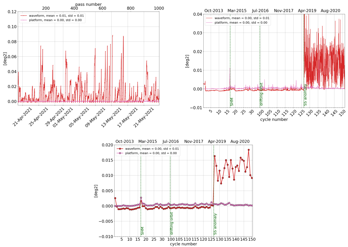
Figure 13: Monitoring per pass for cycle 150 (left), daily monitoring(right) and cyclic monitoring (bottom) of SARAL/AltiKa's mispointing angle: comparison between the one derived from waveform retracking and the one measured by platform startrackers.
