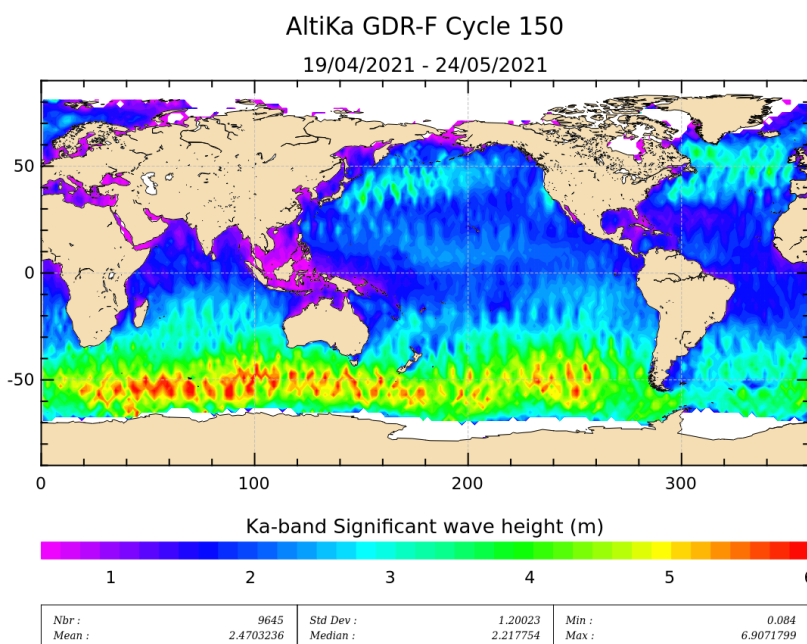
Figure 5: Significant wave height for cycle 150.
