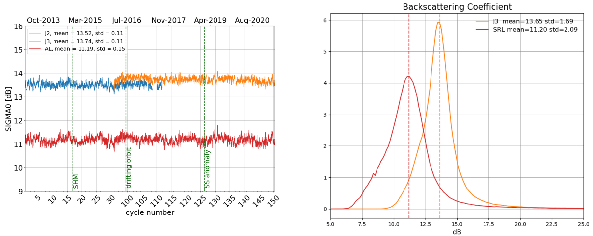
Figure 7: Daily monitoring of backscattering coefficient for Saral/AltiKa, Jason-2 and Jason-3 on the left and histogram for cycle 150 on the right (limited to 66° latitude).
