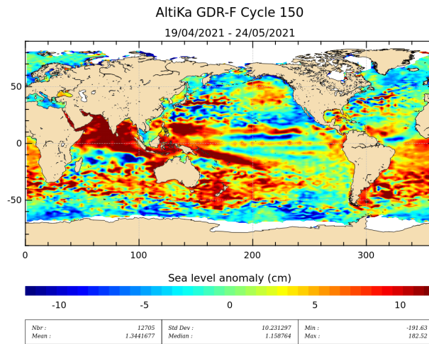
Figure 19: Sea level anomaly relative to MSS for cycle 150.
