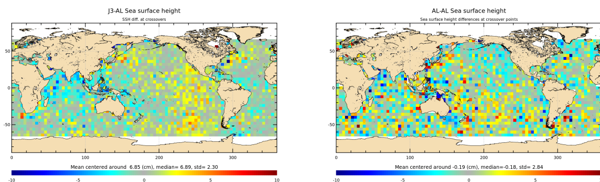
Figure 14: Mean of multi-mission SSH and mono-mission SSH differences at crossovers for cycle 150.
