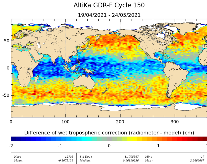
Figure 11: Mean of wet troposphere correction difference (Radiometer-ECMWF model) for cycle 150.
