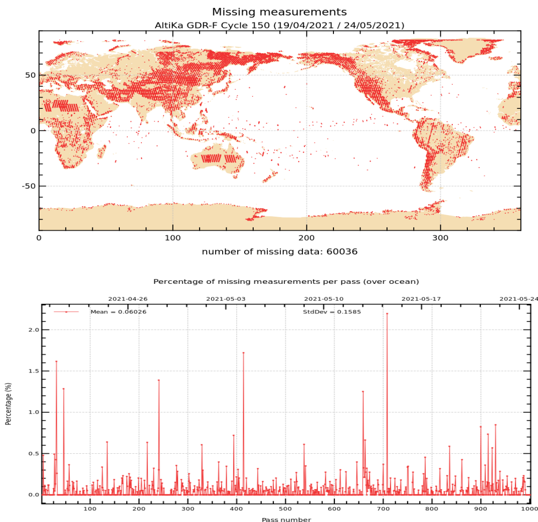
Figure 1: Map of missing measurements for cycle 150 on top. Monitoring of percentage of missing ocean measurements per pass on bottom.
