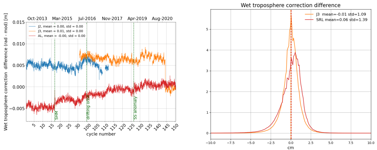
Figure 12: Daily monitoring of wet troposphere differences (Radiometer-ECMWF model) for Saral/AltiKa Jason-2 and Jason-3 (left) and histogram on the right (limited to 66° latitude) for cycle 150 .
