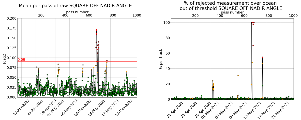
Figure 3: [left] Mispointing cycle 150, [right] Percentage of rejected measurement by threshold on square off-nadir angle.
