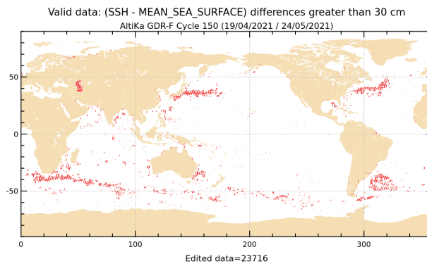
Figure 20: SLA higher than 30 cm for cycle 150.
