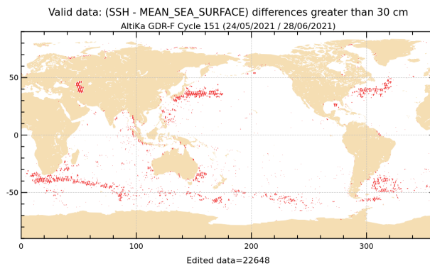
Figure 20: SLA higher than 30 cm for cycle 151.
