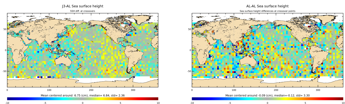
Figure 14: Mean of multi-mission SSH and mono-mission SSH differences at crossovers for cycle 151.
