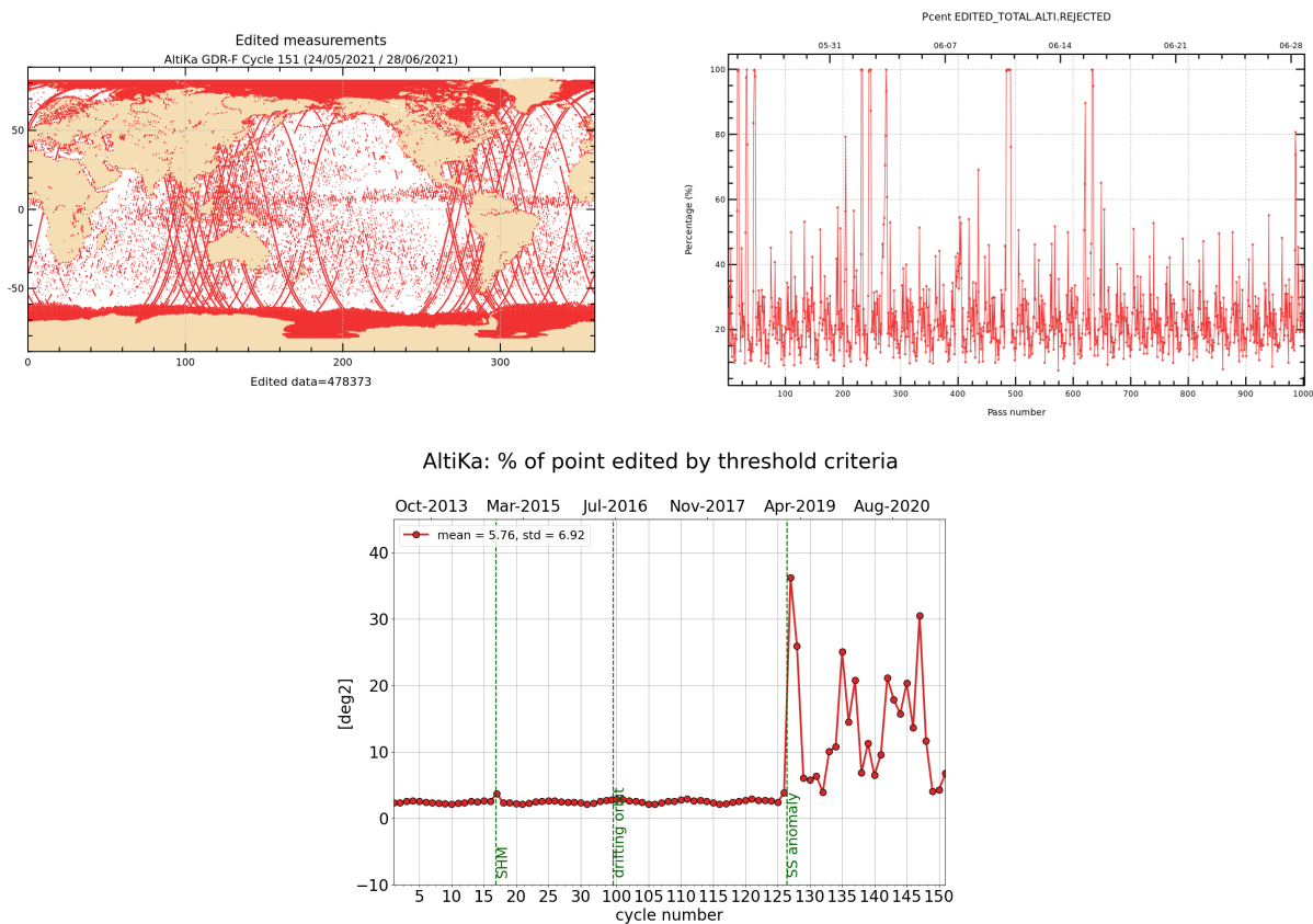
Figure 2: Rejected measurements on thresholds criteria : Cycle 151, map and monitoring of % of rejected measurements per track (top), whole time serie / % of rejected measurements per cycle (bottom).
