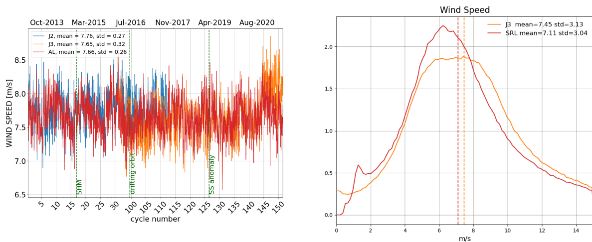
Figure 10: Daily monitoring of altimeter wind speed for Saral/AltiKa, Jason-2 and Jason-3 on the left and histogram for cycle 151 on the right (limited to 66° latitude).
