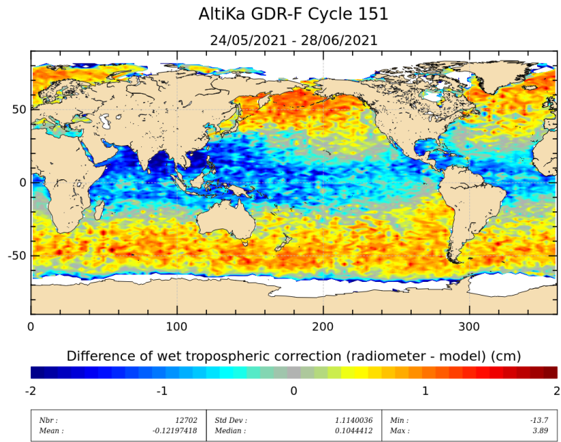
Figure 11: Mean of wet troposphere correction difference (Radiometer-ECMWF model) for cycle 151.
