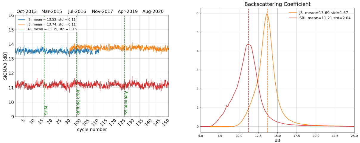
Figure 7: Daily monitoring of backscattering coefficient for Saral/AltiKa, Jason-2 and Jason-3 on the left and histogram for cycle 151 on the right (limited to 66° latitude).
