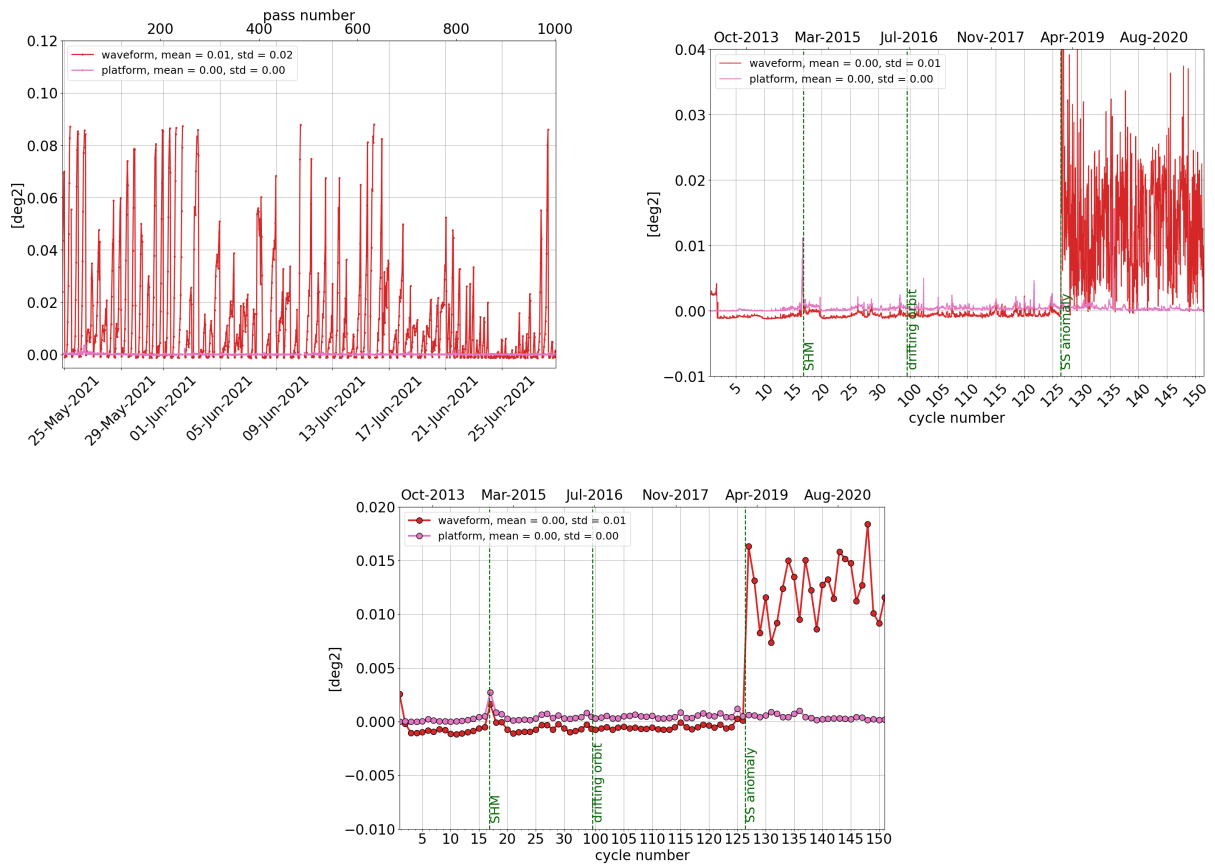
Figure 13: Monitoring per pass for cycle 151 (left), daily monitoring(right) and cyclic monitoring (bottom) of SARAL/AltiKa's mispointing angle: comparison between the one derived from waveform retracking and the one measured by platform startrackers.
