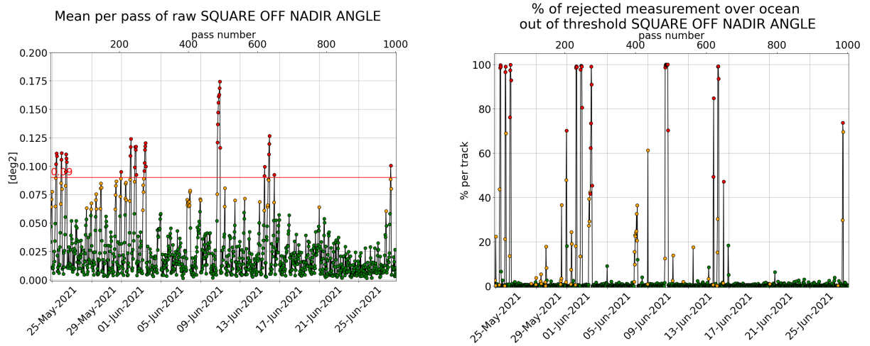
Figure 3: [left] Mispointing cycle 151, [right] Percentage of rejected measurement by threshold on square off-nadir angle.
