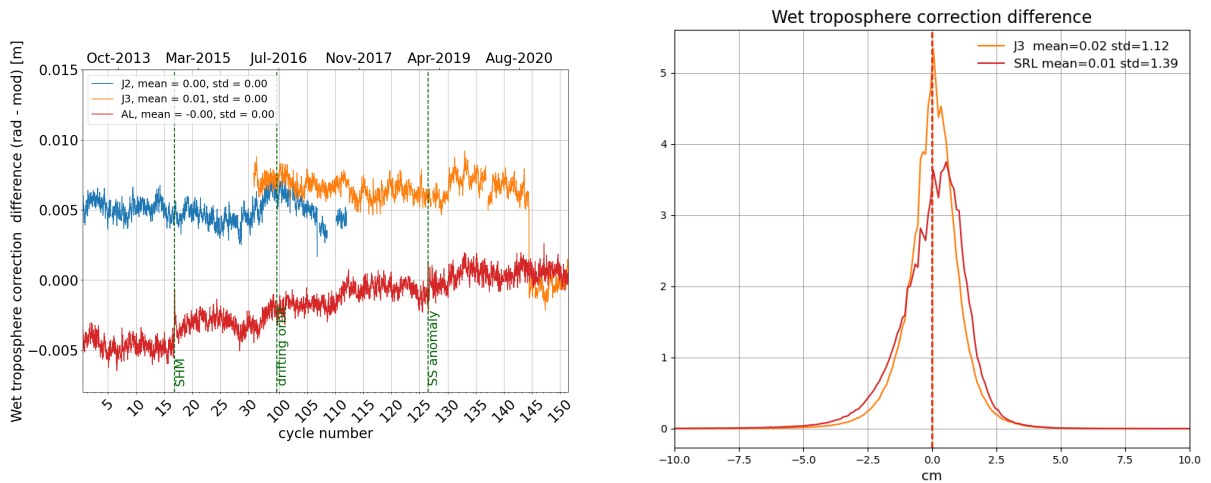
Figure 12: Daily monitoring of wet troposphere differences (Radiometer-ECMWF model) for Saral/AltiKa Jason-2 and Jason-3 (left) and histogram on the right (limited to 66° latitude) for cycle 151 .
