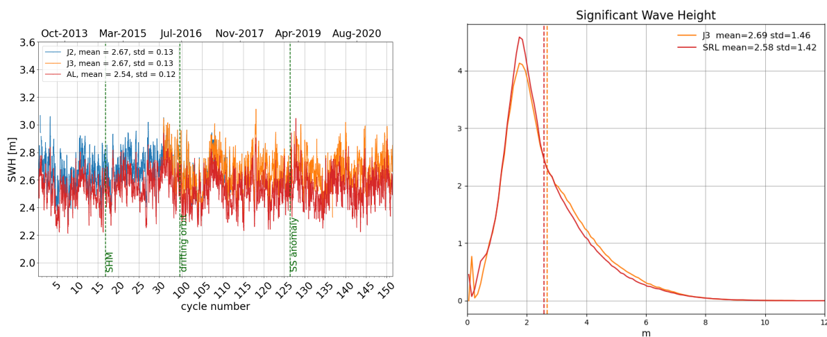
Figure 6: Daily monitoring of significant wave height for AltiKa (Ka-band) Jason-2 and Jason-3 (Ku-band) on the left and histogram for cycle 151 on the right (limited to 66° latitude).
