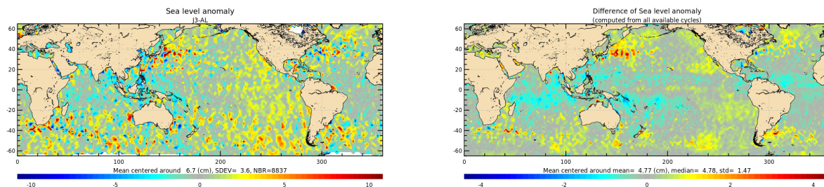
Figure 21: Jason-3 – Saral/AltiKa SLA differences for cycle 151 (left) and averaged over the whole Saral/AltiKa period (right).
