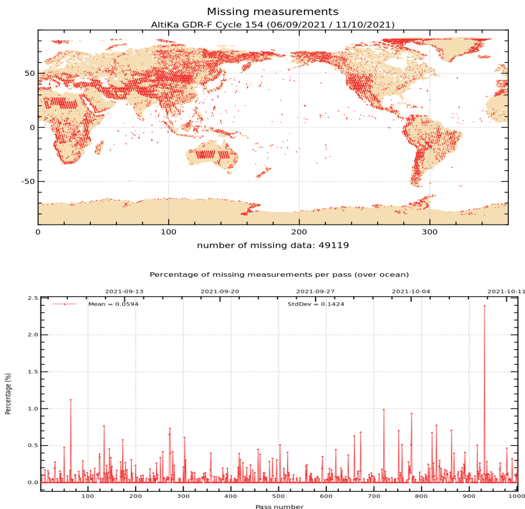
Figure 1: Map of missing measurements for cycle 154 on top. Monitoring of percentage of missing ocean measurements per pass on bottom.
