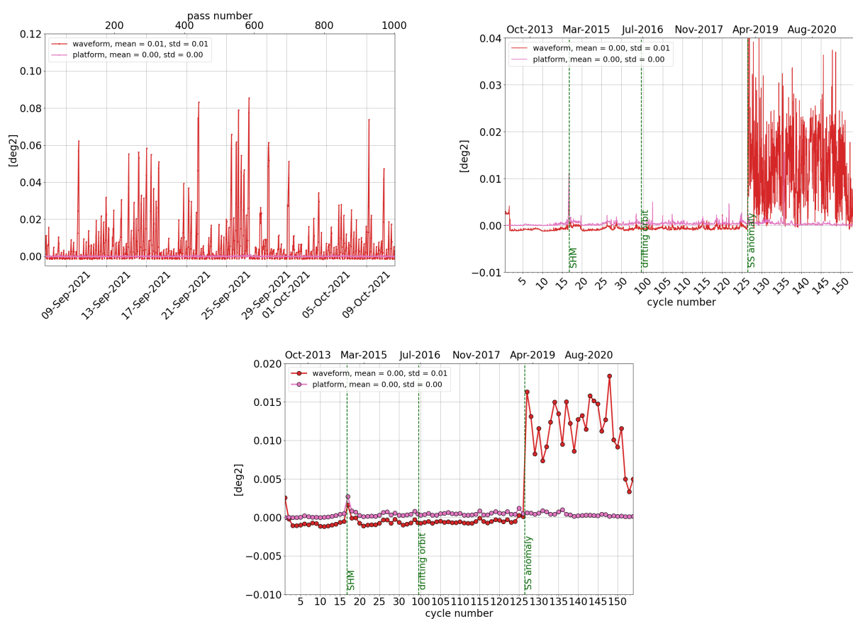
Figure 13: Monitoring per pass for cycle 154 (left), daily monitoring(right) and cyclic monitoring (bottom) of SARAL/AltiKa's mispointing angle: comparison between the one derived from waveform retracking and the one measured by platform startrackers.
