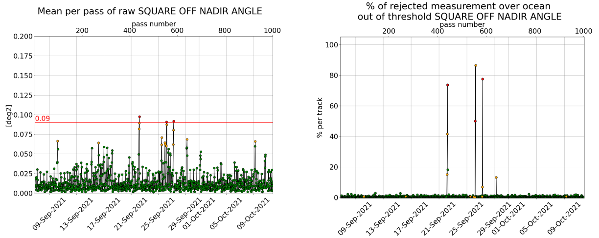
Figure 3: [left] Mispointing cycle 154, [right] Percentage of rejected measurement by threshold on square off-nadir angle.
