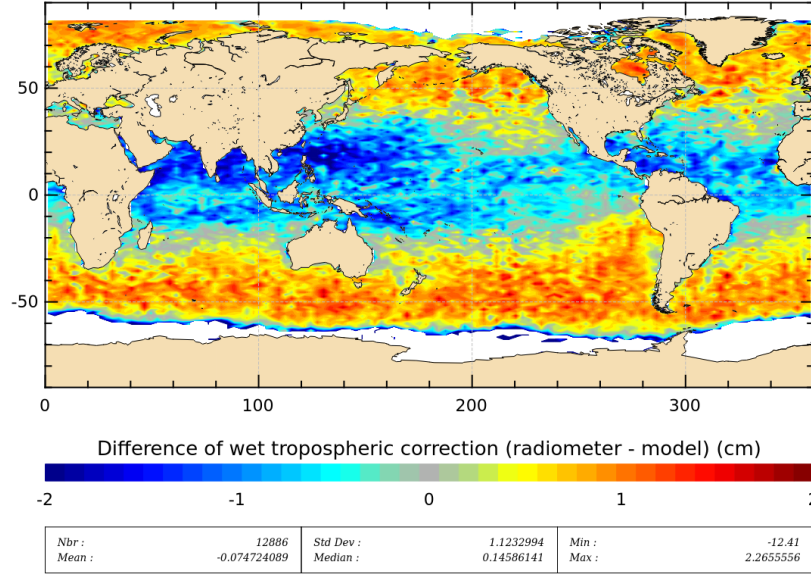
Figure 11: Mean of wet troposphere correction difference (Radiometer-ECMWF model) for cycle 154.
