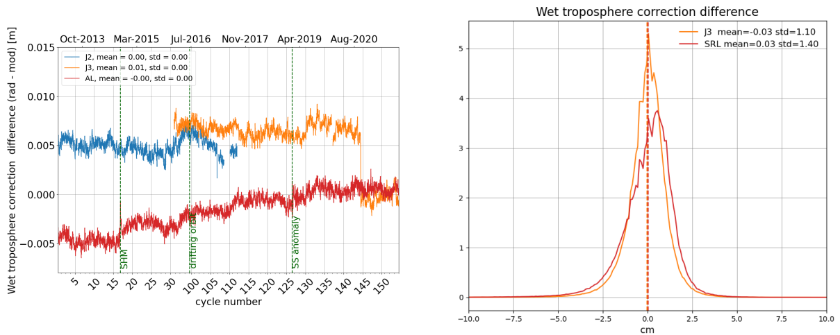
Figure 12: Daily monitoring of wet troposphere differences (Radiometer-ECMWF model) for Saral/AltiKa Jason-2 and Jason-3 (left) and histogram on the right (limited to 66° latitude) for cycle 154 .
