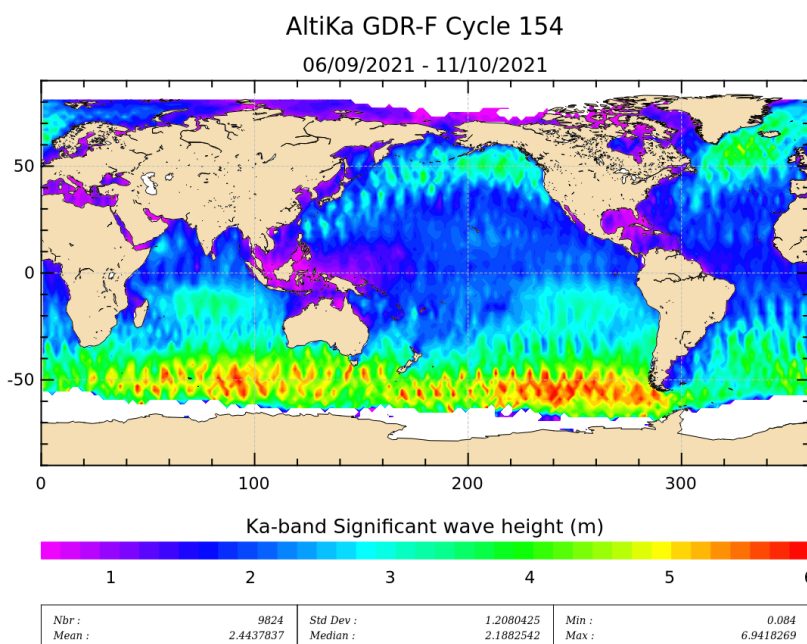
Figure 5: Significant wave height for cycle 154.
