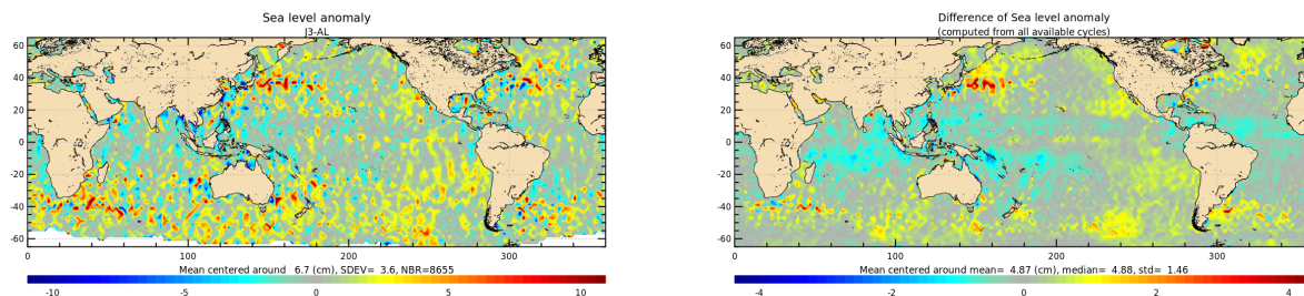
Figure 21: Jason-3 – Saral/AltiKa SLA differences for cycle 154 (left) and averaged over the whole Saral/AltiKa period (right).
