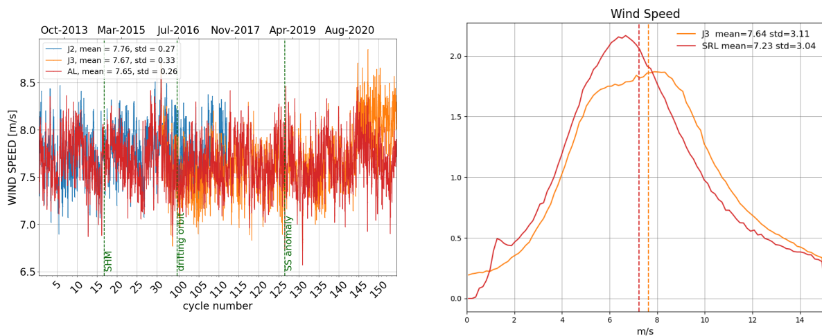
Figure 10: Daily monitoring of altimeter wind speed for Saral/AltiKa, Jason-2 and Jason-3 on the left and histogram for cycle 154 on the right (limited to 66° latitude).
