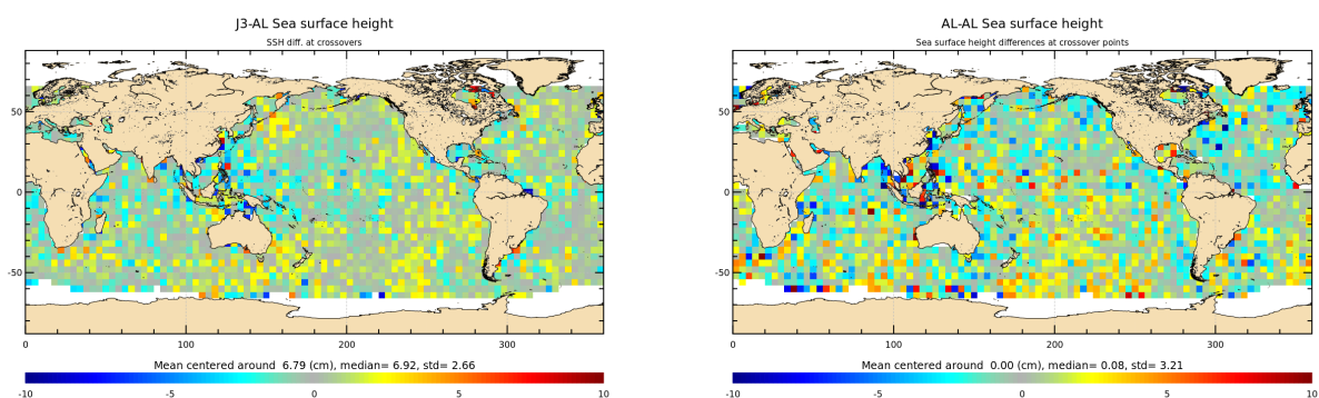
Figure 14: Mean of multi-mission SSH and mono-mission SSH differences at crossovers for cycle 154.
