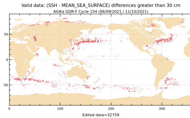
Figure 20: SLA higher than 30 cm for cycle 154.
