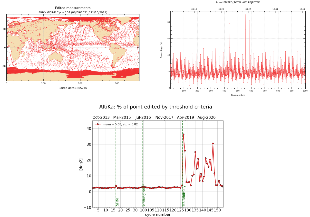
Figure 2: Rejected measurements on thresholds criteria : Cycle 154, map and monitoring of % of rejected measurements per track (top), whole time serie / % of rejected measurements per cycle (bottom).
