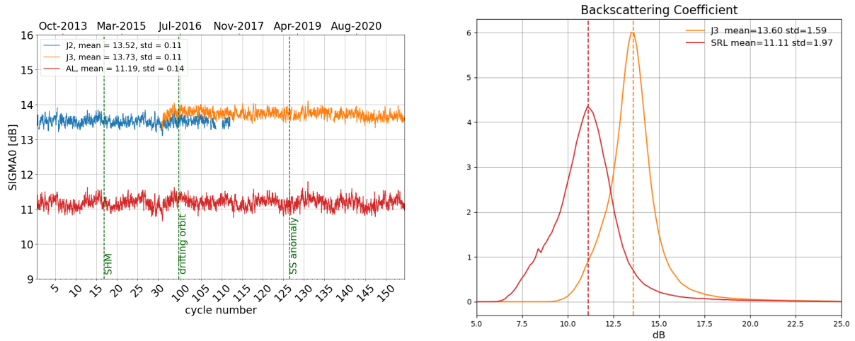
Figure 7: Daily monitoring of backscattering coefficient for Saral/AltiKa, Jason-2 and Jason-3 on the left and histogram for cycle 154 on the right (limited to 66° latitude).
