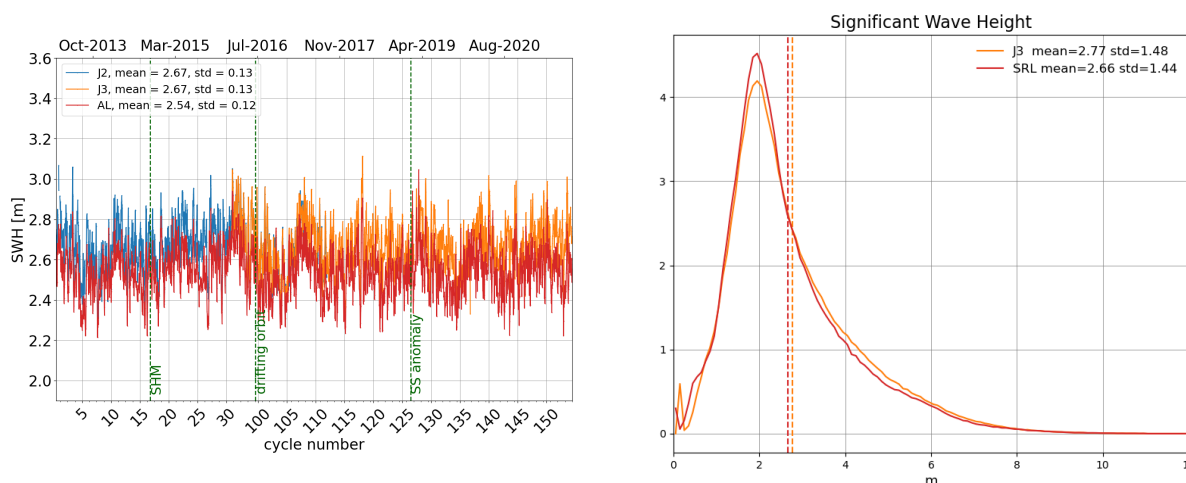
Figure 6: Daily monitoring of significant wave height for AltiKa (Ka-band) Jason-2 and Jason-3 (Ku-band) on the left and histogram for cycle 154 on the right (limited to 66^\circ latitude).
