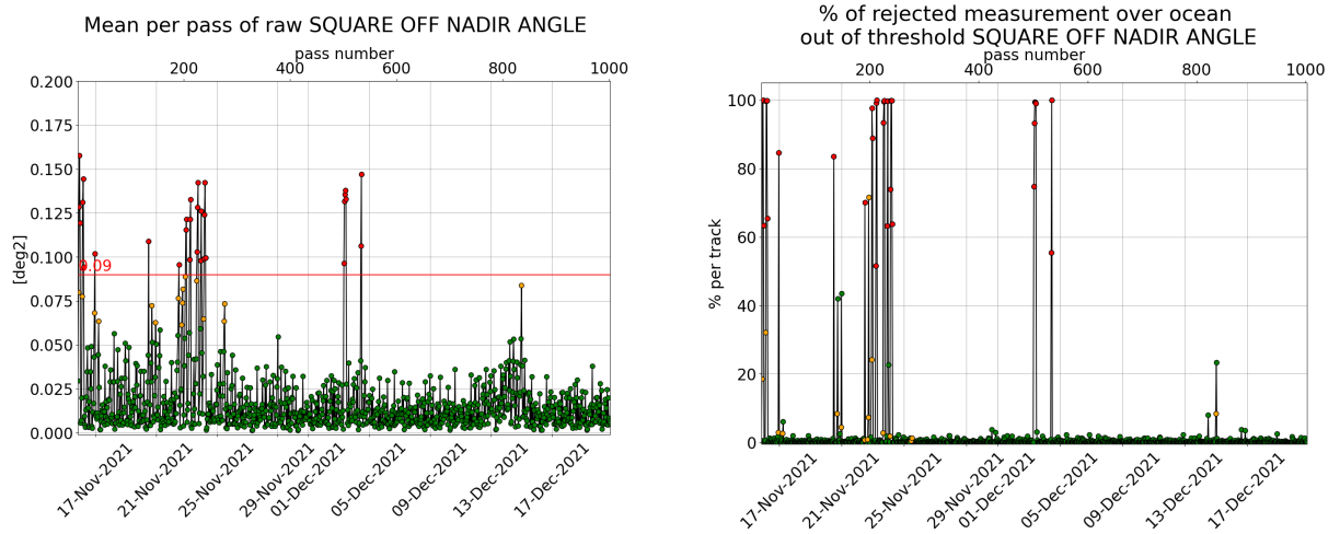
Figure 3: [left] Mispointing cycle 156, [right] Percentage of rejected measurement by threshold on square off-nadir angle.
