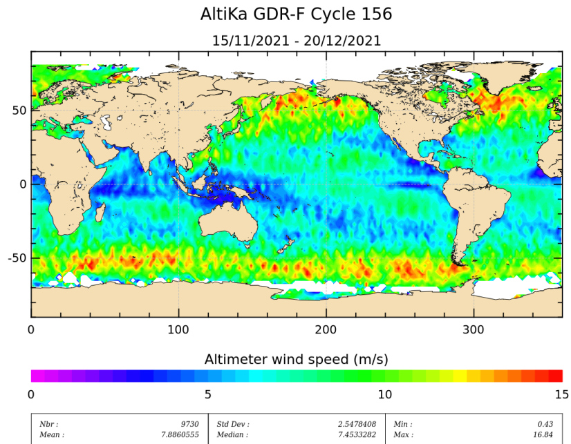
Figure 9: Altimeter wind speed for cycle 156.
