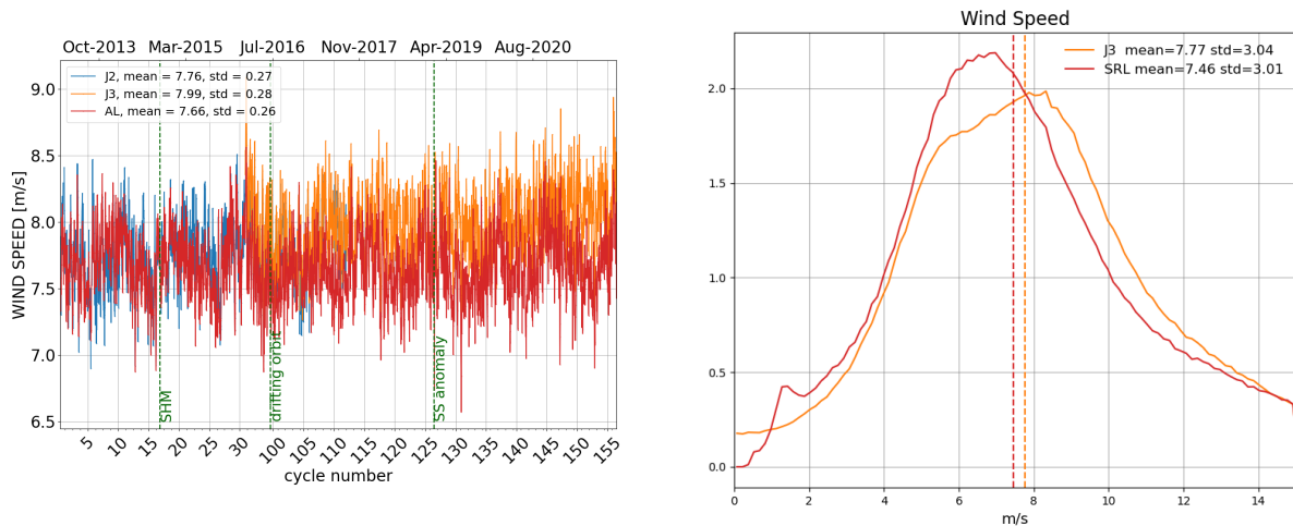
Figure 10: Daily monitoring of altimeter wind speed for Saral/AltiKa, Jason-2 and Jason-3 on the left and histogram for cycle 156 on the right (limited to 66° latitude).
