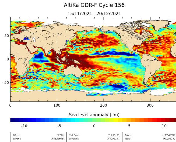
Figure 19: Sea level anomaly relative to MSS for cycle 156.
