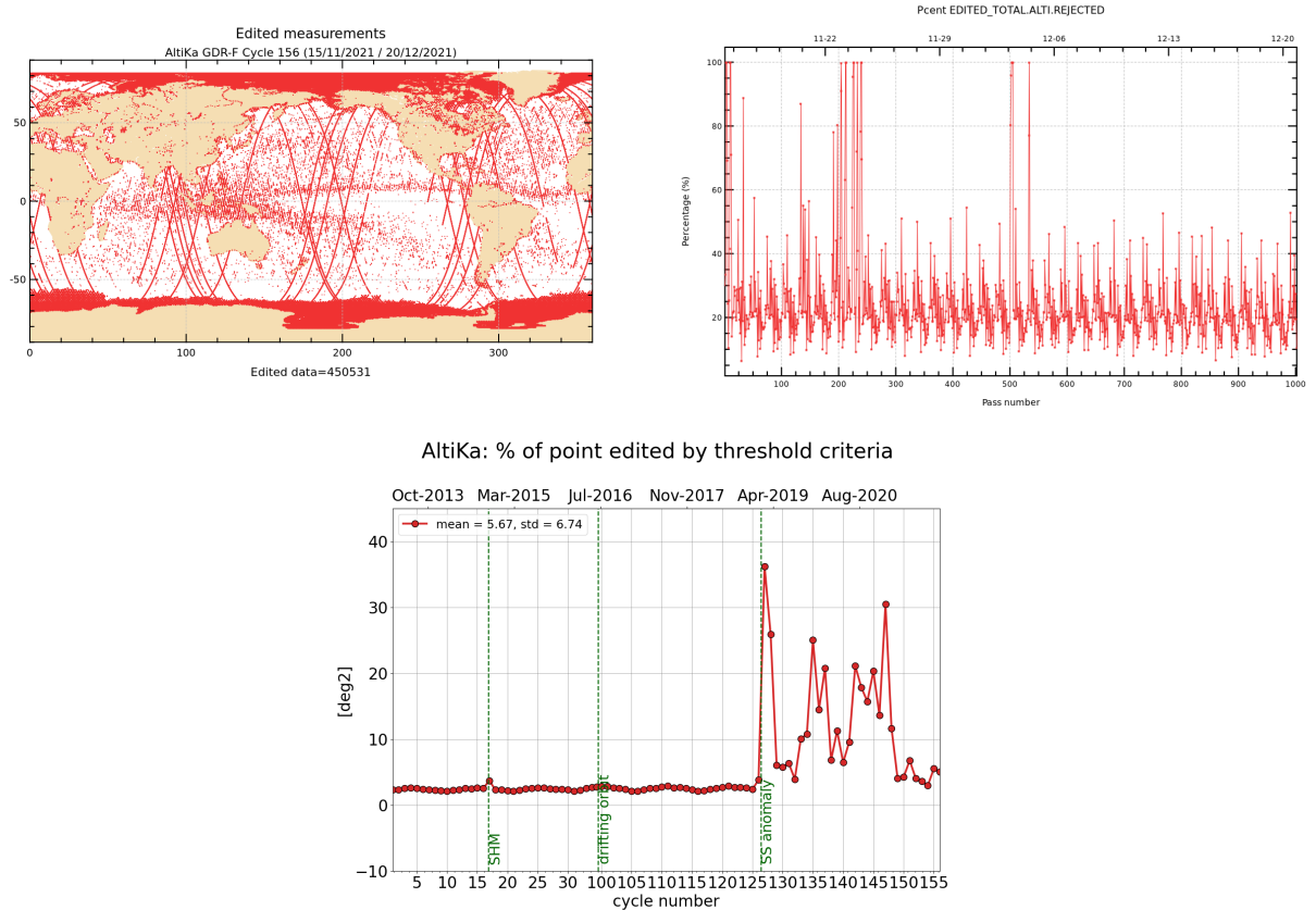
Figure 2: Rejected measurements on thresholds criteria : Cycle 156, map and monitoring of % of rejected measurements per track (top), whole time serie / % of rejected measurements per cycle (bottom).
