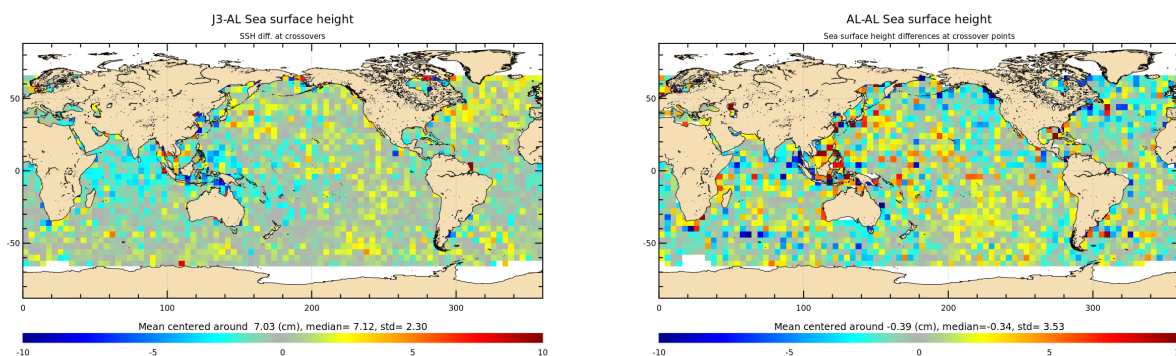
Figure 14: Mean of multi-mission SSH and mono-mission SSH differences at crossovers for cycle 156.
