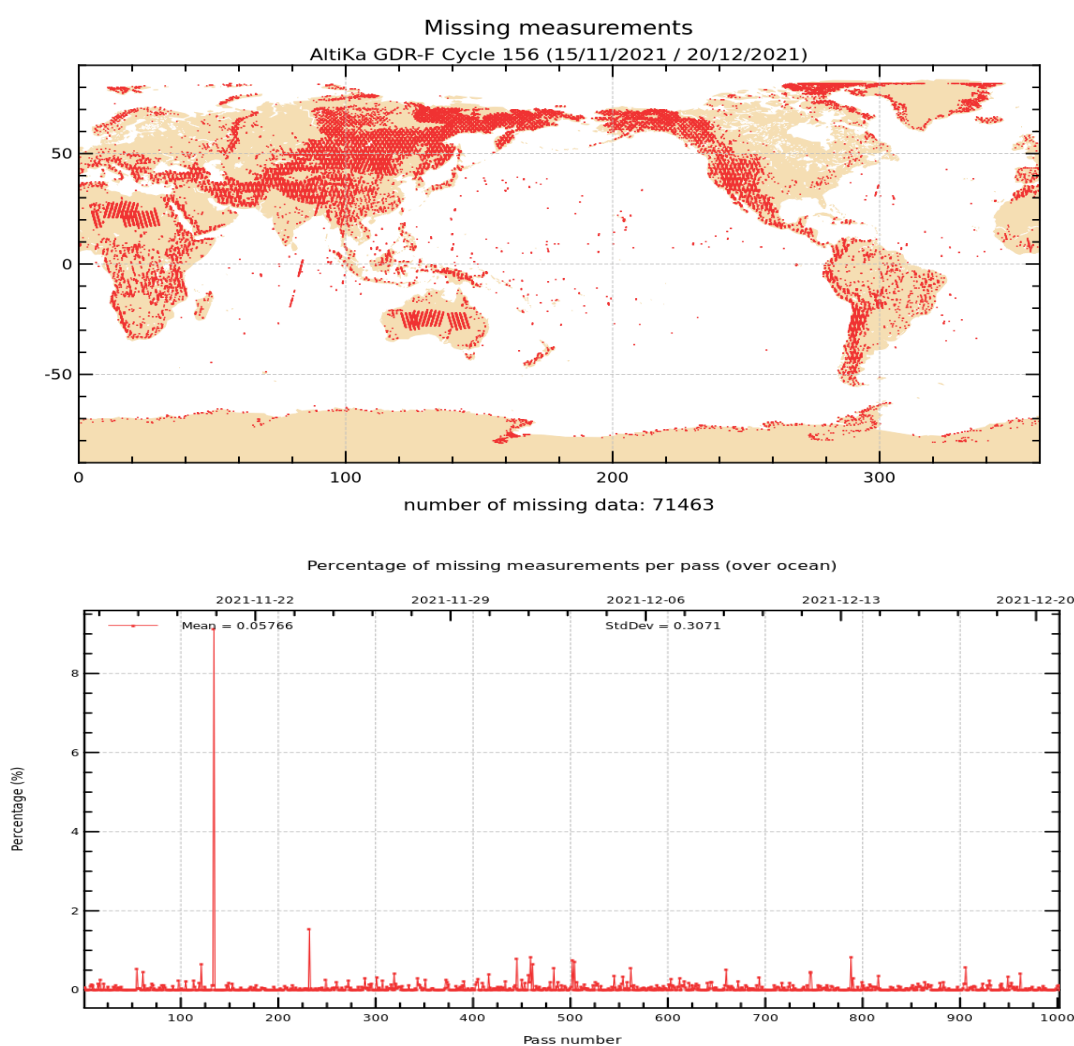
Figure 1: Map of missing measurements for cycle 156 on top. Monitoring of percentage of missing ocean measurements per pass on bottom.
