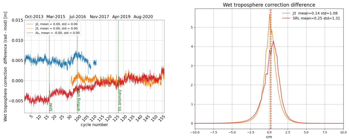
Figure 12: Daily monitoring of wet troposphere differences (Radiometer-ECMWF model) for Saral/AltiKa Jason-2 and Jason-3 (left) and histogram on the right (limited to 66° latitude) for cycle 156 .
