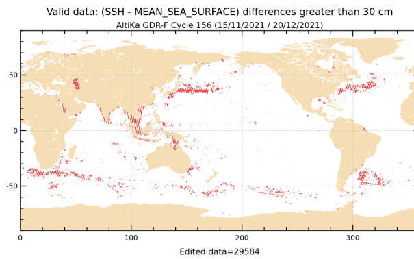
Figure 20: SLA higher than 30 cm for cycle 156.
