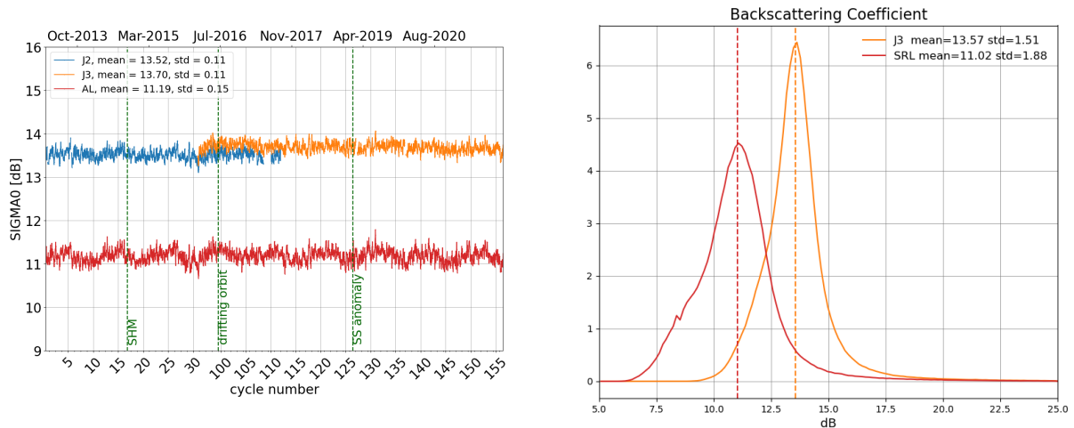
Figure 7: Daily monitoring of backscattering coefficient for Saral/AltiKa, Jason-2 and Jason-3 on the left and histogram for cycle 156 on the right (limited to 66° latitude).
