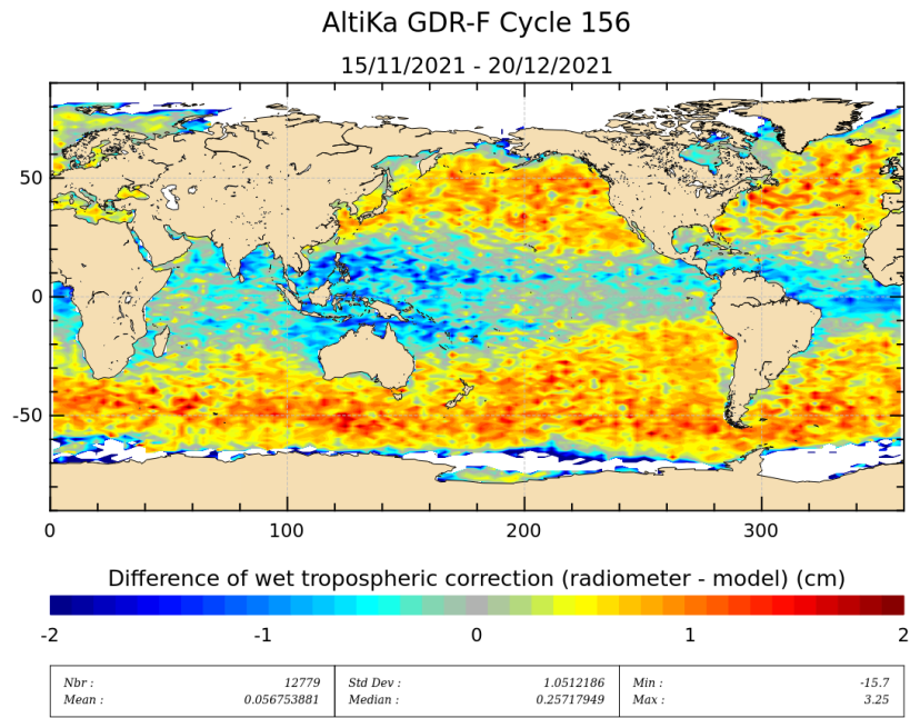
Figure 11: Mean of wet troposphere correction difference (Radiometer-ECMWF model) for cycle 156.
