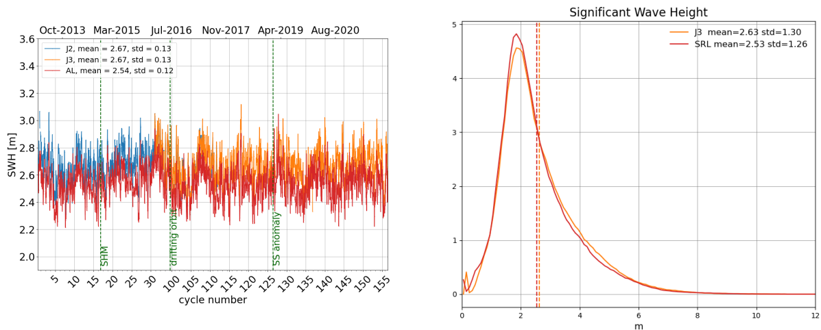
Figure 6: Daily monitoring of significant wave height for AltiKa (Ka-band) Jason-2 and Jason-3 (Ku-band) on the left and histogram for cycle 156 on the right (limited to 66° latitude).
