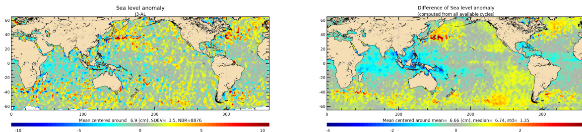
Figure 21: Jason-3 – Saral/AltiKa SLA differences for cycle 156 (left) and averaged over the whole Saral/AltiKa period (right).
