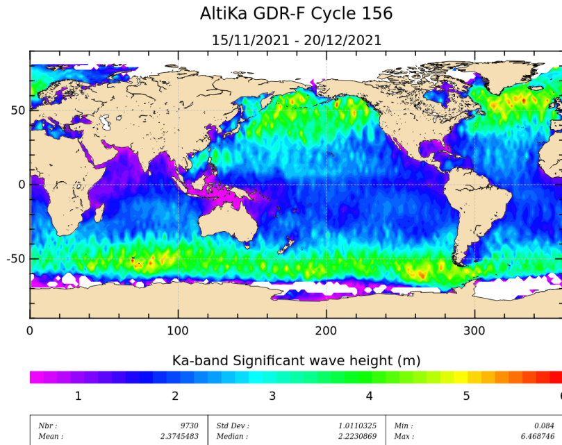
Figure 5: Significant wave height for cycle 156.
