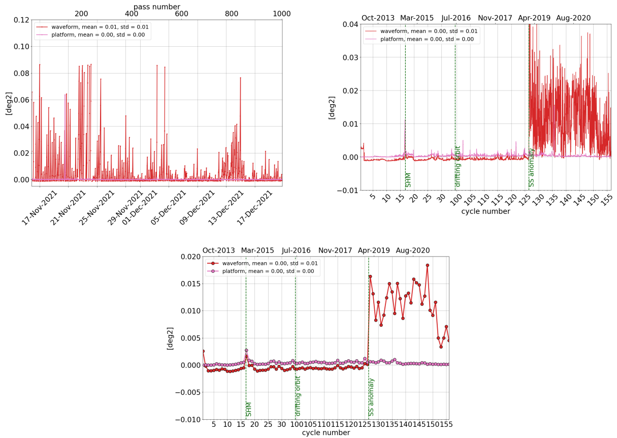
Figure 13: Monitoring per pass for cycle 156 (left), daily monitoring(right) and cyclic monitoring (bottom) of SARAL/AltiKa's mispointing angle: comparison between the one derived from waveform retracking and the one measured by platform startrackers.
