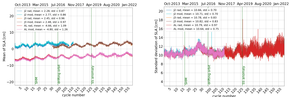
Figure 18: Daily monitoring of the mean (right) and standard deviation (left) of SLA for Saral/AltiKa, Jason-2 and Jason-3.
