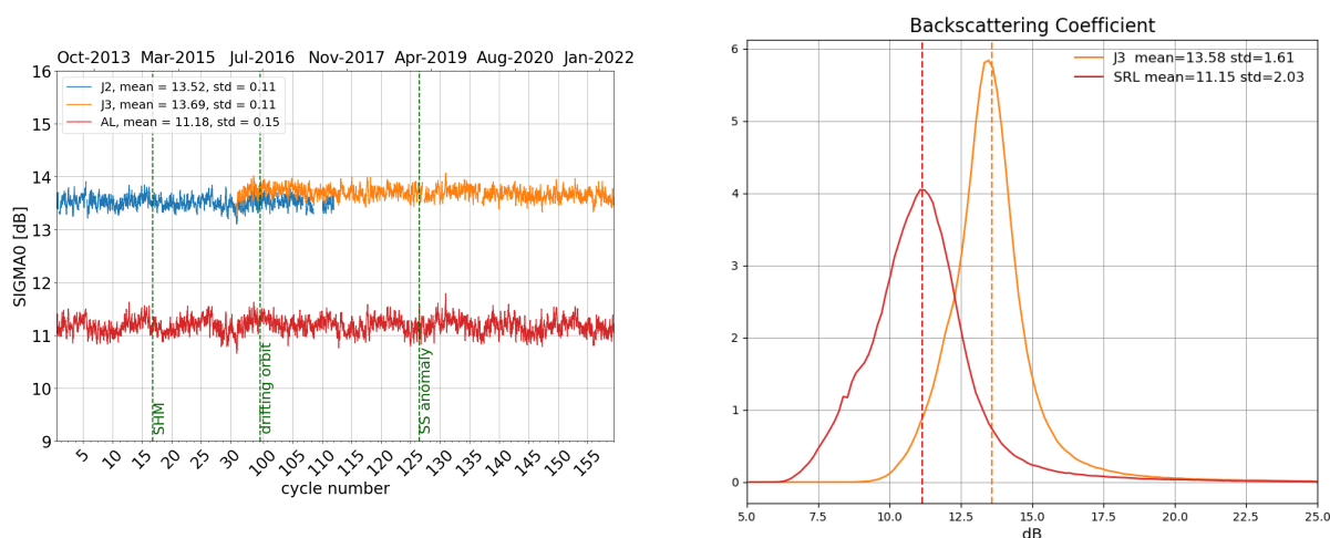
Figure 7: Daily monitoring of backscattering coefficient for Saral/AltiKa, Jason-2 and Jason-3 on the left and histogram for cycle 159 on the right (limited to 66° latitude).
