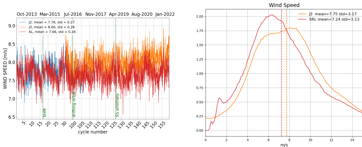
Figure 10: Daily monitoring of altimeter wind speed for Saral/AltiKa, Jason-2 and Jason-3 on the left and histogram for cycle 159 on the right (limited to 66° latitude).
