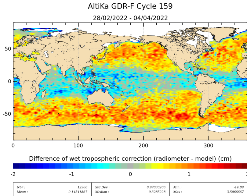
Figure 11: Mean of wet troposphere correction difference (Radiometer-ECMWF model) for cycle 159.
