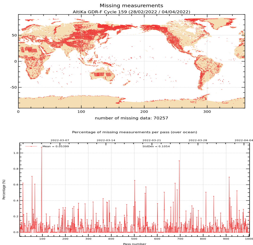
Figure 1: Map of missing measurements for cycle 159 on top. Monitoring of percentage of missing ocean measurements per pass on bottom.
