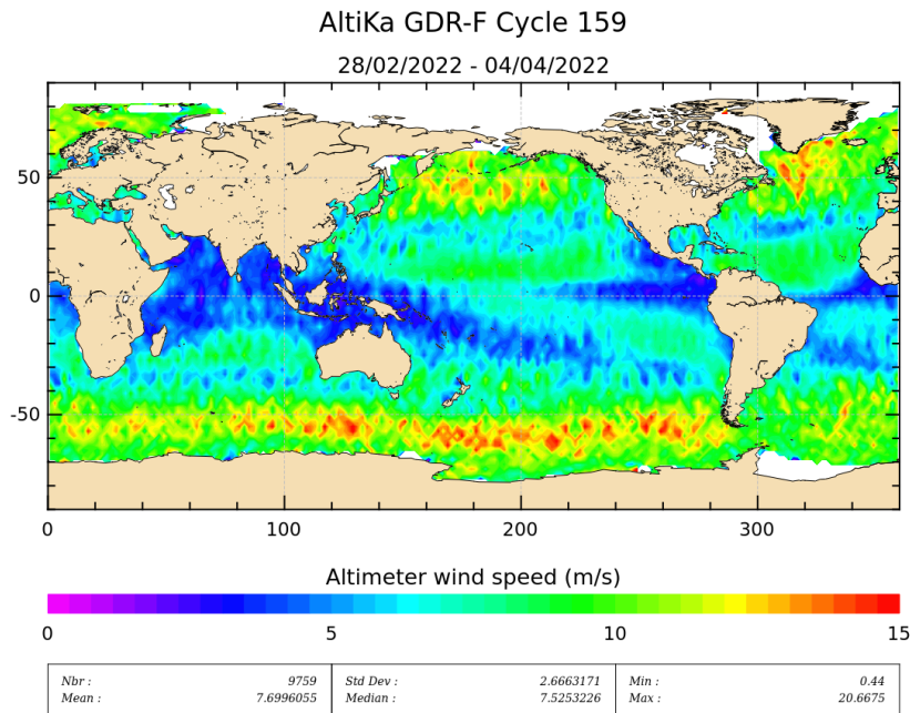
Figure 9: Altimeter wind speed for cycle 159.
