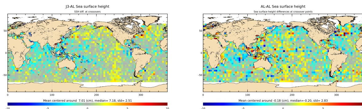
Figure 14: Mean of multi-mission SSH and mono-mission SSH differences at crossovers for cycle 159.
