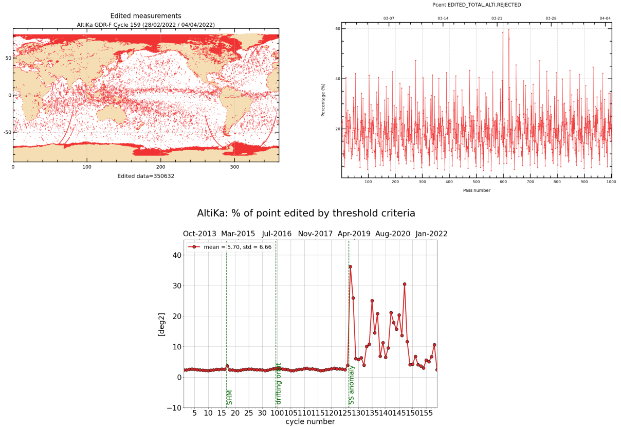
Figure 2: Rejected measurements on thresholds criteria : Cycle 159, map and monitoring of % of rejected measurements per track (top), whole time serie / % of rejected measurements per cycle (bottom).
