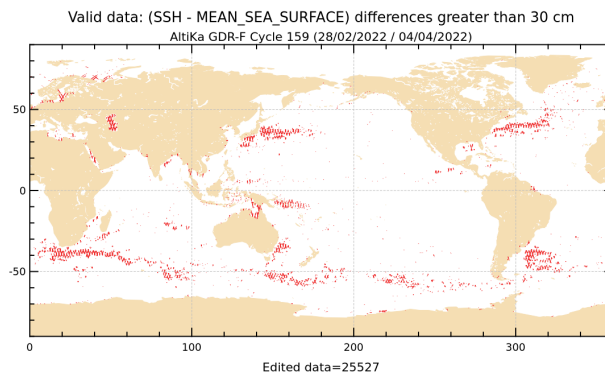
Figure 20: SLA higher than 30 cm for cycle 159.
