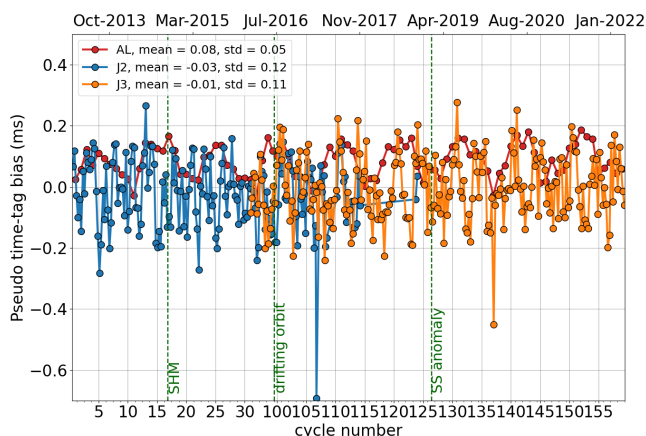
Figure 17: Cyclic monitoring of pseudo time tag bias for Saral/AltiKa.
