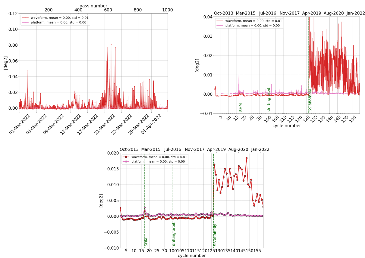
Figure 13: Monitoring per pass for cycle 159 (left), daily monitoring(right) and cyclic monitoring (bottom) of SARAL/AltiKa's mispointing angle: comparison between the one derived from waveform retracking and the one measured by platform startrackers.
