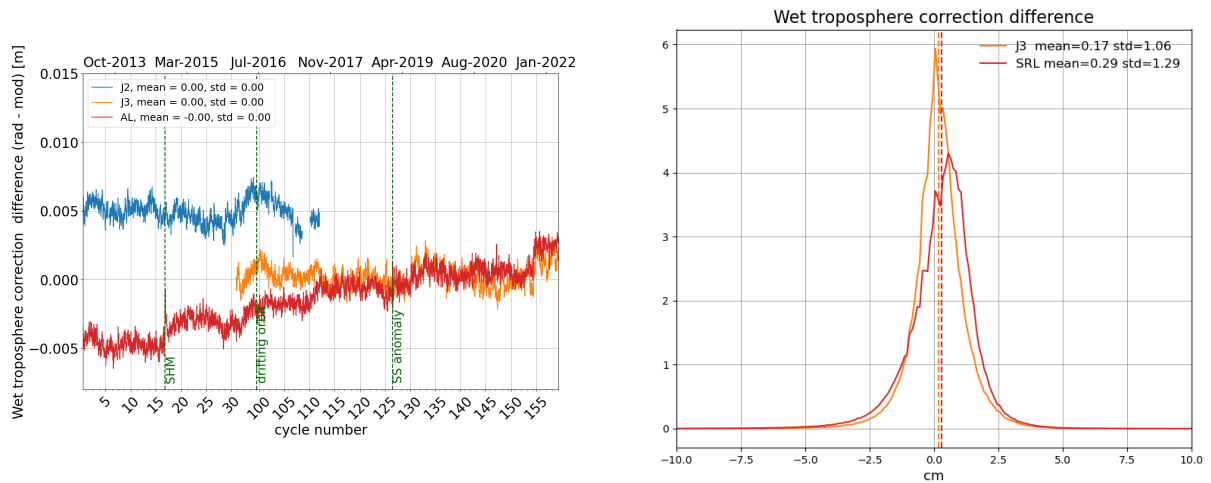
Figure 12: Daily monitoring of wet troposphere differences (Radiometer-ECMWF model) for Saral/AltiKa Jason-2 and Jason-3 (left) and histogram on the right (limited to 66° latitude) for cycle 159 .
