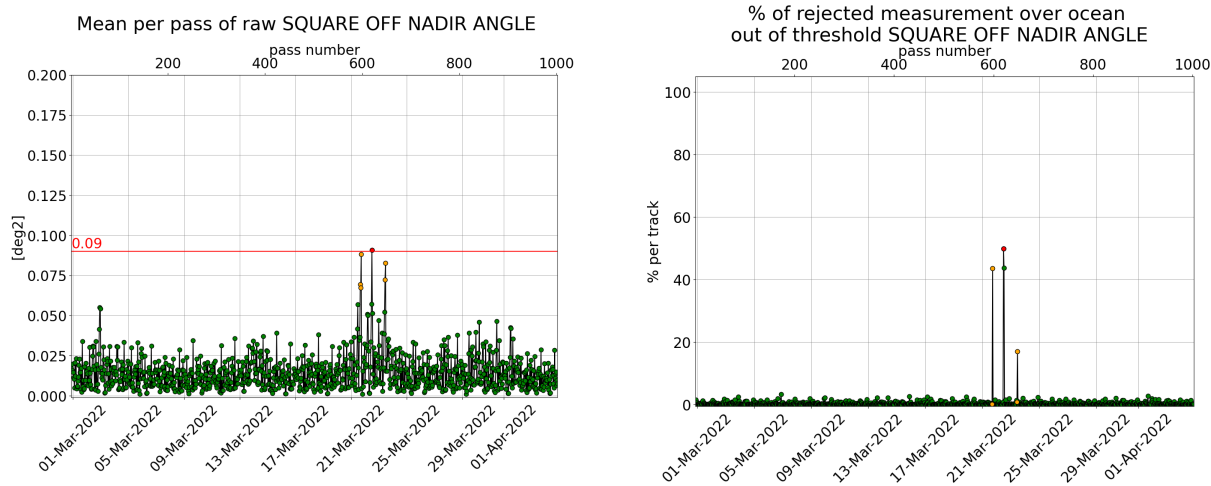
Figure 3: [left] Mispointing cycle 159, [right] Percentage of rejected measurement by threshold on square off-nadir angle.
