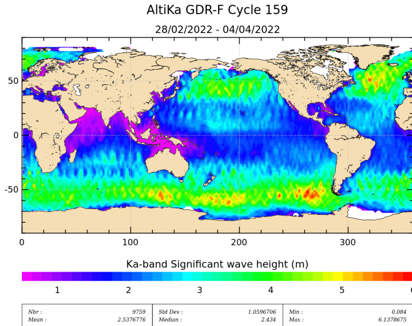
Figure 5: Significant wave height for cycle 159.
