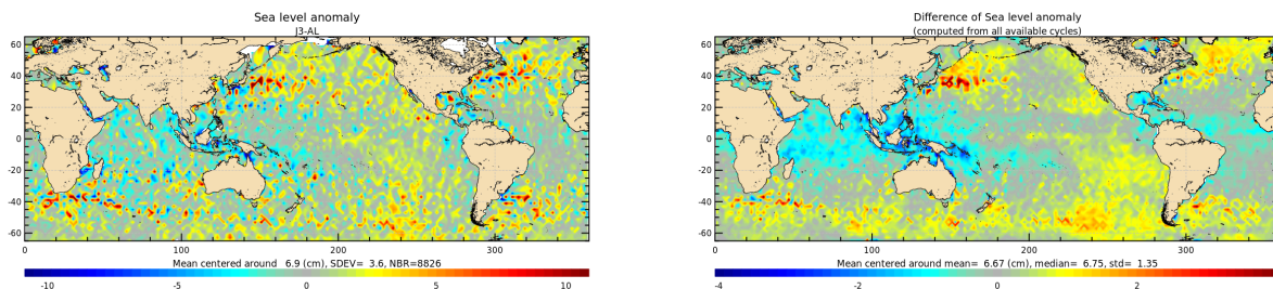
Figure 21: Jason-3 – Saral/AltiKa SLA differences for cycle 159 (left) and averaged over the whole Saral/AltiKa period (right).
