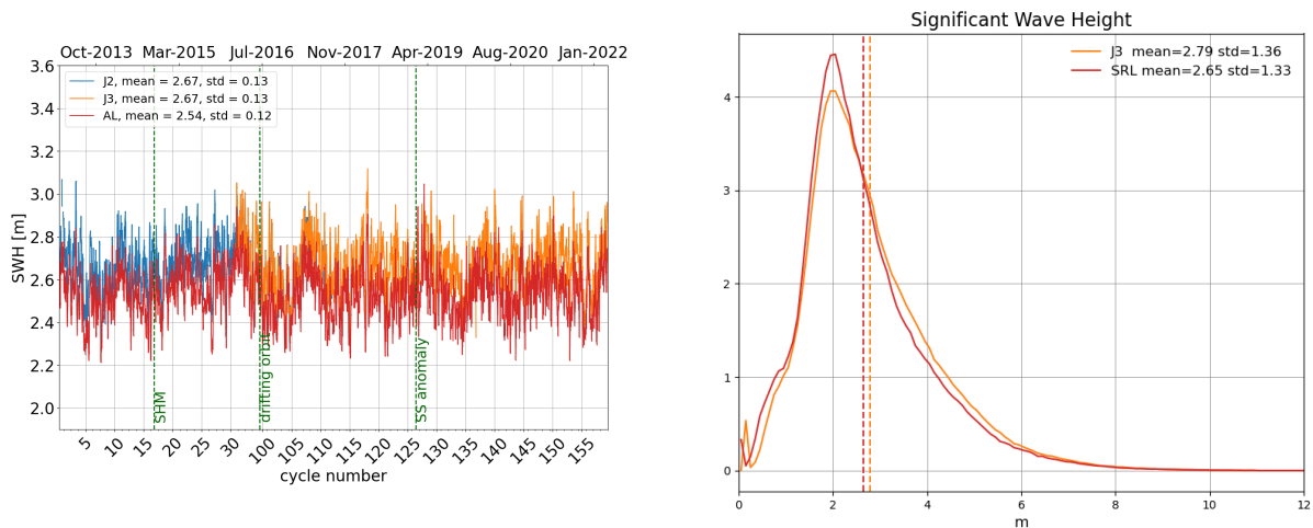
Figure 6: Daily monitoring of significant wave height for AltiKa (Ka-band) Jason-2 and Jason-3 (Ku-band) on the left and histogram for cycle 159 on the right (limited to 66^\circ latitude).
