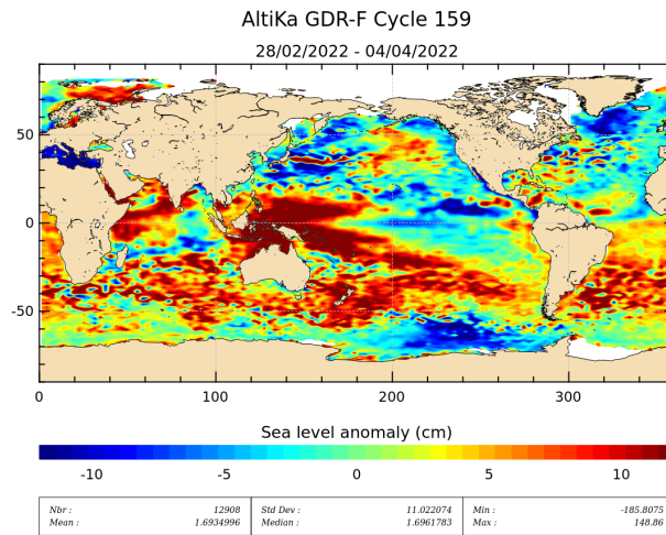
Figure 19: Sea level anomaly relative to MSS for cycle 159.
