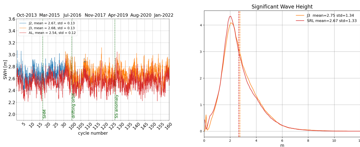
Figure 6: Daily monitoring of significant wave height for AltiKa (Ka-band) Jason-2 and Jason-3 (Ku-band) on the left and histogram for cycle 160 on the right (limited to 66° latitude).
