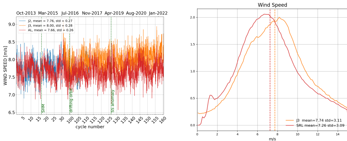
Figure 10: Daily monitoring of altimeter wind speed for Saral/AltiKa, Jason-2 and Jason-3 on the left and histogram for cycle 160 on the right (limited to 66° latitude).
