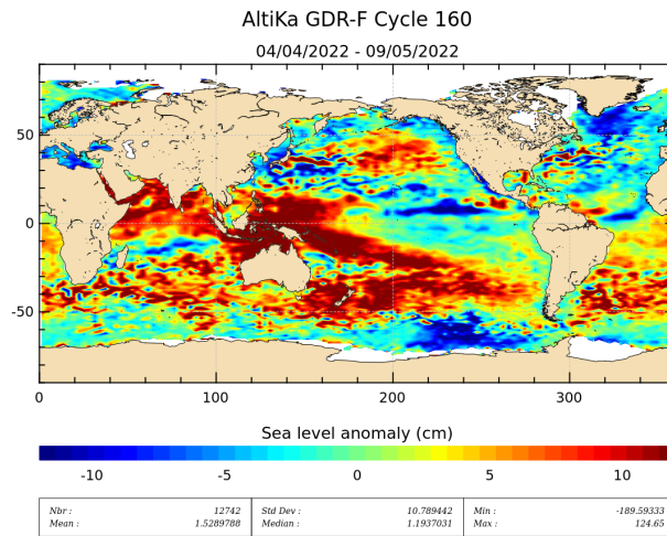
Figure 19: Sea level anomaly relative to MSS for cycle 160.
