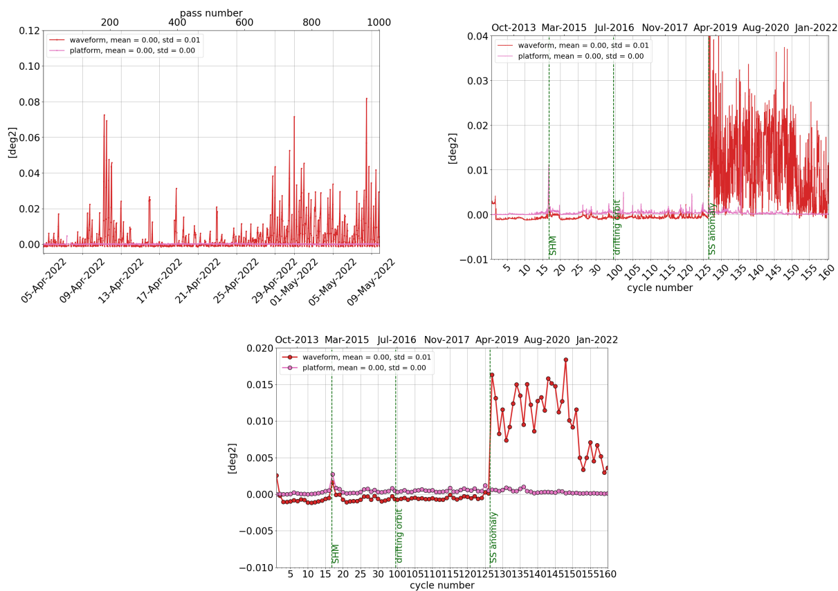
Figure 13: Monitoring per pass for cycle 160 (left), daily monitoring(right) and cyclic monitoring (bottom) of SARAL/AltiKa's mispointing angle: comparison between the one derived from waveform retracking and the one measured by platform startrackers.
