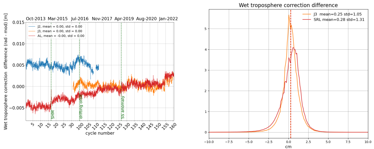
Figure 12: Daily monitoring of wet troposphere differences (Radiometer-ECMWF model) for Saral/AltiKa Jason-2 and Jason-3 (left) and histogram on the right (limited to 66° latitude) for cycle 160 .
