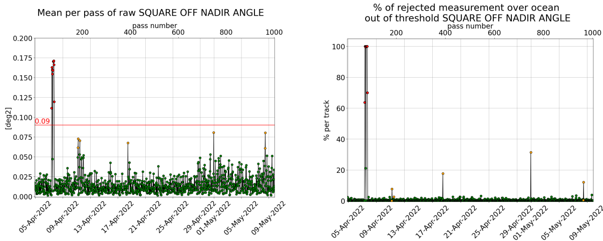
Figure 3: [left] Mispointing cycle 160, [right] Percentage of rejected measurement by threshold on square off-nadir angle.
