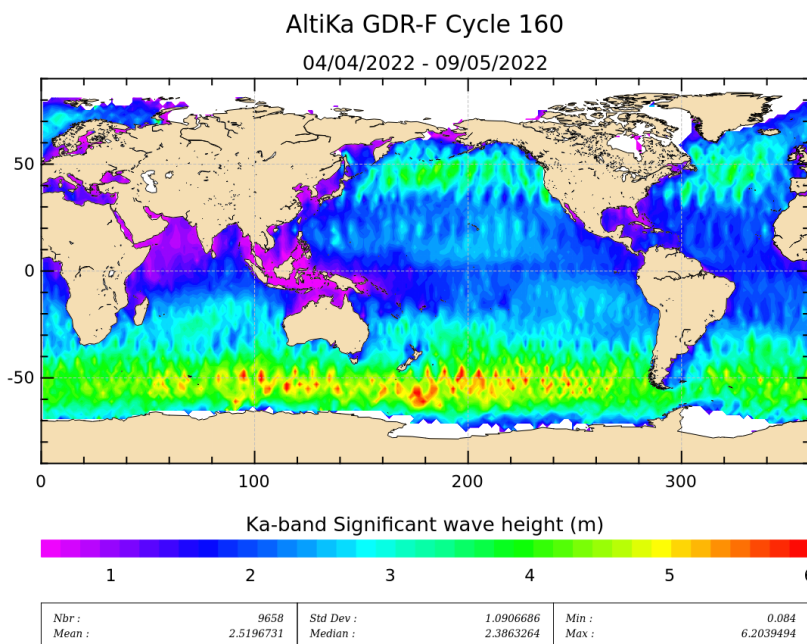
Figure 5: Significant wave height for cycle 160.
