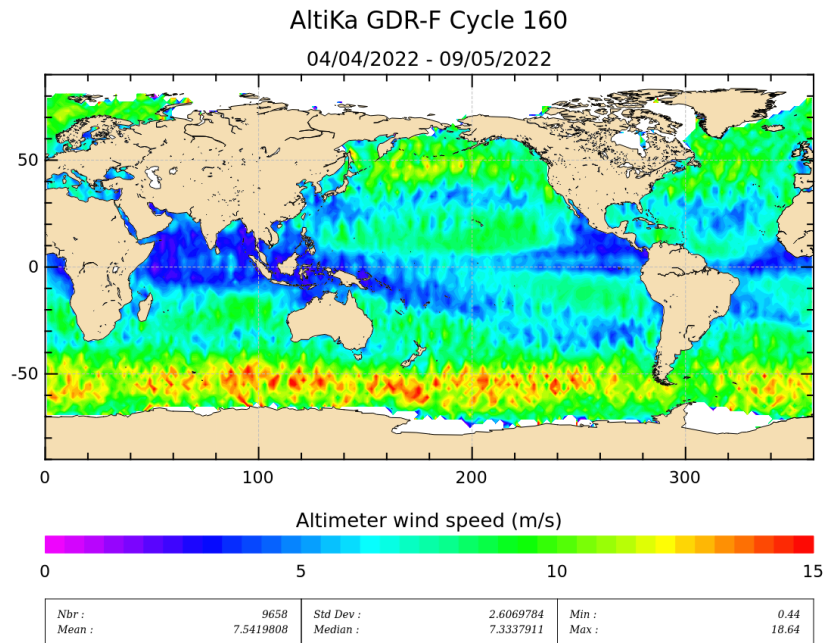
Figure 9: Altimeter wind speed for cycle 160.
