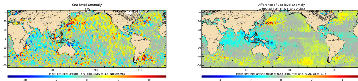
Figure 21: Jason-3 – Saral/AltiKa SLA differences for cycle 160 (left) and averaged over the whole Saral/AltiKa period (right).
