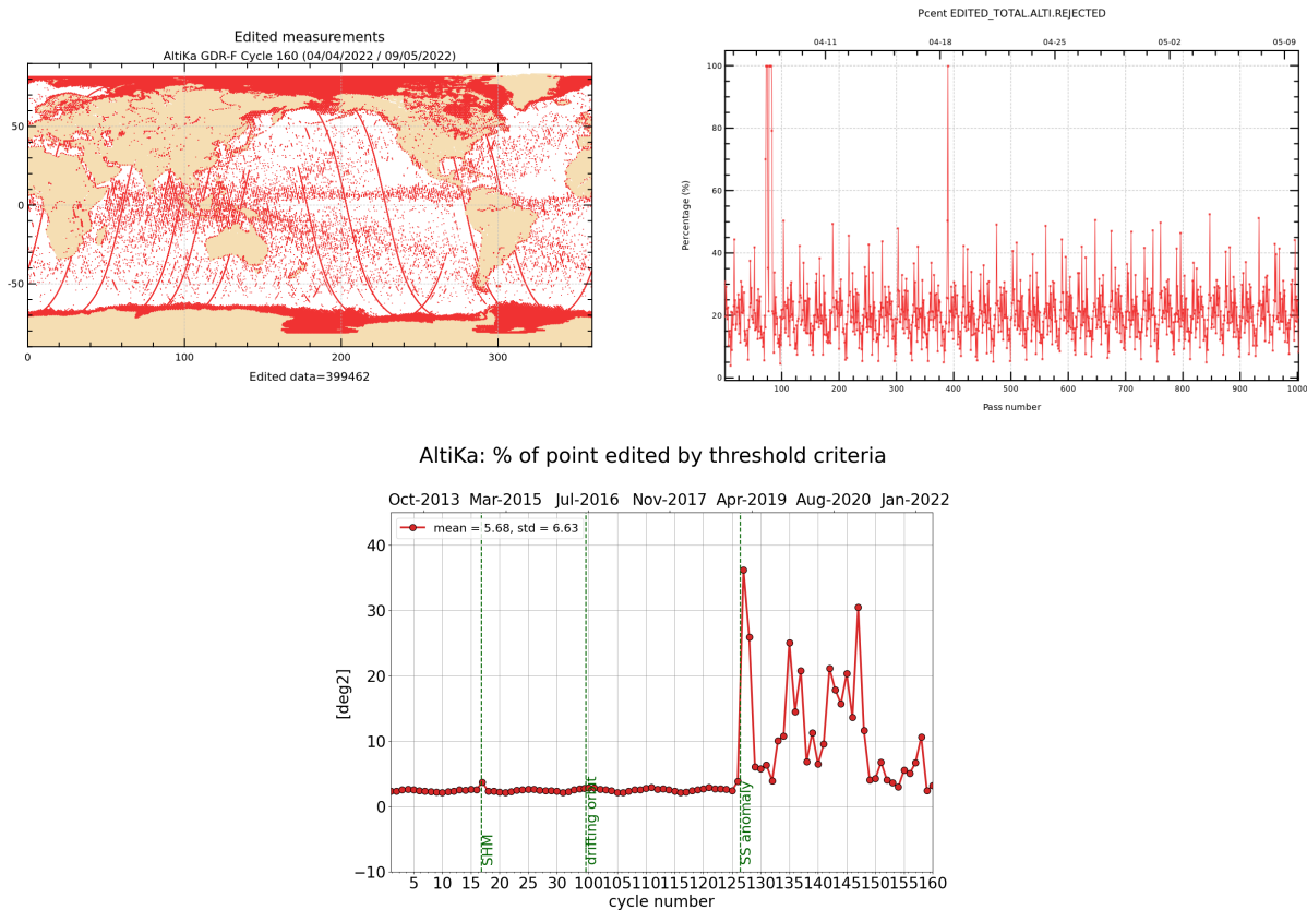
Figure 2: Rejected measurements on thresholds criteria : Cycle 160, map and monitoring of % of rejected measurements per track (top), whole time serie / % of rejected measurements per cycle (bottom).
