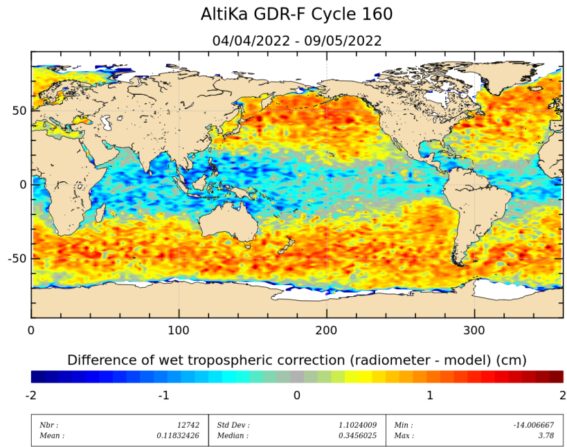
Figure 11: Mean of wet troposphere correction difference (Radiometer-ECMWF model) for cycle 160.
