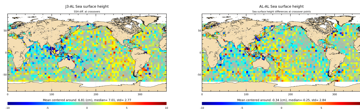
Figure 14: Mean of multi-mission SSH and mono-mission SSH differences at crossovers for cycle 160.
