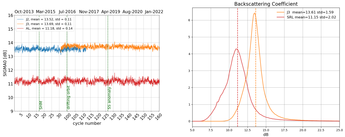
Figure 7: Daily monitoring of backscattering coefficient for Saral/AltiKa, Jason-2 and Jason-3 on the left and histogram for cycle 160 on the right (limited to 66° latitude).
