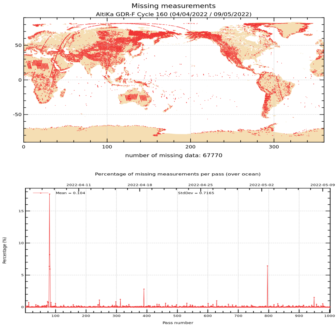
Figure 1: Map of missing measurements for cycle 160 on top. Monitoring of percentage of missing ocean measurements per pass on bottom.
