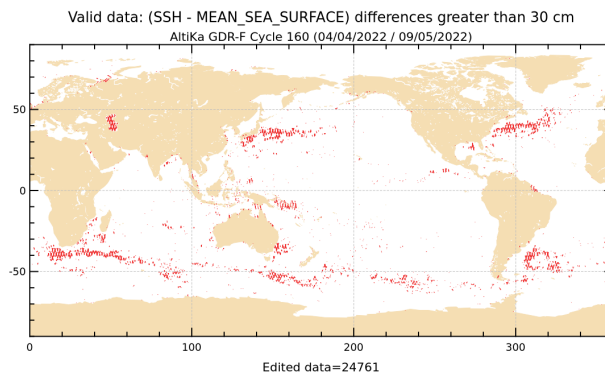
Figure 20: SLA higher than 30 cm for cycle 160.
