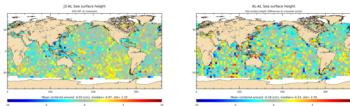
Figure 14: Mean of multi-mission SSH and mono-mission SSH differences at crossovers for cycle 164.
