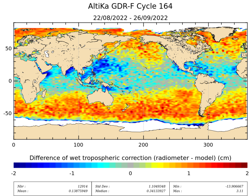
Figure 11: Mean of wet troposphere correction difference (Radiometer-ECMWF model) for cycle 164.
