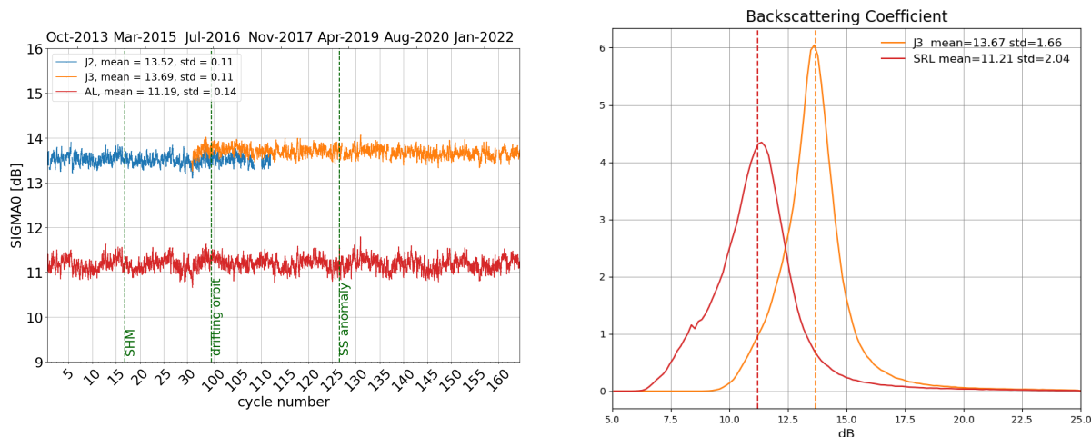
Figure 7: Daily monitoring of backscattering coefficient for Saral/AltiKa, Jason-2 and Jason-3 on the left and histogram for cycle 164 on the right (limited to 66° latitude).
