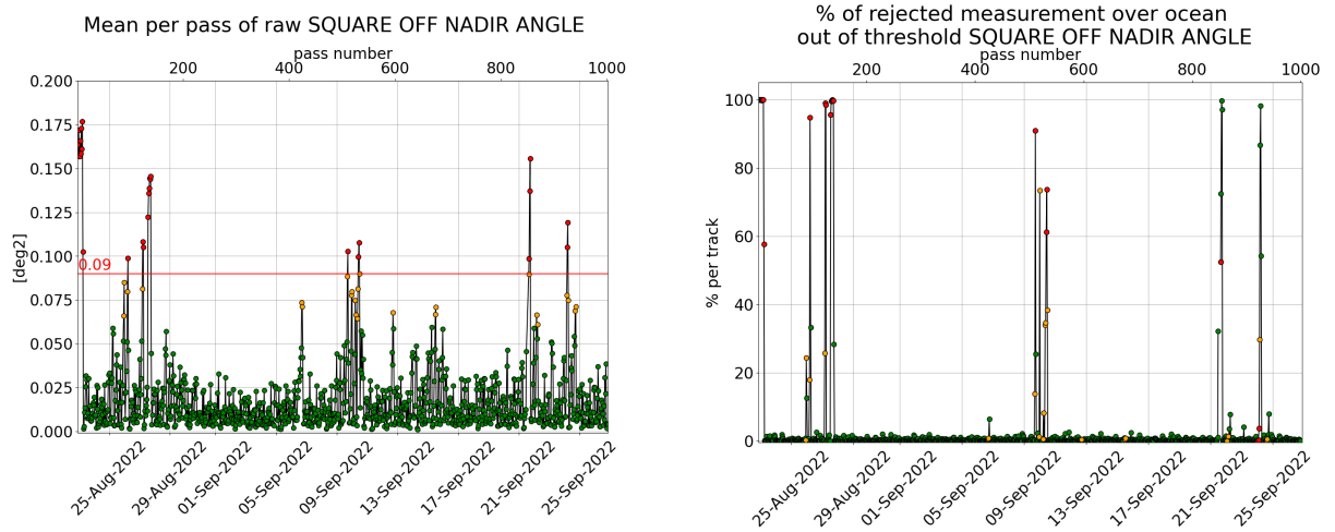
Figure 3: [left] Mispointing cycle 164, [right] Percentage of rejected measurement by threshold on square off-nadir angle.
