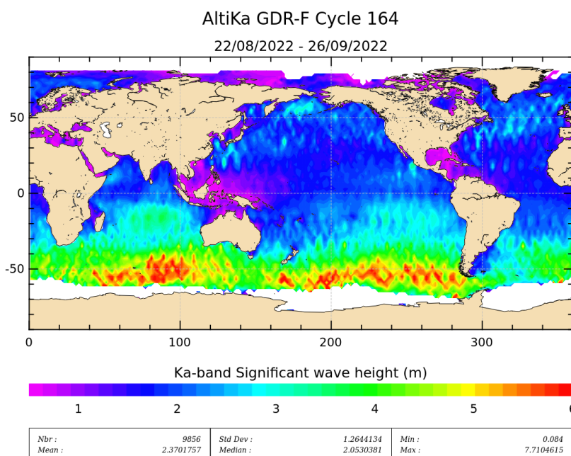
Figure 5: Significant wave height for cycle 164.
