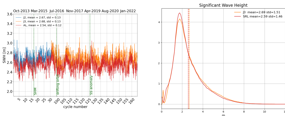
Figure 6: Daily monitoring of significant wave height for AltiKa (Ka-band) Jason-2 and Jason-3 (Ku-band) on the left and histogram for cycle 164 on the right (limited to 66^\circ latitude).
