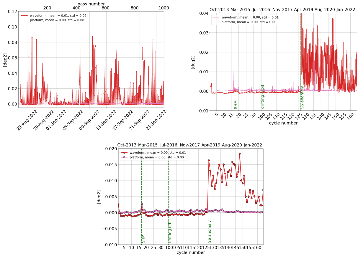
Figure 13: Monitoring per pass for cycle 164 (left), daily monitoring(right) and cyclic monitoring (bottom) of SARAL/AltiKa's mispointing angle: comparison between the one derived from waveform retracking and the one measured by platform startrackers.
