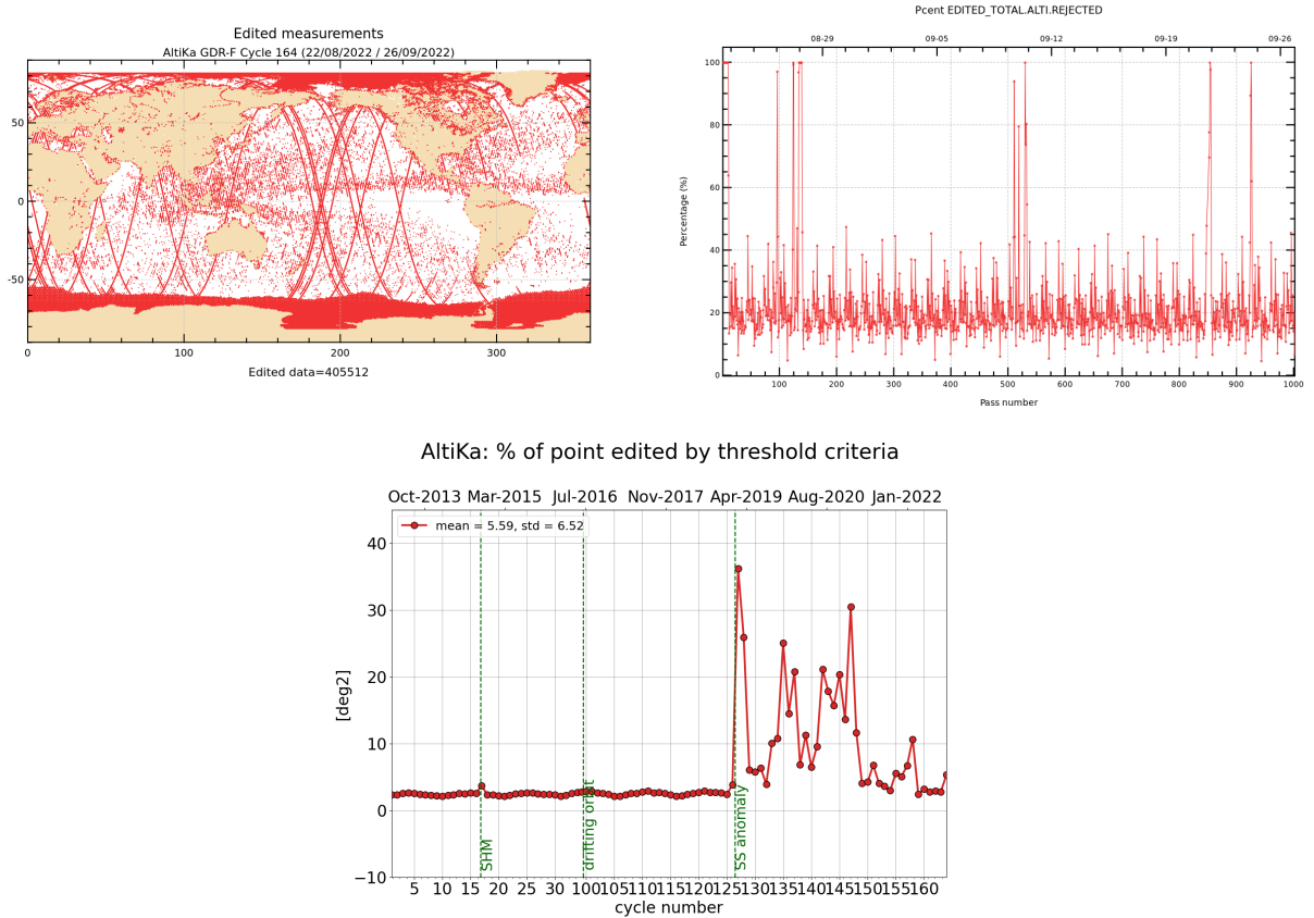
Figure 2: Rejected measurements on thresholds criteria : Cycle 164, map and monitoring of % of rejected measurements per track (top), whole time serie / % of rejected measurements per cycle (bottom).
