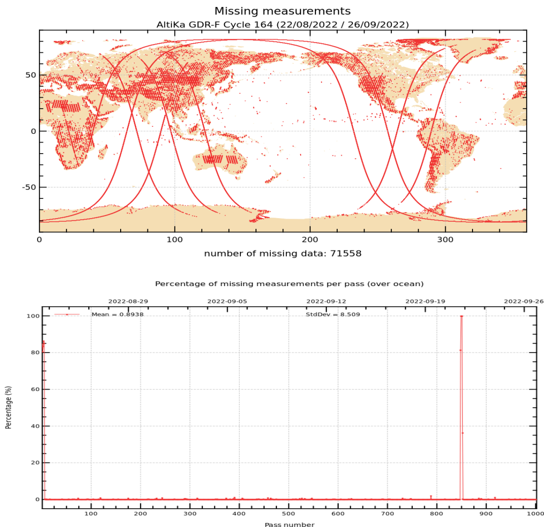
Figure 1: Map of missing measurements for cycle 164 on top. Monitoring of percentage of missing ocean measurements per pass on bottom.
