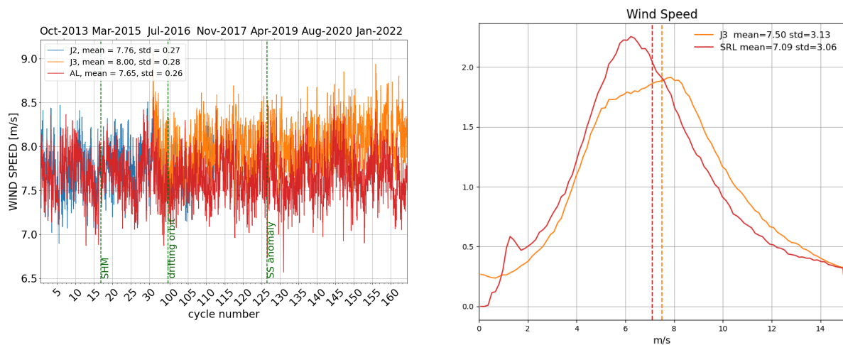
Figure 10: Daily monitoring of altimeter wind speed for Saral/AltiKa, Jason-2 and Jason-3 on the left and histogram for cycle 164 on the right (limited to 66° latitude).
