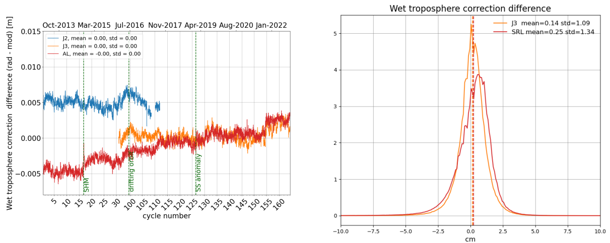
Figure 12: Daily monitoring of wet troposphere differences (Radiometer-ECMWF model) for Saral/AltiKa Jason-2 and Jason-3 (left) and histogram on the right (limited to 66° latitude) for cycle 164 .
