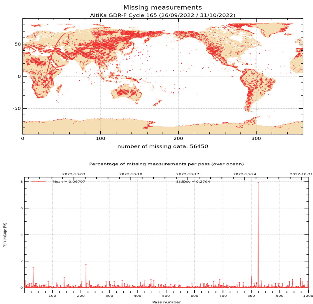
Figure 1: Map of missing measurements for cycle 165 on top. Monitoring of percentage of missing ocean measurements per pass on bottom.
