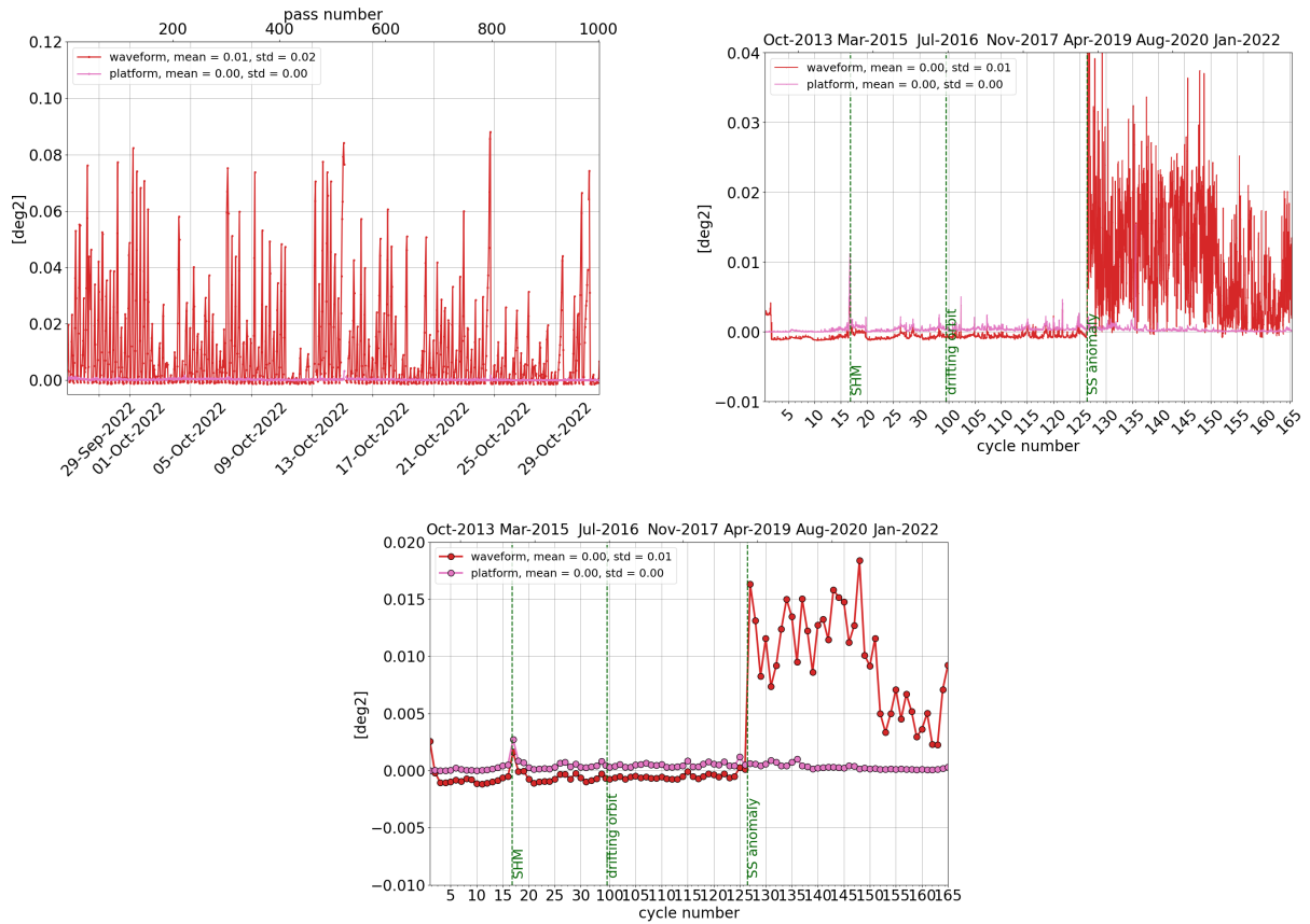
Figure 13: Monitoring per pass for cycle 165 (left), daily monitoring(right) and cyclic monitoring (bottom) of SARAL/AltiKa's mispointing angle: comparison between the one derived from waveform retracking and the one measured by platform startrackers.
