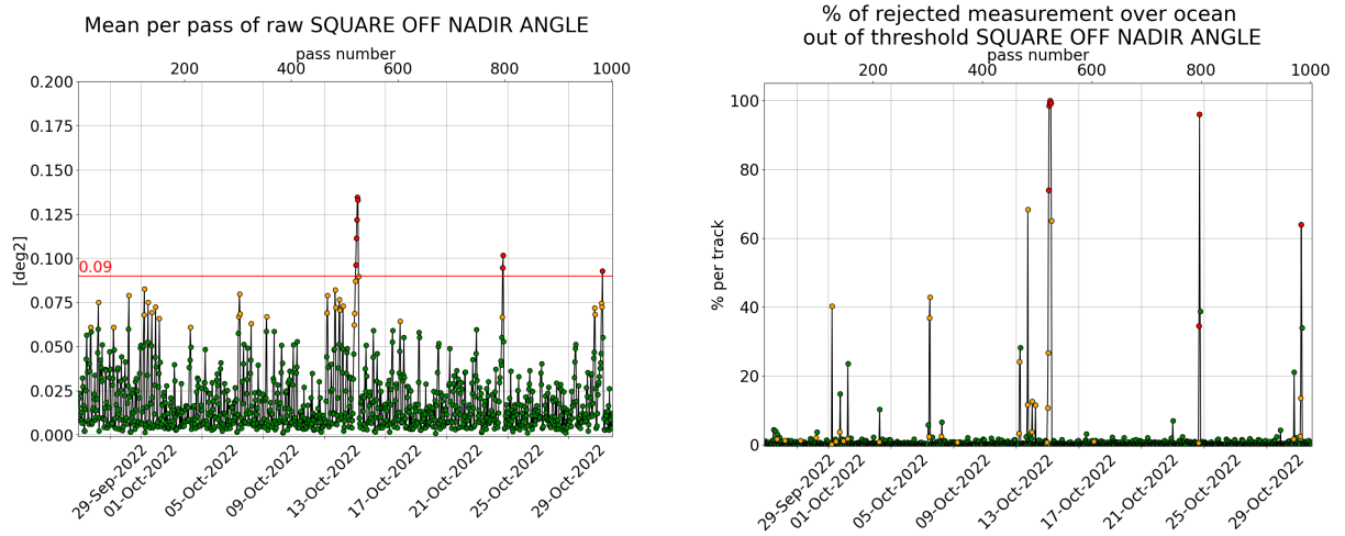
Figure 3: [left] Mispointing cycle 165, [right] Percentage of rejected measurement by threshold on square off-nadir angle.
