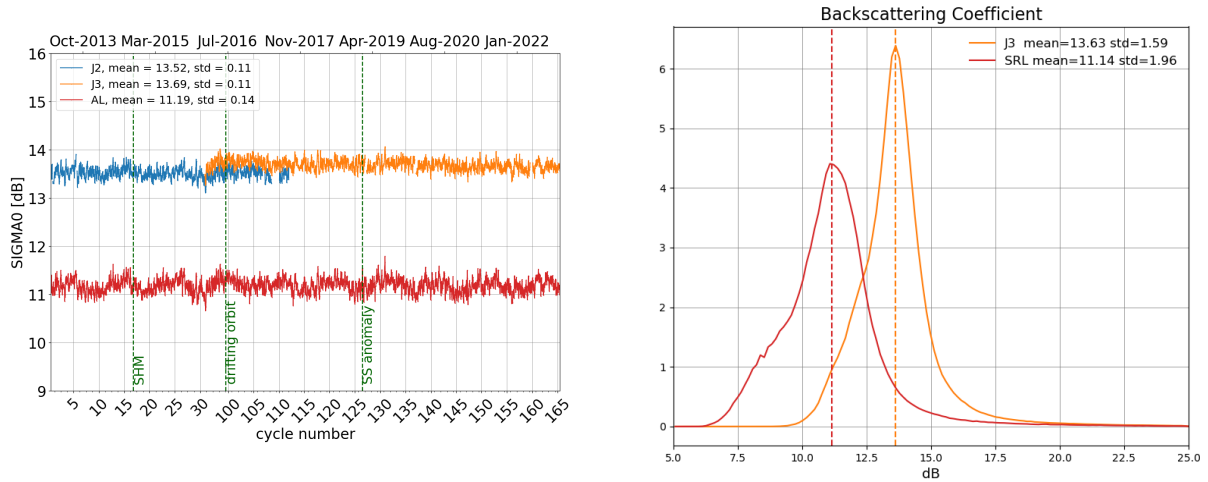
Figure 7: Daily monitoring of backscattering coefficient for Saral/AltiKa, Jason-2 and Jason-3 on the left and histogram for cycle 165 on the right (limited to 66° latitude).
