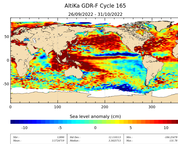
Figure 19: Sea level anomaly relative to MSS for cycle 165.
