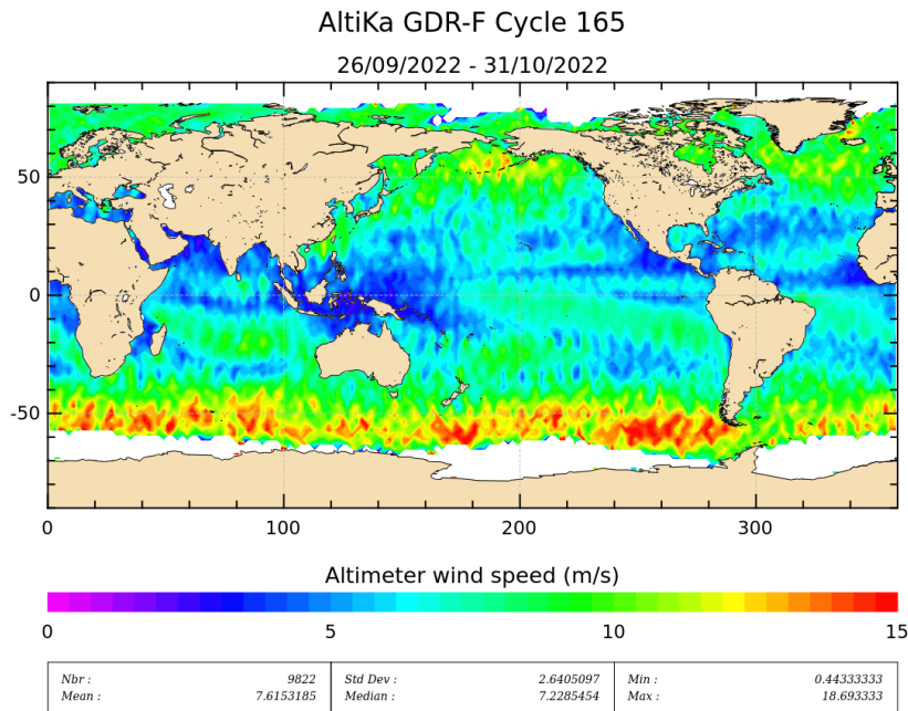
Figure 9: Altimeter wind speed for cycle 165.
