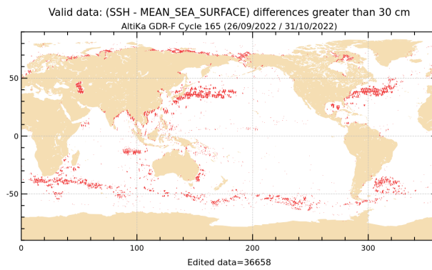
Figure 20: SLA higher than 30 cm for cycle 165.
