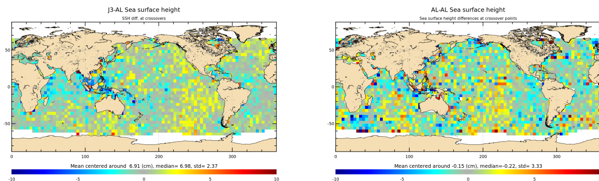
Figure 14: Mean of multi-mission SSH and mono-mission SSH differences at crossovers for cycle 165.
