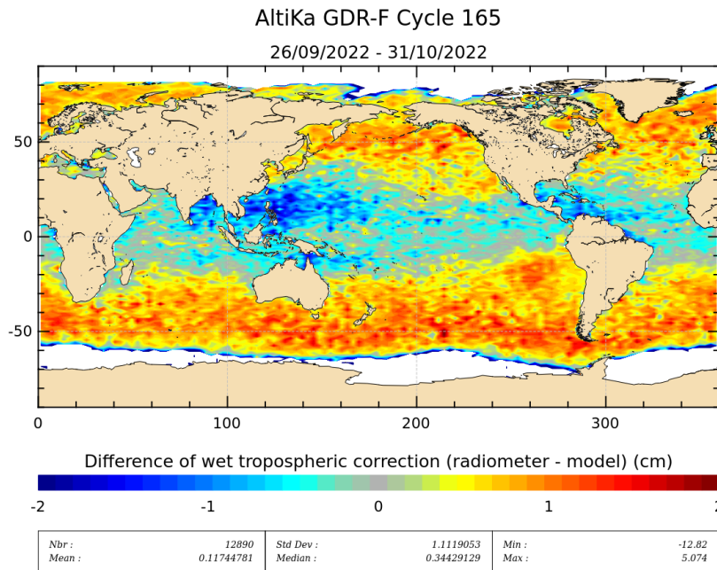
Figure 11: Mean of wet troposphere correction difference (Radiometer-ECMWF model) for cycle 165.
