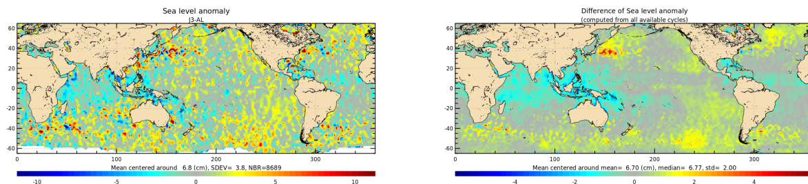
Figure 21: Jason-3 – Saral/AltiKa SLA differences for cycle 165 (left) and averaged over the whole Saral/AltiKa period (right).
