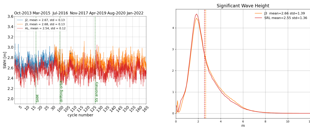
Figure 6: Daily monitoring of significant wave height for AltiKa (Ka-band) Jason-2 and Jason-3 (Ku-band) on the left and histogram for cycle 165 on the right (limited to 66^\circ latitude).
