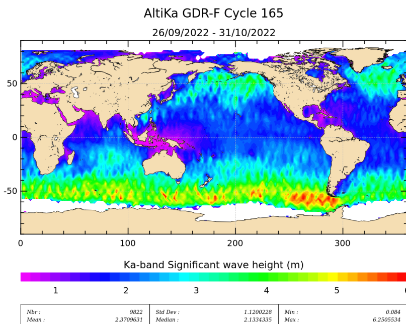
Figure 5: Significant wave height for cycle 165.
