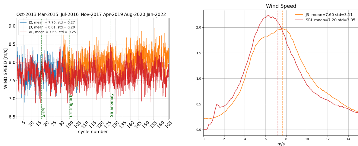
Figure 10: Daily monitoring of altimeter wind speed for Saral/AltiKa, Jason-2 and Jason-3 on the left and histogram for cycle 165 on the right (limited to 66° latitude).
