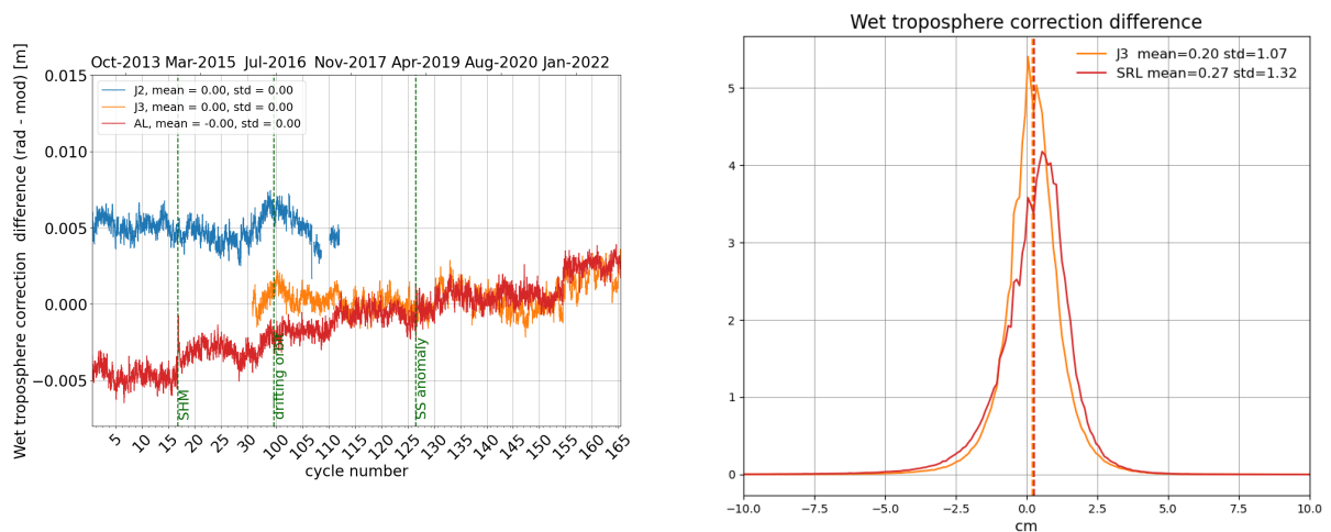
Figure 12: Daily monitoring of wet troposphere differences (Radiometer-ECMWF model) for Saral/AltiKa Jason-2 and Jason-3 (left) and histogram on the right (limited to 66° latitude) for cycle 165 .
