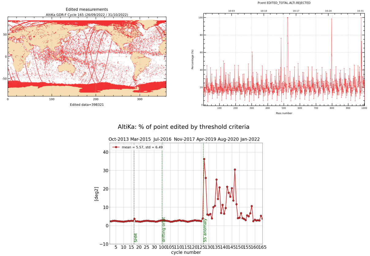
Figure 2: Rejected measurements on thresholds criteria : Cycle 165, map and monitoring of % of rejected measurements per track (top), whole time serie / % of rejected measurements per cycle (bottom).
