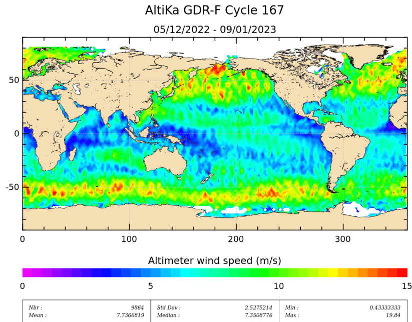
Figure 9: Altimeter wind speed for cycle 167.
