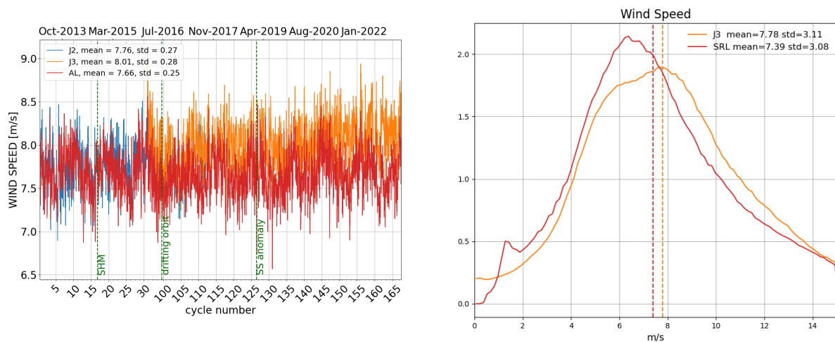
Figure 10: Daily monitoring of altimeter wind speed for Saral/AltiKa, Jason-2 and Jason-3 on the left and histogram for cycle 167 on the right (limited to 66° latitude).
