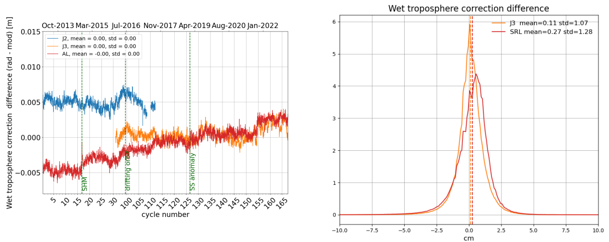
Figure 12: Daily monitoring of wet troposphere differences (Radiometer-ECMWF model) for Saral/AltiKa Jason-2 and Jason-3 (left) and histogram on the right (limited to 66° latitude) for cycle 167 .
