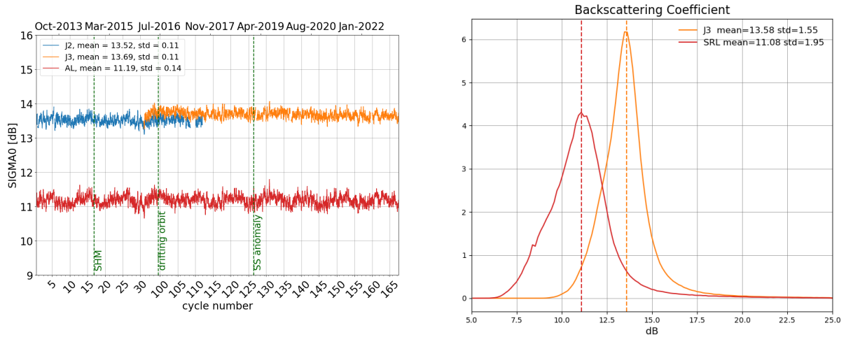
Figure 7: Daily monitoring of backscattering coefficient for Saral/AltiKa, Jason-2 and Jason-3 on the left and histogram for cycle 167 on the right (limited to 66° latitude).
