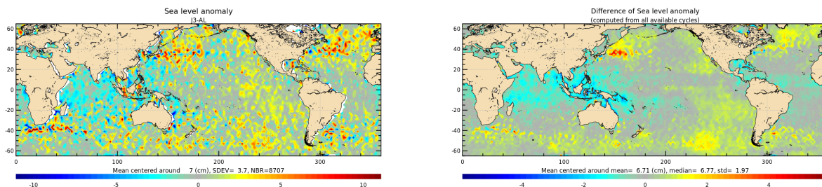
Figure 21: Jason-3 – Saral/AltiKa SLA differences for cycle 167 (left) and averaged over the whole Saral/AltiKa period (right).
