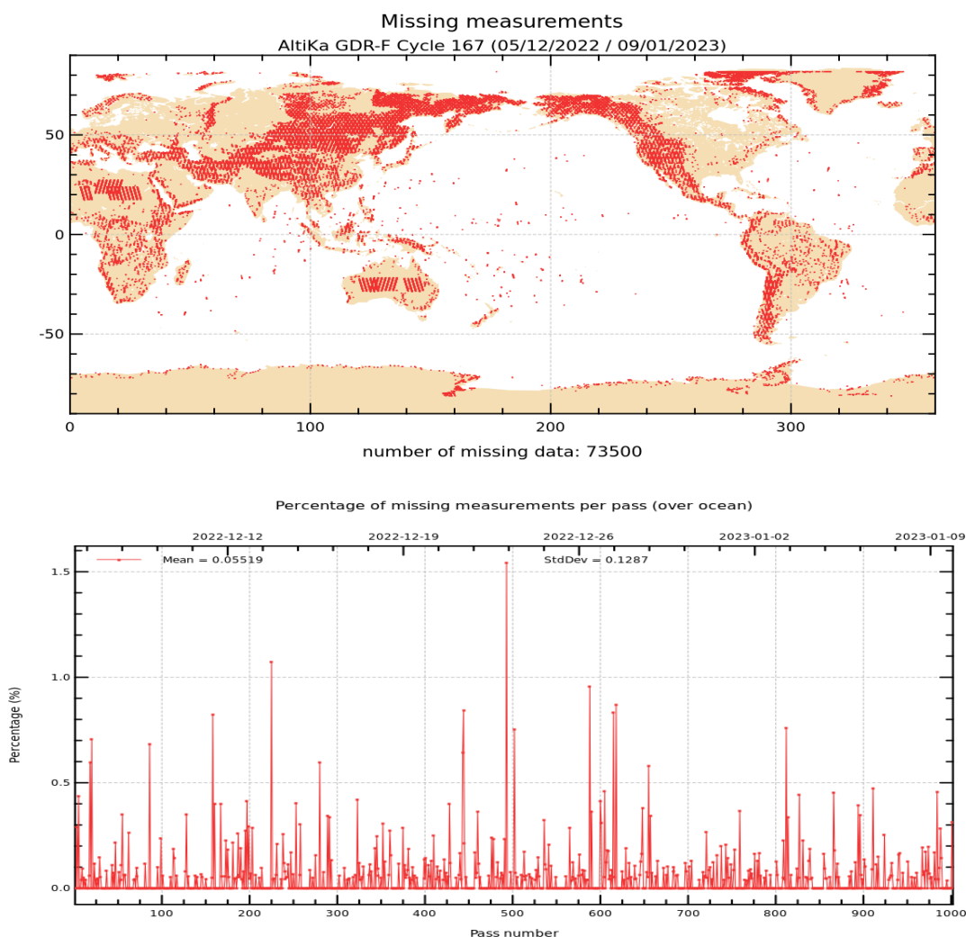
Figure 1: Map of missing measurements for cycle 167 on top. Monitoring of percentage of missing ocean measurements per pass on bottom.
