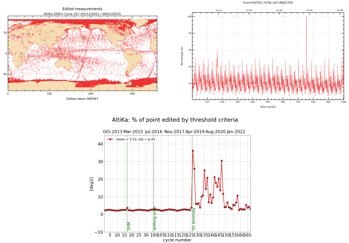
Figure 2: Rejected measurements on thresholds criteria : Cycle 167, map and monitoring of % of rejected measurements per track (top), whole time serie / % of rejected measurements per cycle (bottom).
