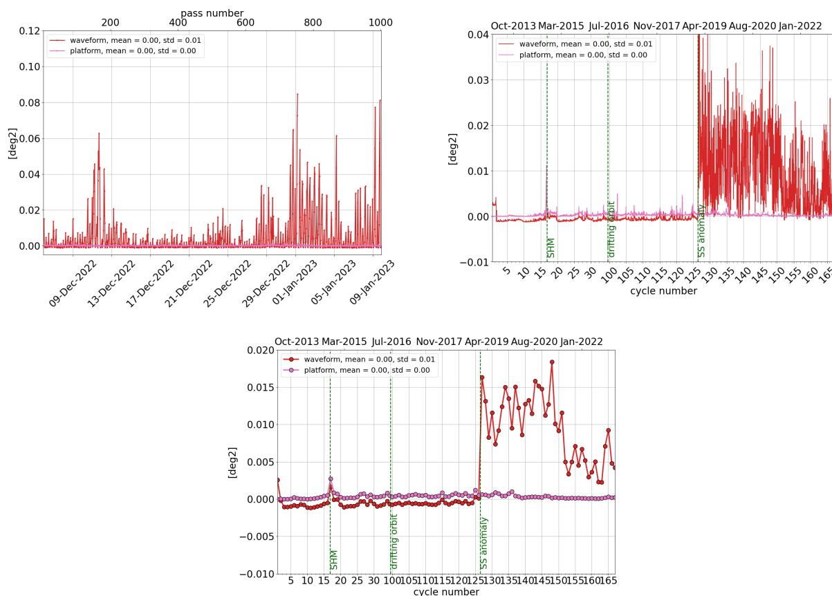
Figure 13: Monitoring per pass for cycle 167 (left), daily monitoring(right) and cyclic monitoring (bottom) of SARAL/AltiKa's mispointing angle: comparison between the one derived from waveform retracking and the one measured by platform startrackers.
