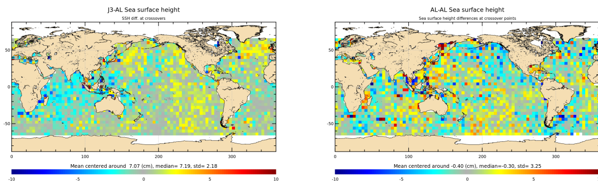
Figure 14: Mean of multi-mission SSH and mono-mission SSH differences at crossovers for cycle 167.
