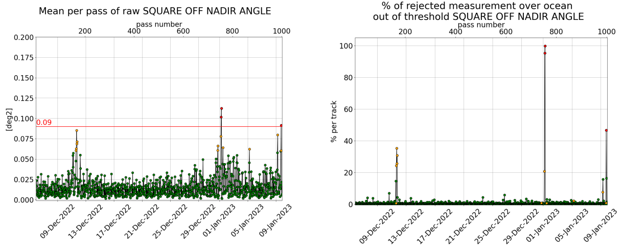
Figure 3: [left] Mispointing cycle 167, [right] Percentage of rejected measurement by threshold on square off-nadir angle.
