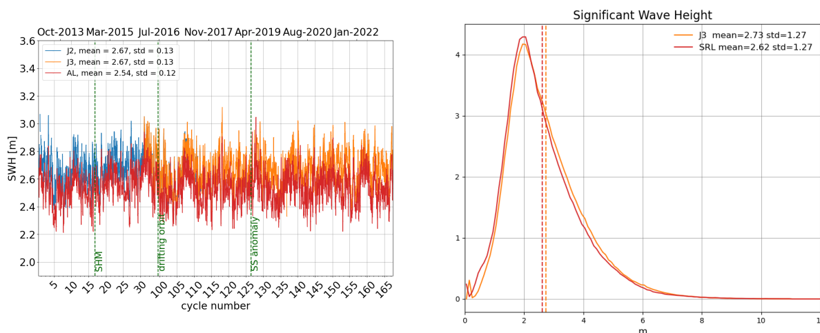
Figure 6: Daily monitoring of significant wave height for AltiKa (Ka-band) Jason-2 and Jason-3 (Ku-band) on the left and histogram for cycle 167 on the right (limited to 66^\circ latitude).
