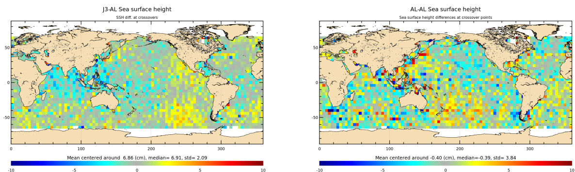
Figure 14: Mean of multi-mission SSH and mono-mission SSH differences at crossovers for cycle 172.
