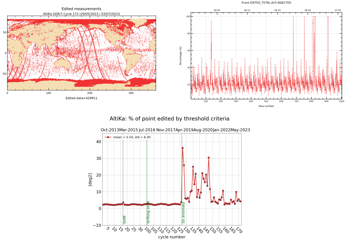
Figure 2: Rejected measurements on thresholds criteria : Cycle 172, map and monitoring of % of rejected measurements per track (top), whole time serie / % of rejected measurements per cycle (bottom).
