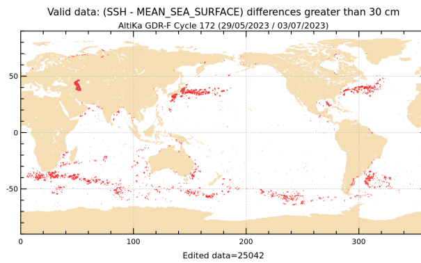
Figure 20: SLA higher than 30 cm for cycle 172.
