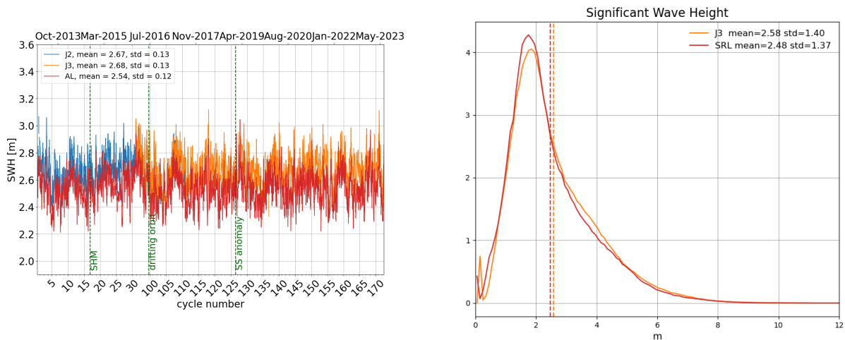
Figure 6: Daily monitoring of significant wave height for AltiKa (Ka-band) Jason-2 and Jason-3 (Ku-band) on the left and histogram for cycle 172 on the right (limited to 66° latitude).
