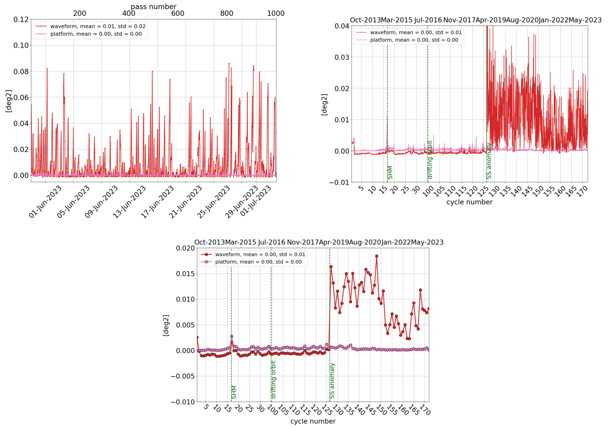
Figure 13: Monitoring per pass for cycle 172 (left), daily monitoring(right) and cyclic monitoring (bottom) of SARAL/AltiKa's mispointing angle: comparison between the one derived from waveform retracking and the one measured by platform startrackers.
