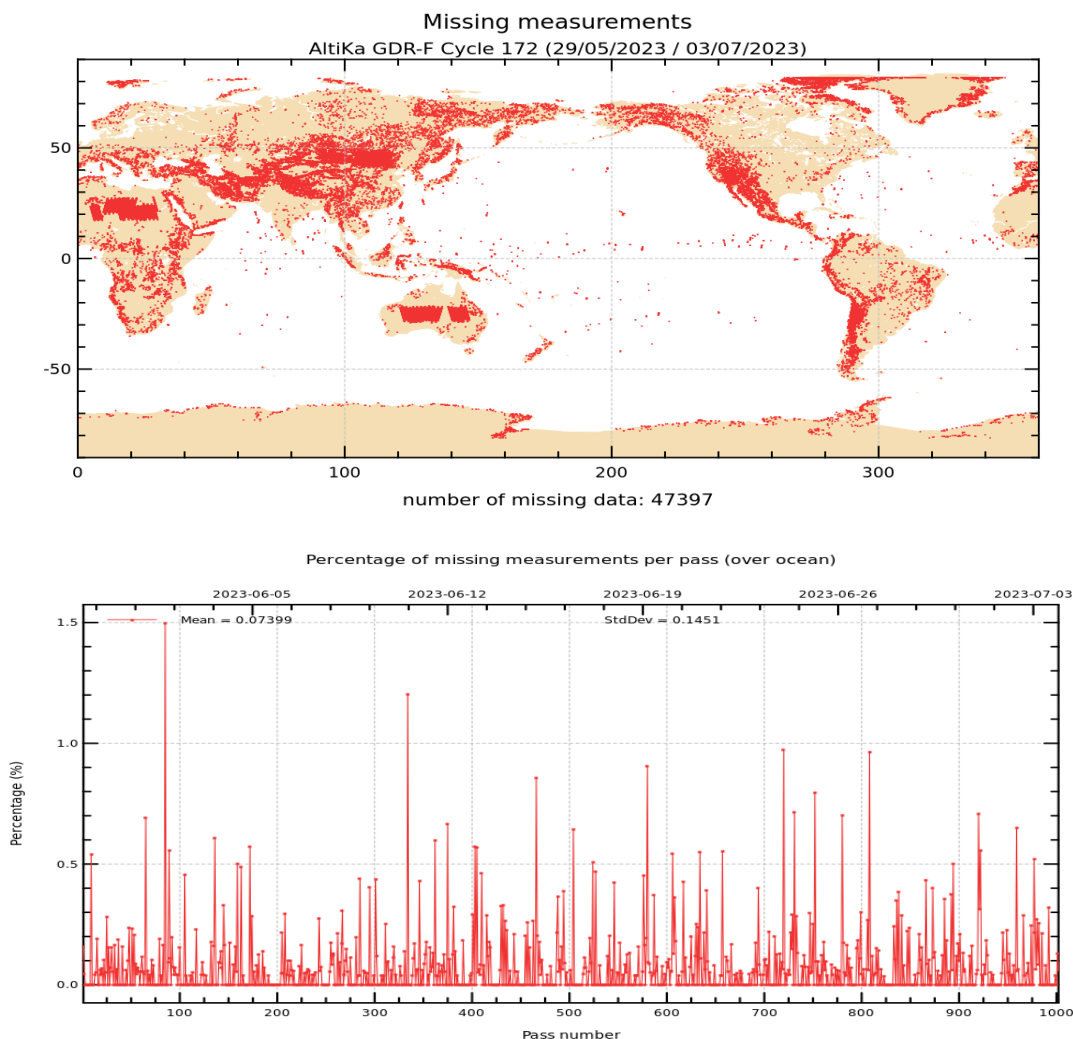
Figure 1: Map of missing measurements for cycle 172 on top. Monitoring of percentage of missing ocean measurements per pass on bottom.
