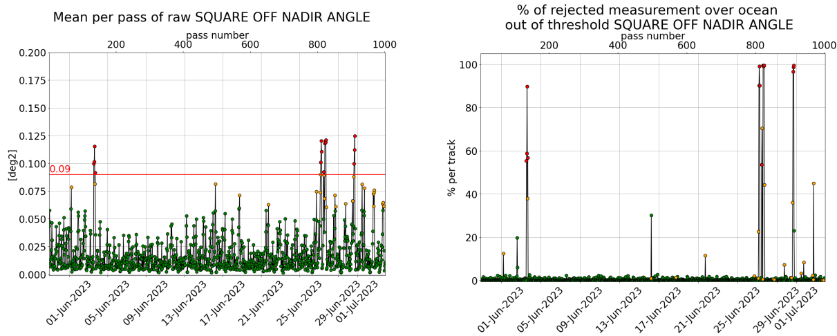
Figure 3: [left] Mispointing cycle 172, [right] Percentage of rejected measurement by threshold on square off-nadir angle.
