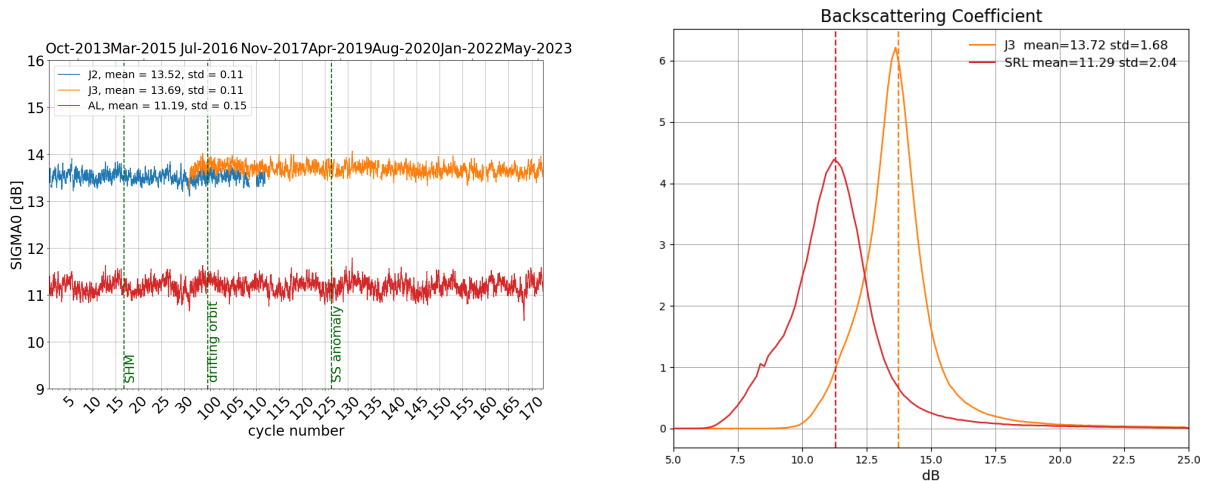
Figure 7: Daily monitoring of backscattering coefficient for Saral/AltiKa, Jason-2 and Jason-3 on the left and histogram for cycle 172 on the right (limited to 66° latitude).
