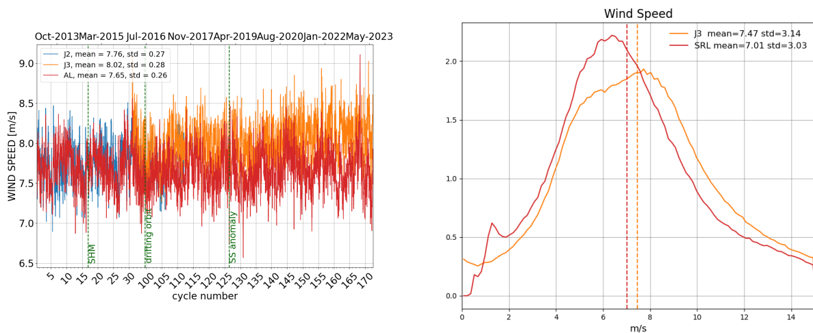
Figure 10: Daily monitoring of altimeter wind speed for Saral/AltiKa, Jason-2 and Jason-3 on the left and histogram for cycle 172 on the right (limited to 66° latitude).
