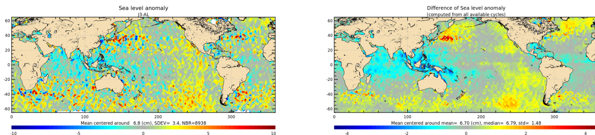
Figure 21: Jason-3 – Saral/AltiKa SLA differences for cycle 172 (left) and averaged over the whole Saral/AltiKa period (right).
