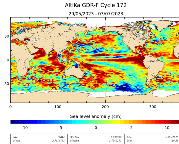
Figure 19: Sea level anomaly relative to MSS for cycle 172.
