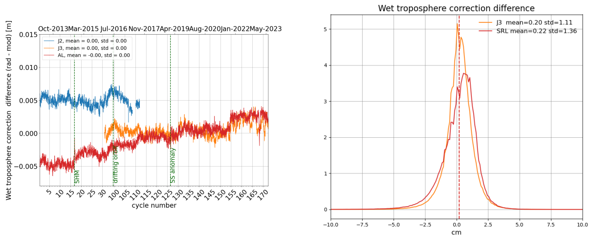
Figure 12: Daily monitoring of wet troposphere differences (Radiometer-ECMWF model) for Saral/AltiKa Jason-2 and Jason-3 (left) and histogram on the right (limited to 66° latitude) for cycle 172 .
