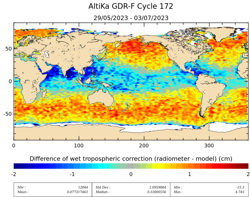
Figure 11: Mean of wet troposphere correction difference (Radiometer-ECMWF model) for cycle 172.
