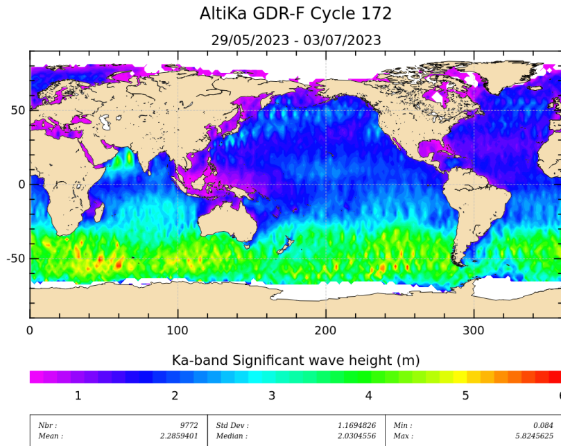
Figure 5: Significant wave height for cycle 172.
