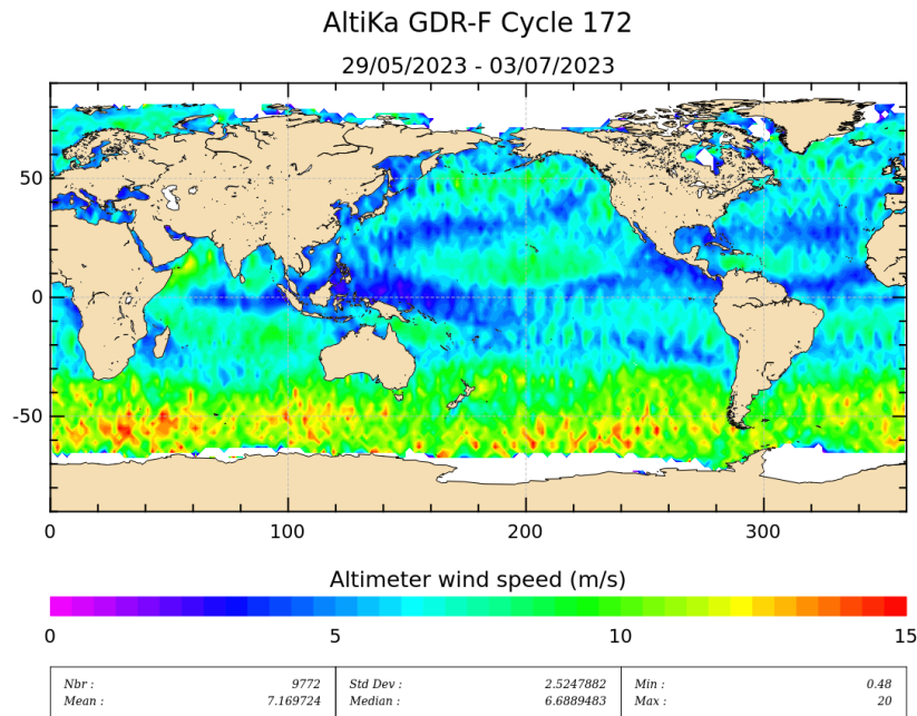
Figure 9: Altimeter wind speed for cycle 172.
