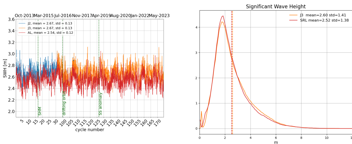
Figure 6: Daily monitoring of significant wave height for AltiKa (Ka-band) Jason-2 and Jason-3 (Ku-band) on the left and histogram for cycle 174 on the right (limited to 66^\circ latitude).
