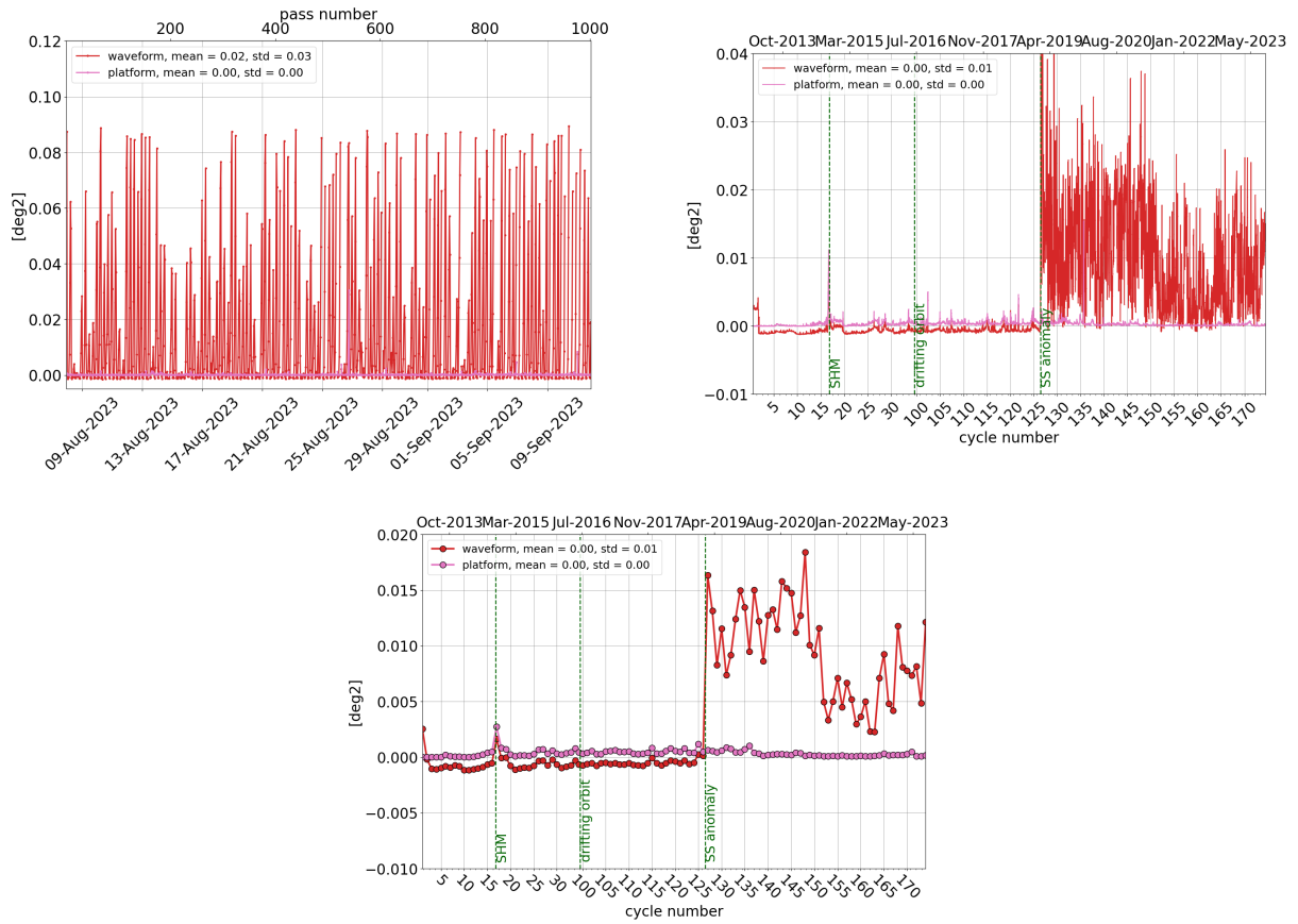
Figure 13: Monitoring per pass for cycle 174 (left), daily monitoring(right) and cyclic monitoring (bottom) of SARAL/AltiKa's mispointing angle: comparison between the one derived from waveform retracking and the one measured by platform startrackers.
