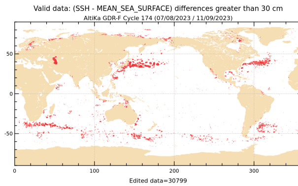
Figure 20: SLA higher than 30 cm for cycle 174.
