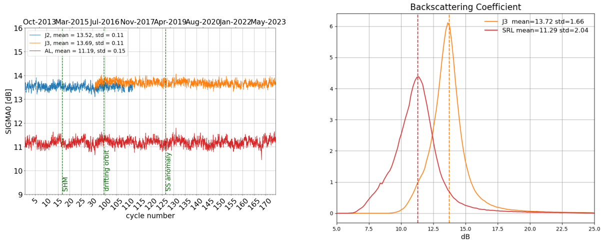
Figure 7: Daily monitoring of backscattering coefficient for Saral/AltiKa, Jason-2 and Jason-3 on the left and histogram for cycle 174 on the right (limited to 66° latitude).
