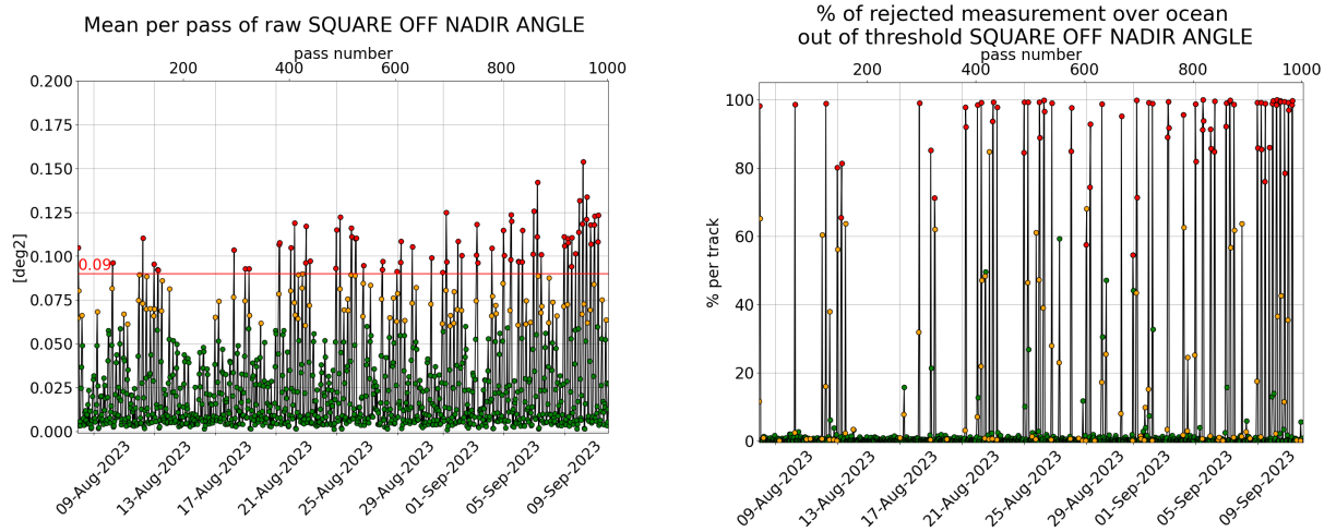
Figure 3: [left] Mispointing cycle 174, [right] Percentage of rejected measurement by threshold on square off-nadir angle.
