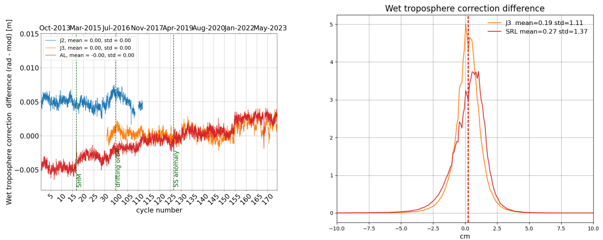
Figure 12: Daily monitoring of wet troposphere differences (Radiometer-ECMWF model) for Saral/AltiKa Jason-2 and Jason-3 (left) and histogram on the right (limited to 66° latitude) for cycle 174 .
