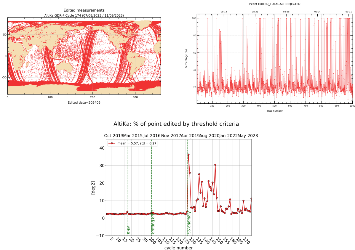
Figure 2: Rejected measurements on thresholds criteria : Cycle 174, map and monitoring of % of rejected measurements per track (top), whole time serie / % of rejected measurements per cycle (bottom).
