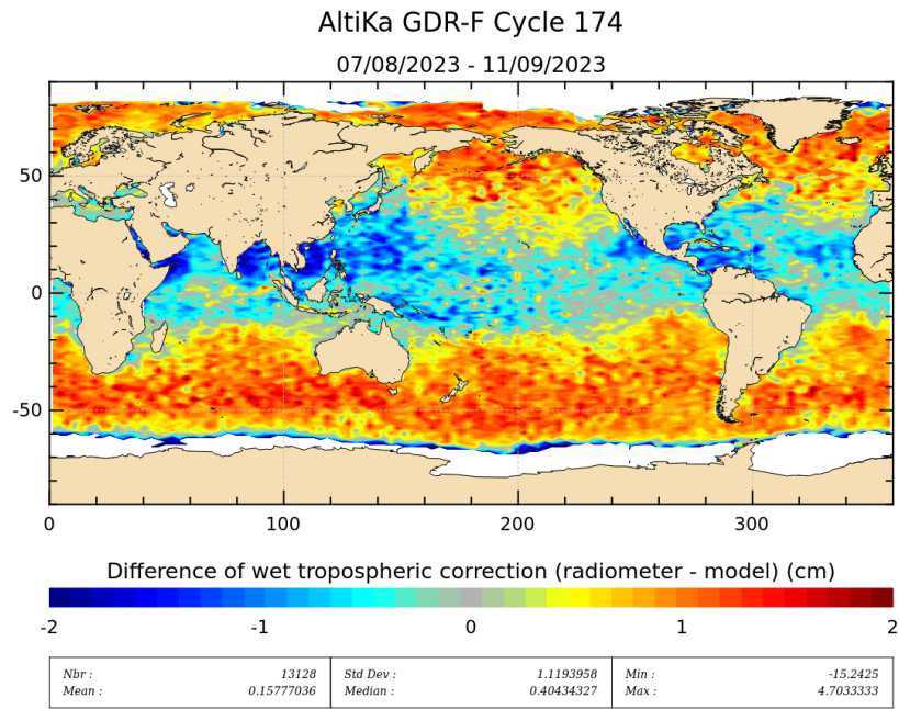
Figure 11: Mean of wet troposphere correction difference (Radiometer-ECMWF model) for cycle 174.
