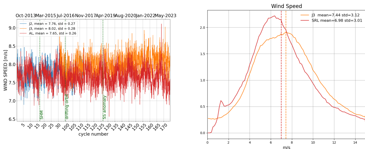
Figure 10: Daily monitoring of altimeter wind speed for Saral/AltiKa, Jason-2 and Jason-3 on the left and histogram for cycle 174 on the right (limited to 66° latitude).
