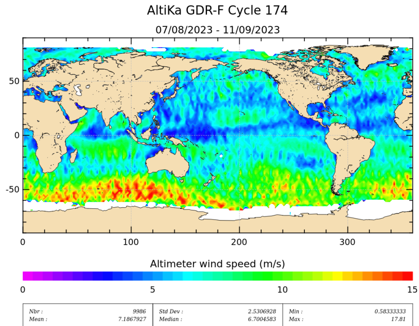
Figure 9: Altimeter wind speed for cycle 174.
