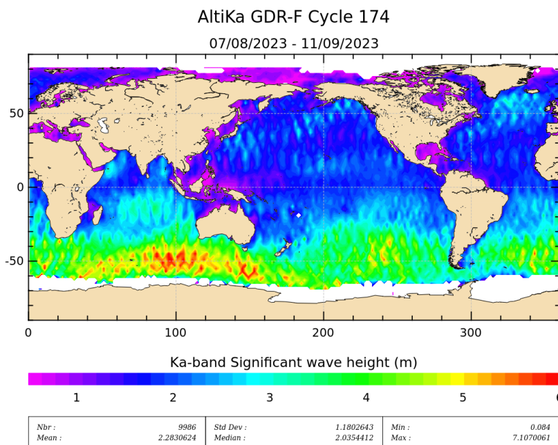
Figure 5: Significant wave height for cycle 174.
