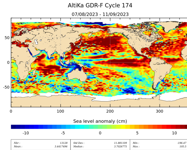
Figure 19: Sea level anomaly relative to MSS for cycle 174.
