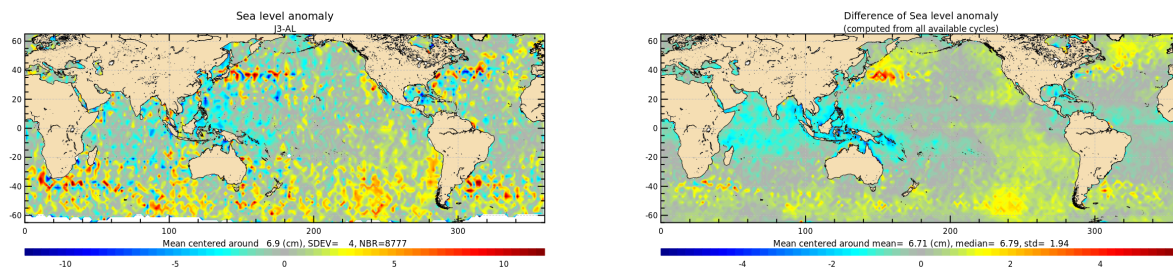
Figure 21: Jason-3 – Saral/AltiKa SLA differences for cycle 174 (left) and averaged over the whole Saral/AltiKa period (right).
