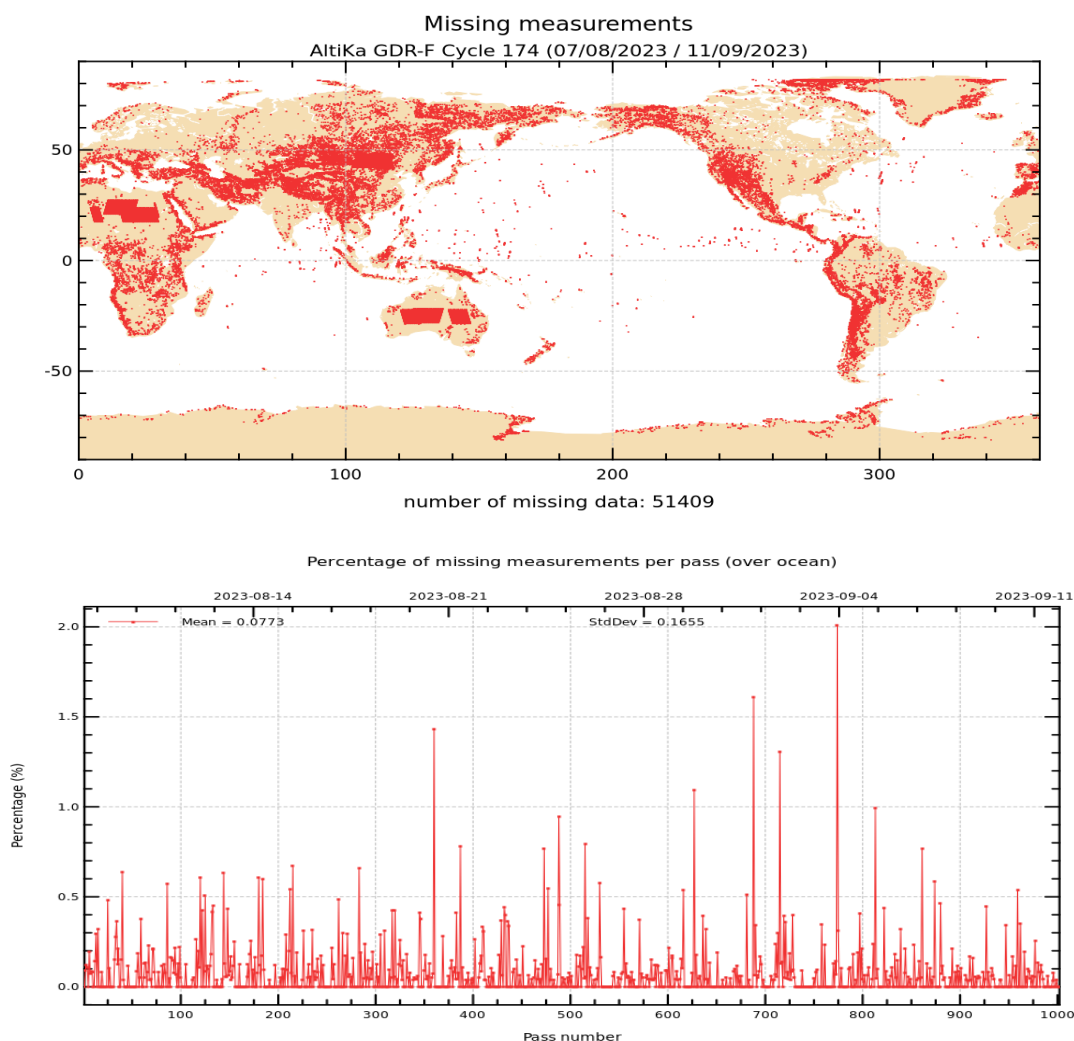
Figure 1: Map of missing measurements for cycle 174 on top. Monitoring of percentage of missing ocean measurements per pass on bottom.
