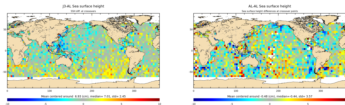
Figure 14: Mean of multi-mission SSH and mono-mission SSH differences at crossovers for cycle 174.
