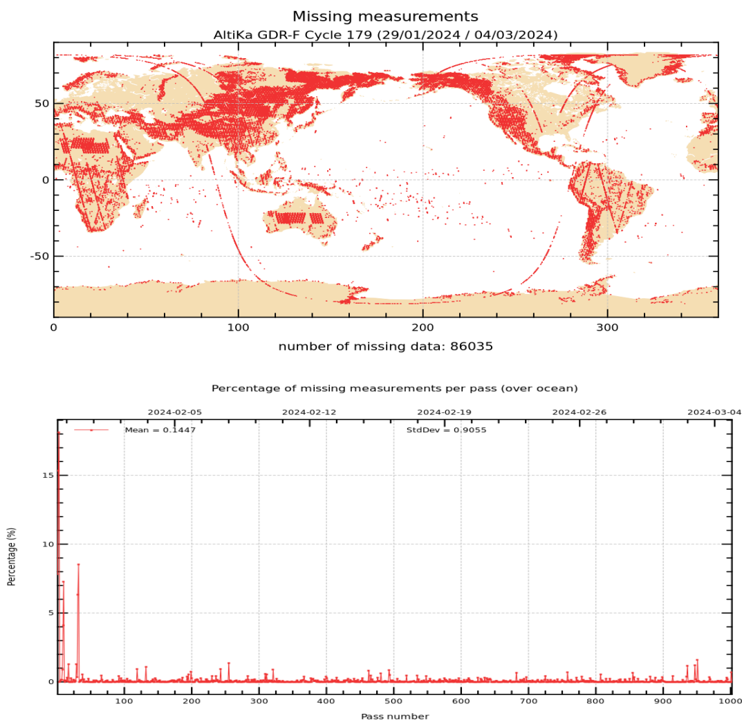
Figure 1: Map of missing measurements for cycle 179 on top. Monitoring of percentage of missing ocean measurements per pass on bottom.
