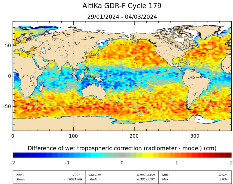
Figure 11: Mean of wet troposphere correction difference (Radiometer-ECMWF model) for cycle 179.
