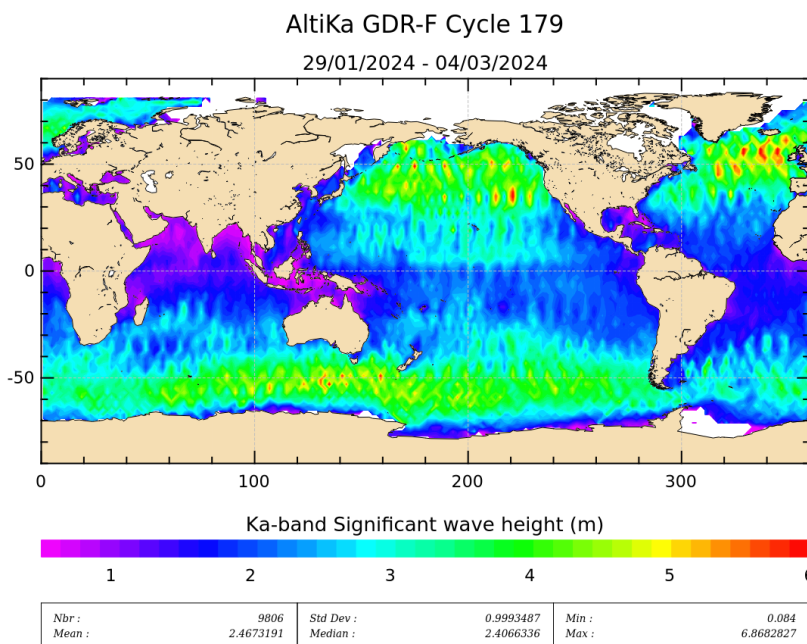
Figure 5: Significant wave height for cycle 179.
