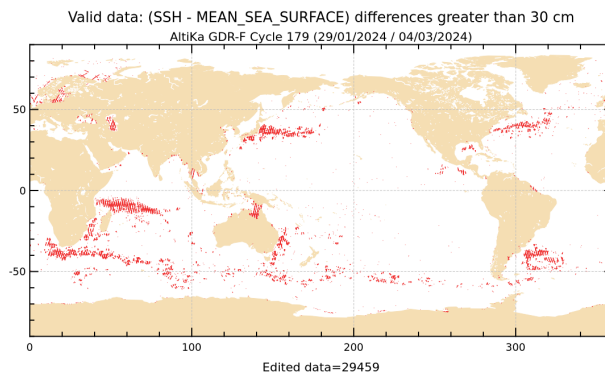
Figure 20: SLA higher than 30 cm for cycle 179.
