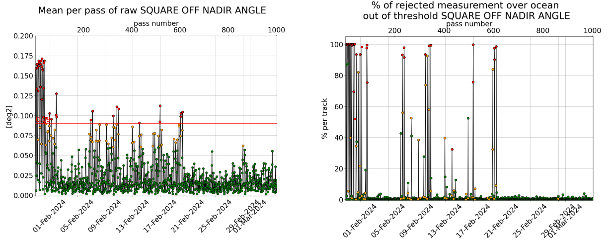
Figure 3: [left] Mispointing cycle 179, [right] Percentage of rejected measurement by threshold on square off-nadir angle.
