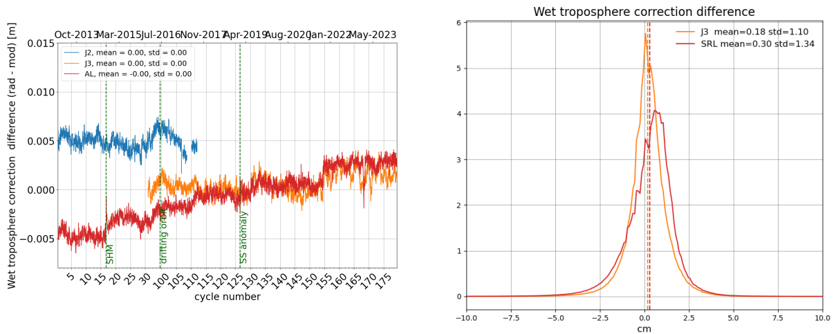
Figure 12: Daily monitoring of wet troposphere differences (Radiometer-ECMWF model) for Saral/AltiKa Jason-2 and Jason-3 (left) and histogram on the right (limited to 66° latitude) for cycle 179 .
