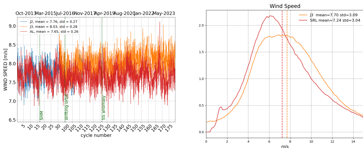
Figure 10: Daily monitoring of altimeter wind speed for Saral/AltiKa, Jason-2 and Jason-3 on the left and histogram for cycle 179 on the right (limited to 66° latitude).
