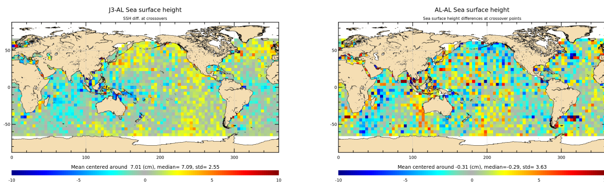
Figure 14: Mean of multi-mission SSH and mono-mission SSH differences at crossovers for cycle 179.
