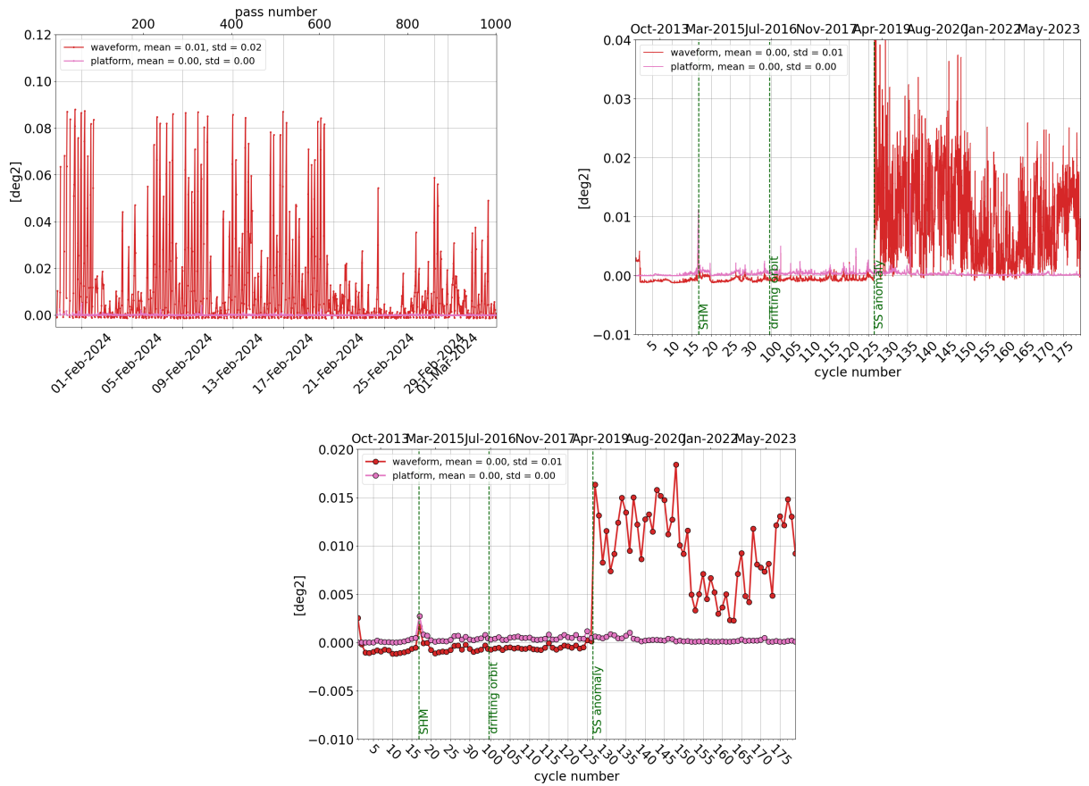
Figure 13: Monitoring per pass for cycle 179 (left), daily monitoring (right) and cyclic monitoring (bottom) of SARAL/AltiKa's mispointing angle: comparison between the one derived from waveform retracking and the one measured by platform startrackers.
