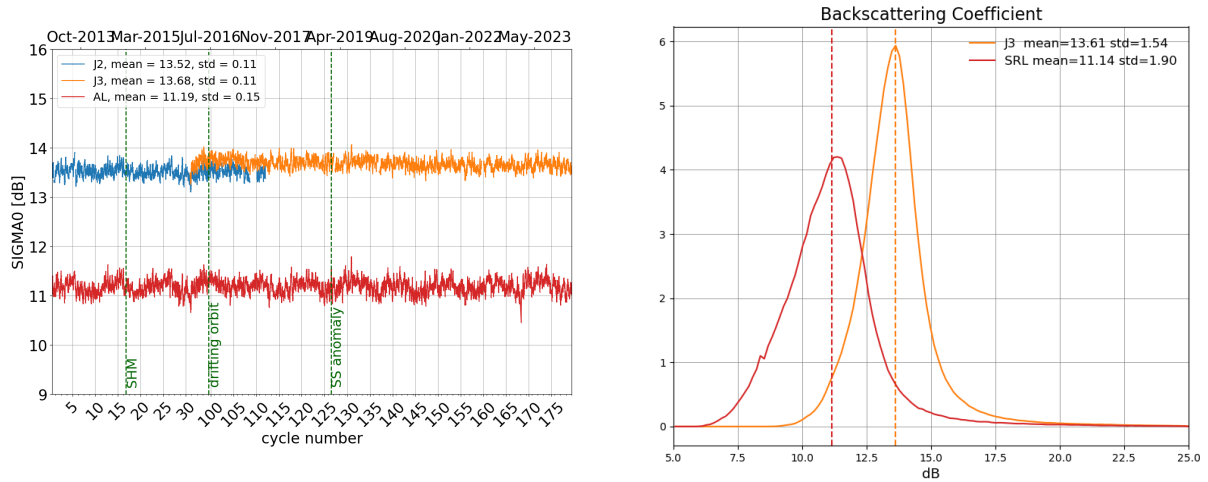
Figure 7: Daily monitoring of backscattering coefficient for Saral/AltiKa, Jason-2 and Jason-3 on the left and histogram for cycle 179 on the right (limited to 66° latitude).
