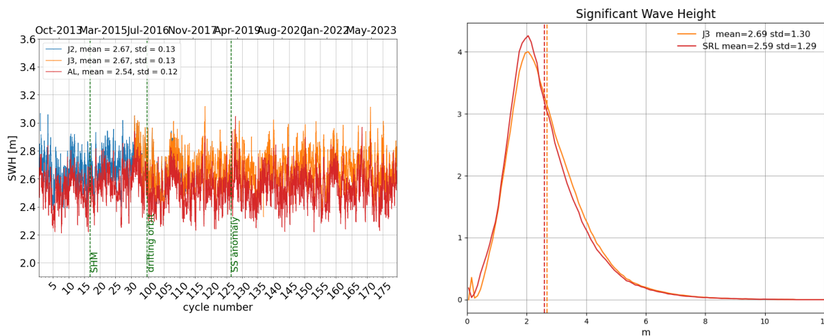
Figure 6: Daily monitoring of significant wave height for AltiKa (Ka-band) Jason-2 and Jason-3 (Ku-band) on the left and histogram for cycle 179 on the right (limited to 66^\circ latitude).
