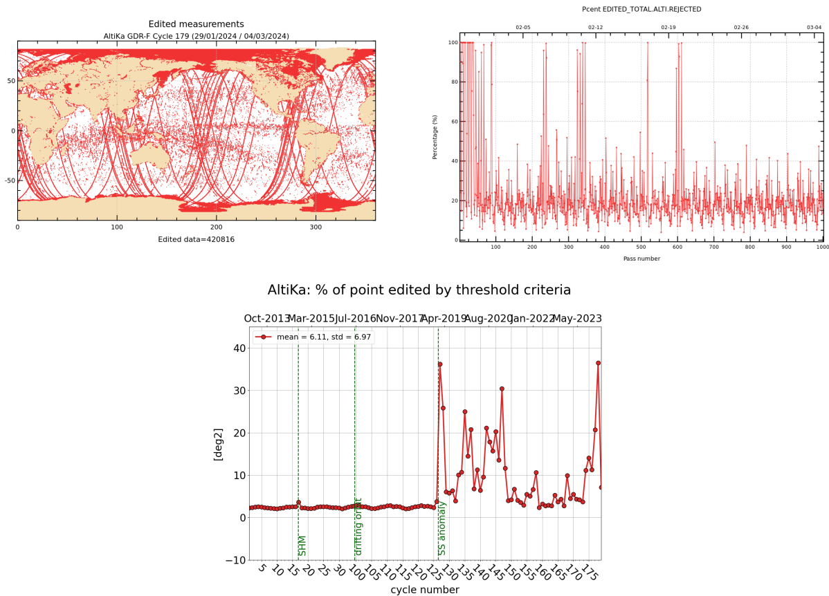
Figure 2: Rejected measurements on thresholds criteria : Cycle 179, map and monitoring of % of rejected measurements per track (top), whole time serie / % of rejected measurements per cycle (bottom).
