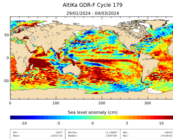
Figure 19: Sea level anomaly relative to MSS for cycle 179.
