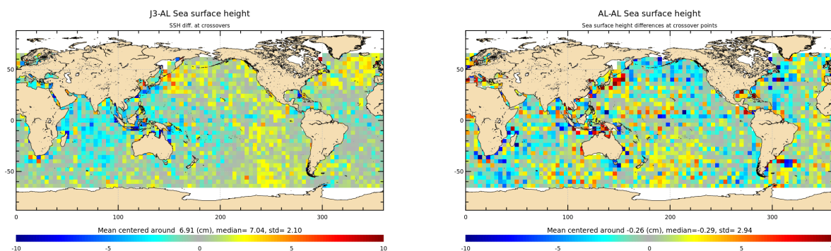
Figure 14: Mean of multi-mission SSH and mono-mission SSH differences at crossovers for cycle 180.
