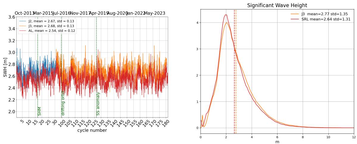
Figure 6: Daily monitoring of significant wave height for AltiKa (Ka-band) Jason-2 and Jason-3 (Ku-band) on the left and histogram for cycle 180 on the right (limited to 66^\circ latitude).
