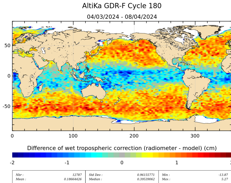
Figure 11: Mean of wet troposphere correction difference (Radiometer-ECMWF model) for cycle 180.
