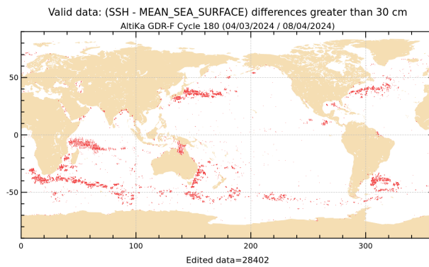
Figure 20: SLA higher than 30 cm for cycle 180.
