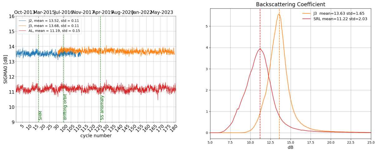
Figure 7: Daily monitoring of backscattering coefficient for Saral/AltiKa, Jason-2 and Jason-3 on the left and histogram for cycle 180 on the right (limited to 66° latitude).
