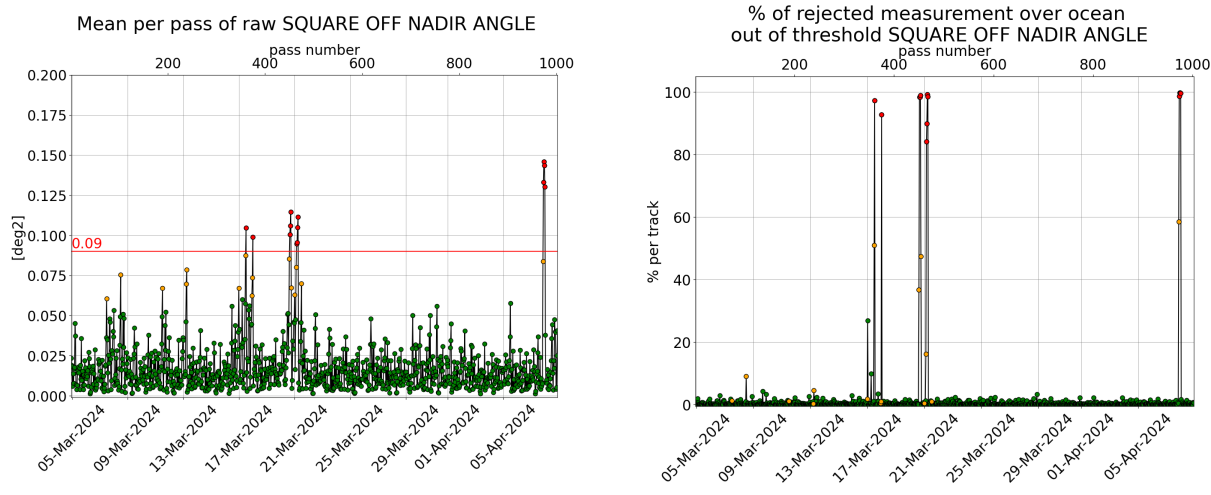
Figure 3: [left] Mispointing cycle 180, [right] Percentage of rejected measurement by threshold on square off-nadir angle.
