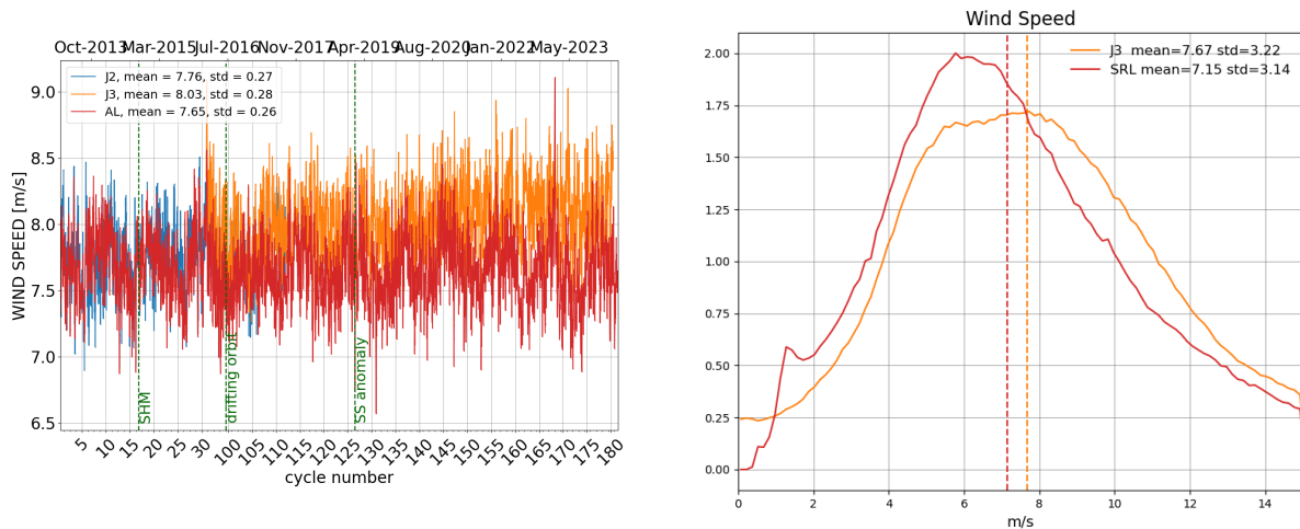
Figure 10: Daily monitoring of altimeter wind speed for Saral/AltiKa, Jason-2 and Jason-3 on the left and histogram for cycle 180 on the right (limited to 66° latitude).
