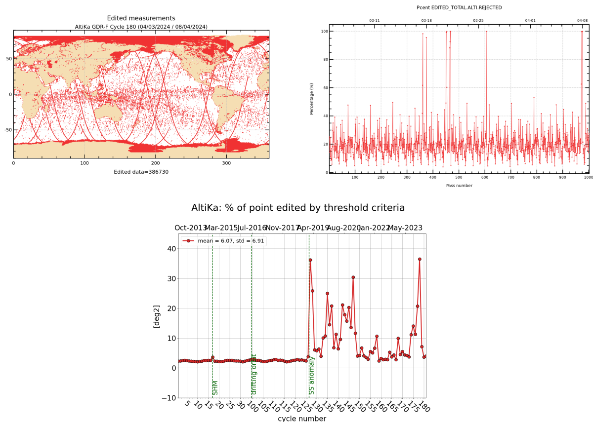
Figure 2: Rejected measurements on thresholds criteria : Cycle 180, map and monitoring of % of rejected measurements per track (top), whole time serie / % of rejected measurements per cycle (bottom).
