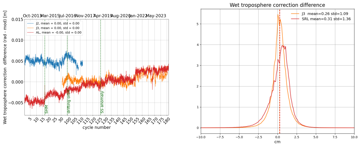
Figure 12: Daily monitoring of wet troposphere differences (Radiometer-ECMWF model) for Saral/AltiKa Jason-2 and Jason-3 (left) and histogram on the right (limited to 66° latitude) for cycle 180 .
