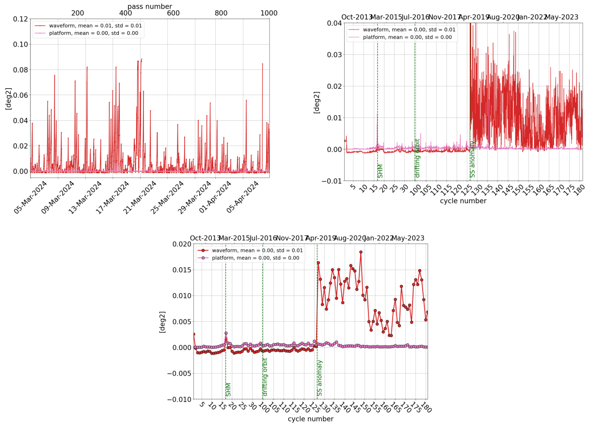
Figure 13: Monitoring per pass for cycle 180 (left), daily monitoring(right) and cyclic monitoring (bottom) of SARAL/AltiKa's mispointing angle: comparison between the one derived from waveform retracking and the one measured by platform startrackers.
