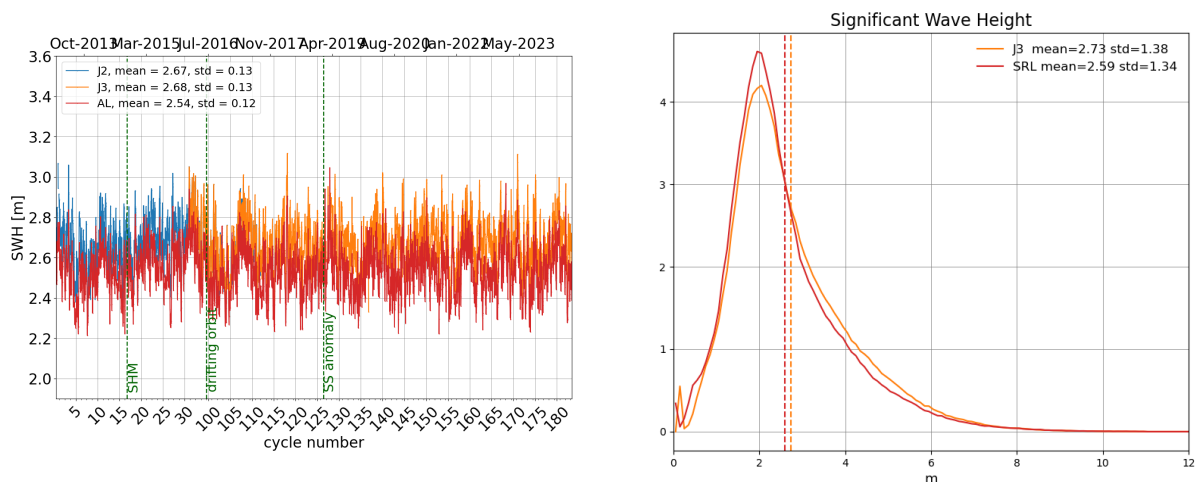
Figure 6: Daily monitoring of significant wave height for AltiKa (Ka-band) Jason-2 and Jason-3 (Ku-band) on the left and histogram for cycle 181 on the right (limited to 66^\circ latitude).
