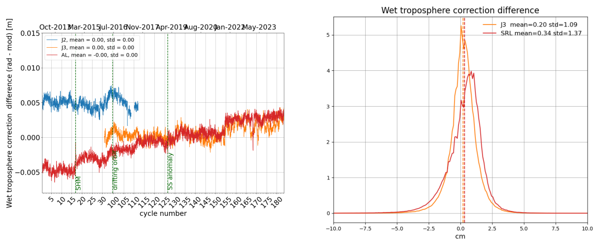
Figure 12: Daily monitoring of wet troposphere differences (Radiometer-ECMWF model) for Saral/AltiKa Jason-2 and Jason-3 (left) and histogram on the right (limited to 66° latitude) for cycle 181 .
