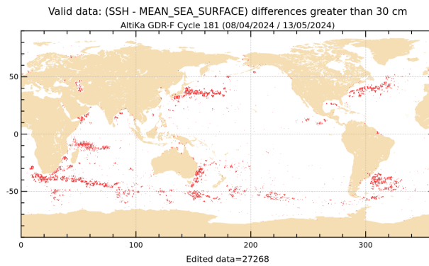
Figure 20: SLA higher than 30 cm for cycle 181.
