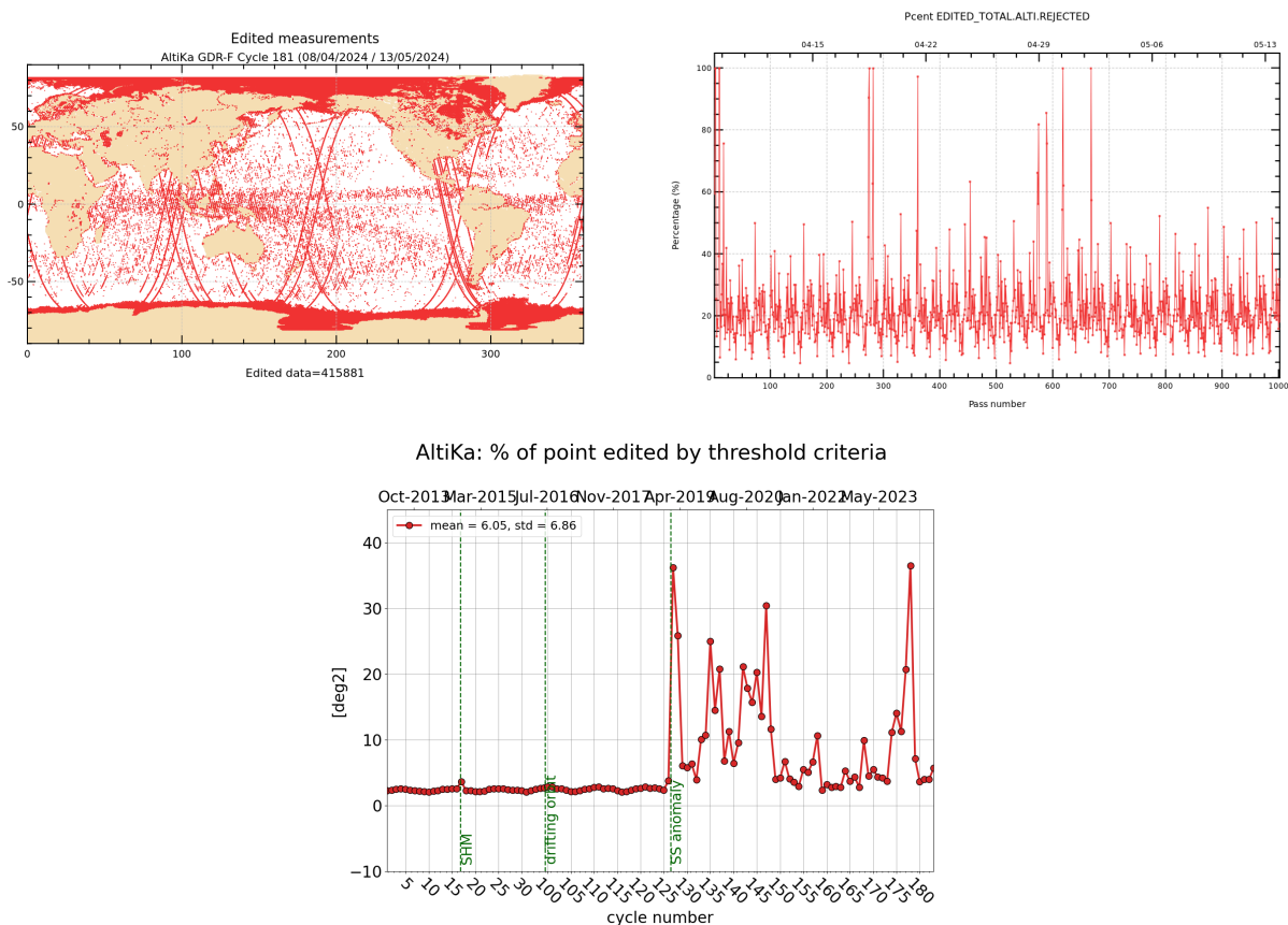
Figure 2: Rejected measurements on thresholds criteria : Cycle 181, map and monitoring of % of rejected measurements per track (top), whole time serie / % of rejected measurements per cycle (bottom).
