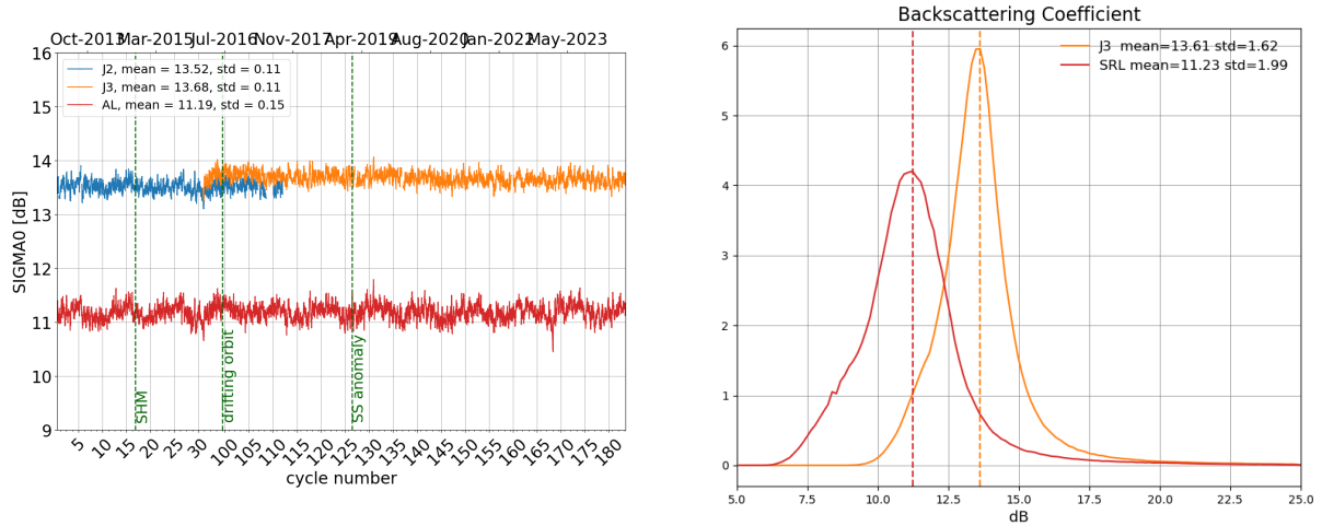
Figure 7: Daily monitoring of backscattering coefficient for Saral/AltiKa, Jason-2 and Jason-3 on the left and histogram for cycle 181 on the right (limited to 66° latitude).
