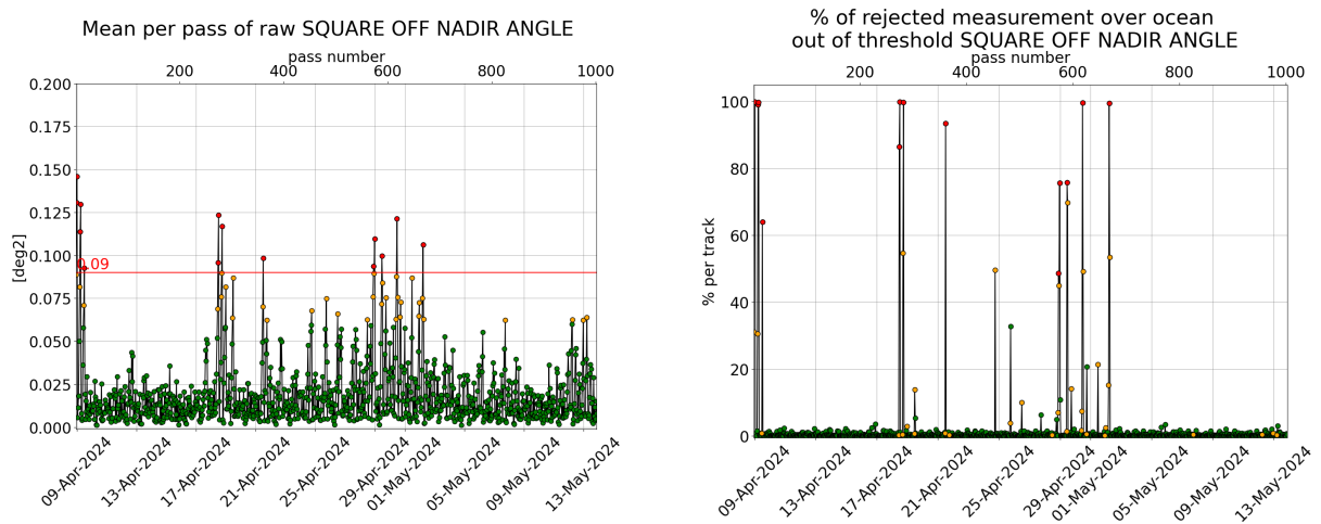
Figure 3: [left] Mispointing cycle 181, [right] Percentage of rejected measurement by threshold on square off-nadir angle.
