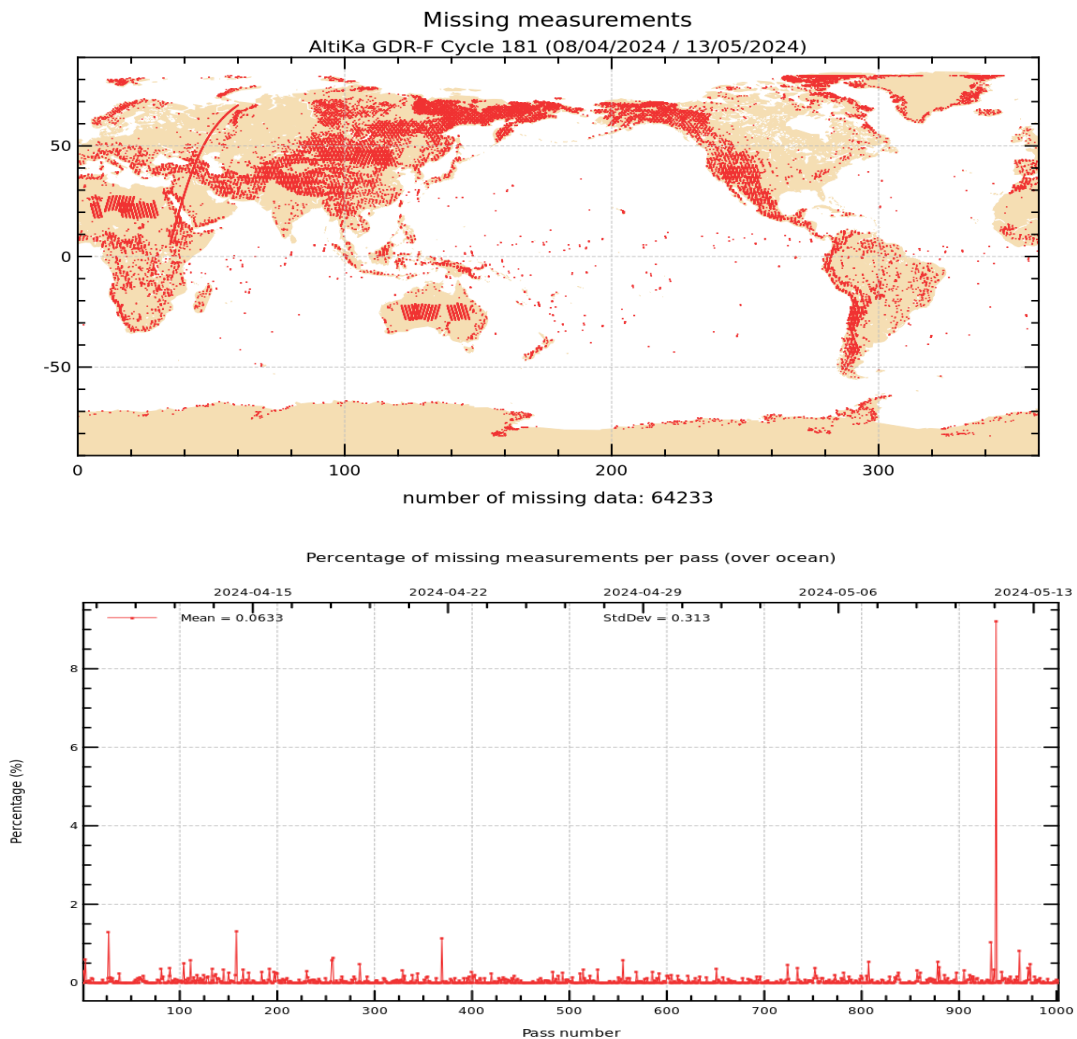
Figure 1: Map of missing measurements for cycle 181 on top. Monitoring of percentage of missing ocean measurements per pass on bottom.
