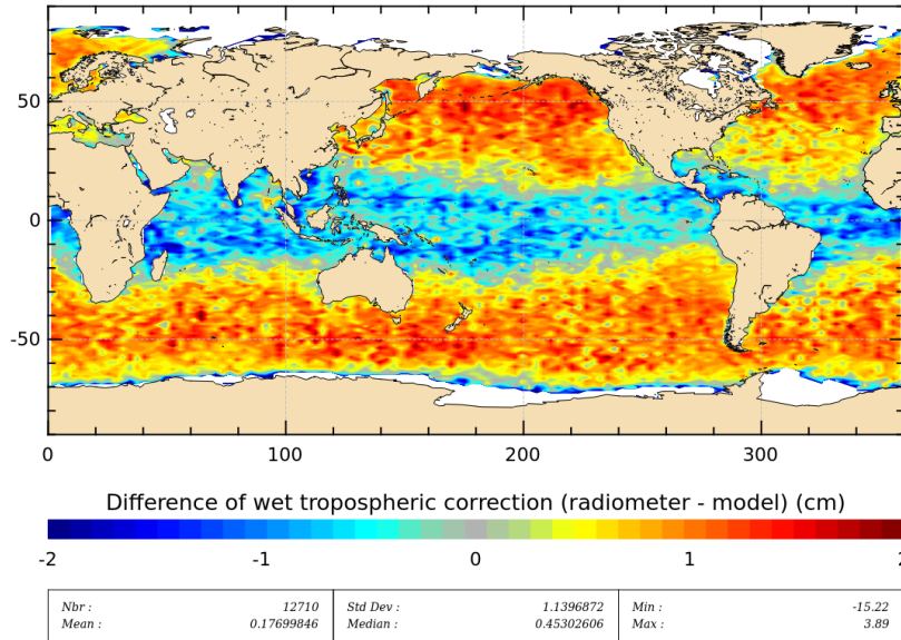
Figure 11: Mean of wet troposphere correction difference (Radiometer-ECMWF model) for cycle 181.
