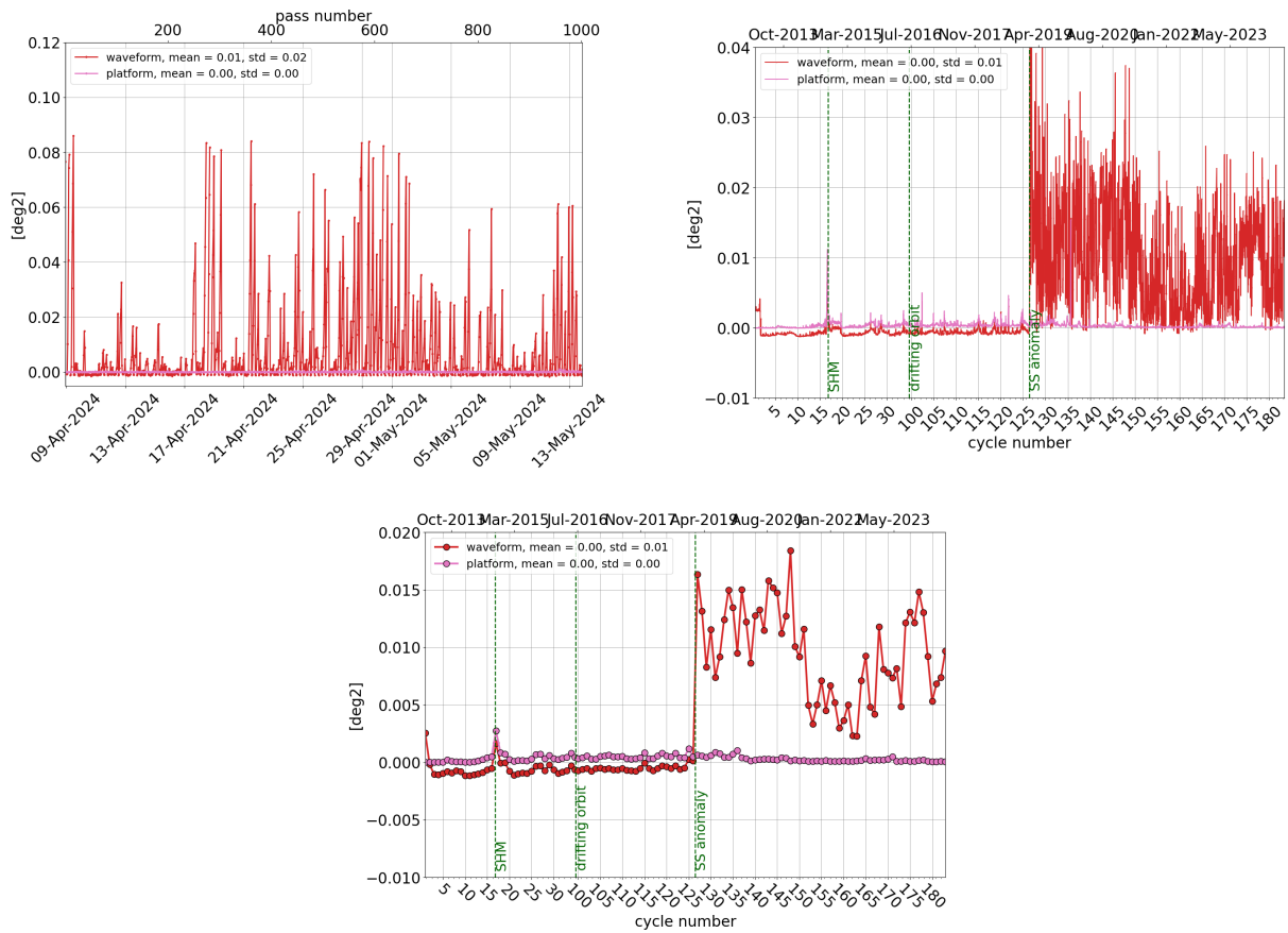
Figure 13: Monitoring per pass for cycle 181 (left), daily monitoring(right) and cyclic monitoring (bottom) of SARAL/AltiKa's mispointing angle: comparison between the one derived from waveform retracking and the one measured by platform startrackers.
