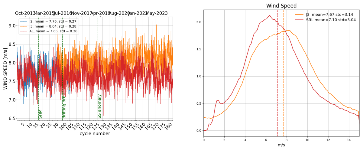
Figure 10: Daily monitoring of altimeter wind speed for Saral/AltiKa, Jason-2 and Jason-3 on the left and histogram for cycle 181 on the right (limited to 66° latitude).
