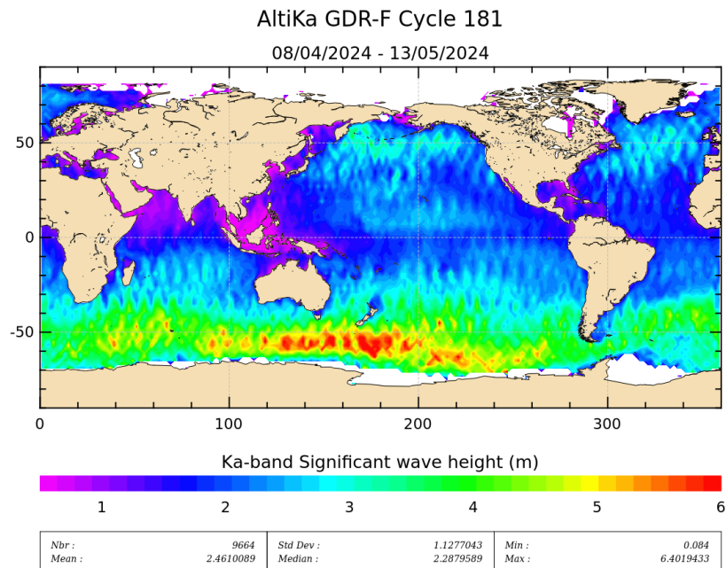
Figure 5: Significant wave height for cycle 181.
