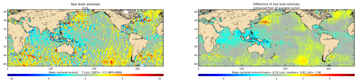
Figure 21: Jason-3 – Saral/AltiKa SLA differences for cycle 181 (left) and averaged over the whole Saral/AltiKa period (right).
