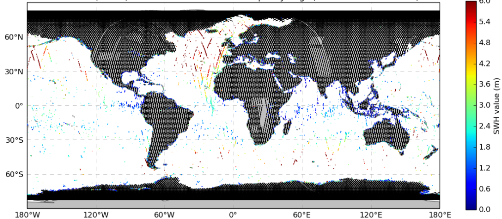
SWH_nsec (colors) edited from thresholds and quality flags (Black = default Values)
