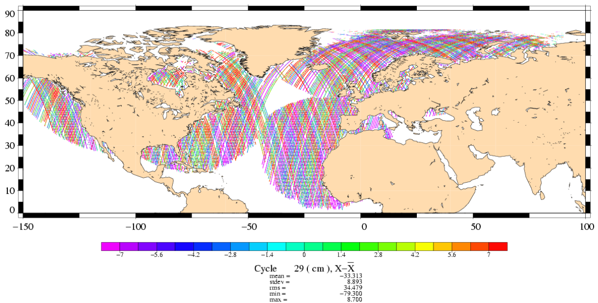
Corrected SLA (GIM iono, ECMWF (gaussian) wet tropo configuration) ERS-2 (Cycle 097) – Envisat (Cycle 029)
