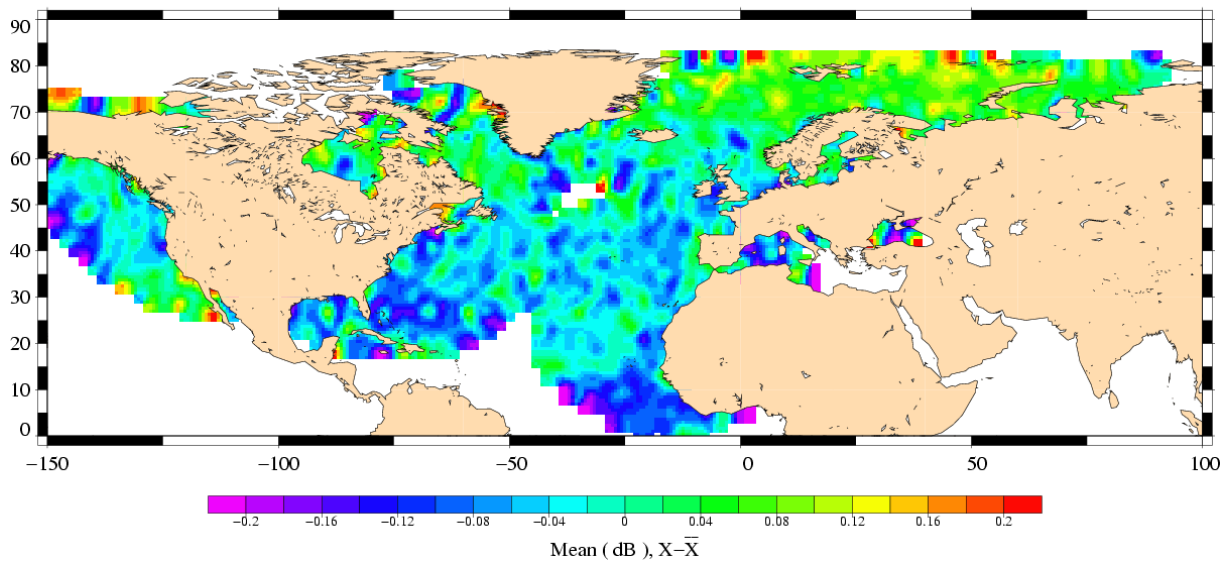
Sigma0 differences ERS-2 (Cycle 097) – Envisat (Cycle 029)
