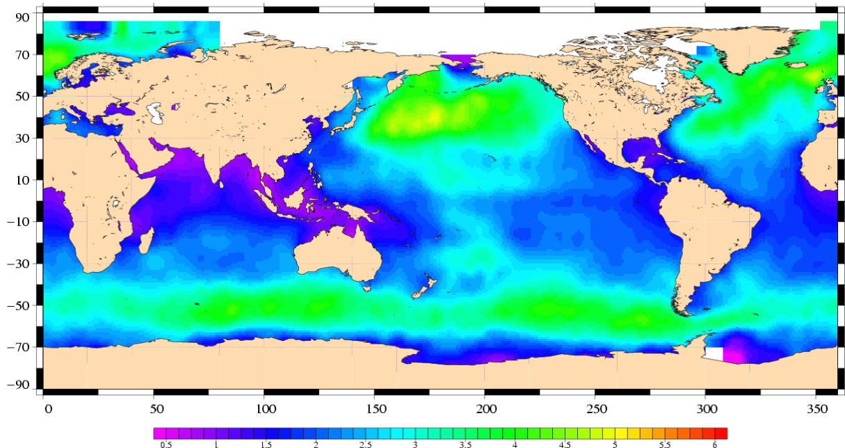
Significant Wave Height (m) Envisat Cycle 034 17/01/2005 – 21/02/2005
