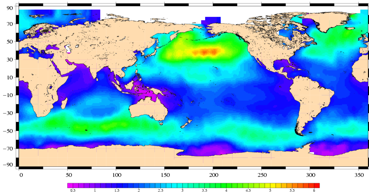
Significant Wave Height (m) Envisat Cycle 043 28/11/2005 – 02/01/2006
