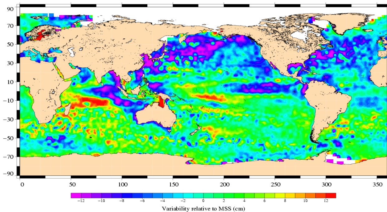
Envisat Cycle 055 22/01/2007 – 26/02/2007
