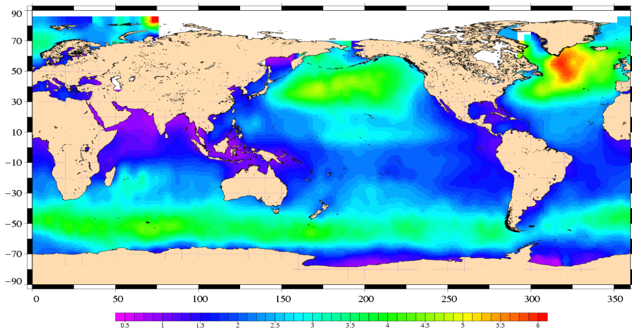
Significant Wave Height (m) Envisat Cycle 055 22/01/2007 – 26/02/2007
