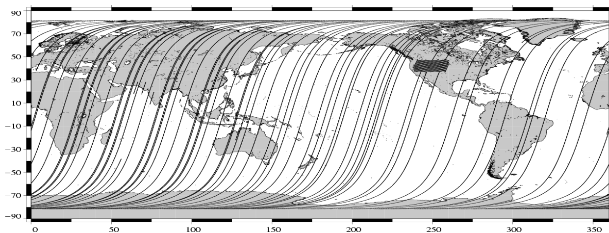
Missing measurements (Descending passes) Envisat Cycle 056 (26/02/2007 / 02/04/2007)
