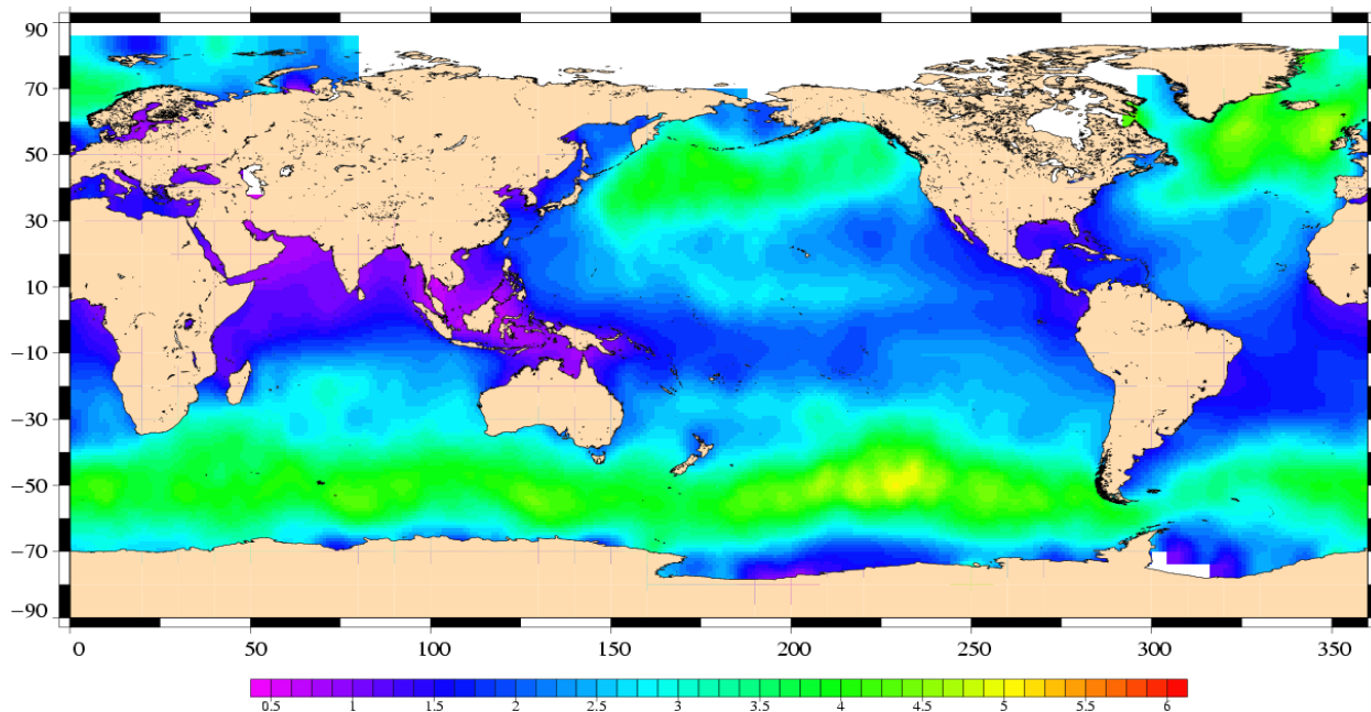
Significant Wave Height (m) Envisat Cycle 056 26/02/2007 – 02/04/2007
