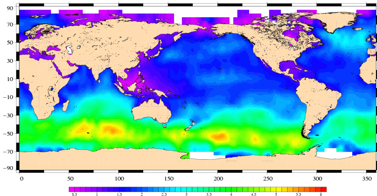
Significant Wave Height (m) Envisat Cycle 058 07/05/2007 – 11/06/2007
