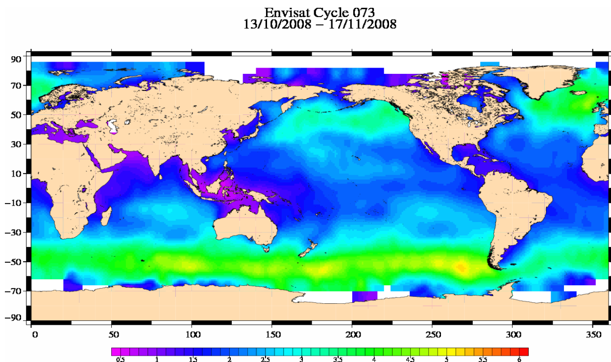
Significant Wave Height (m) Envisat Cycle 073 13/10/2008 – 17/11/2008
