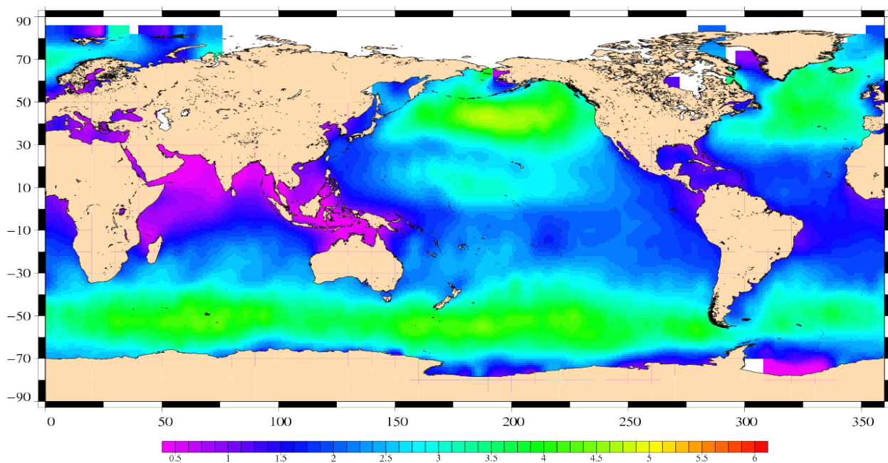
Significant Wave Height (m) Envisat Cycle 087 15/02/2010 – 22/03/2010
