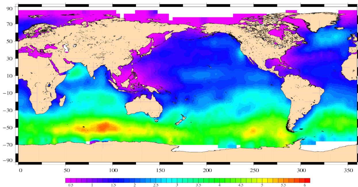
Significant Wave Height (m) Envisat Cycle 090 31/05/2010 – 05/07/2010
