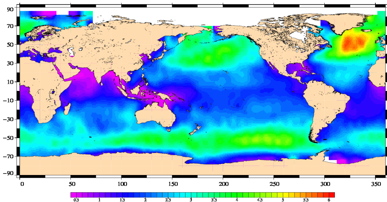
Significant Wave Height (m) Envisat Cycle 099 25/01/2011 – 24/02/2011
