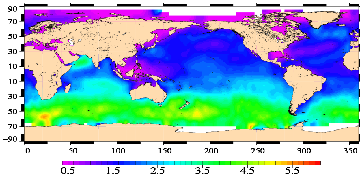
Significant Wave Height (m) Envisat Cycle 104 24/06/2011 – 24/07/2011
