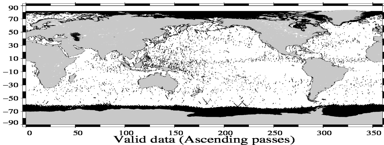
Valid data (Ascending passes) Envisat Cycle 104 (24/06/2011 / 24/07/2011)
