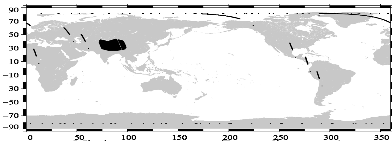
Missing measurements (Descending passes) Envisat Cycle 104 (24/06/2011 / 24/07/2011)
