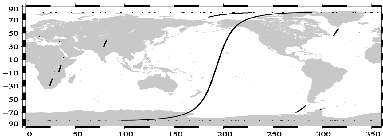
Missing measurements (Descending passes) Envisat Cycle 104 (24/06/2011 / 24/07/2011)
