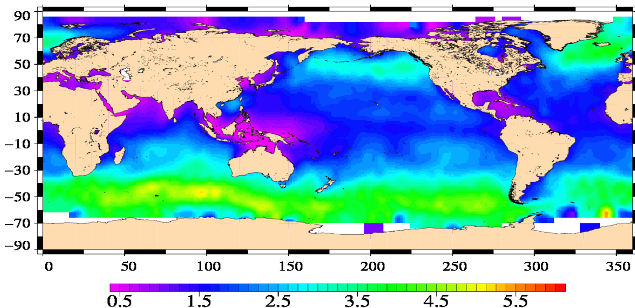
Significant Wave Height (m) Envisat Cycle 107 22/09/2011 – 22/10/2011
