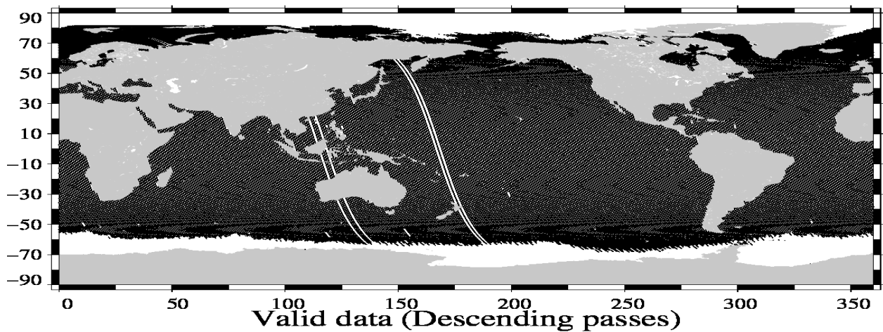
Valid data (Descending passes) Envisat Cycle 107 (22/09/2011 / 22/10/2011)
