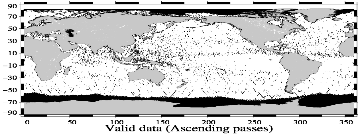
Valid data (Ascending passes) Envisat Cycle 107 (22/09/2011 / 22/10/2011)
