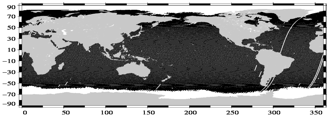
Valid data (Descending passes) Envisat Cycle 107 (22/09/2011 / 22/10/2011)
