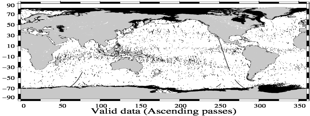
Valid data (Ascending passes) Envisat Cycle 111 (20/01/2012 / 19/02/2012)
