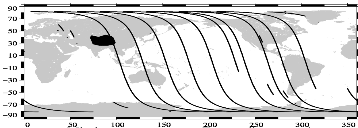
Missing measurements (Descending passes) Envisat Cycle 111 (20/01/2012 / 19/02/2012)
