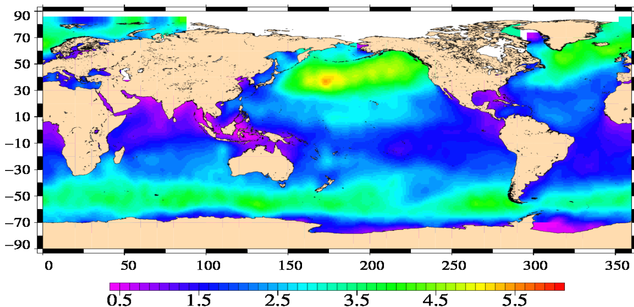
Significant Wave Height (m) Envisat Cycle 111 20/01/2012 – 19/02/2012
