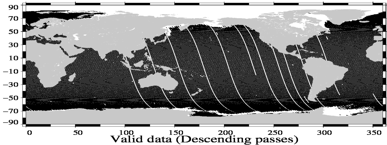
Valid data (Descending passes) Envisat Cycle 111 (20/01/2012 / 19/02/2012)
