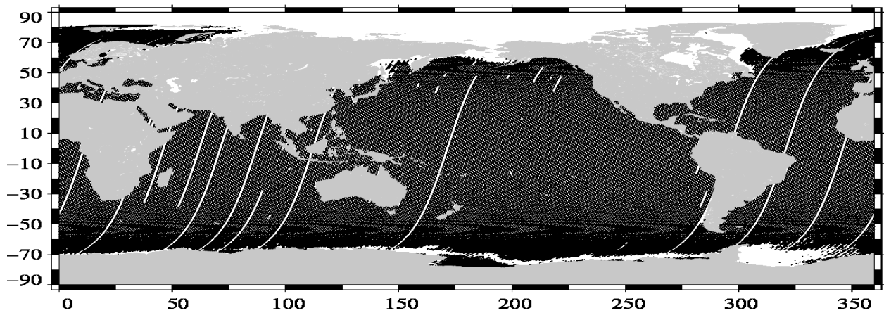
Valid data (Descending passes) Envisat Cycle 111 (20/01/2012 / 19/02/2012)
