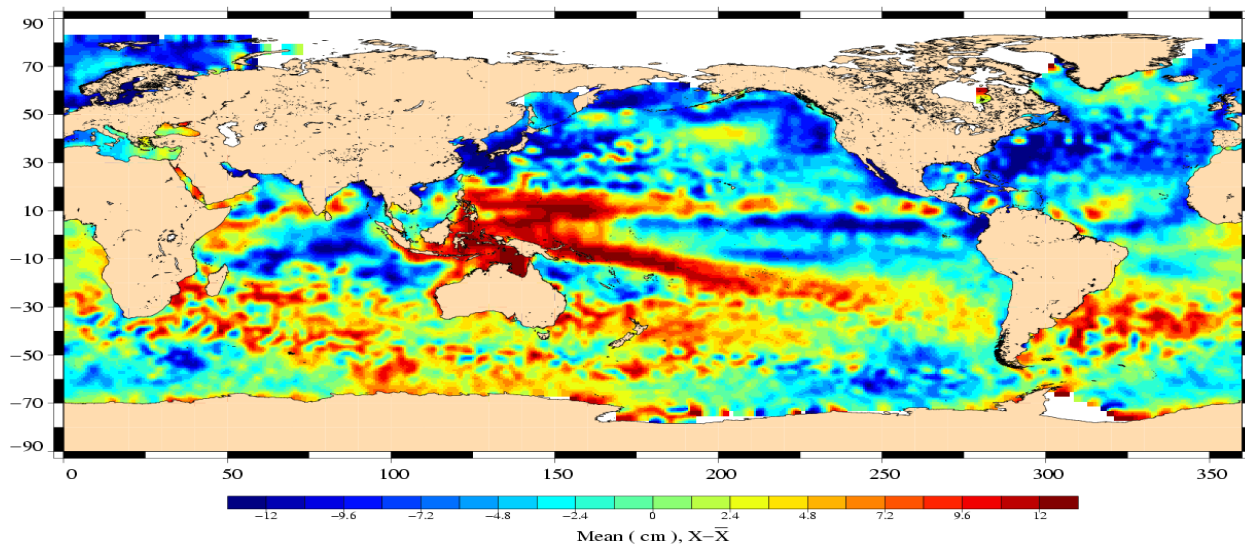
Variability relative to MSS (cm) Envisat Cycle 046 (13/03/2006 to 17/04/2006)
