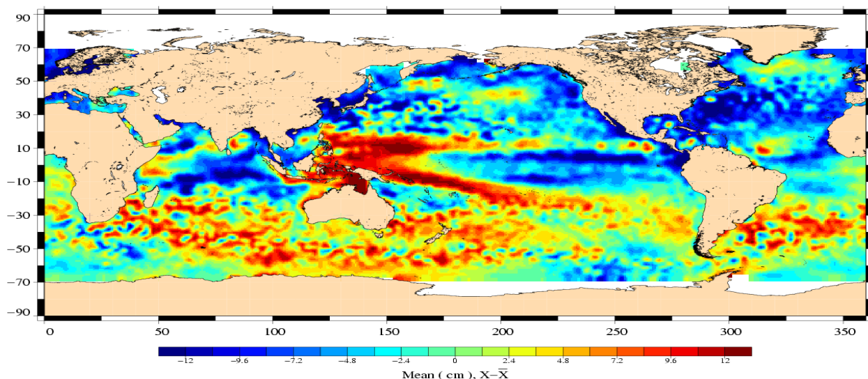
Variability relative to MSS (cm) Jason (13/03/2006 to 17/04/2006)
