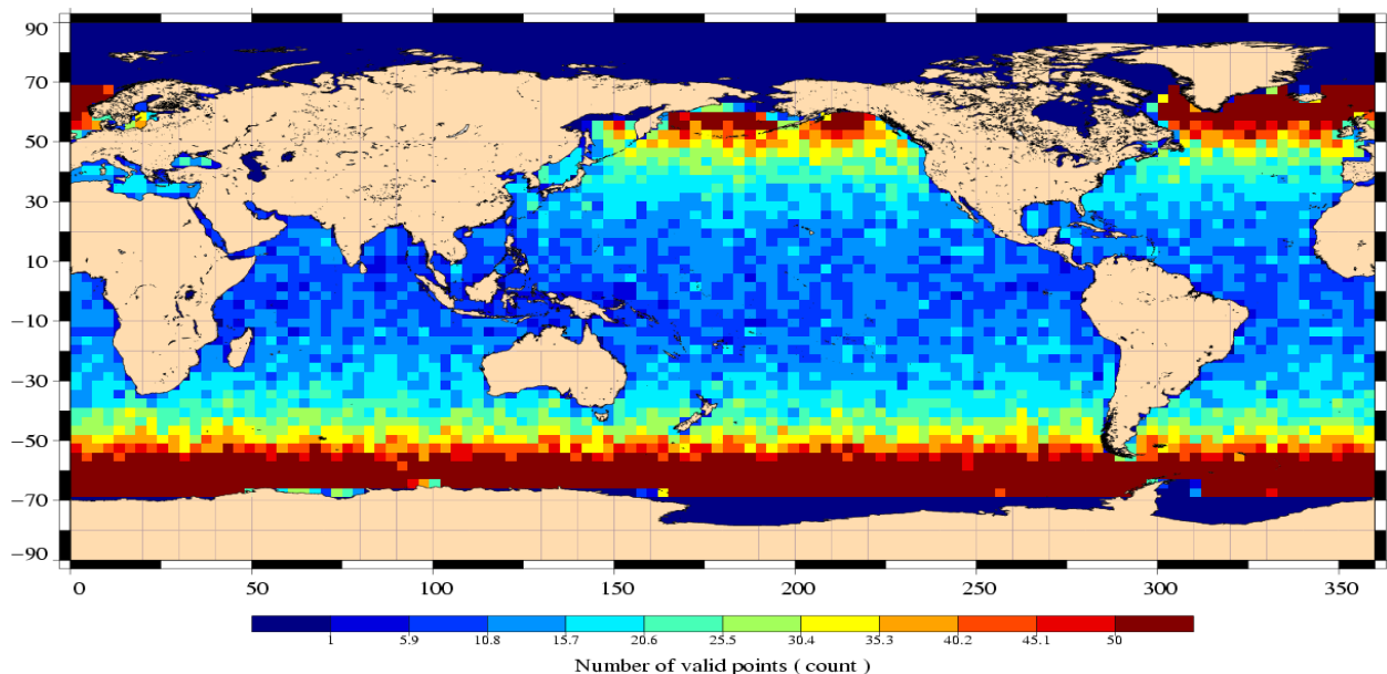
Number of Jason/Envisat 10 days cross-over points Cycle 046 (13/03/2006 – 17/04/2006)
